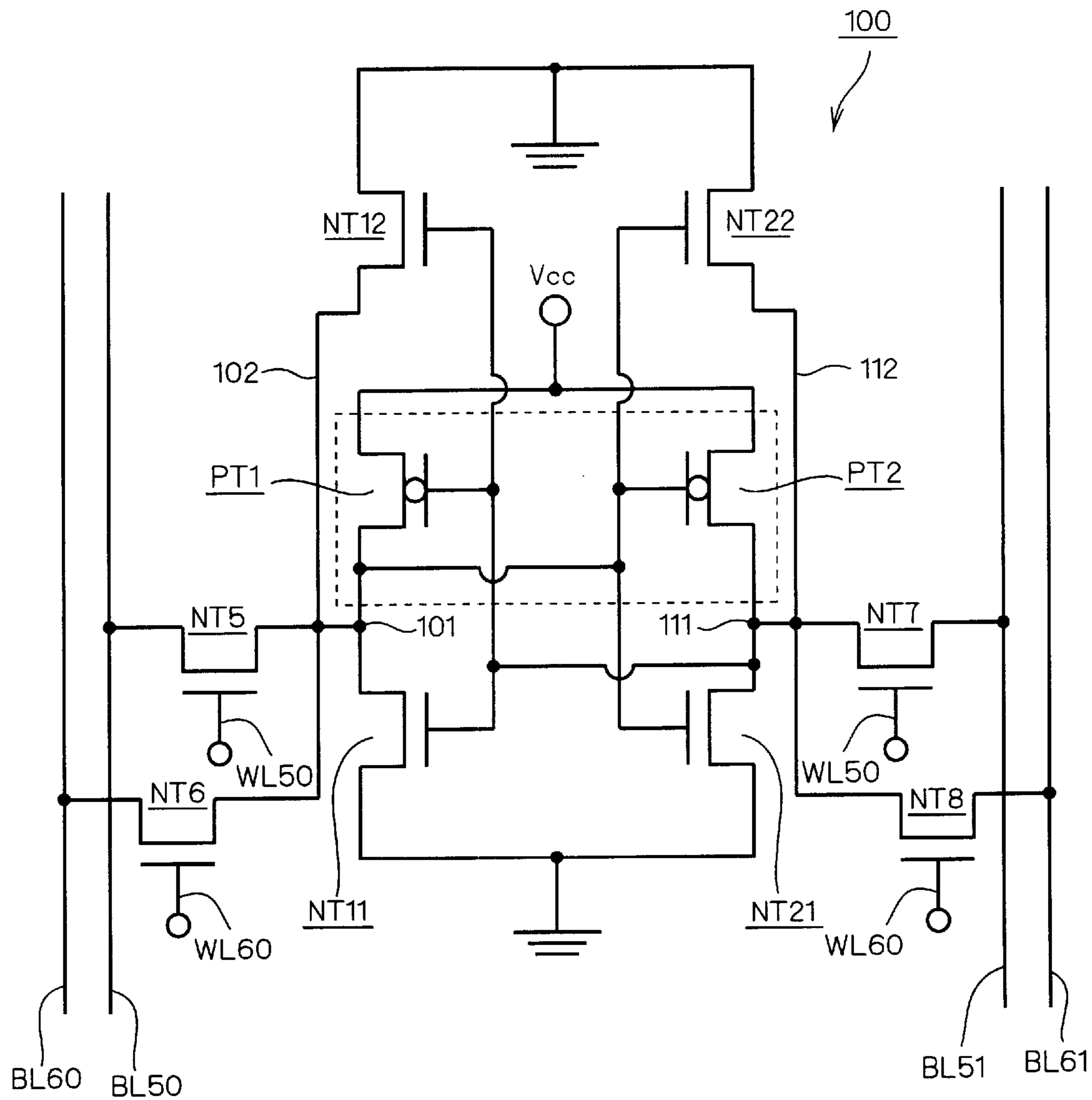
FIG. 37 PRIOR ART
