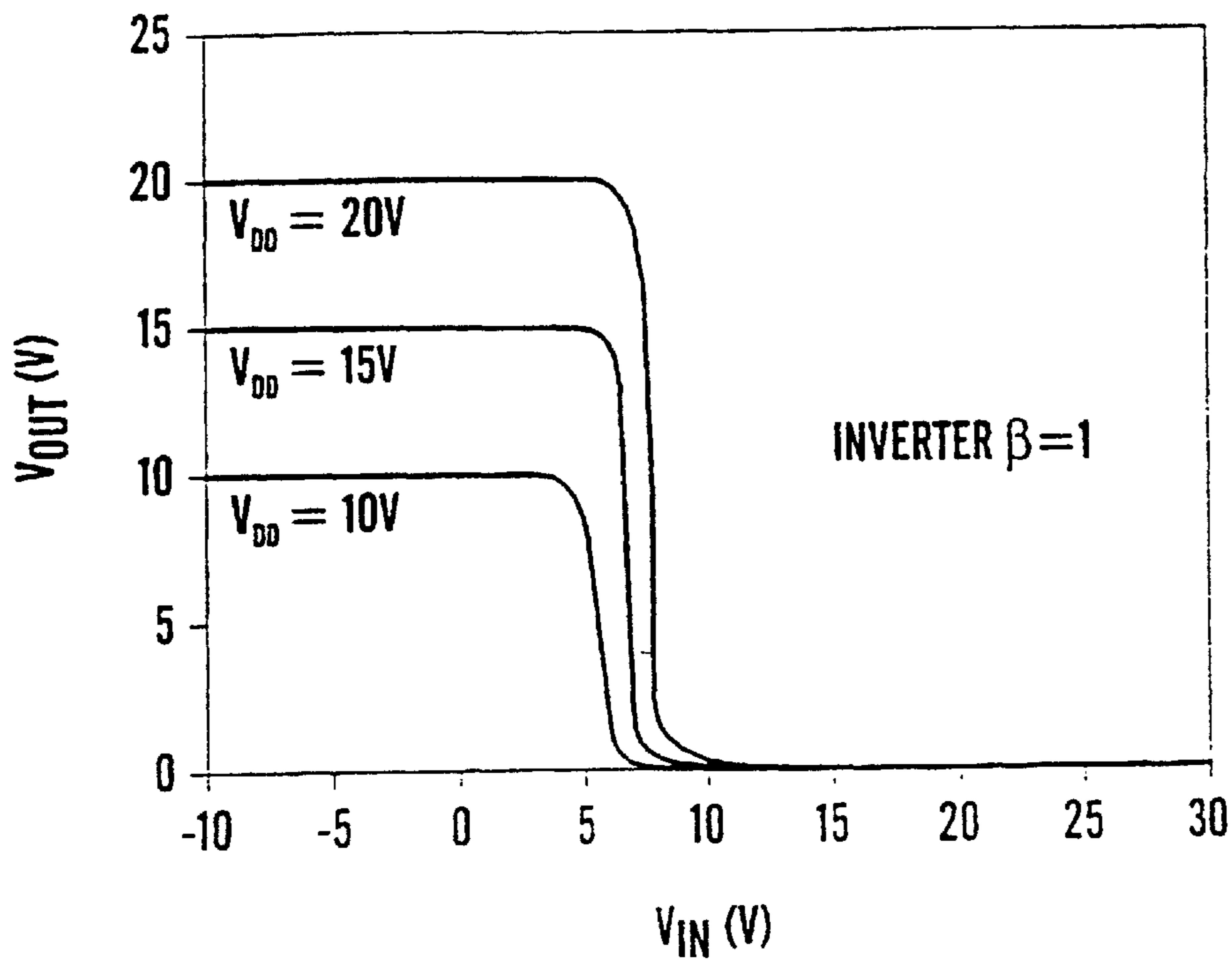
VOLTAGE TRANSFER CURVE OF a-Si:H / PENTACENE INVERTER
