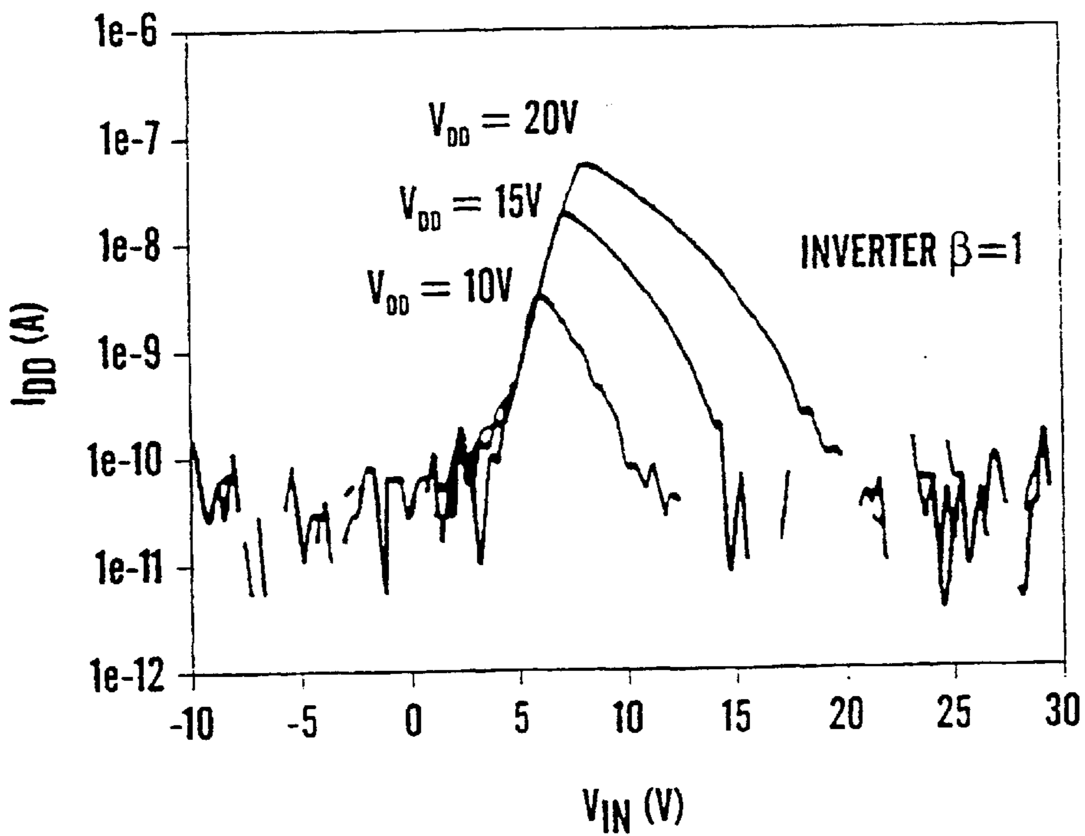
TRANSIENT CURRENT OF a-Si:H / PENTACENE INVERTER
