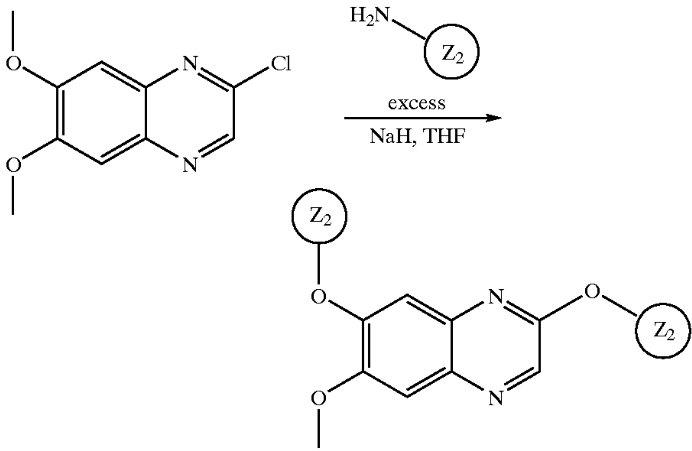
Scheme III
