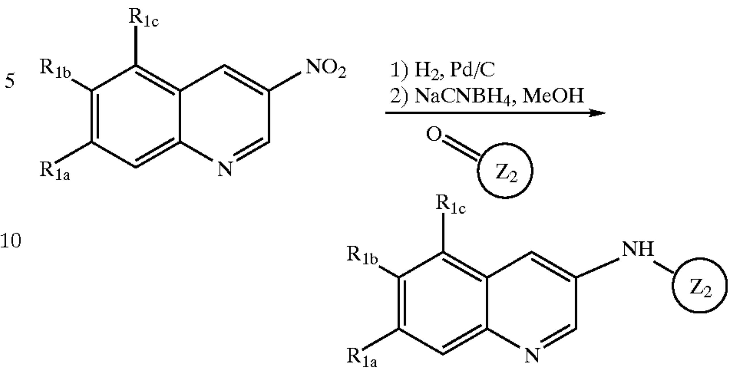
Scheme IV
