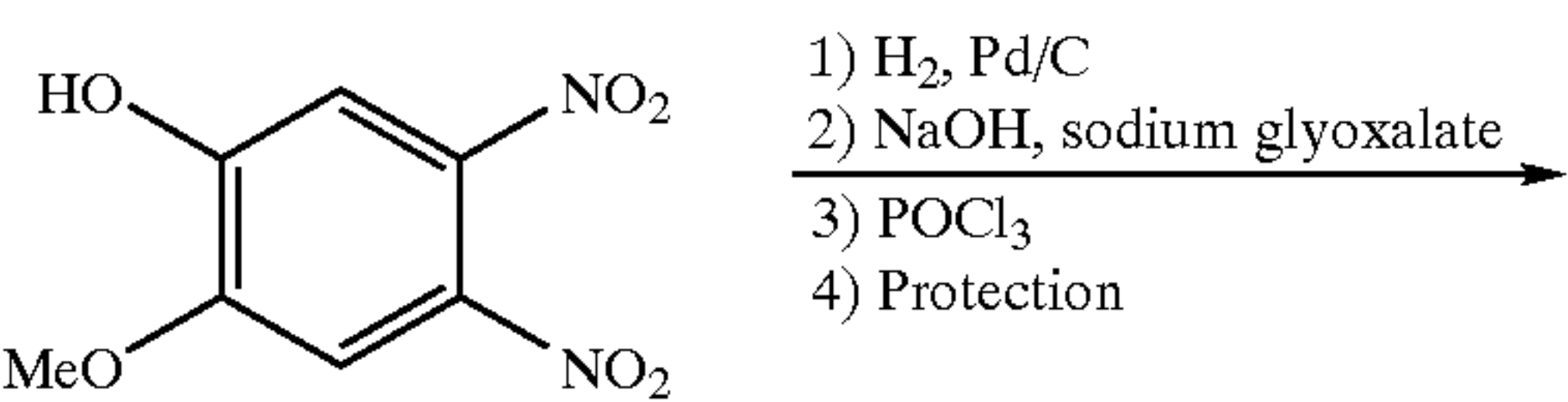
Scheme VIII
