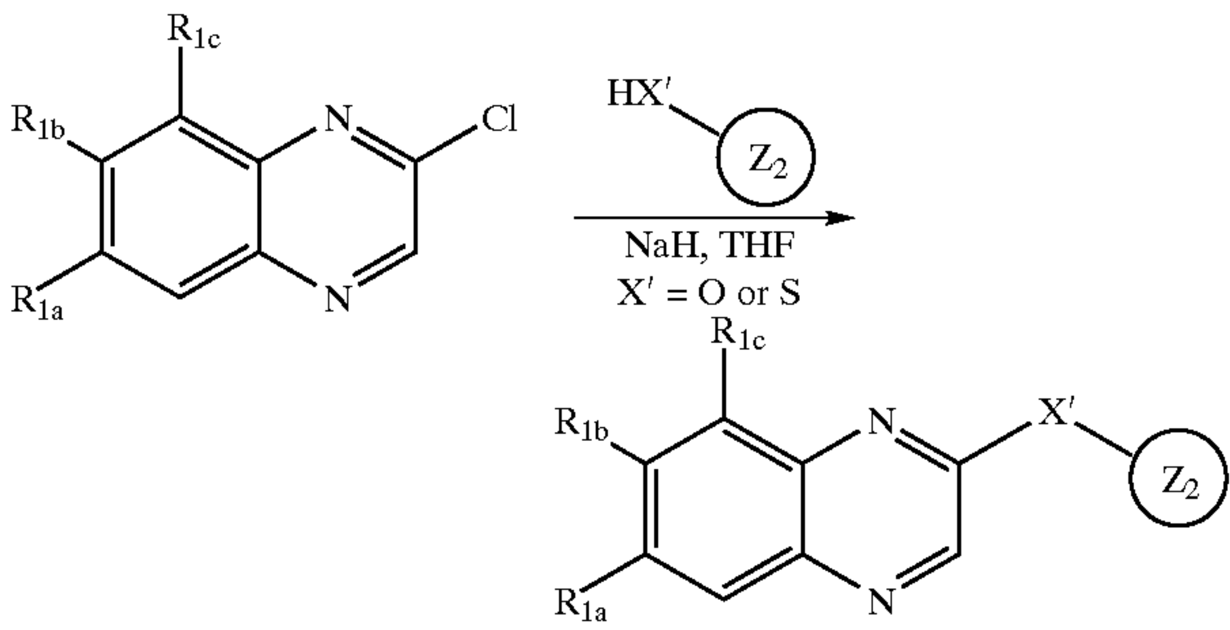
Scheme II
