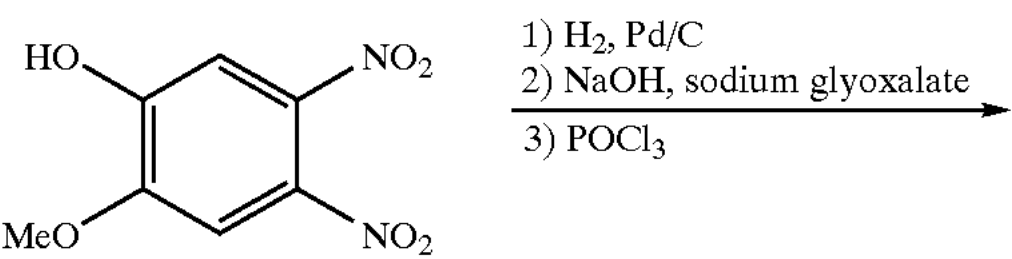
Scheme VII
