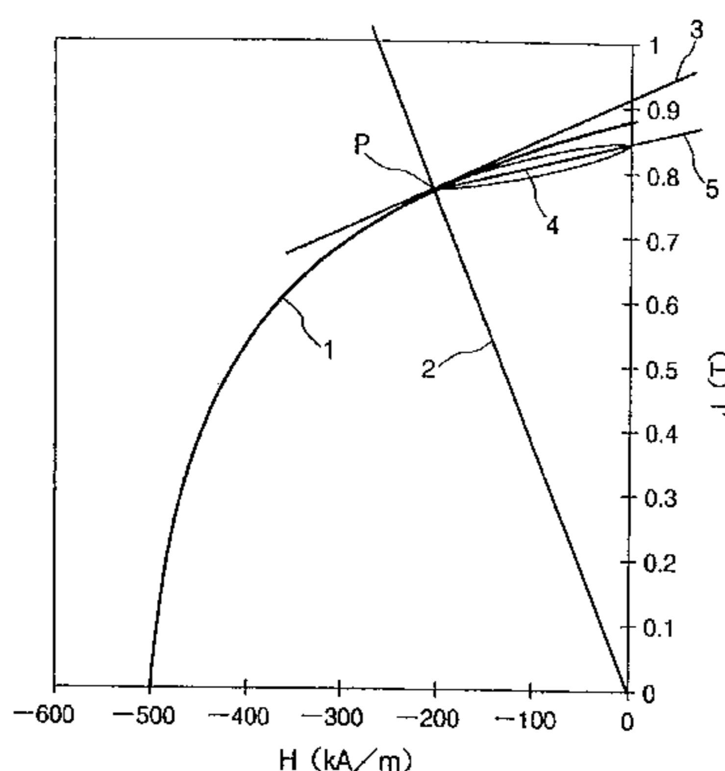
No.1: Demagnetization Curve No.2: Straight Line Having a Gradient of -3.8 \times 10^{-6} H/m in the J-H diagram No.3: Tangential Line at Intersectioning Point P No.4: Recoil Curve No.5: Straight Line Representing a Gradient of the Recoil Curve
