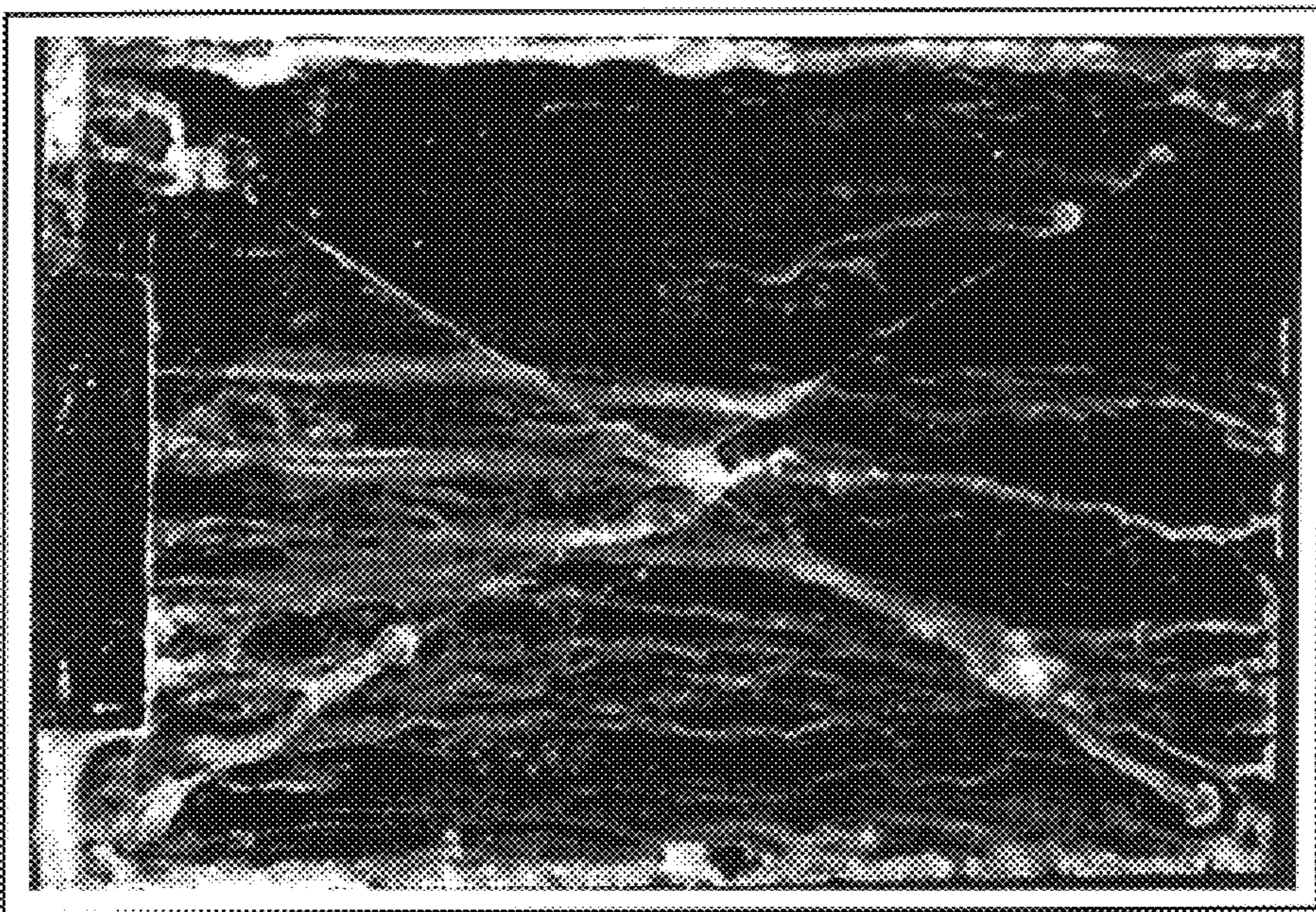
ACID ZINC-NICKEL PLATED 4130 STEEL WITH TCP POST TREATMENT- FIG-12 AFTER 1000 HOUR EXPOSURE TO ASTM B117 NEUTRAL SALT FOG
