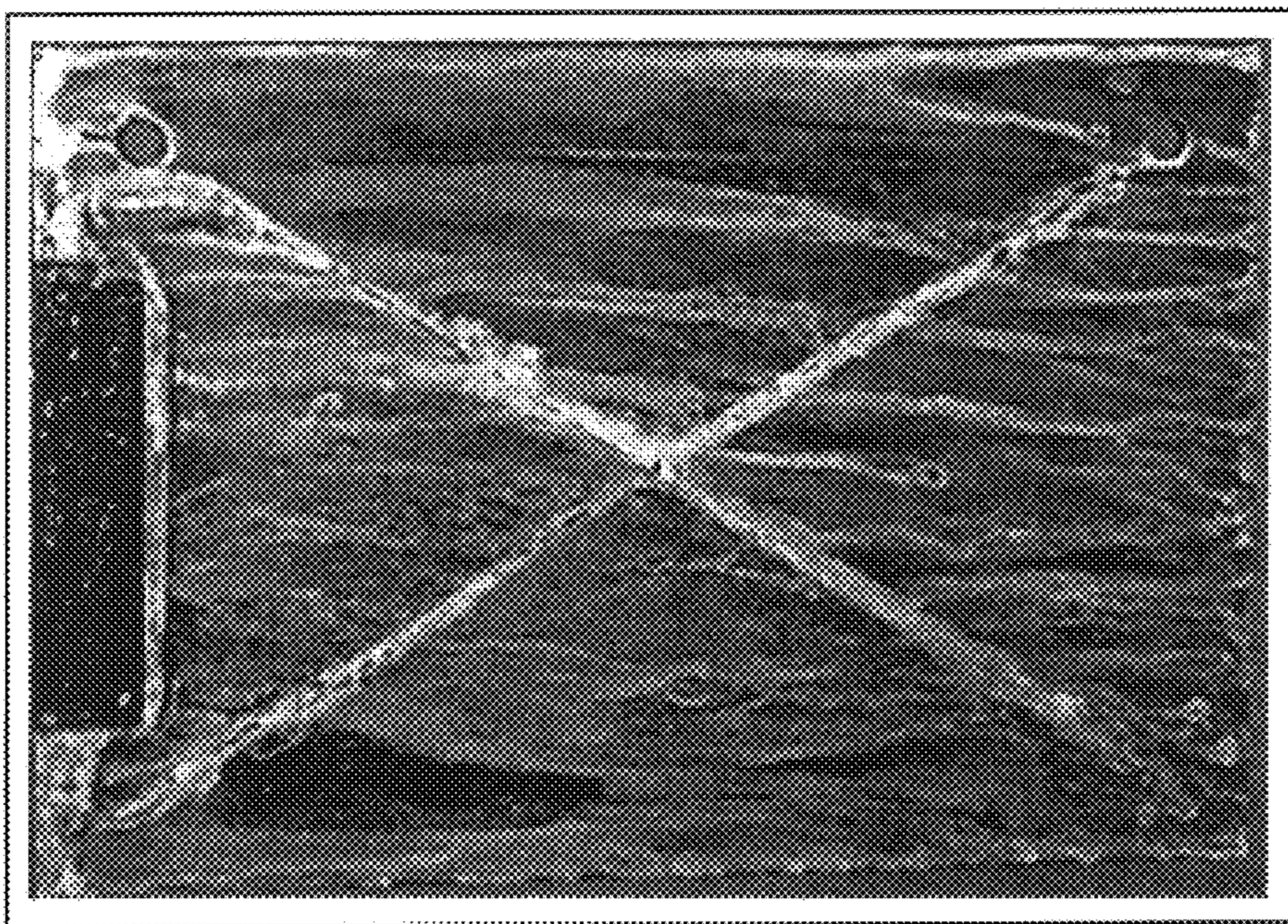
BASIC ZINC-NICKEL PLATED 4130 STEEL WITH TCP POST TREATMENT- FIG-11 AFTER 1000 HOUR EXPOSURE TO ASTM B117 NEUTRAL SALT FOG
