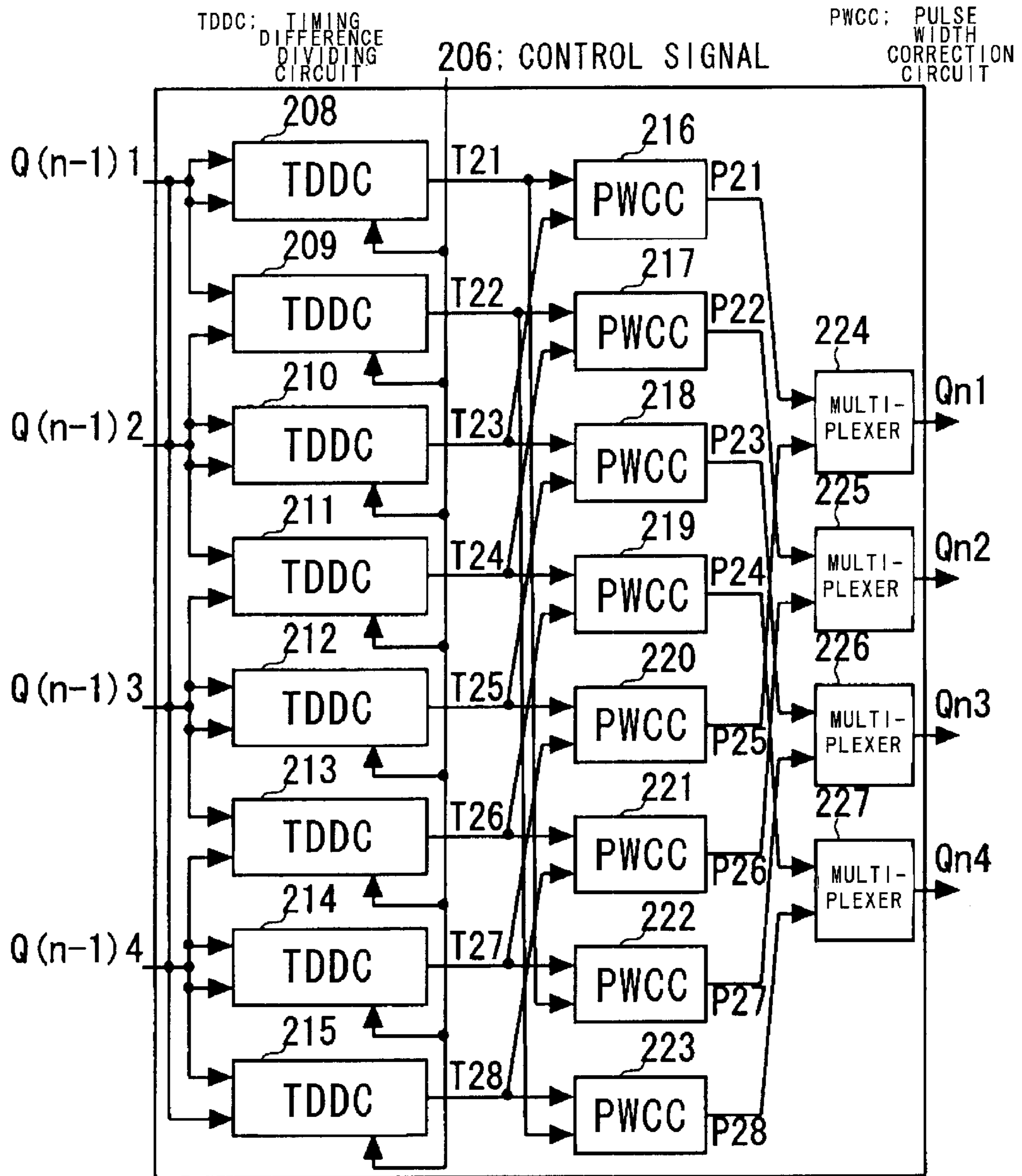
202-n: FOUR-PHASE CLOCK MULTIPLICATION CIRCUIT
