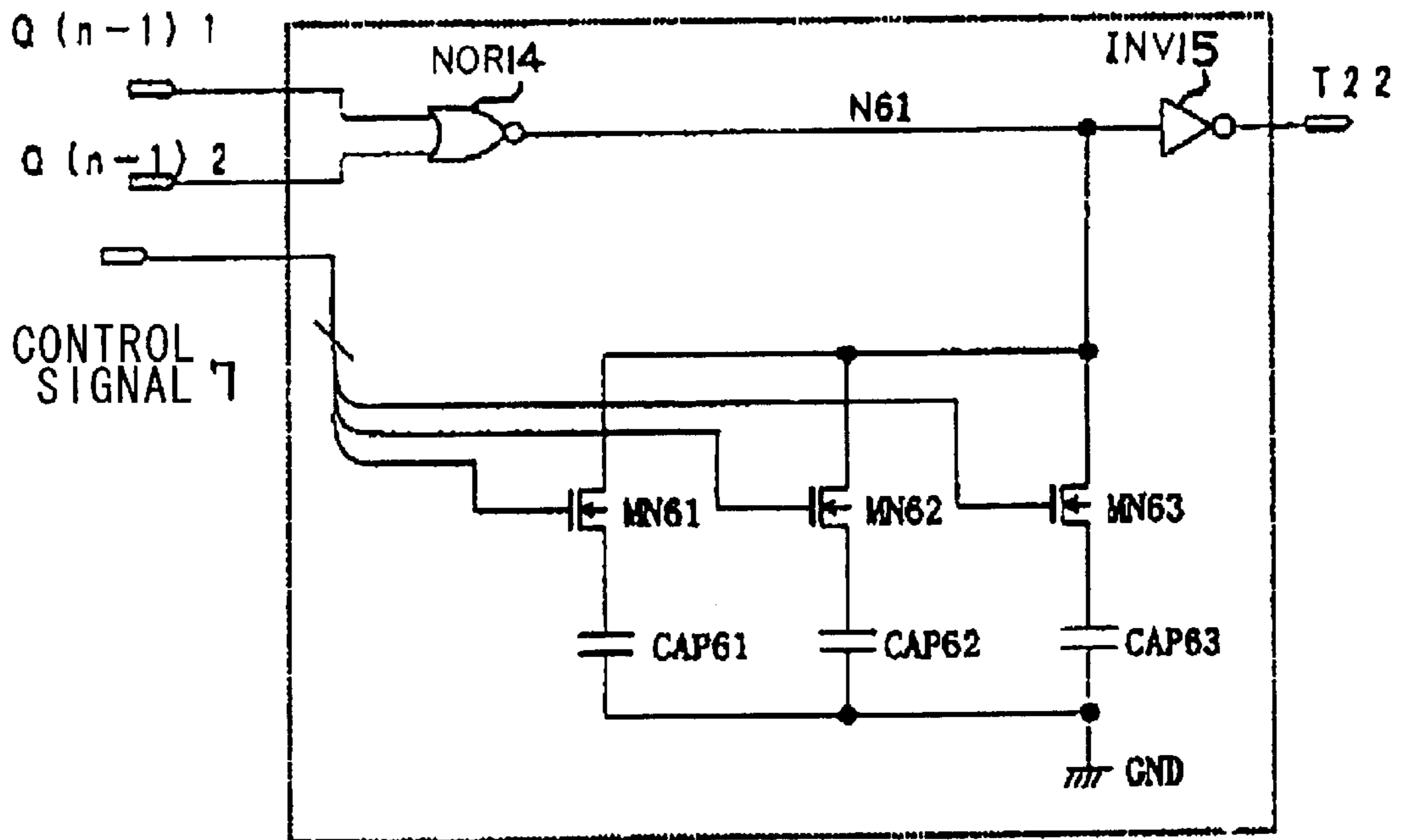
TIMING DIFFERENCE DIVIDING CIRCUIT 209
