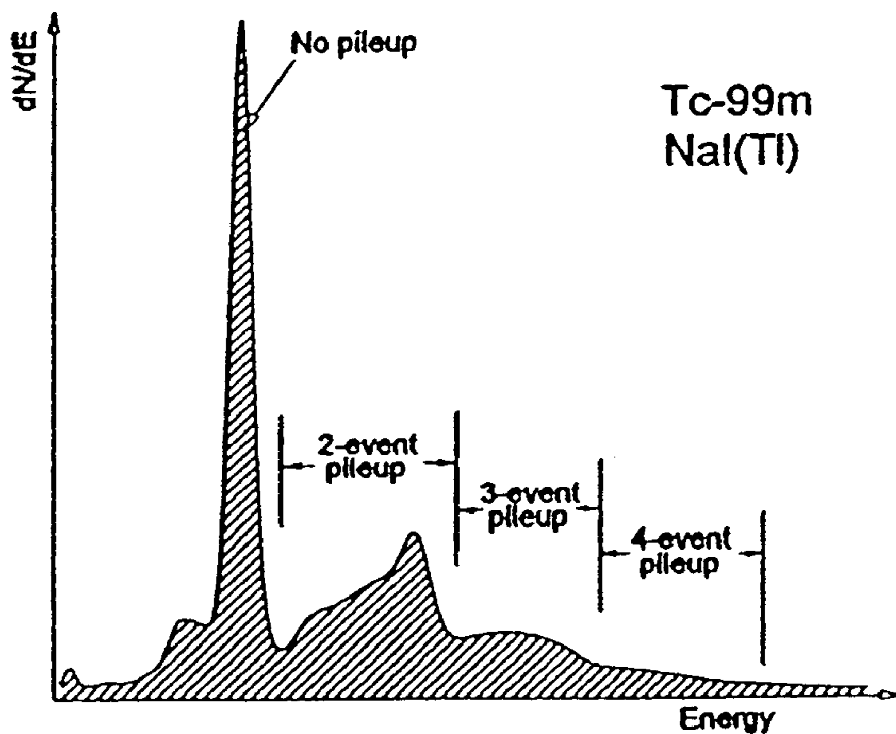
FIG. 16 Delay-line pulse-clipping (256 ns) energy spectrum of 99m Tc at 2 \times 10^6 cps. The pileup fraction is larger than the 'area under the curve' indicates because each count in the pileup region is made up of several counts.
