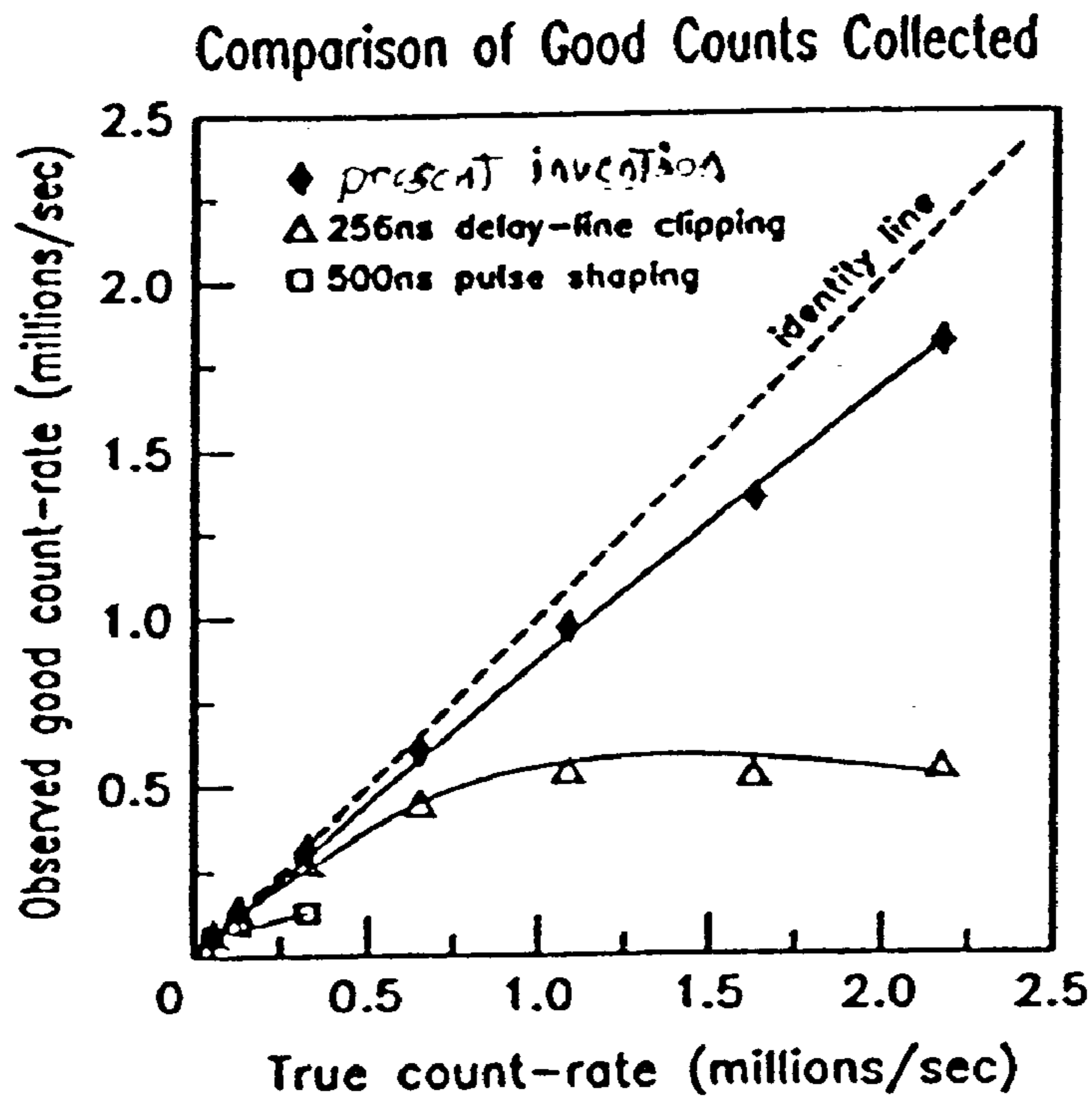
FIG. 15 Photopeak (non-pileup) count rates as a function
