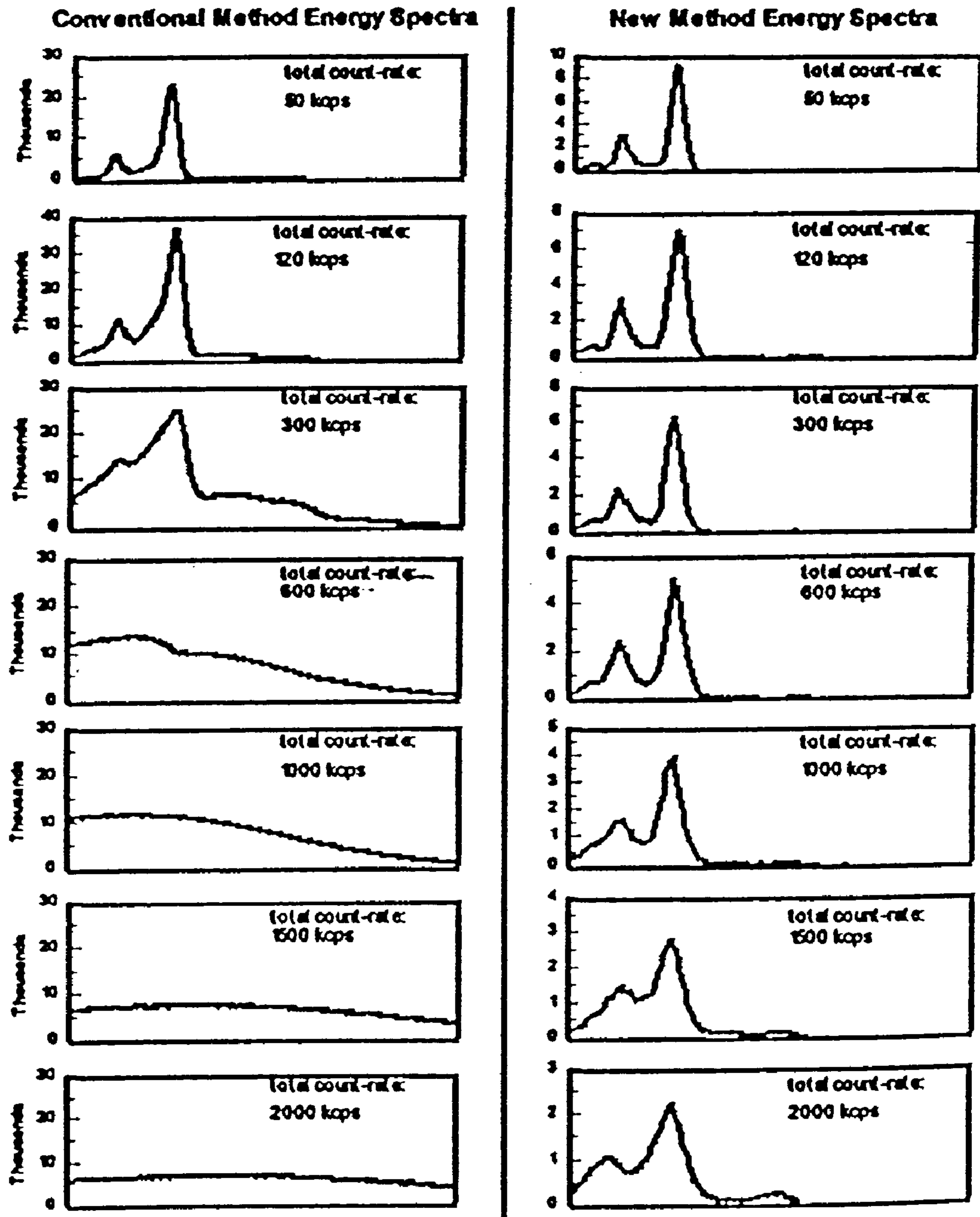
99m Tc energy spectra comparison between the standard and new methods for a 3"x4" NaI(Tl) with a 2" PMT. Pulse shaping time for the standard method is 0.5μs.
