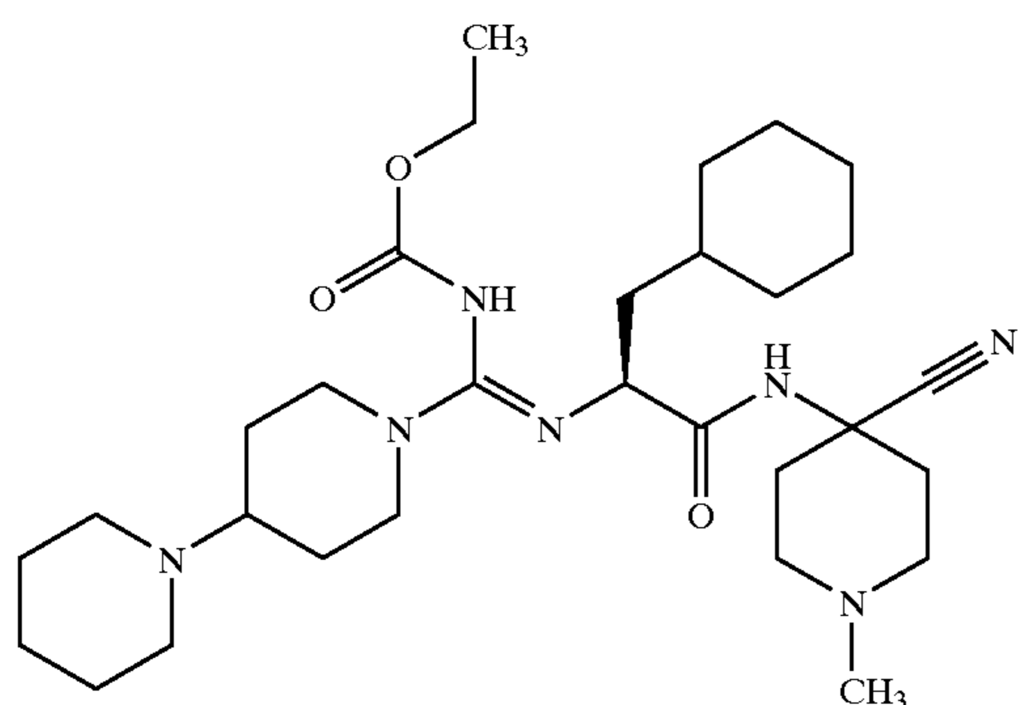
{[1,4']Bipiperidinyl-1'-yl-[1-(4-cyano-1-methyl-piperidin-4-ylcarbamoyl)-2-cyclohexyl-ethylimino]-methyl}-carbamoyl Ethyl Ester; MS: 558 (M+1).
