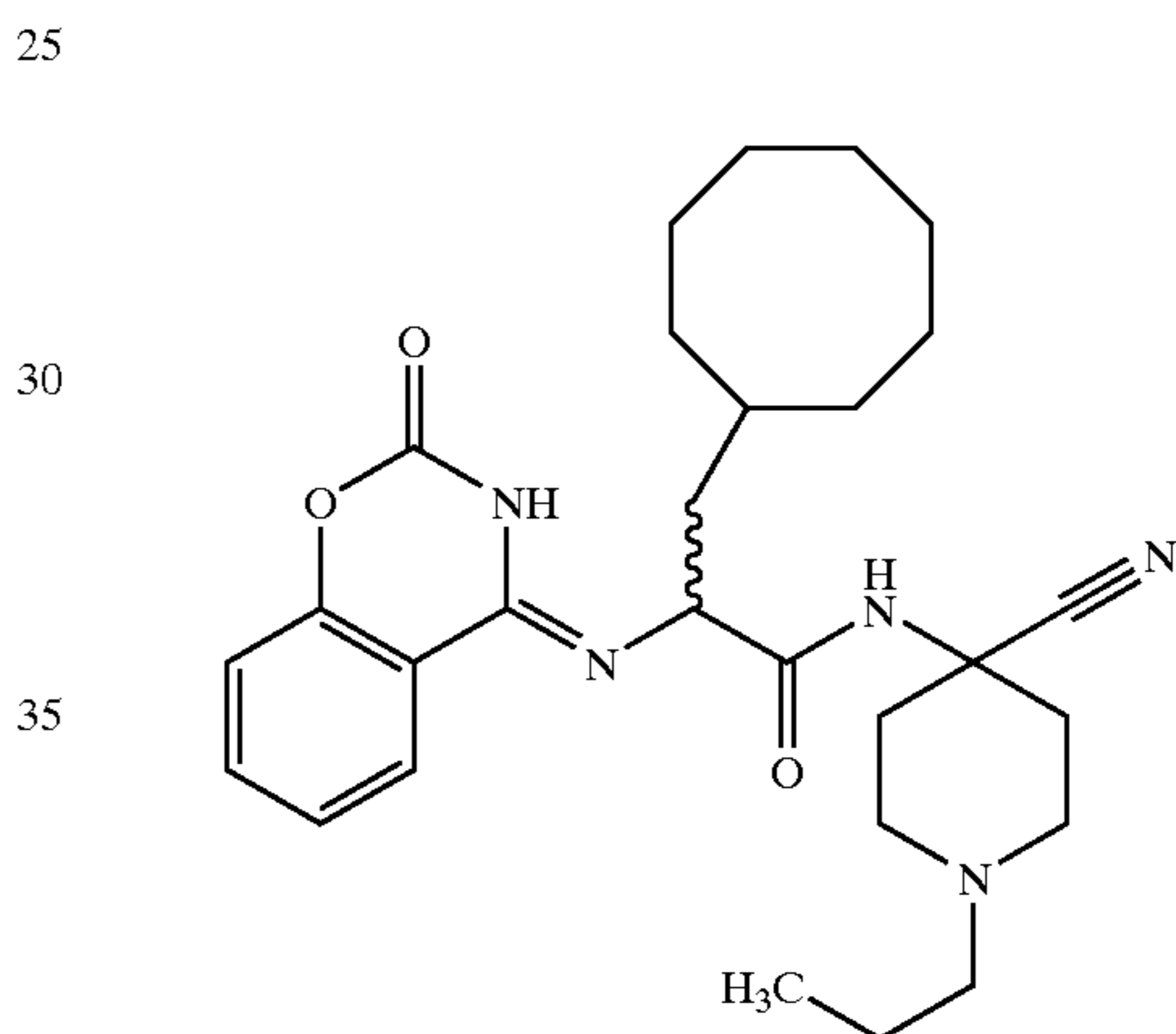
N-(4-Cyano-1-propyl-piperidin-4-yl)-3-cyclooctyl-2-(2-oxo-2,3-dihydro-benzo[e][1,3]oxazin-4-ylideneamino)-propionamide; MS: 494 (M+1)
