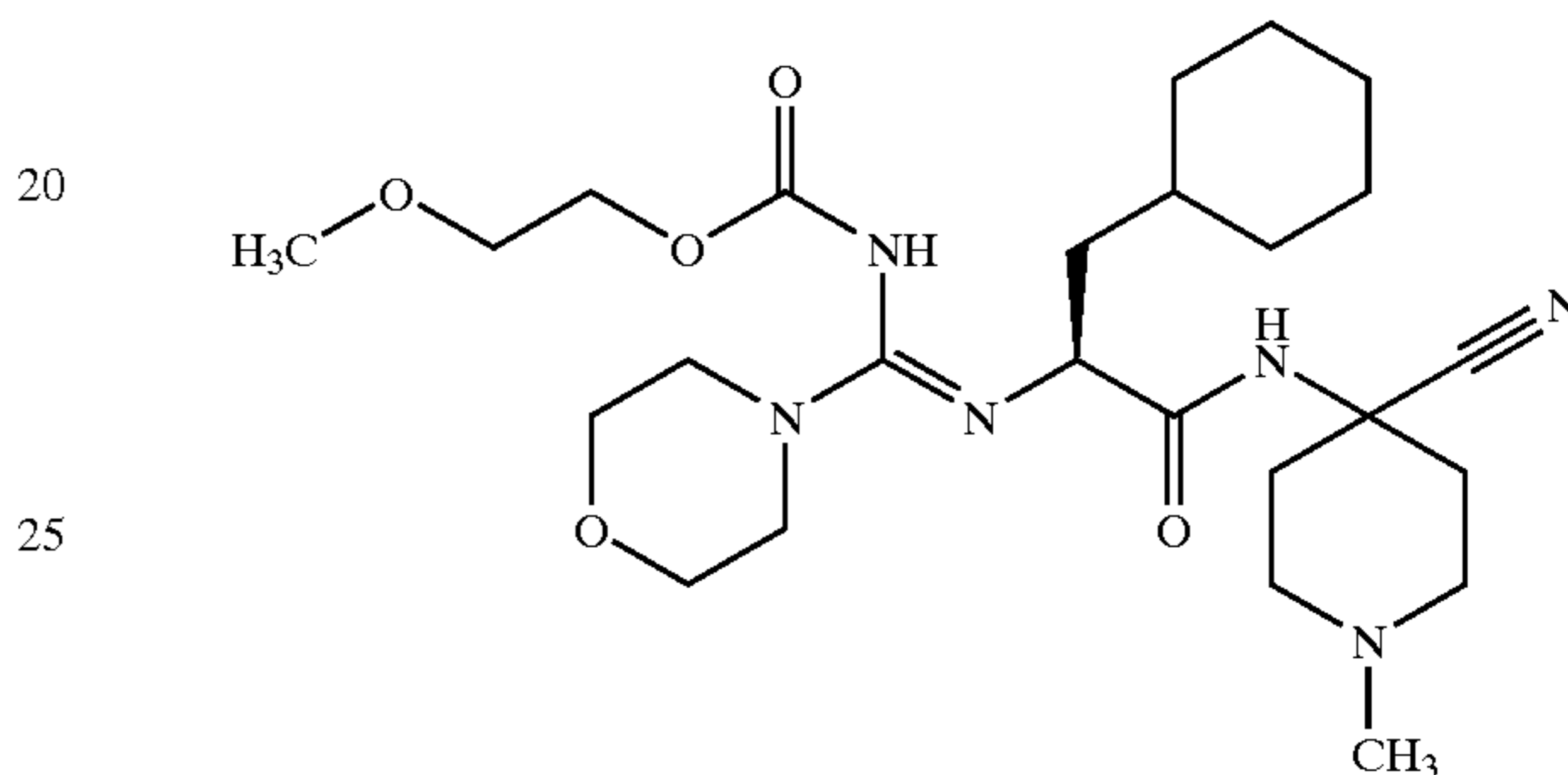
{[1-(4-Cyano-1-methyl-piperidin-4-ylcarbamoyl)-2-cyclohexyl-ethylimino]-morpholin-4-yl-methyl}-carbamic Acid 2-methoxy-ethyl Ester; MS: 507 (M+1)
