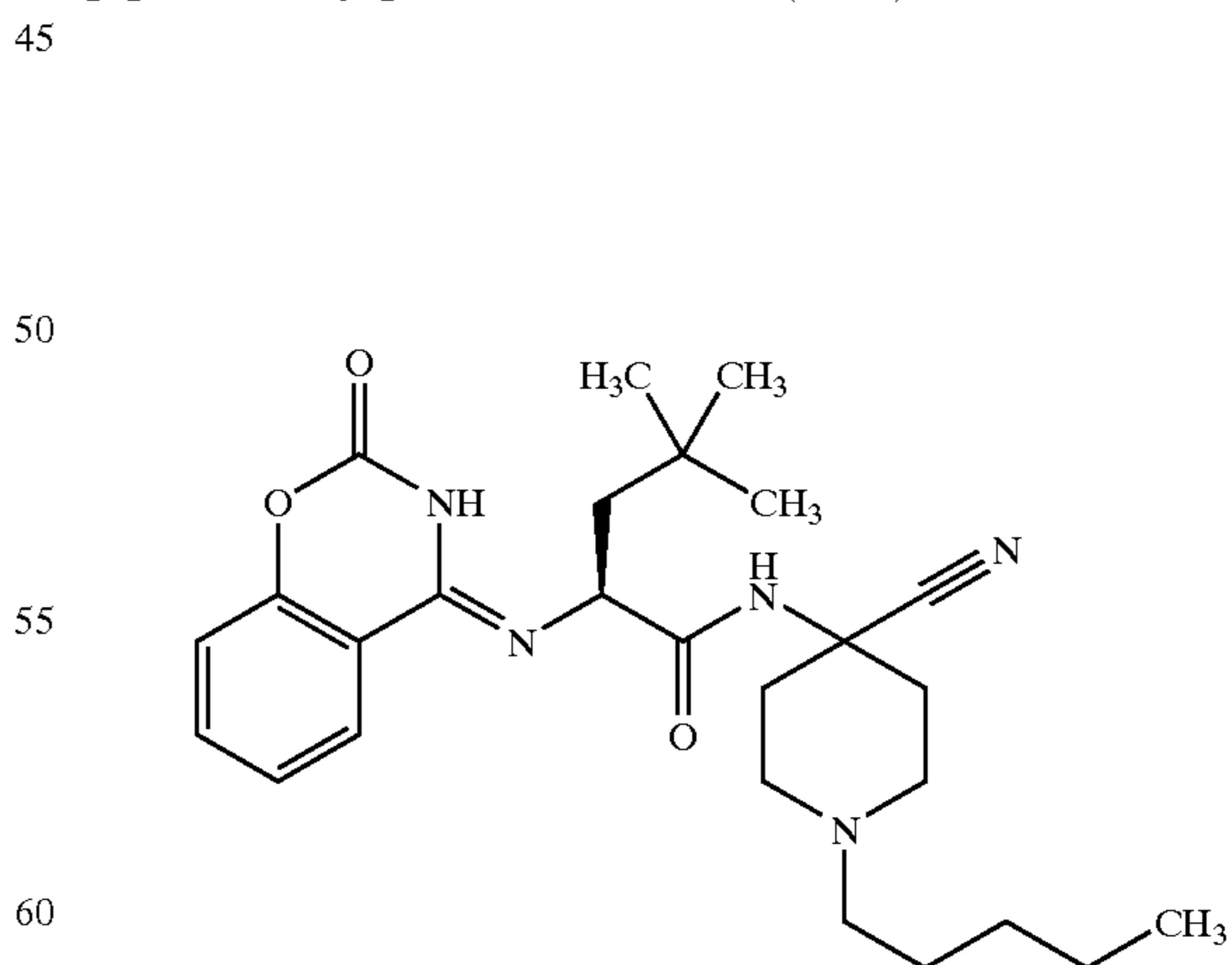
4,4-Dimethyl-2-(2-oxo-2H-benzo[e][1,3]oxazin-4-ylamino)-pentanoic Acid [4-Cyano-1-(3,3-dimethylbutyl)-piperidin-4-yl]-amide; MS: 482 (M+1)
