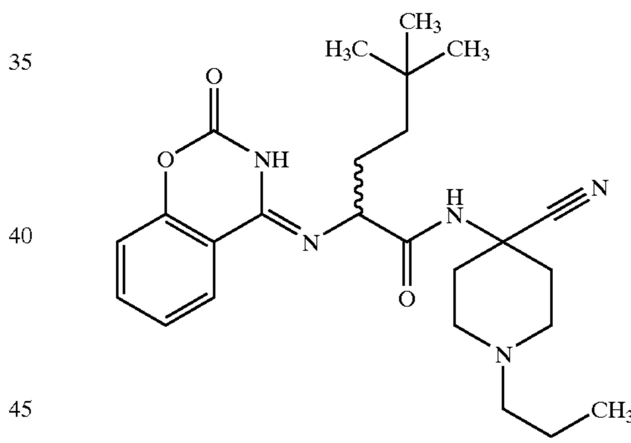
5,5-Dimethyl-2-(2-oxo-2,3-dihydro-benzo[e][1,3]oxazin-4-ylideneamino)-hexanoic Acid (4-cyano-1-propyl-piperidin-4-yl)-amide; MS: 454 (M+1)
