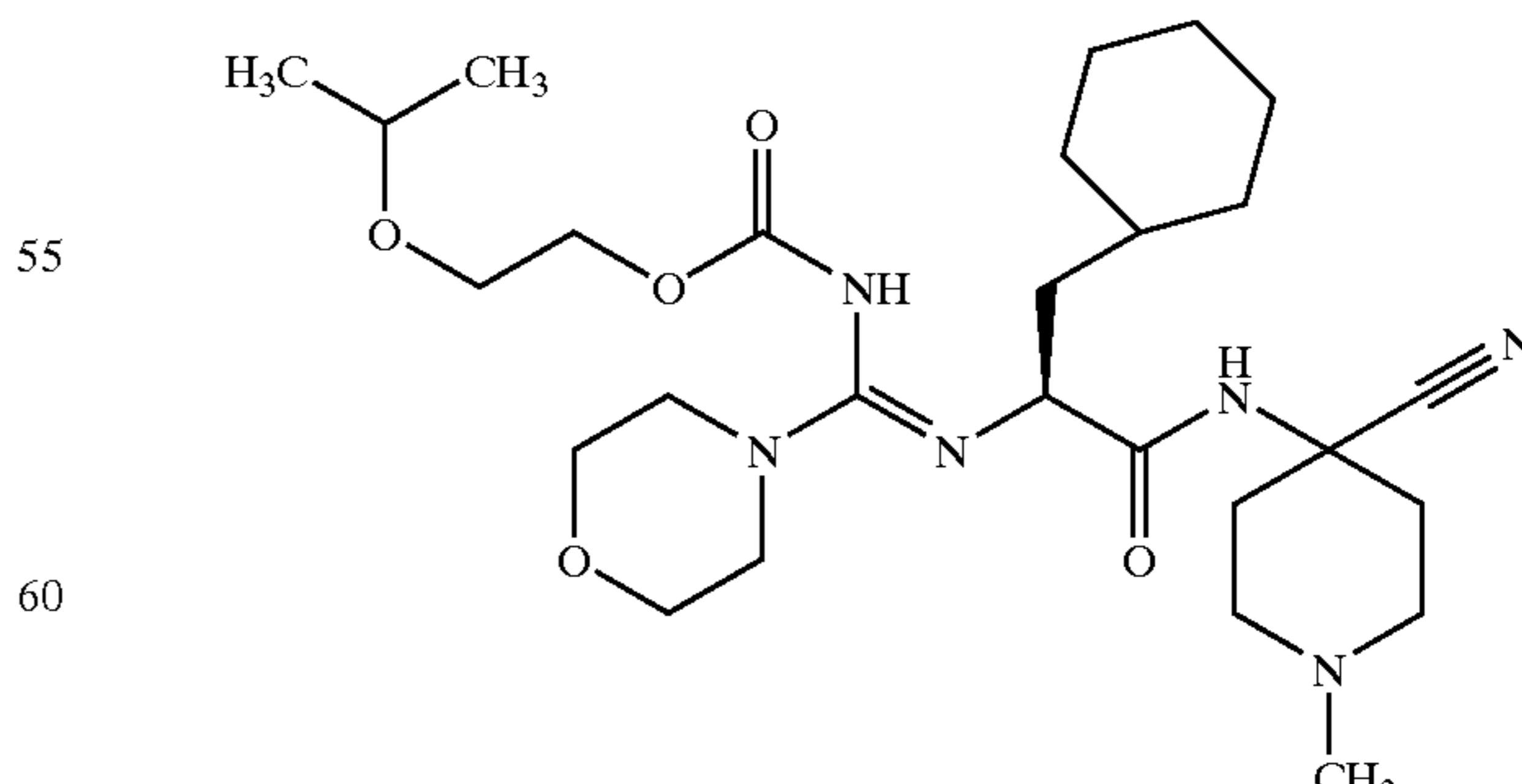
{[1-(4-Cyano-1-methyl-piperidin-4-ylcarbamoyl)-2-cyclohexyl-ethylimino]-morpholin-4-yl-methyl}-carbamic Acid 2-isopropoxy-ethyl Ester; MS: 534 (M+1)
