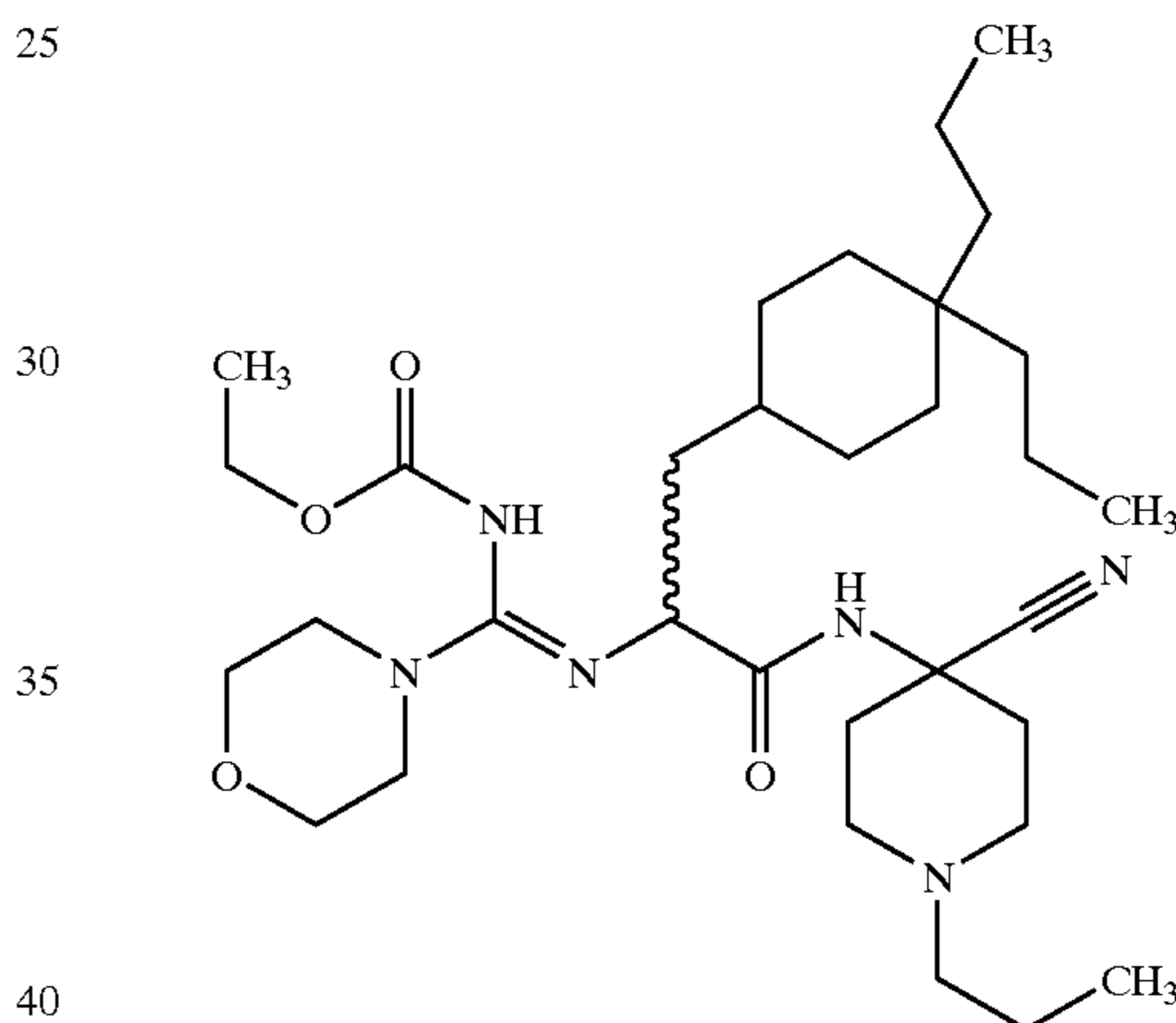
{[1-(4-Cyano-1-propyl-piperidin-4-ylcarbamoyl)-2-(4,4-dipropyl-cyclohexyl)-ethylamino]-morpholin-4-yl-methylene}-carbamic Acid Ethyl Ester; MS: 589 (M+1)
