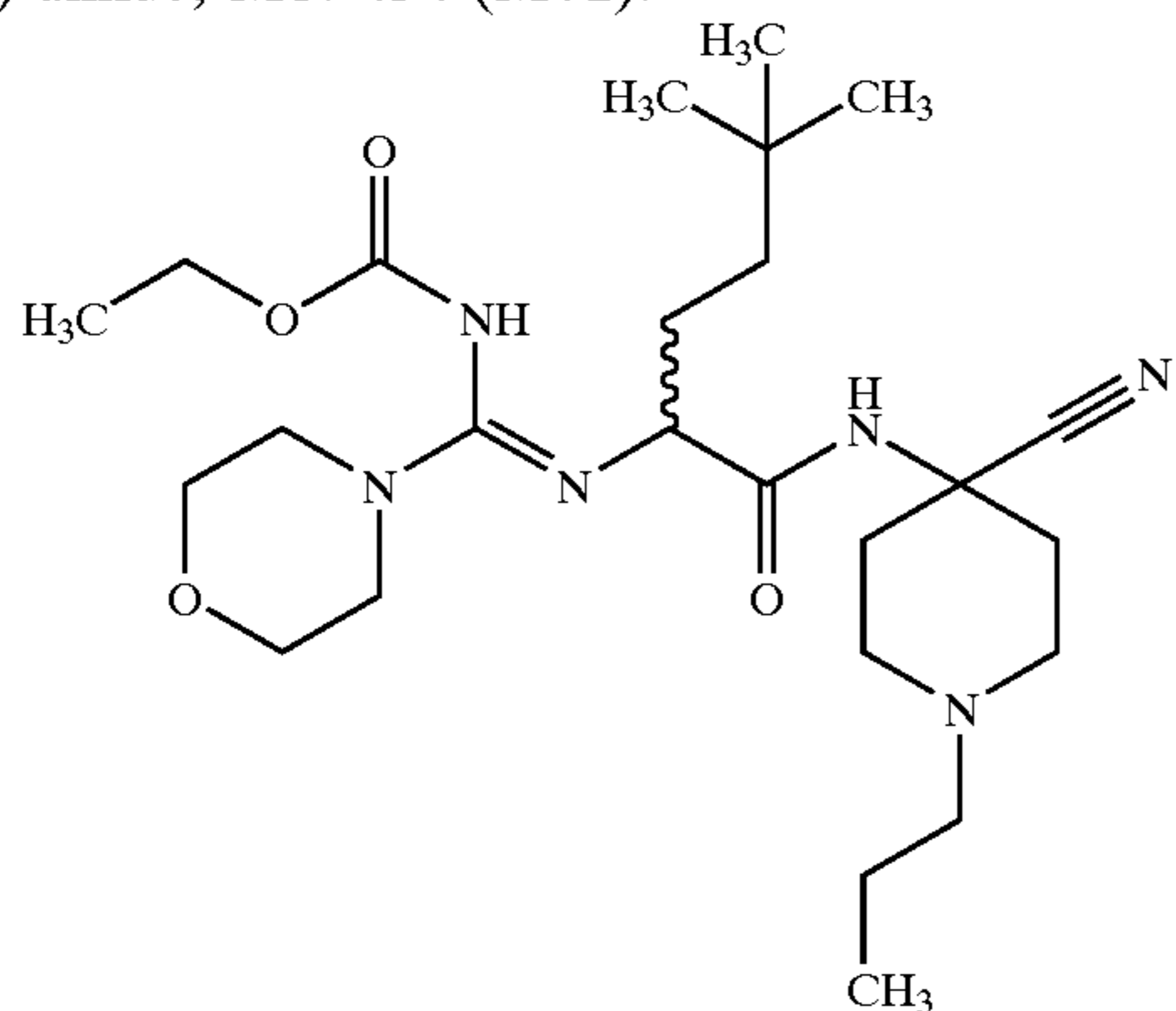
{[1-(4-Cyano-1-propyl-piperidin-4-ylcarbamoyl)-4,4-dimethyl-pentylimino]-morpholin-4-yl-methyl}-carbamic Acid Ethyl Ester; MS: 493 (M+1).
