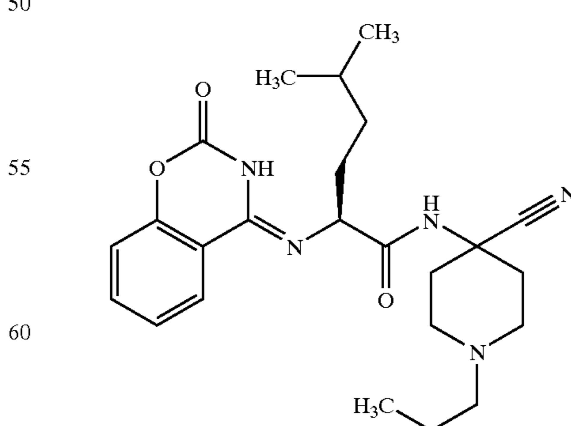
5-Methyl-2-(2-oxo-2,3-dihydro-benzo[e][1,3]oxazin-4-ylideneamino)-hexanoic Acid (4-cyano-1-propyl-piperidin-4-yl)-amide; MS: 440 (M+1)
