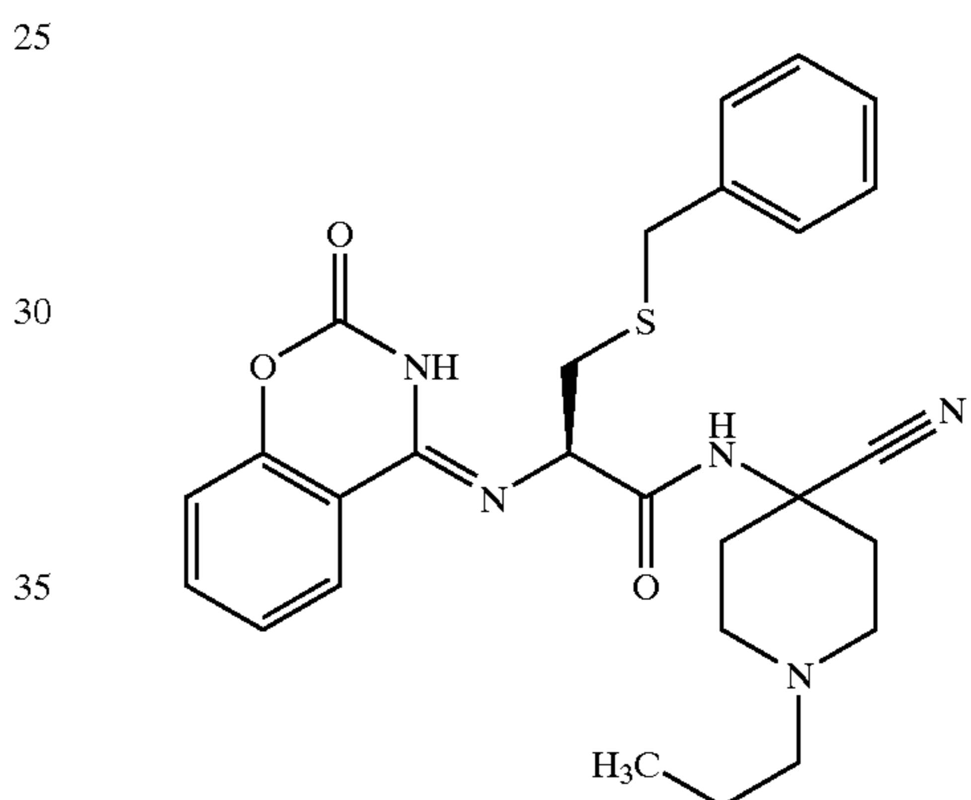
3-Benzylsulfanyl-N-(4-cyano-1-propyl-piperidin-4-yl)-2-(2-oxo-2,3-dihydro-benzo[e][1,3]oxazin-4-ylideneamino)-propionamide; MS: 506 (M+1).
