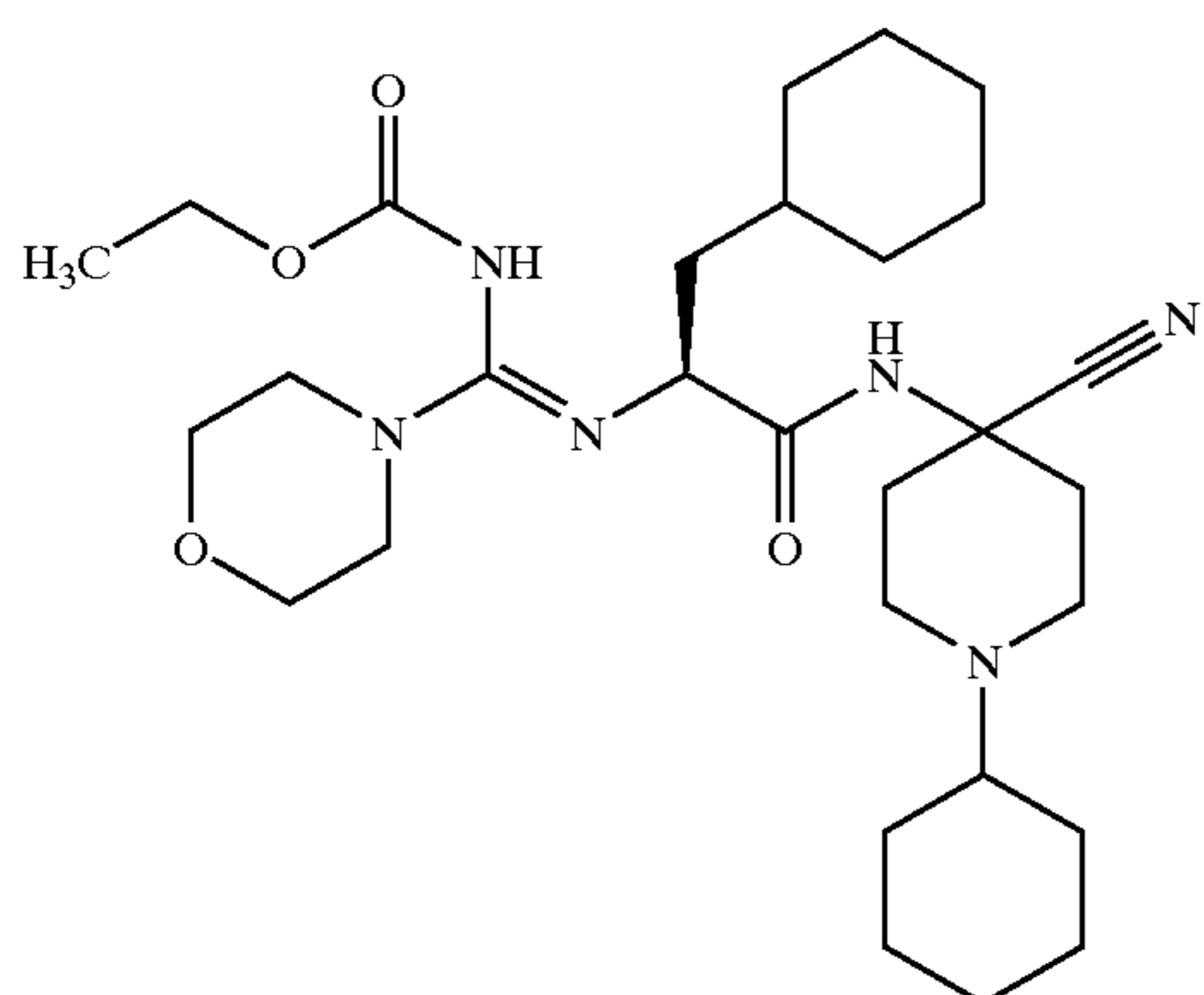
{[1-(4-Cyano-1-cyclohexyl-piperidin-4-ylcarbamoyl)-2-cyclohexyl-ethylamino]-Ester; MS: 545 (M+1)}
