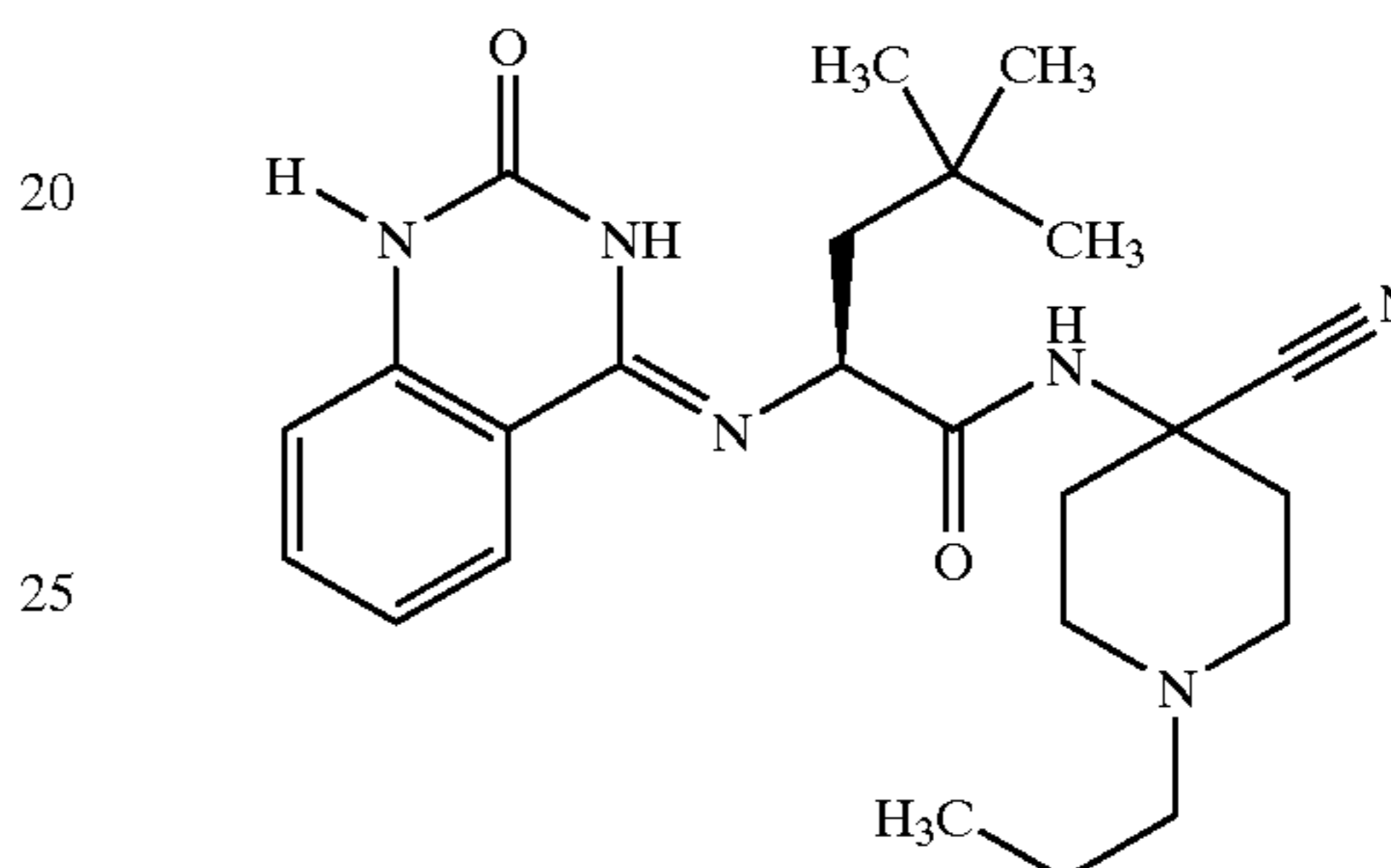
4,4-Dimethyl-2-(2-oxo-2,3-dihydro-1H-quinazolin-4-ylideneamino)-pentanoic Acid (4-cyano-1-propyl-piperidin-4-yl)-amide; MS: 439 (M+1)
