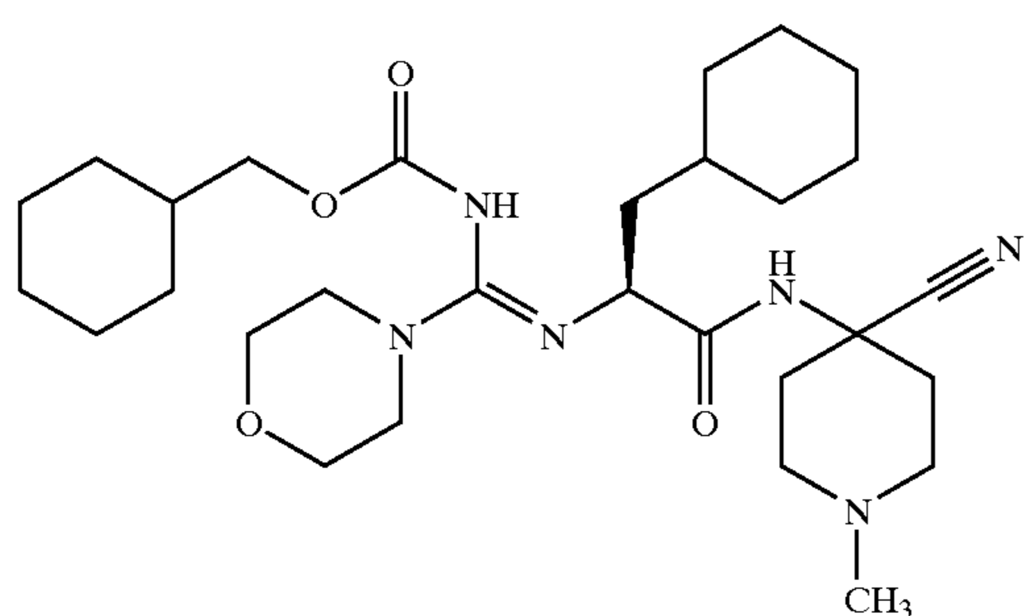
{[1-(4-Cyano-1-methyl-piperidin-4-ylcarbamoyl)-2-cyclohexyl-ethylamino]-morpholin-4-yl-methylene}-carbamic Acid Cyclohexylmethyl Ester; MS: 545 (M+1)
