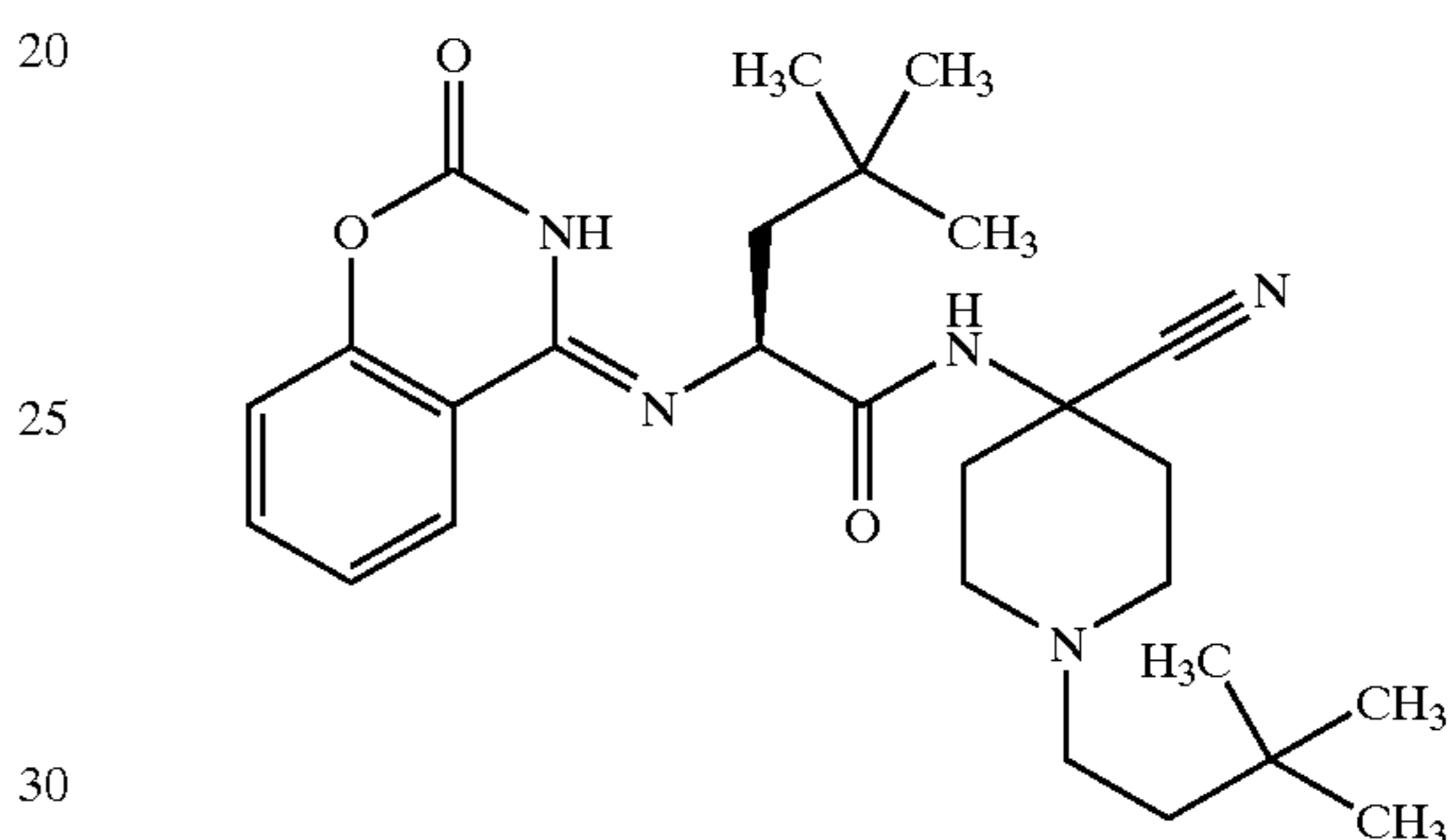
4,4-Dimethyl-2-(2-oxo-2H-benzo[e][1,3]oxazin-4-ylamino)-pentanoic Acid [4-cyano-1-(3,3-dimethyl-butyl)-piperidin-4-yl]-amide; MS: 482 (M+1)
