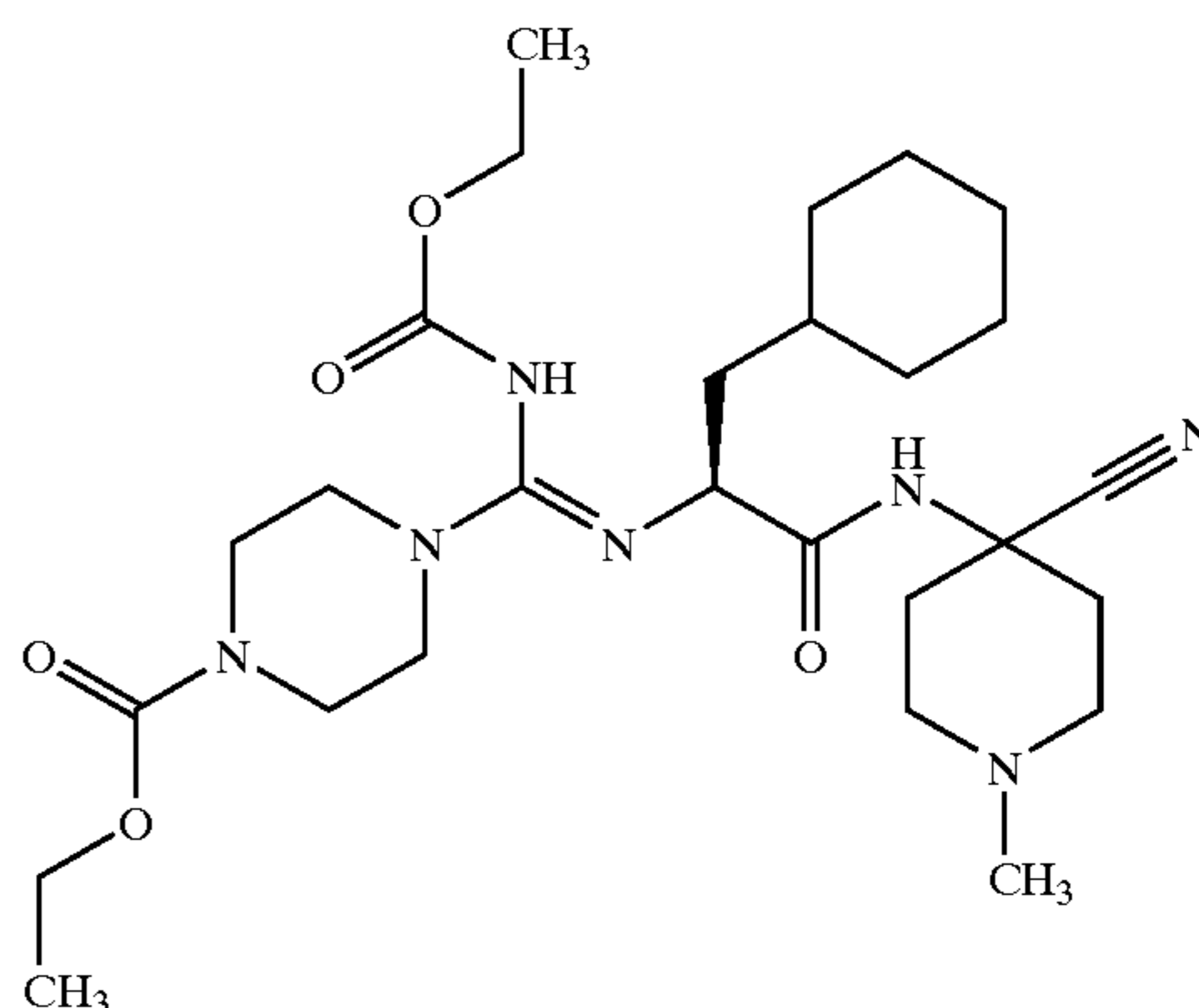
4-[[1-(4-Cyano-1-methyl-piperidin-4-ylcarbamoyl)-2-cyclohexyl-ethylimino]-ethoxycarbonylamino-methyl]-piperazine-1-carboxylic Acid Ethyl Ester; MS: 548 (M+1).
