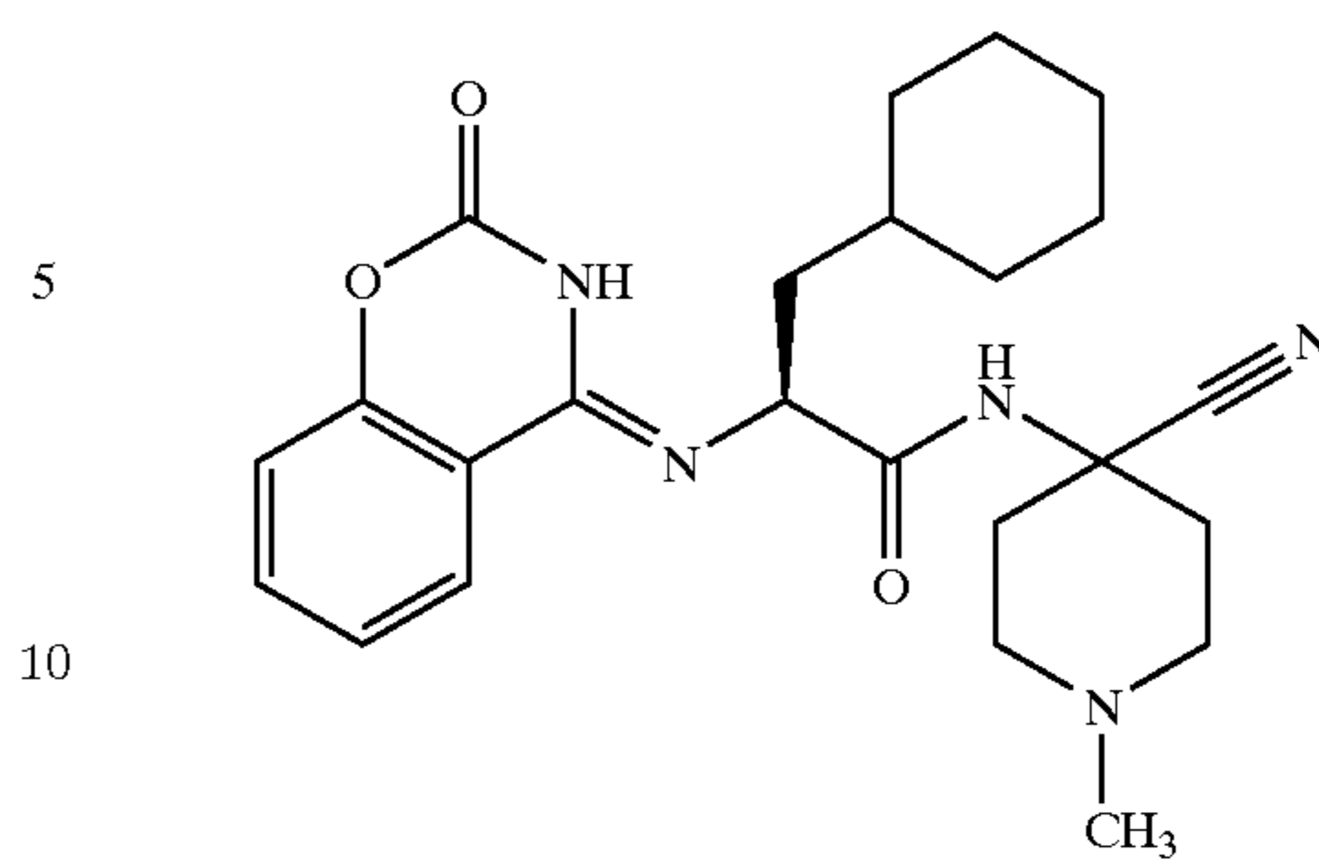
N-(4-Cyano-1-methyl-piperidin-4-yl)-3-cyclohexyl-2-(2-oxo-2,3-dihydro-benzo[e][1,3]oxazin-4-ylideneamino)-propionamide; MS: 438 (M+1).
