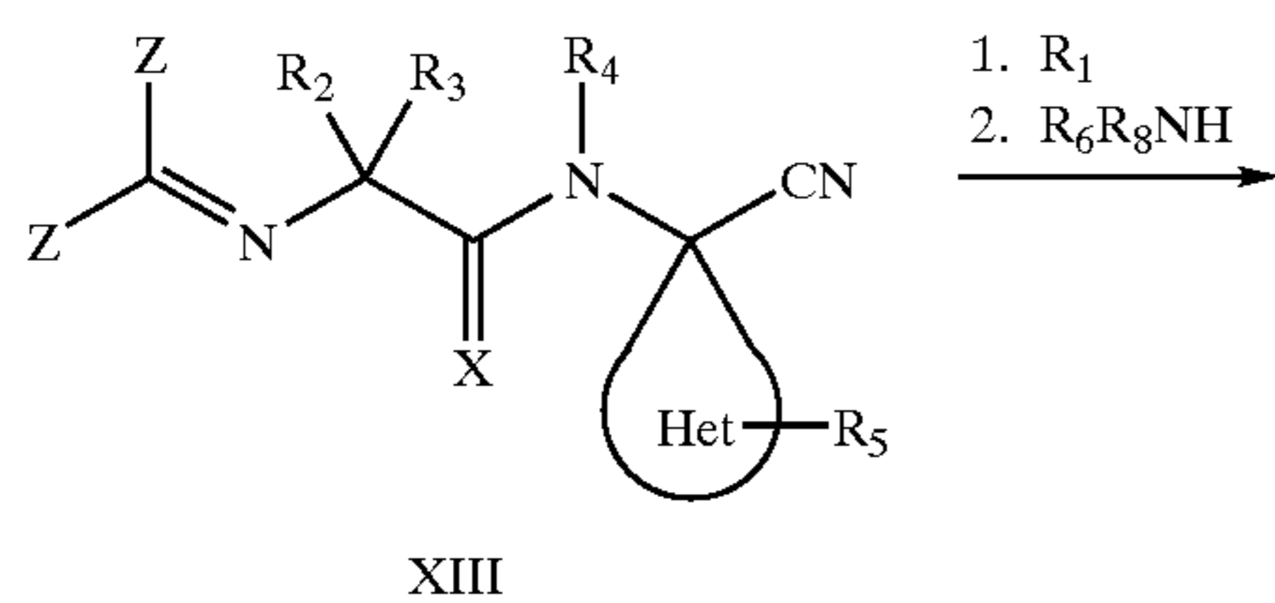
Scheme VII
