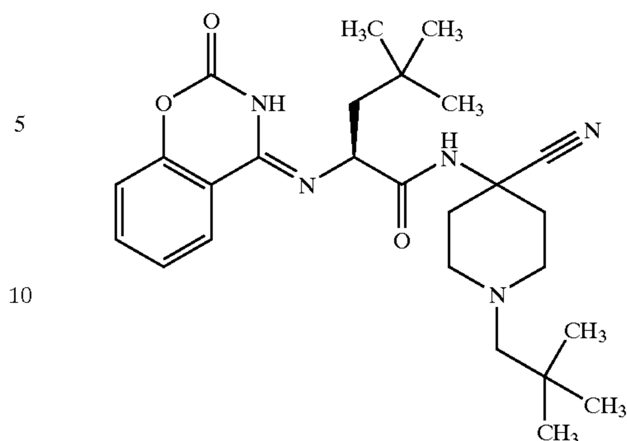
4,4-Dimethyl-2-(2-oxo-2H-benzo[e][1,3]oxazin-4-ylamino)-pentanoic Acid [4-cyano-1-(4-yl)-amide]; MS: 468 (M+1)
