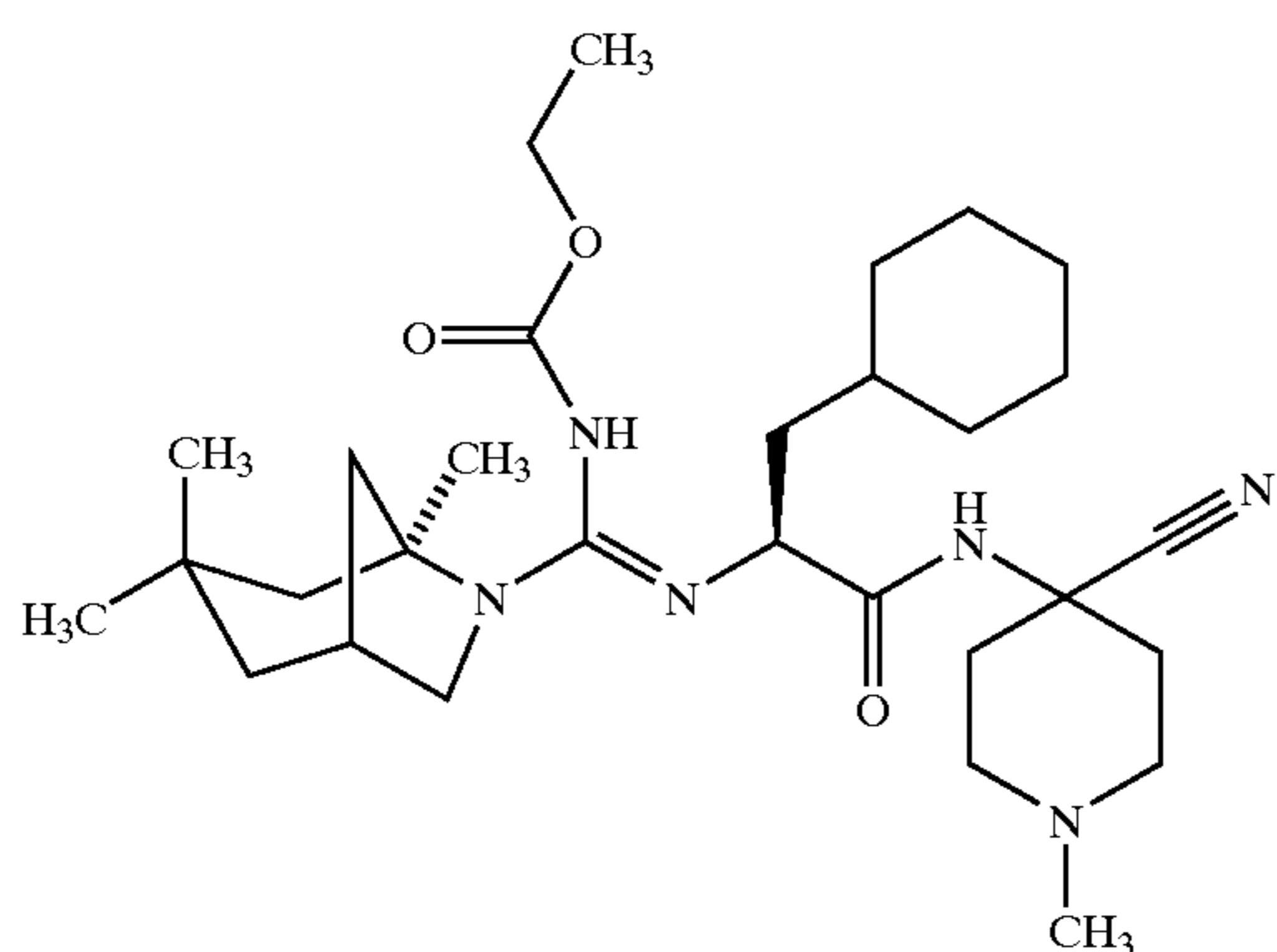
[[1-(4-Cyano-1-methyl-piperidin-4-ylcarbonyl)-2-cyclohexyl-ethylimino]-(3,3,5-trimethyl-6-aza-bicyclo[3.2.1]oct-6-yl)-methyl]-carbamic Acid Ethyl Ester; MS: 543 (M+1).
