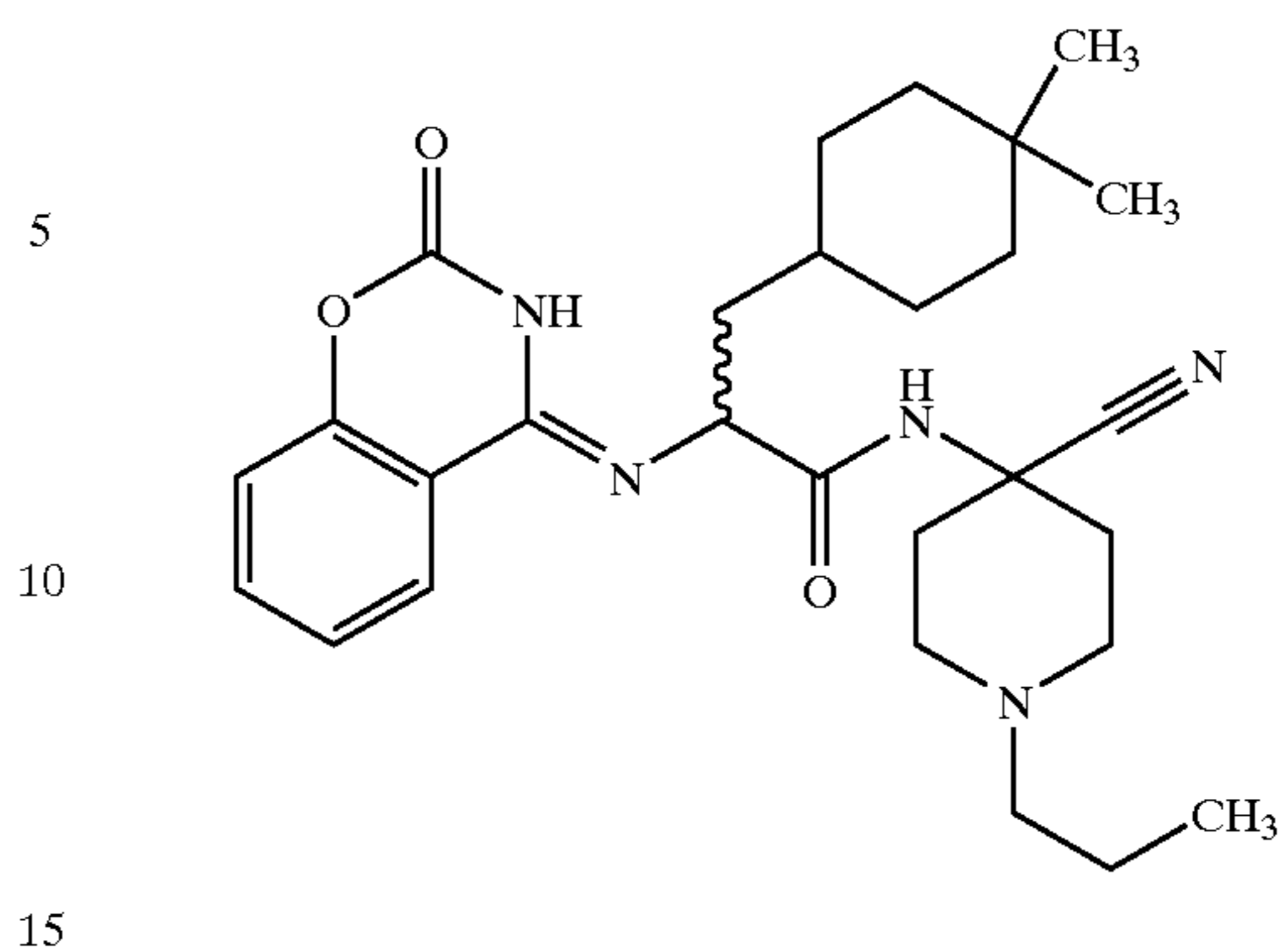
N-(4-Cyano-1-propyl-piperidin-4-yl)-3-(4,4-dimethyl-cyclohexyl)-2-(2-oxo-2H-benzo[e][1,3]oxazin-4-ylamino)-propionamide; MS: 494 (M+1)
