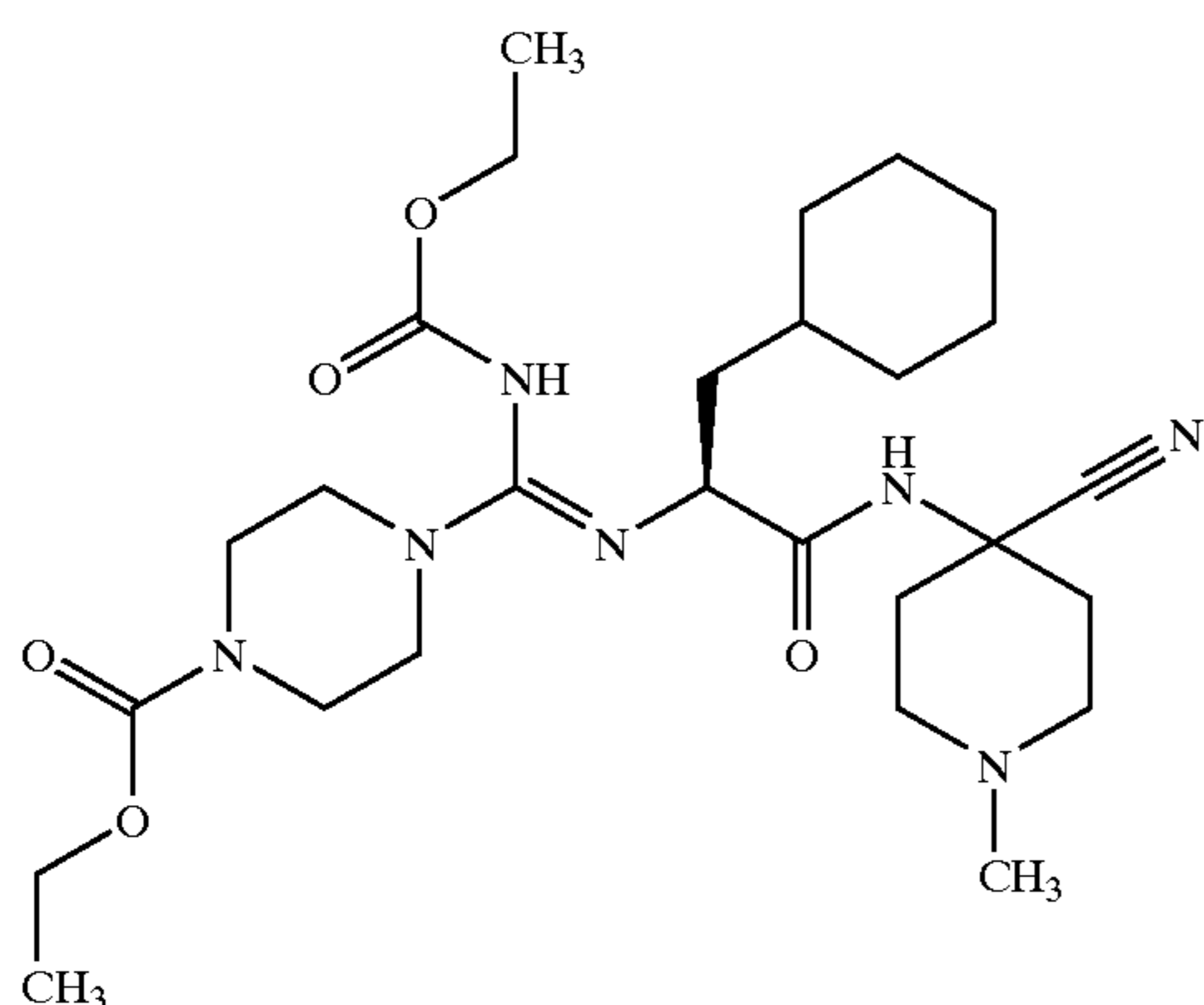
4-[[1-(4-Cyano-1-methyl-piperidin-4-ylcarbonyl)-2-cyclohexyl-ethylimino]-ethoxycarbonylamino-methyl]-piperazine-1-carboxylic Acid Ethyl Ester; MS: 548 (M+1).
