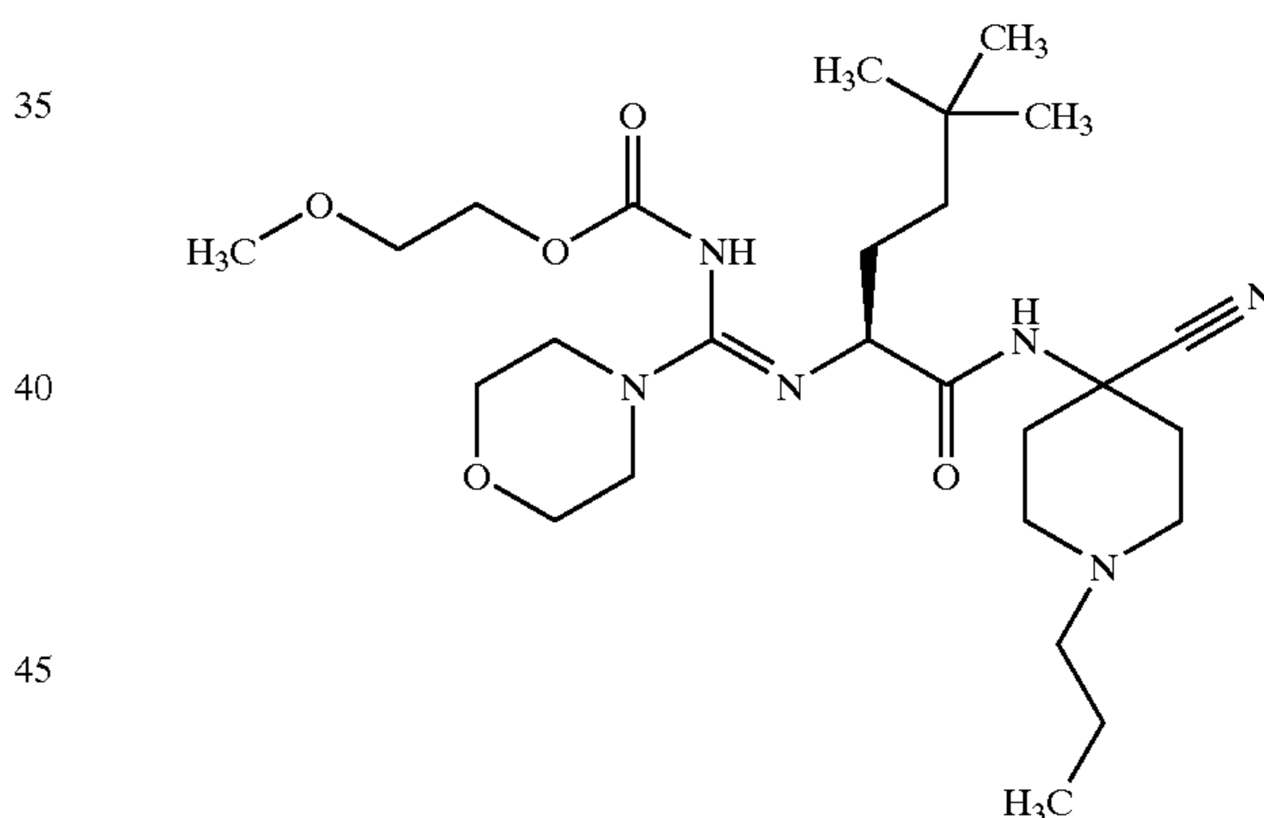
{[1-(4-Cyano-1-propyl-piperidin-4-ylcarbamoyl)-3,3-dimethyl-butylimino]-morpholin-4-yl-methyl}-carbamic Acid 2-methoxy-ethyl Ester; MS: 509 (M+1).
