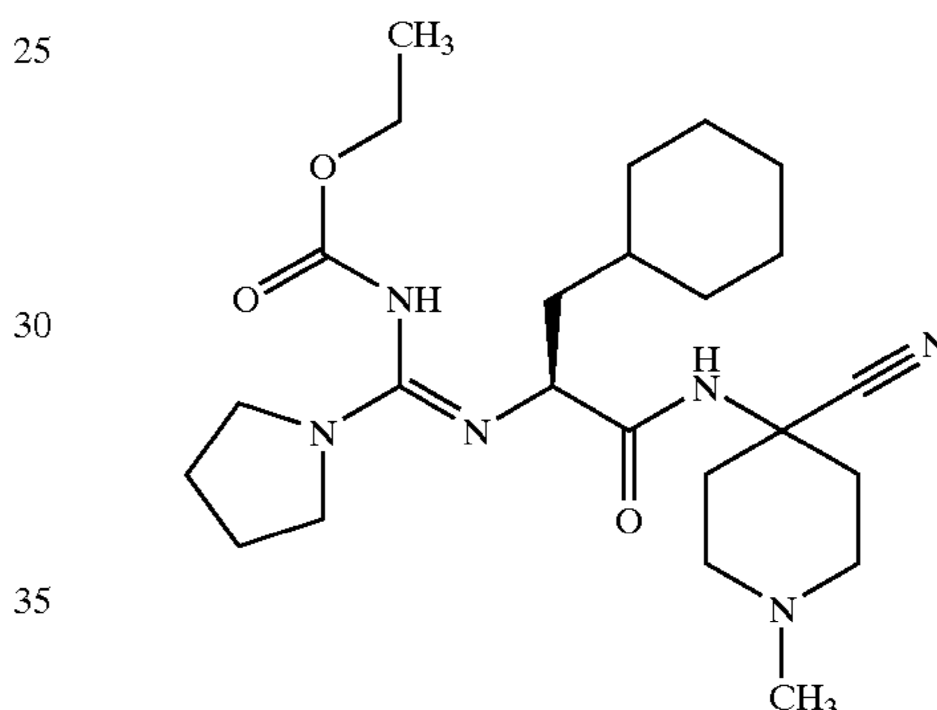
{[1-(4-Cyano-1-methyl-piperidin-4-ylcarbonyl)-2-cyclohexyl-ethylimino]-pyrrolidin-1-yl-methyl}-carbamic Acid Ethyl Ester; MS: 461 (M+1).
