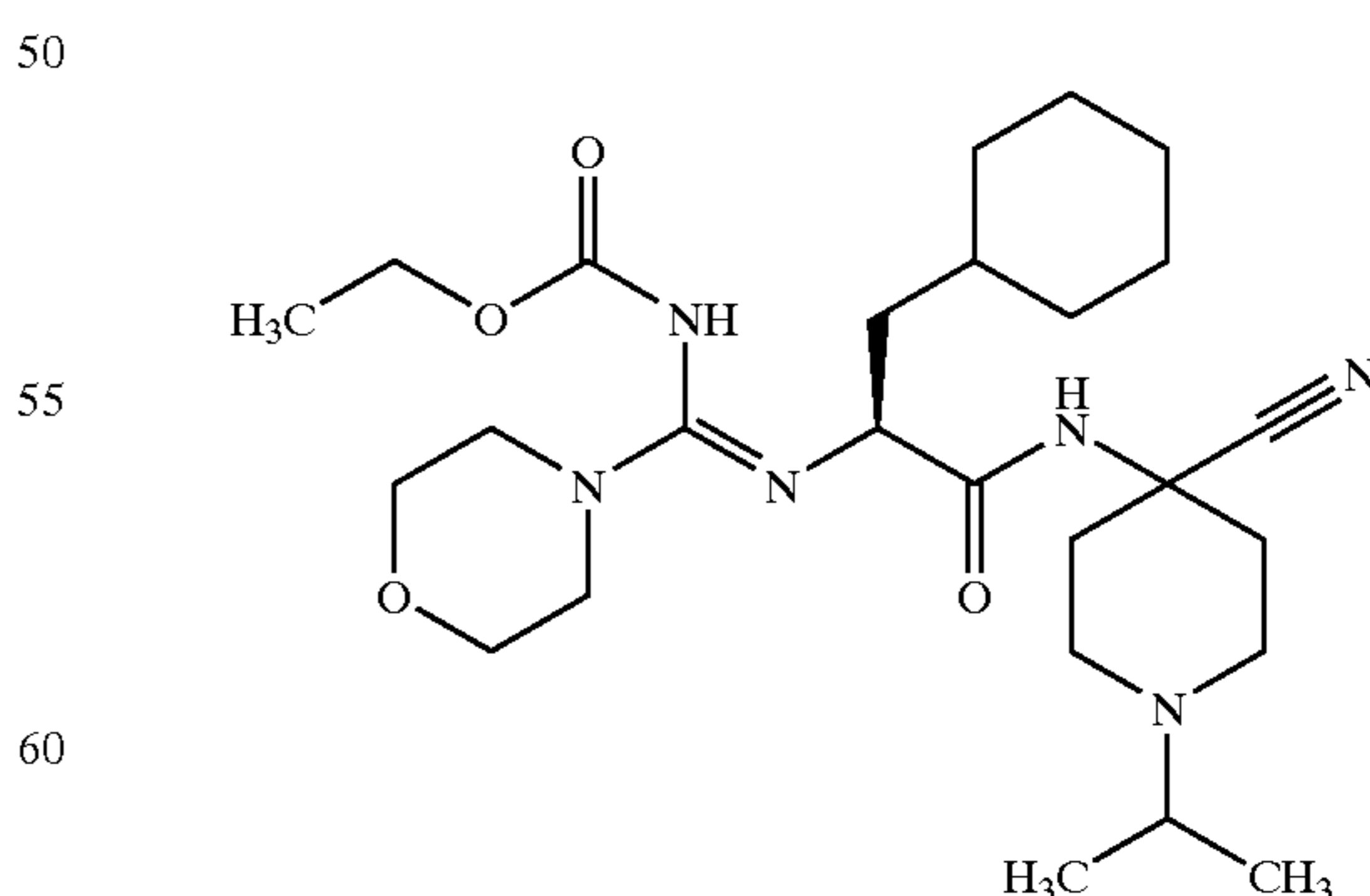
{[1-(4-Cyano-1-isopropyl-piperidin-4-ylcarbamoyl)-2-cyclohexyl-ethylamino]-morpholin-4-yl-methylene}-carbamic Acid Ethyl Ester; MS: 505 (M+1)
