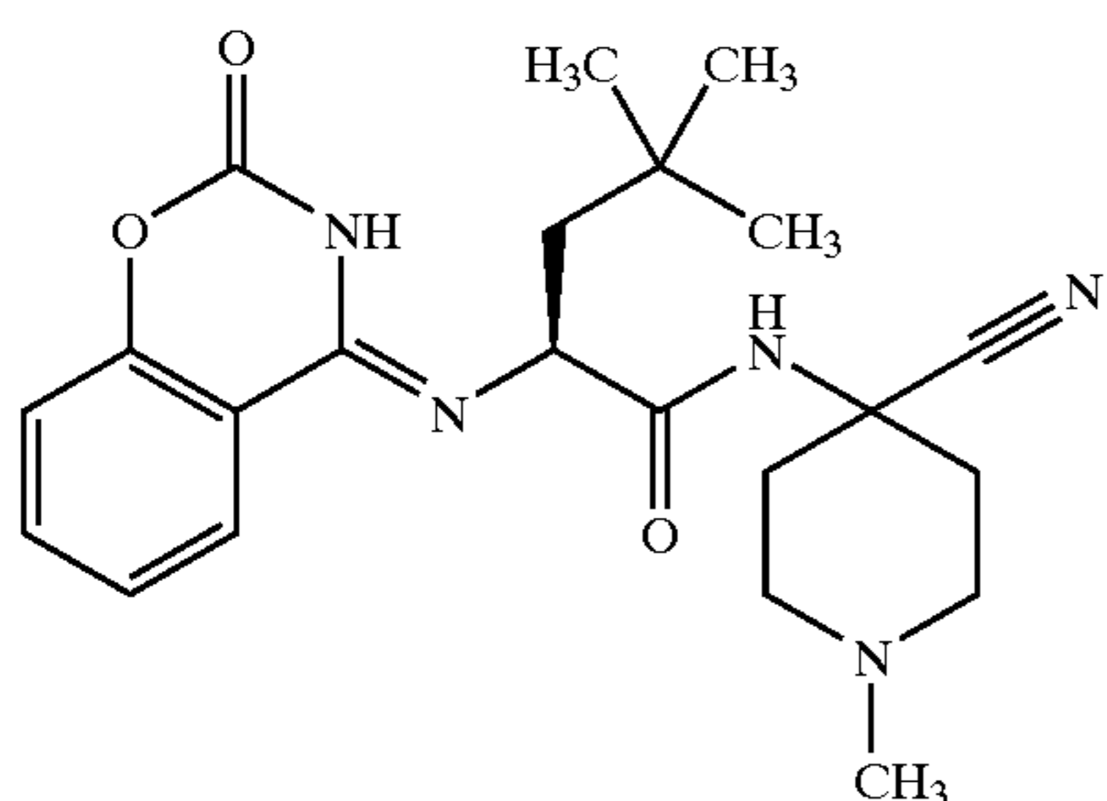
4,4-Dimethyl-2-(2-oxo-2H-benzo[e][1,3]oxazin-4-ylamino)-pentanoic Acid (4-Cyano-1-methyl-piperidin-4-yl)-amide; MS: 412 (M+1)
