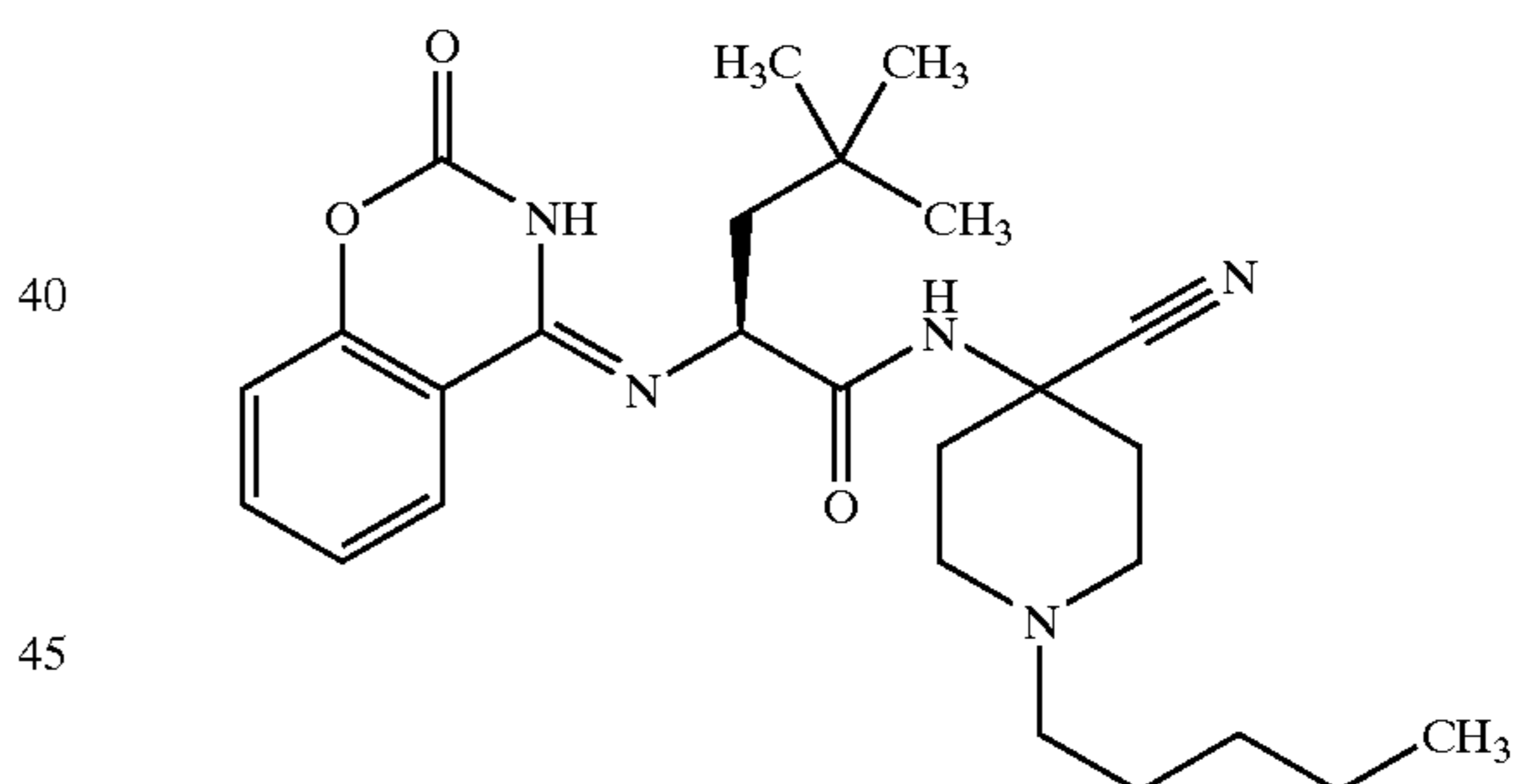
4,4-Dimethyl-2-(2-oxo-2H-benzo[e][1,3]oxazin-4-ylamino)-pentanoic Acid (4-cyano-1-pentyl-piperidin-4-yl)-amide; MS: 468 (M+1)
