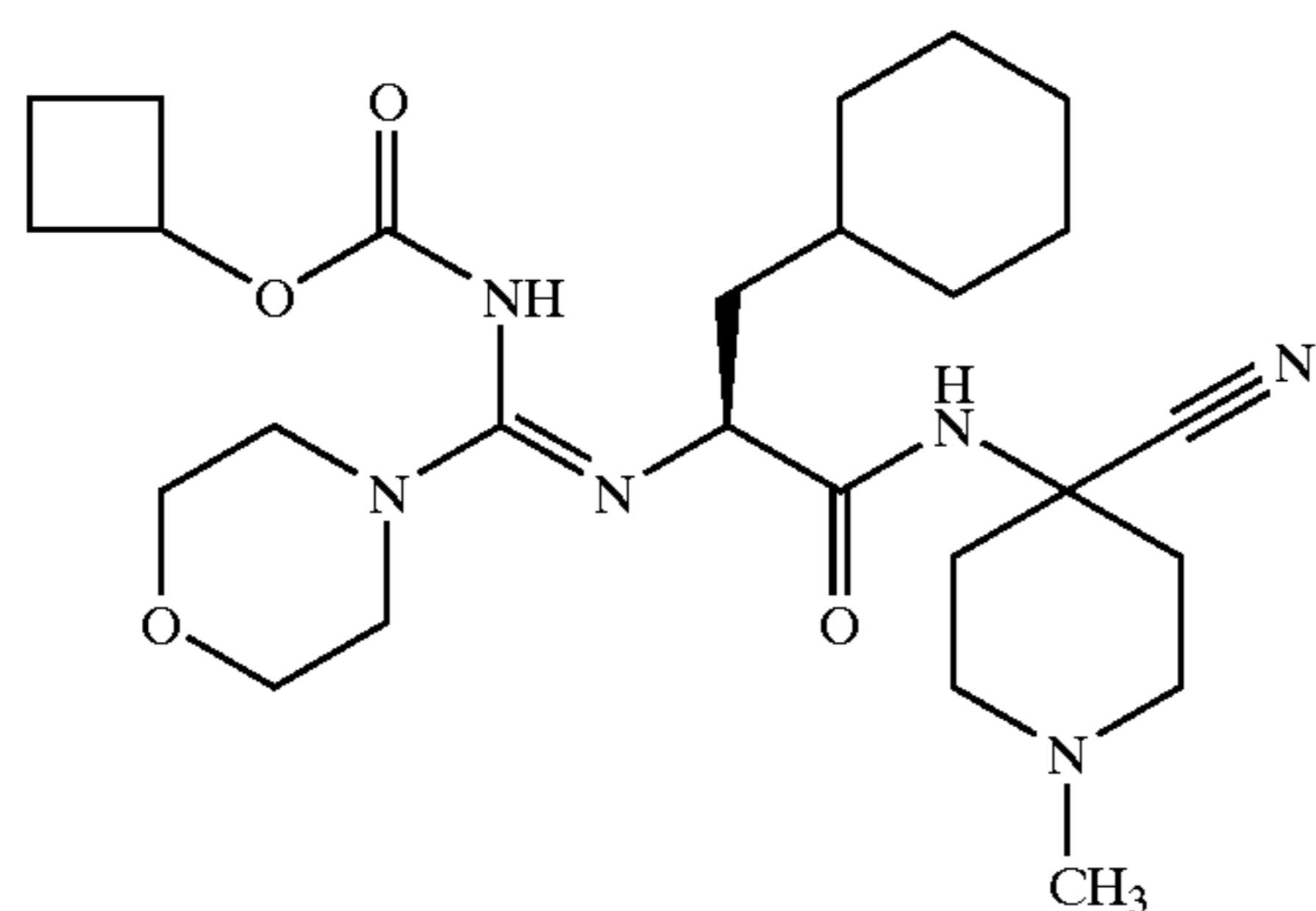
{[-1-(4-Cyano-1-methyl-piperidin-4-ylcarbamoyl)-2-cyclohexyl-ethylamino]-morpholin-4-yl-methylene}-carbamic Acid Cyclobutyl Ester; MS: 503 (M+1)
