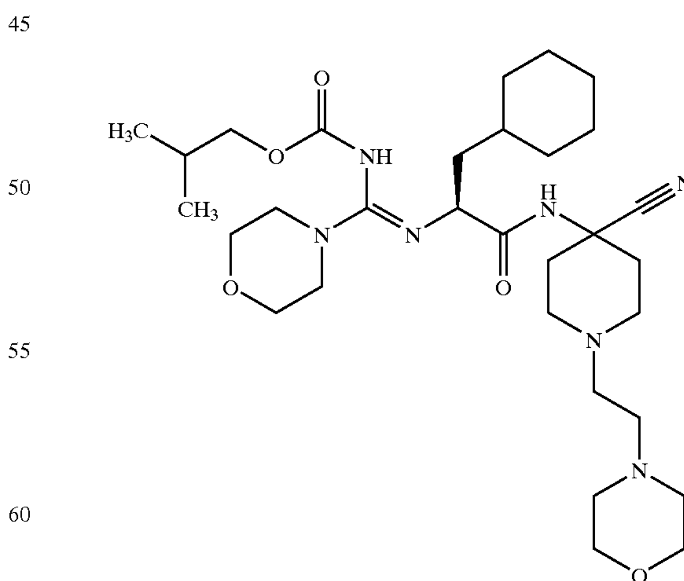
(({1-[4-Cyano-1-(2-morpholin-4-yl-ethyl)-piperidin-4-ylcarbamoyl]-2-cyclohexyl-ethylamino}-morpholin-4-yl-methylene)-carbamic Acid Isobutyl Ester; MS: 604 (M+1)
