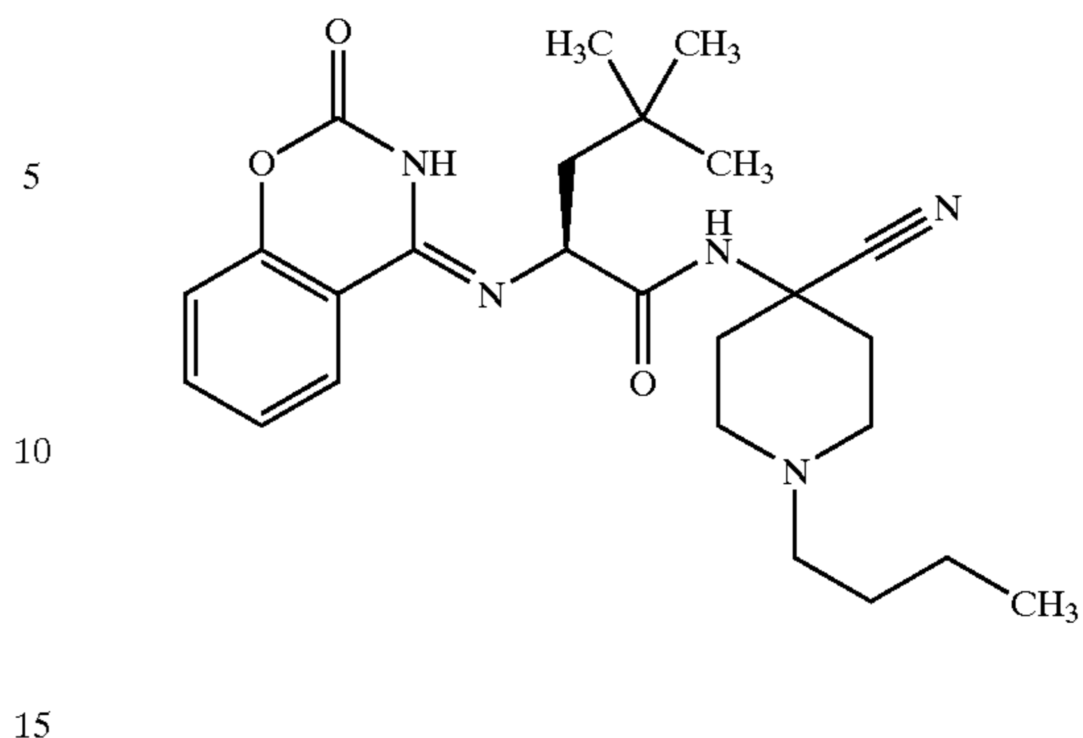
4,4-Dimethyl-2-(2-oxo-2H-benzo[e][1,3]oxazin-4-ylamino)-pentanoic Acid (1-butyl-4-cyano-piperidin-4-yl)-amide; MS: 454 (M+1)
