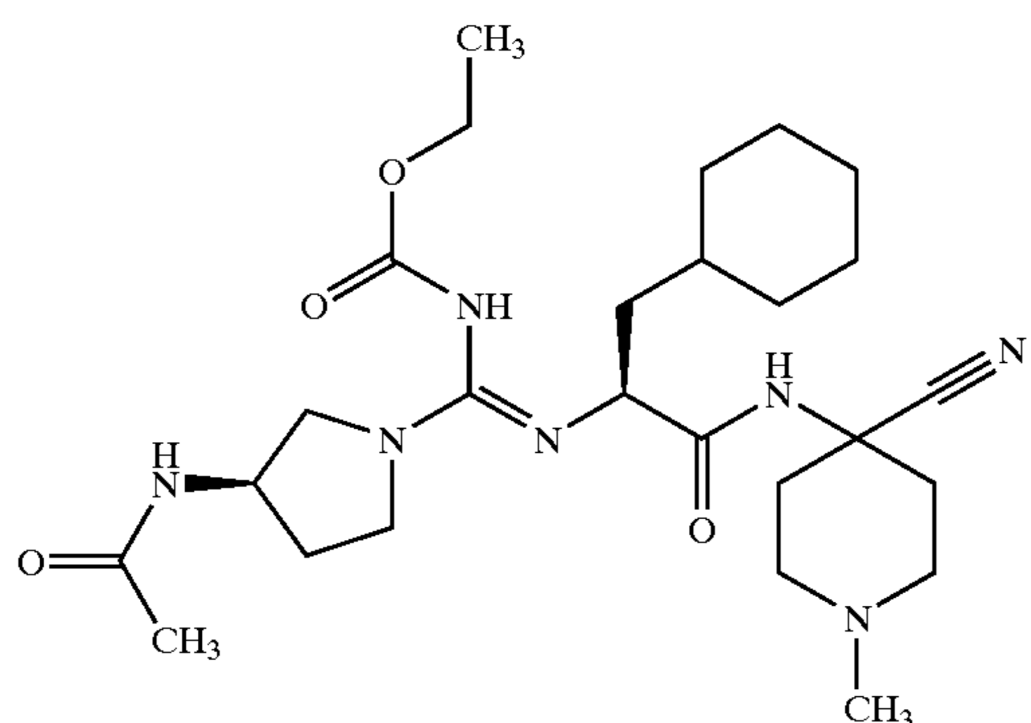
{(3-Acetylamino-pyrrolidin-1-yl)-[1-(4-cyano-1-methyl-piperidin-4-ylcarbonyl)-2-cyclohexylethylimino]-methyl}-carbamic Acid Ethyl Ester; MS: 518 (M+1).
