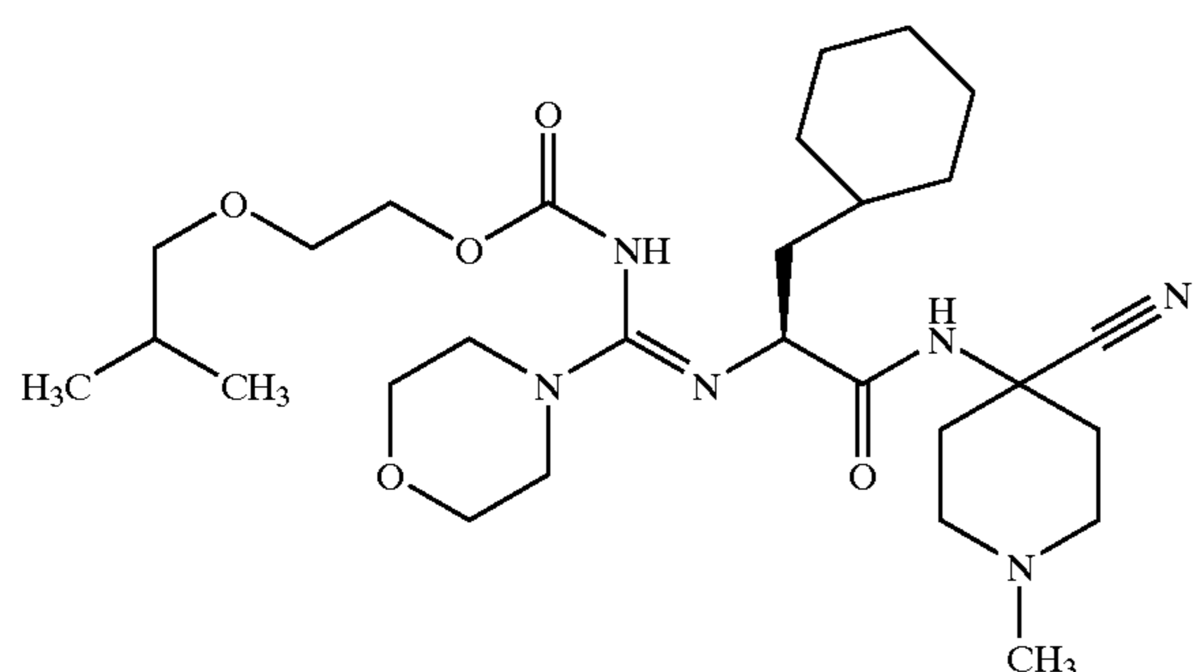
{[1-(4-Cyano-1-methyl-piperidin-4-ylcarbonyl)-2-cyclohexyl-ethylimino]-morpholin-4-yl-methyl}-carbamic Acid 2-isobutoxy-ethyl Ester; MS: 549 (M+1)
