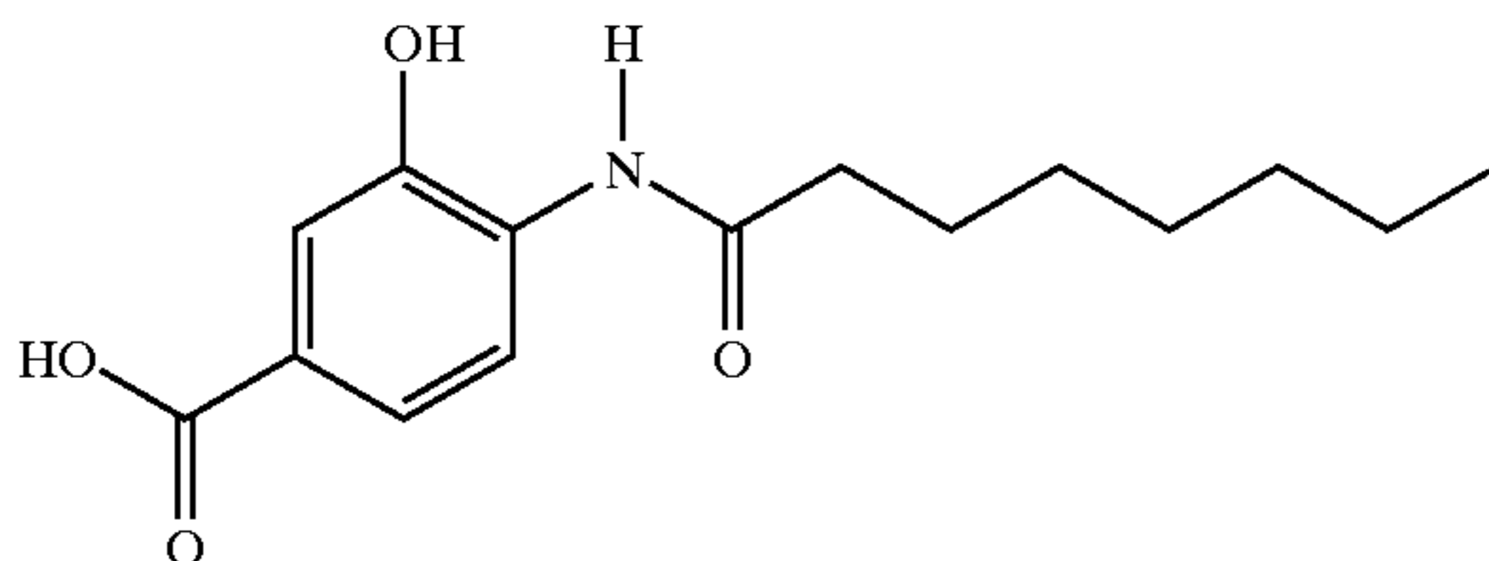
4-octanoylamino-3-hydroxybenzoic acid
