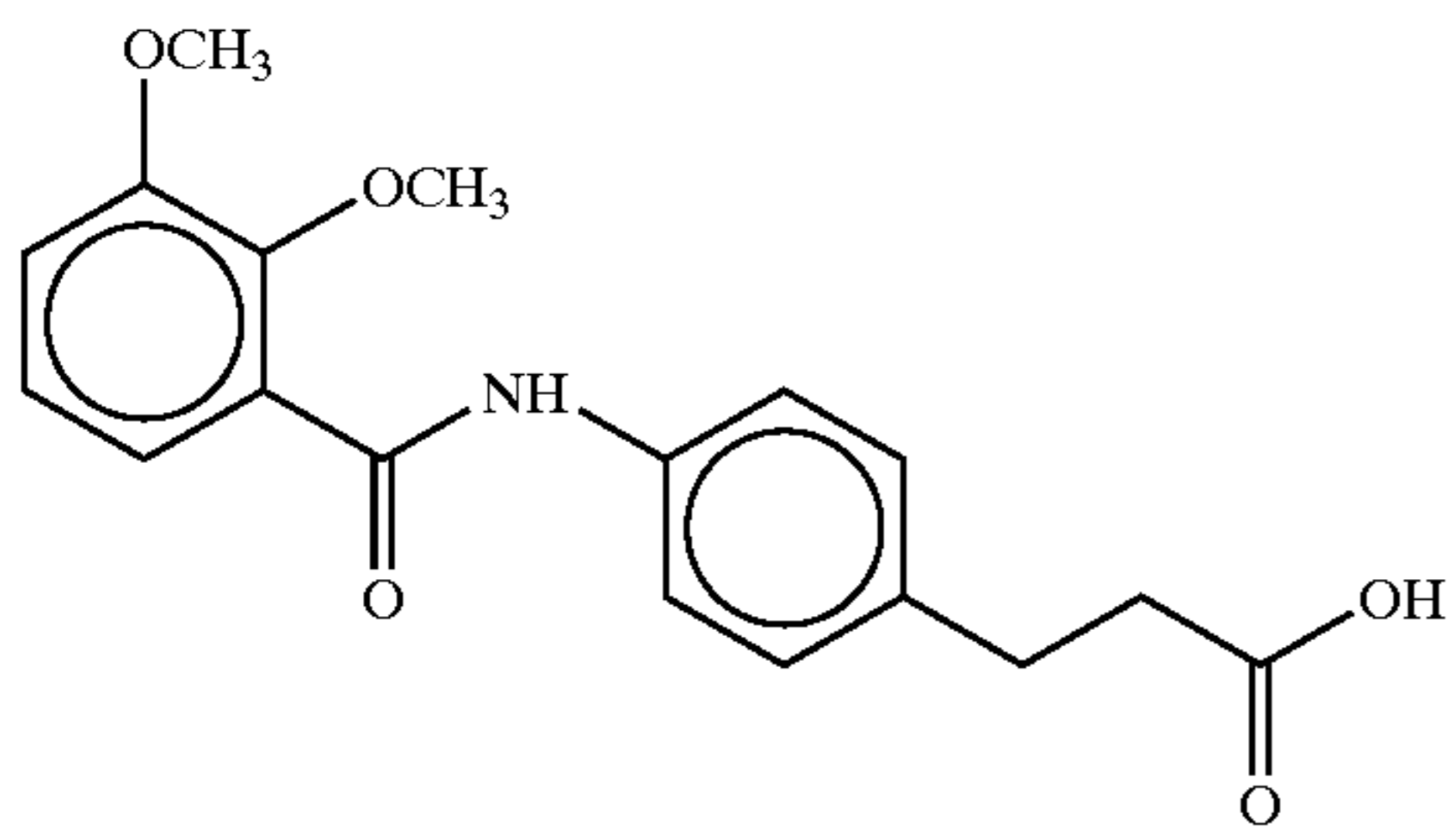
3-[4-(2,3-dimethoxybenzoyl)aminophenyl]propionic acid
