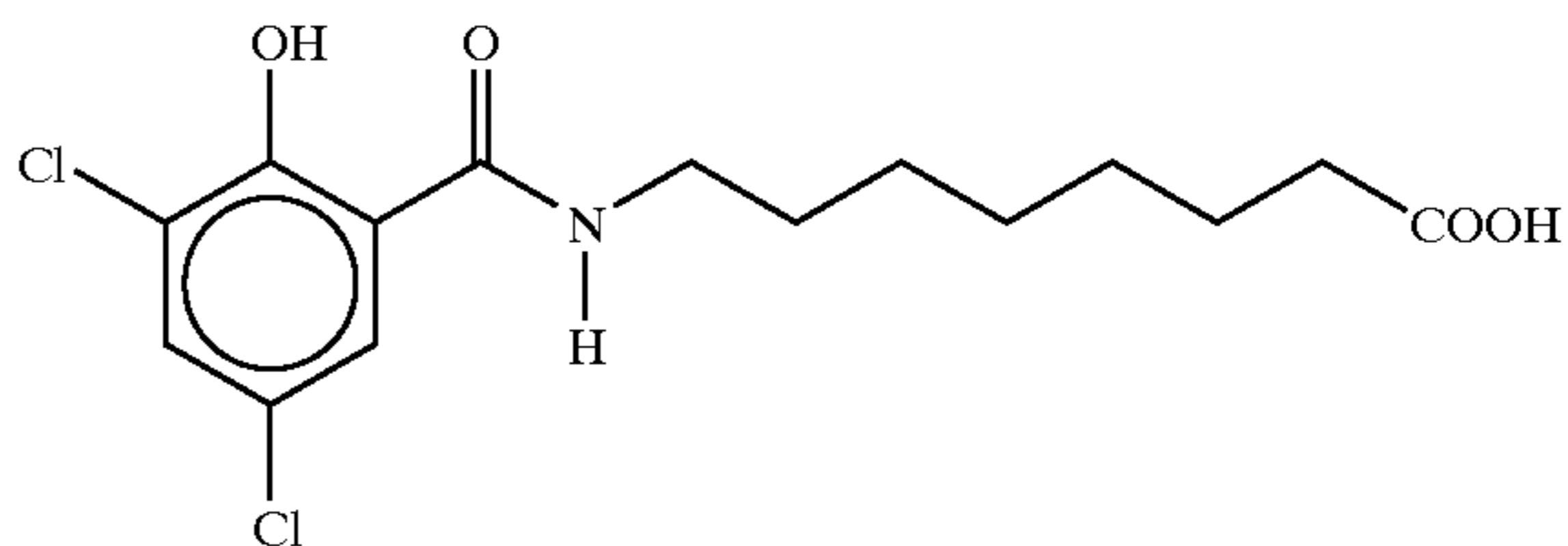
8-[N-(2-acetoxy-3,5-dichlorobenzoyl)aminocaprylic acid
