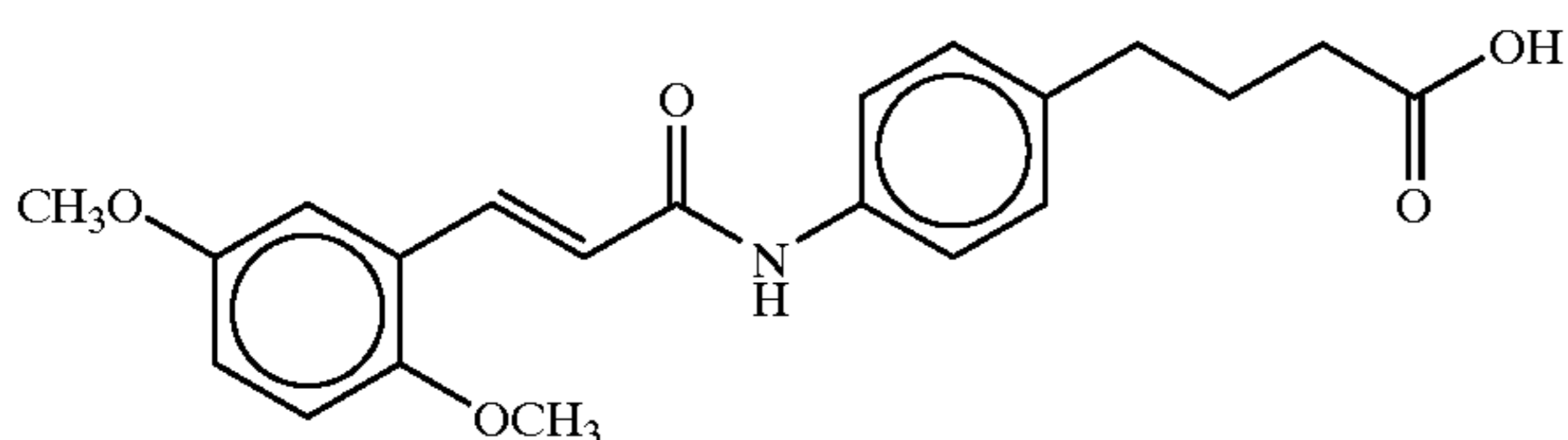
4-(4-(2,5-dimethoxycinnamoyl)aminophenyl)butyric acid
