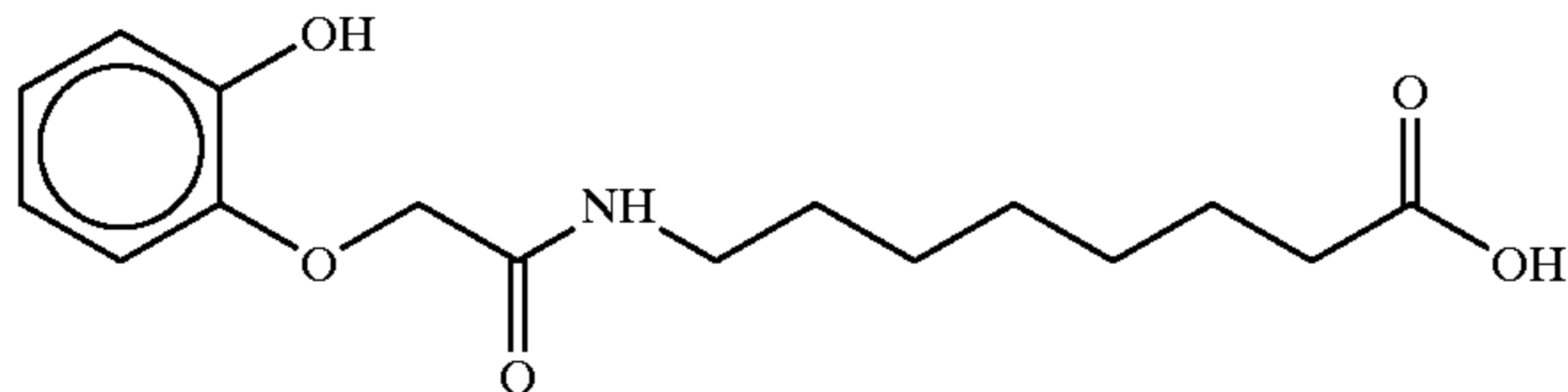
7-(2-hydroxyphenoxyacetyl)aminocaprylic acid
