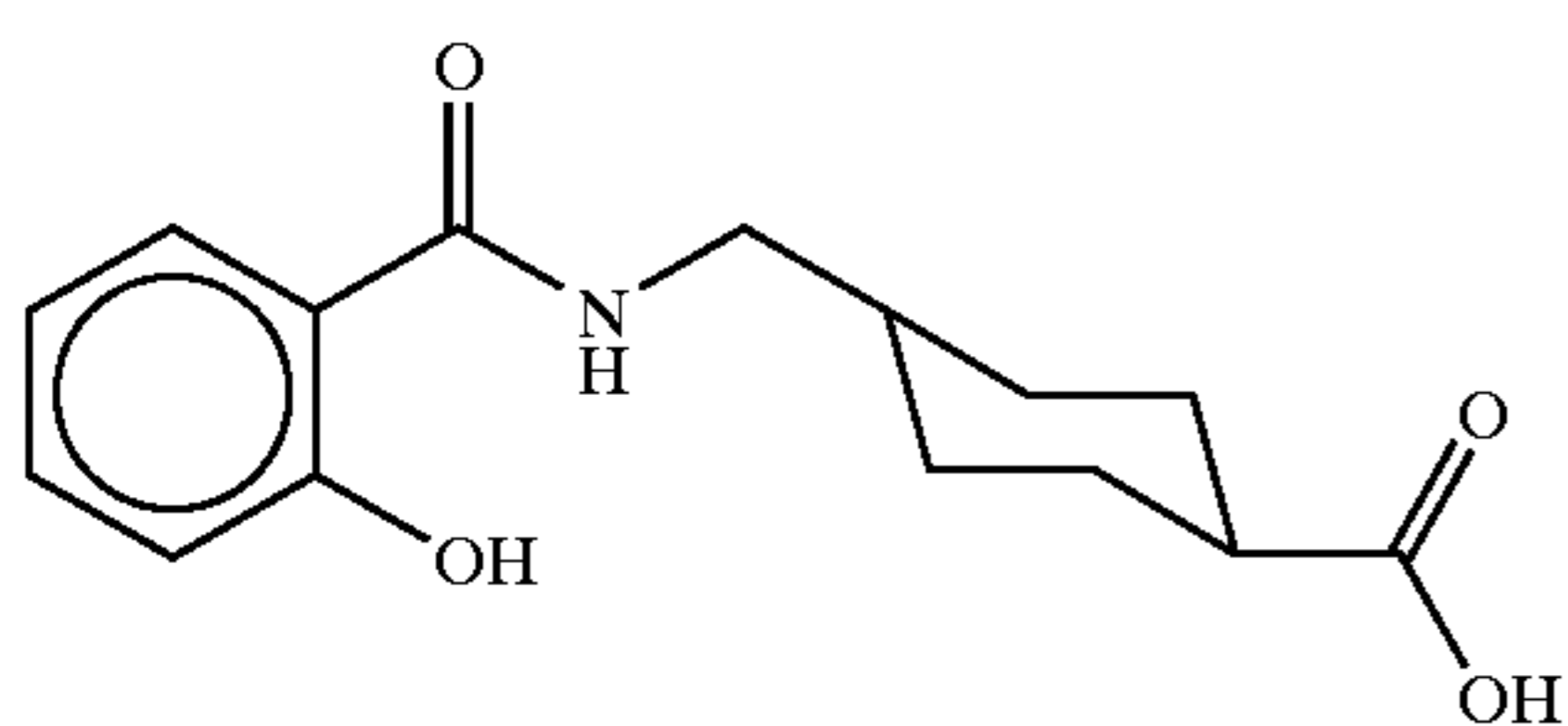
trans-4-(N-salicyloylaminomethyl)cyclohexanecarboxylic acid
