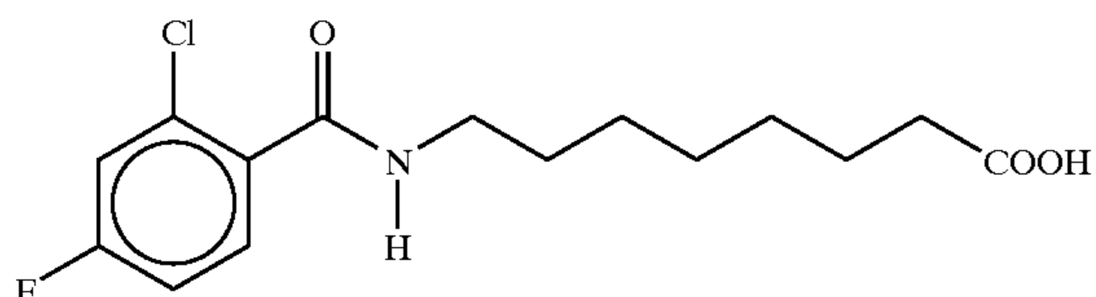
8-(N-2-chloro-4-fluorobenzoyl)aminocaprylic acid
