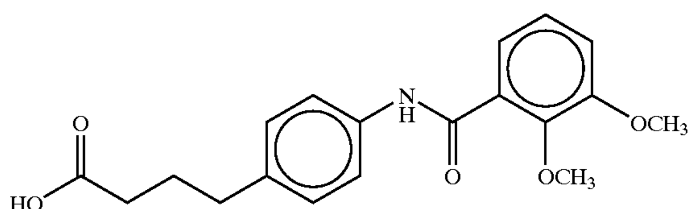
4-(4-(2,3-dimethoxybenzoyl)aminophenyl)butyric acid
