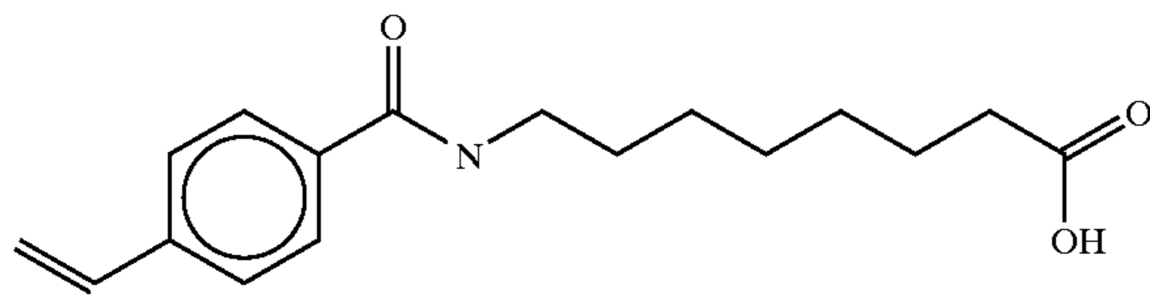
8-(vinylbenzoyl) aminocaproic acid
