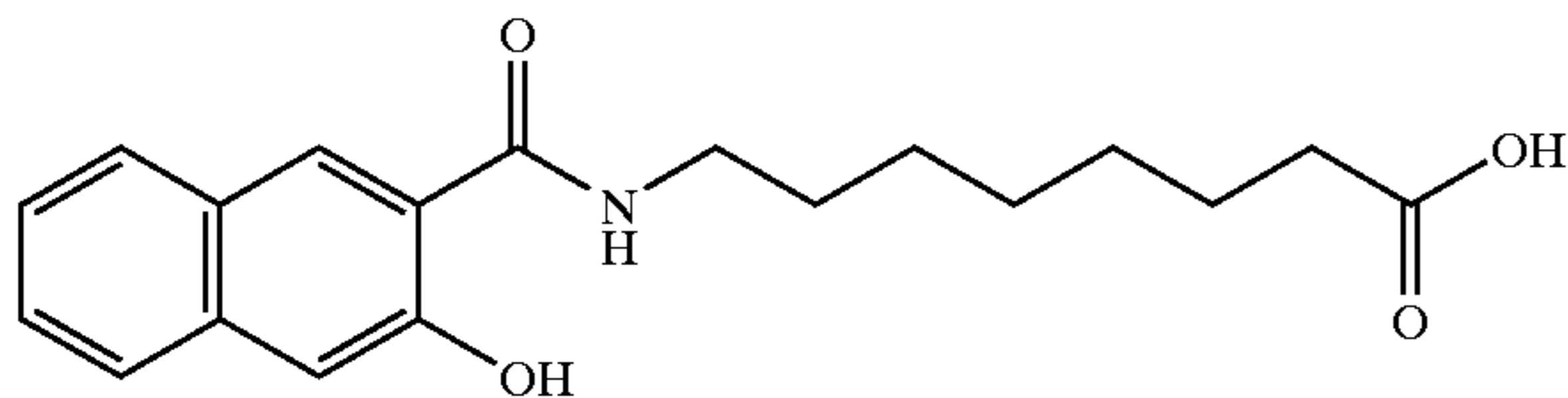
8-(3-hydroxy-2-naphthoyl)aminocaprylic acid
