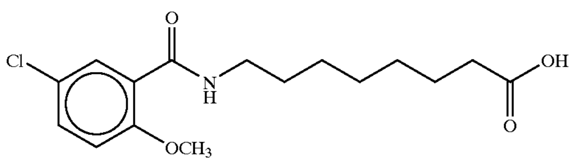
8-(5-chloro-o-anisoyl)aminocaproic acid
