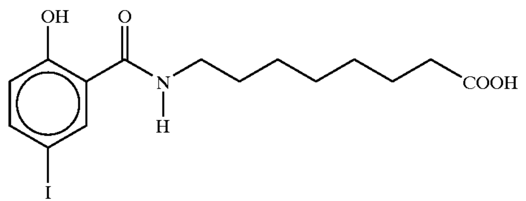
8-(N-(2-hydroxy-5-iodobenzoyl)aminocaprylic acid
