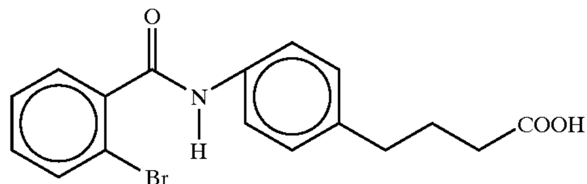
4{4-[N-2-bromobenzoyl]aminophenyl}butyric acid
