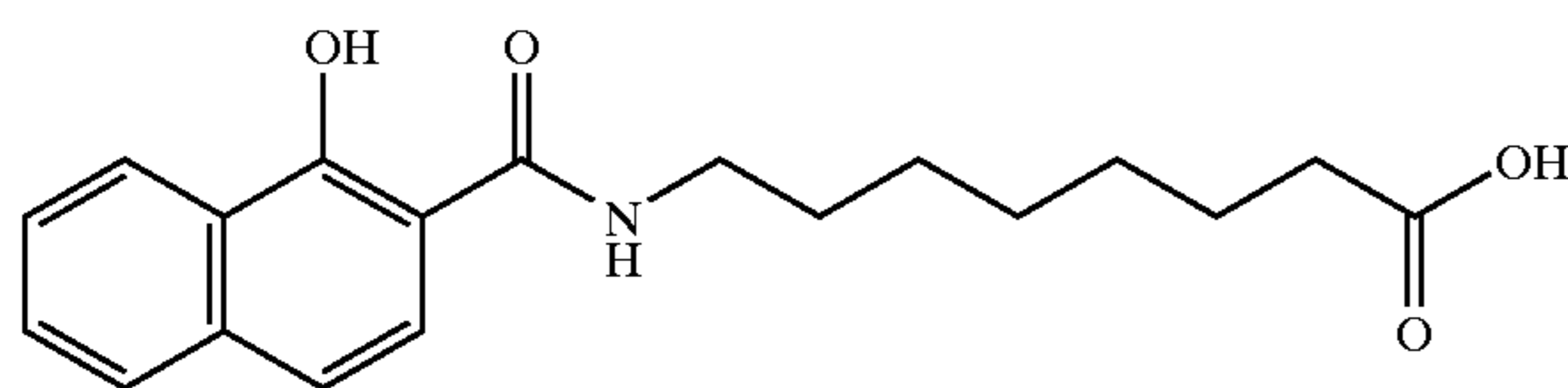
8-(N-1-hydroxy-2-naphthoyl)aminocaprylic acid
