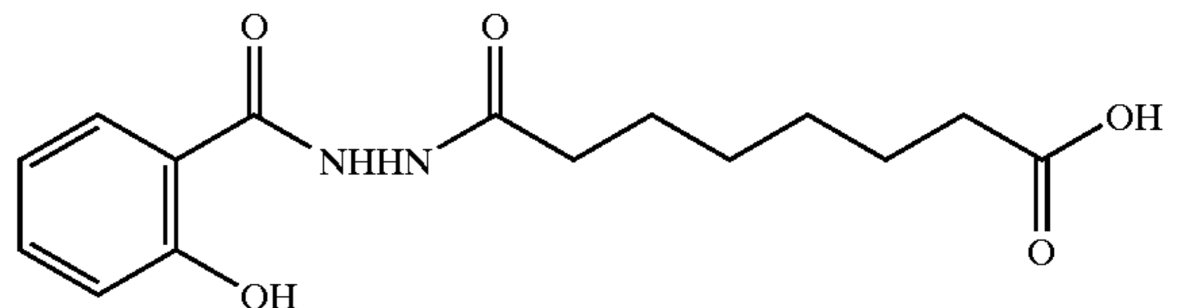
1-salicyloyl-2-suberyl hydrazide
