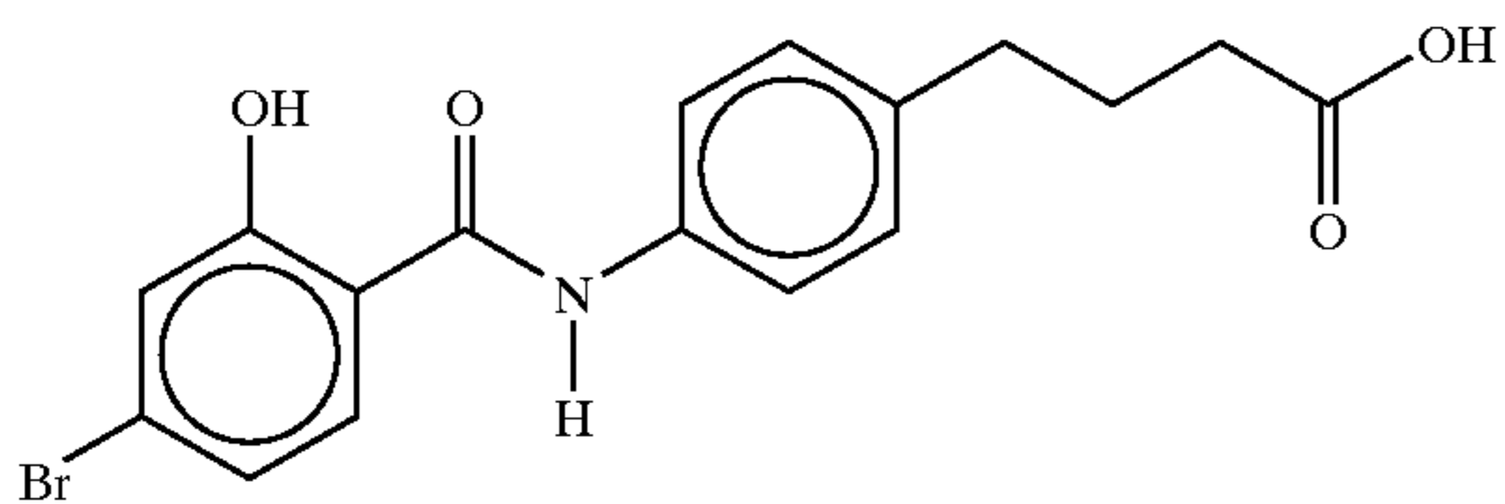
4-[-N-(2-hydroxy-4-bromobenzoyl)aminophenyl]butyric acid
