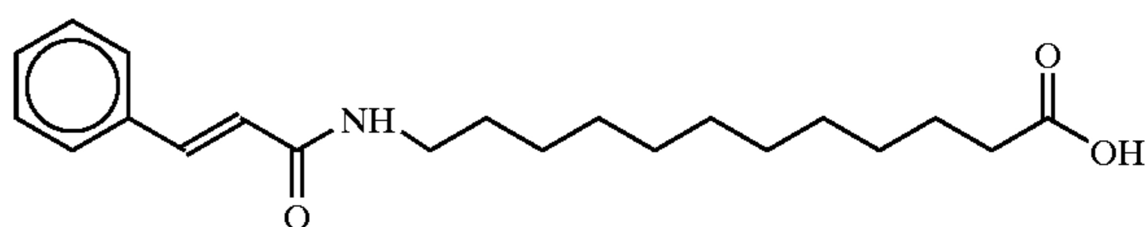
12-cinnamoyldodecanoic acid
