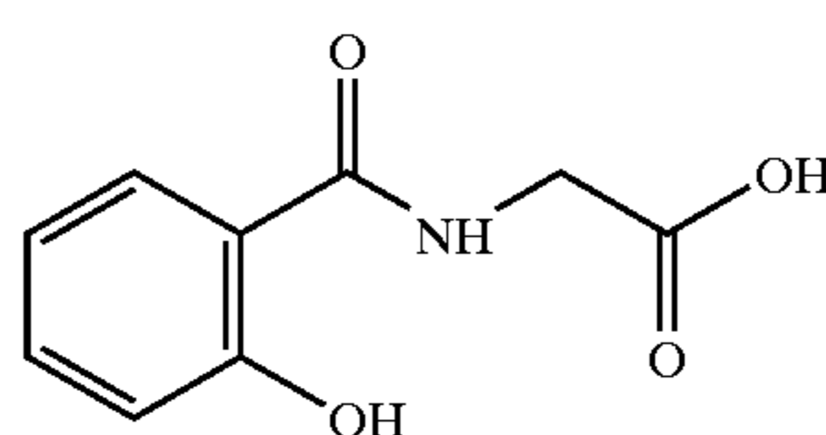
salicyloylglycine
