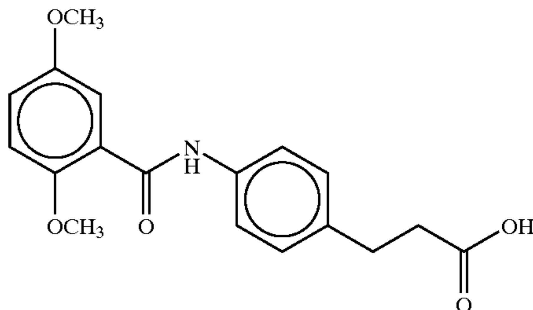
3-(4-(2,5-dimethoxybenzoyl)aminophenyl)propionic acid
