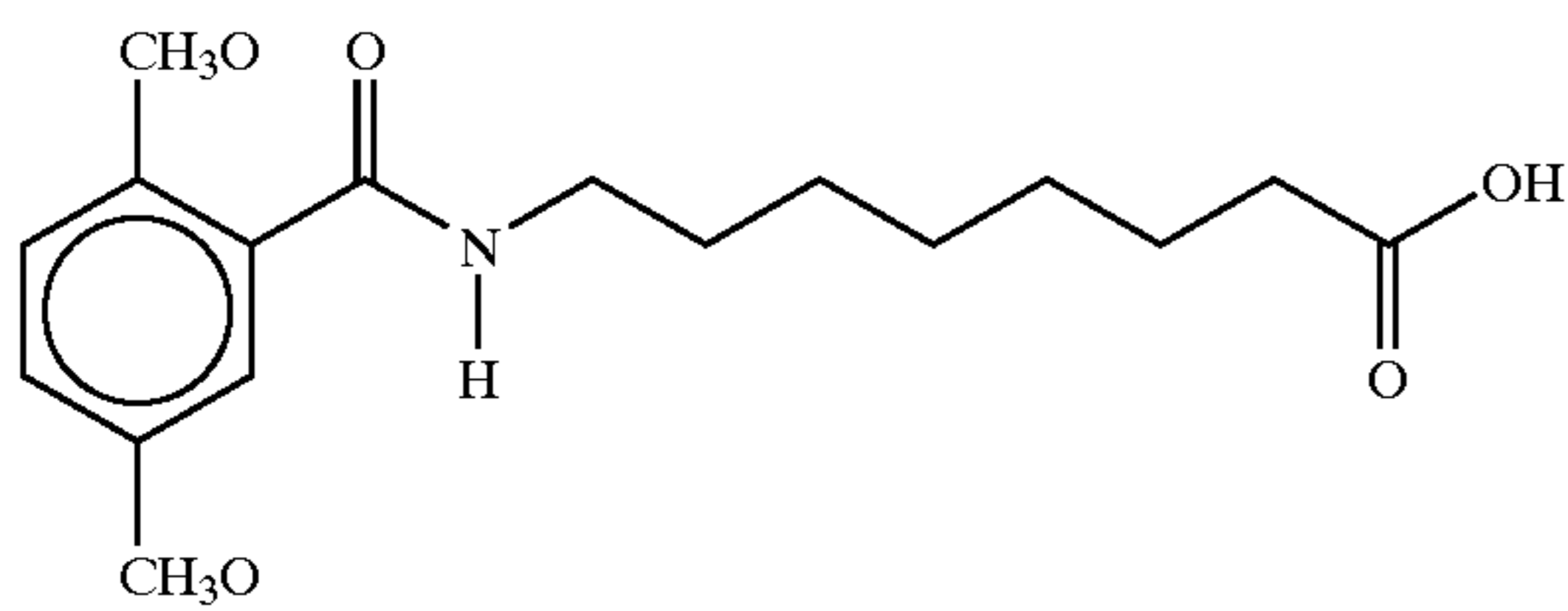
8-(N-2,5-Dimethoxybenzoyl) aminocaprylic acid
