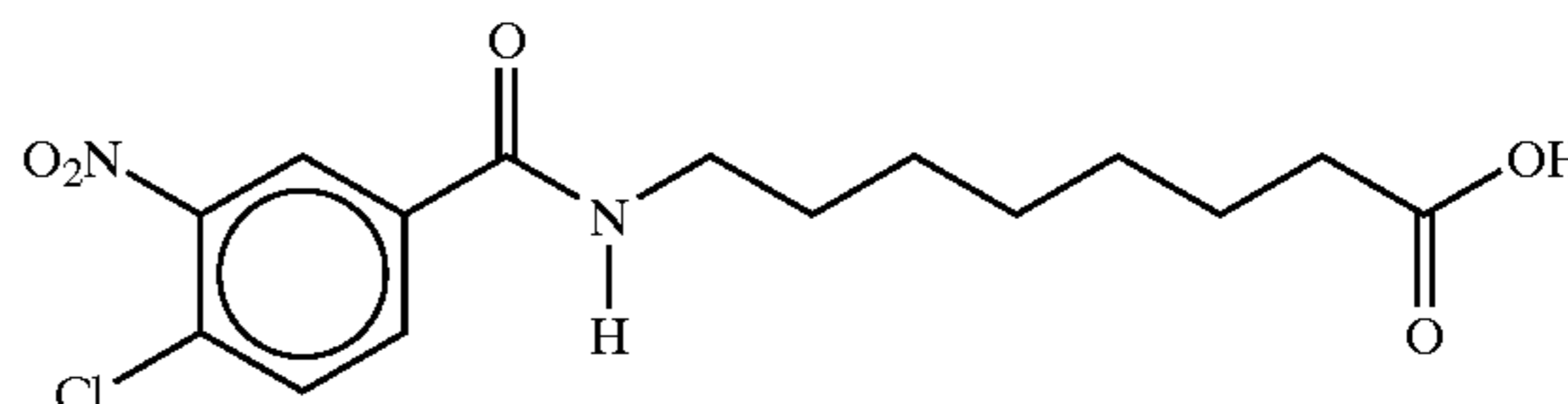
8-(4-chloro-3-nitrobenzoyl)aminocaprylic acid
