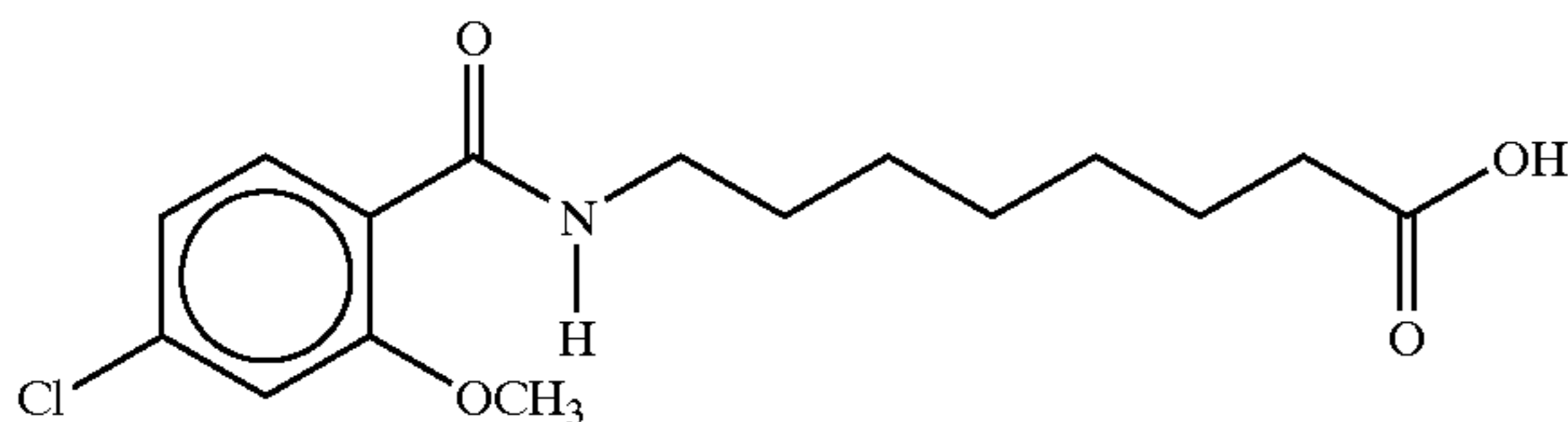
8-(4-chloro-o-anisoyl)aminocaprylic acid
