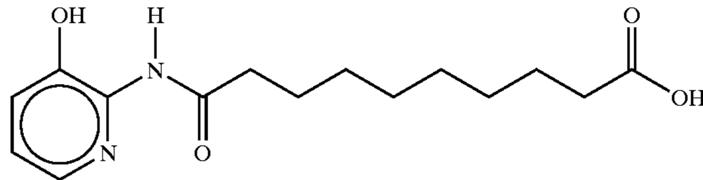
9-[2-(3-hydroxy)pyridylaminocarbonyl]nonanoic acid
