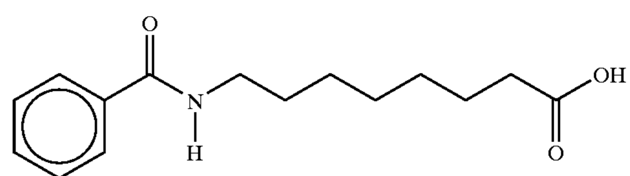
8-(N-benzoyl)aminocaprylic acid
