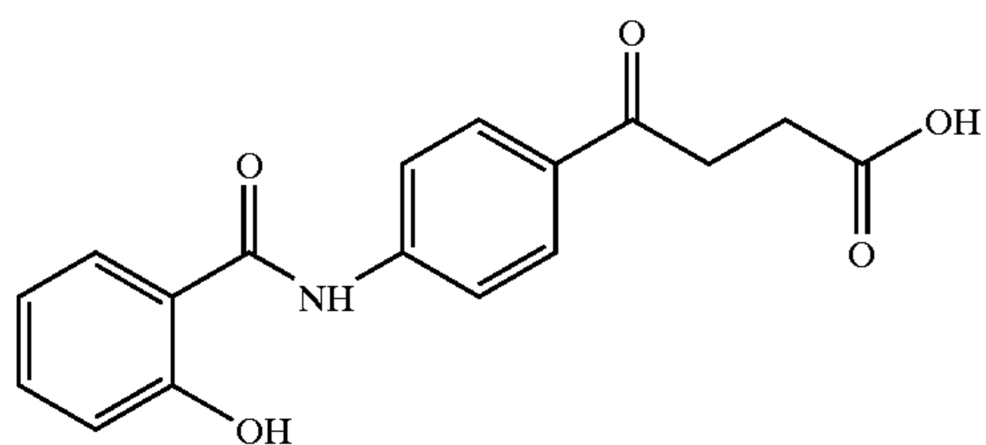
4-(4-salicyloylamino)phenyl-4-oxobutyric acid
