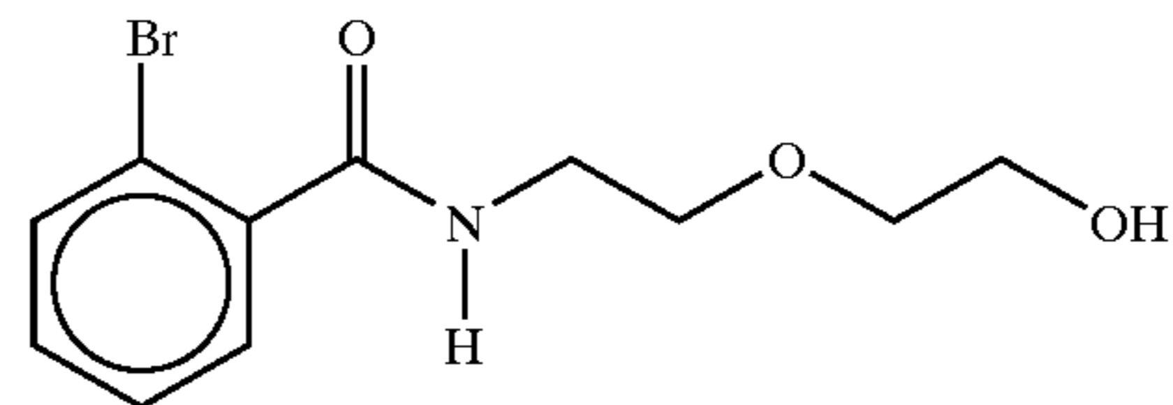
2-[N-(2-bromobenzoyl)aminoethoxy]ethanol
