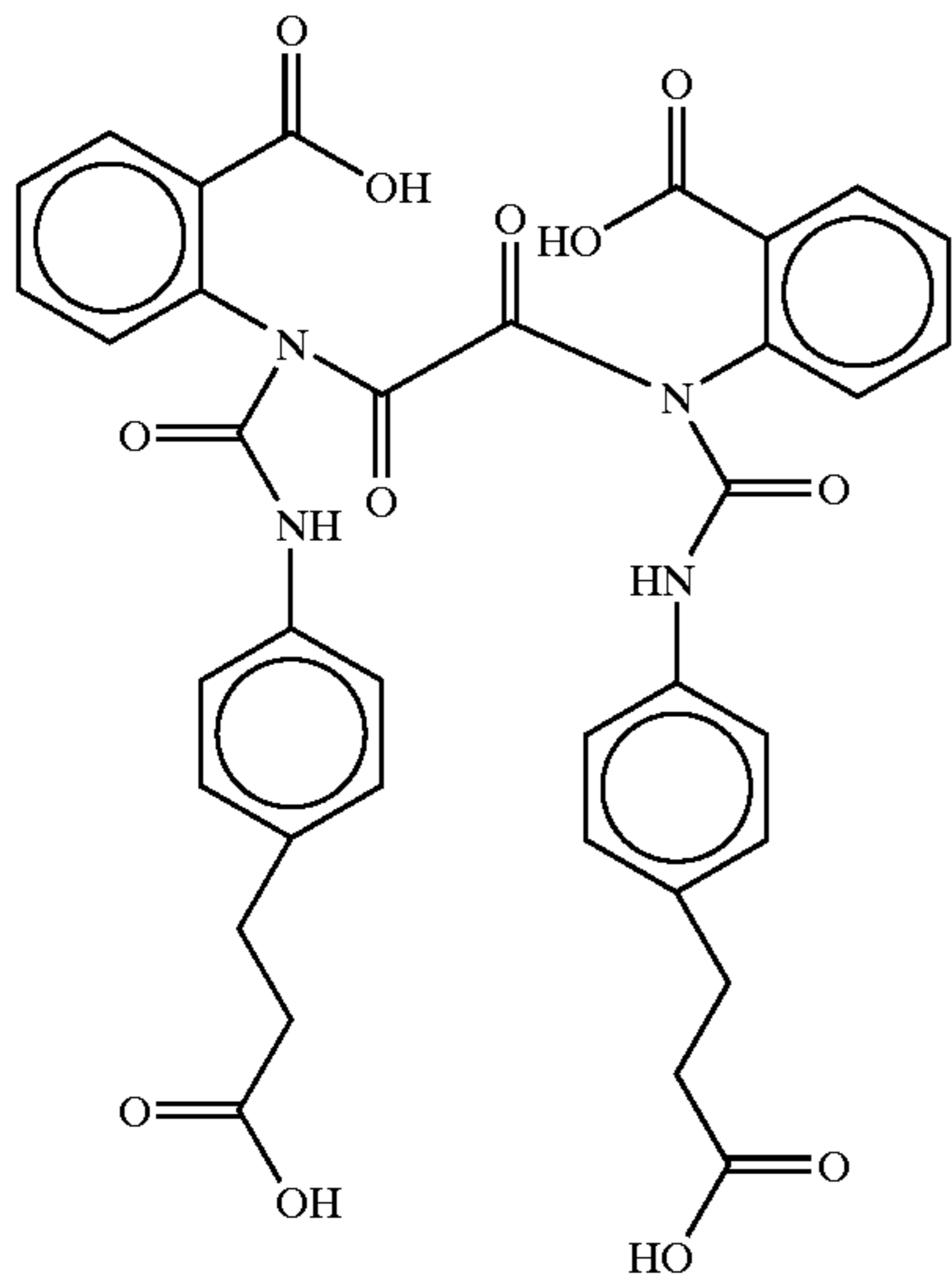
Bis(N-2-carboxyphenyl-N-(N'-3(4-aminophenyl)propionic acid)urea)oxalyldiamide
