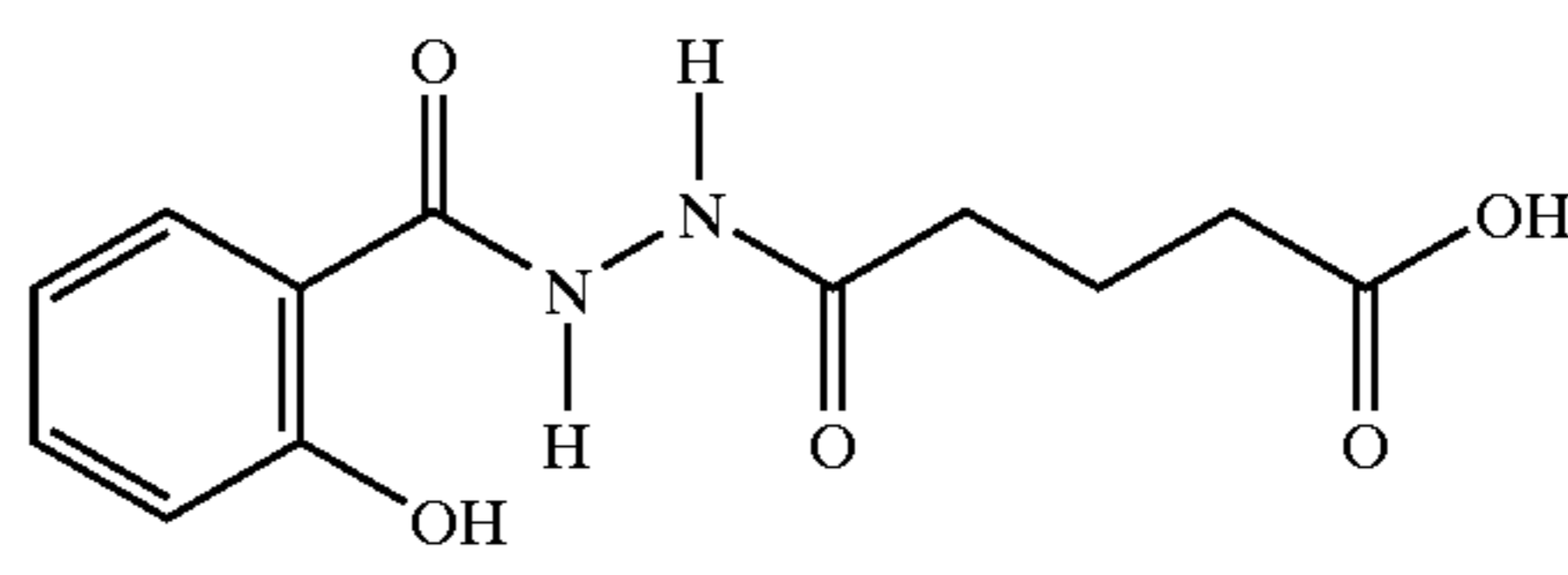
1-salicyloyl-2-glutaryl hydrazide
