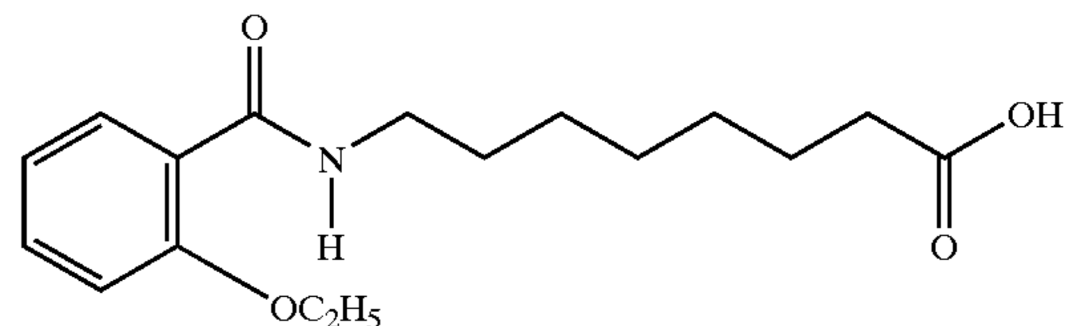
8-(2-ethoxybenzoyl)aminocaprylic acid
