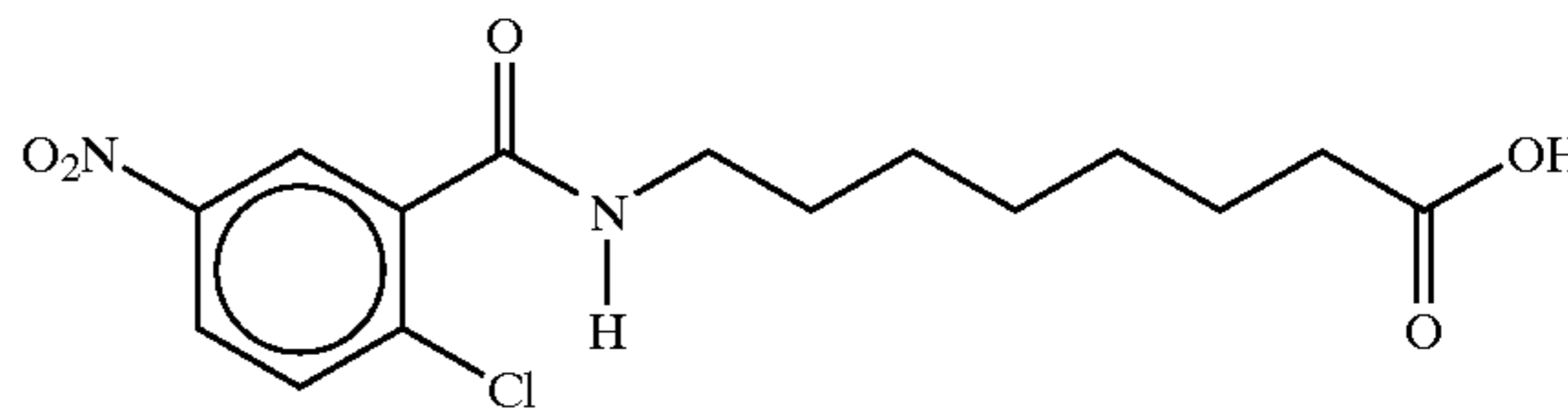
8-(2-chloro-5-nitrobenzoyl)aminocaprylic acid
