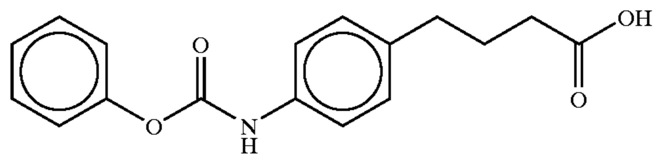
4-(4-phenyloxycarbonylamino)phenyl butyric acid
