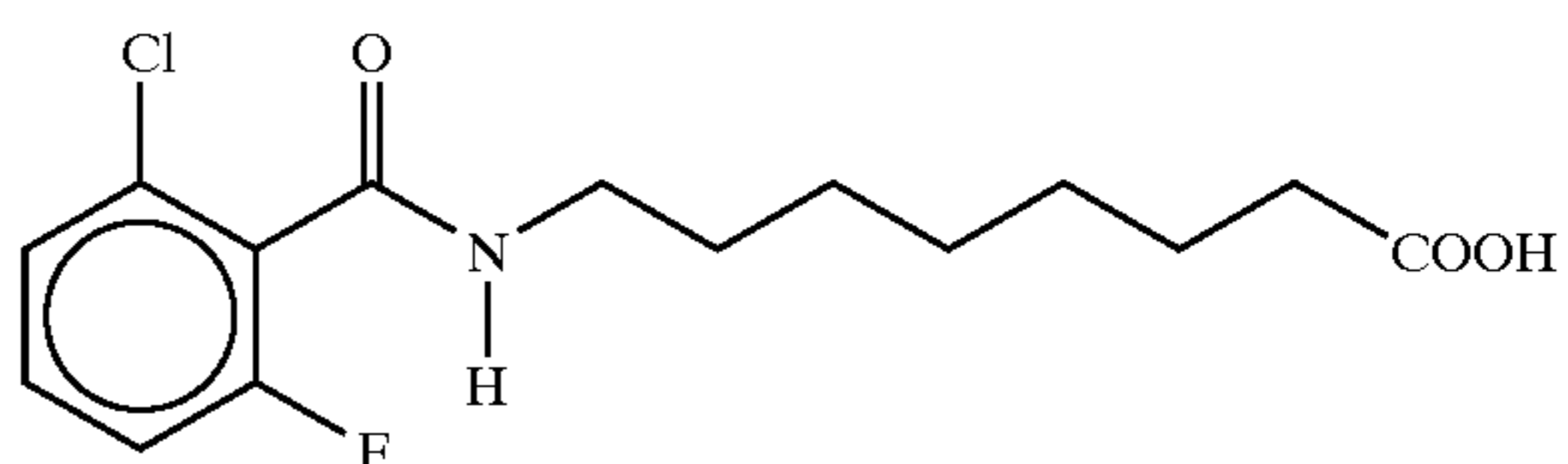
8-N-(2-chloro-6-fluorobenzoyl)aminocaprylic acid
