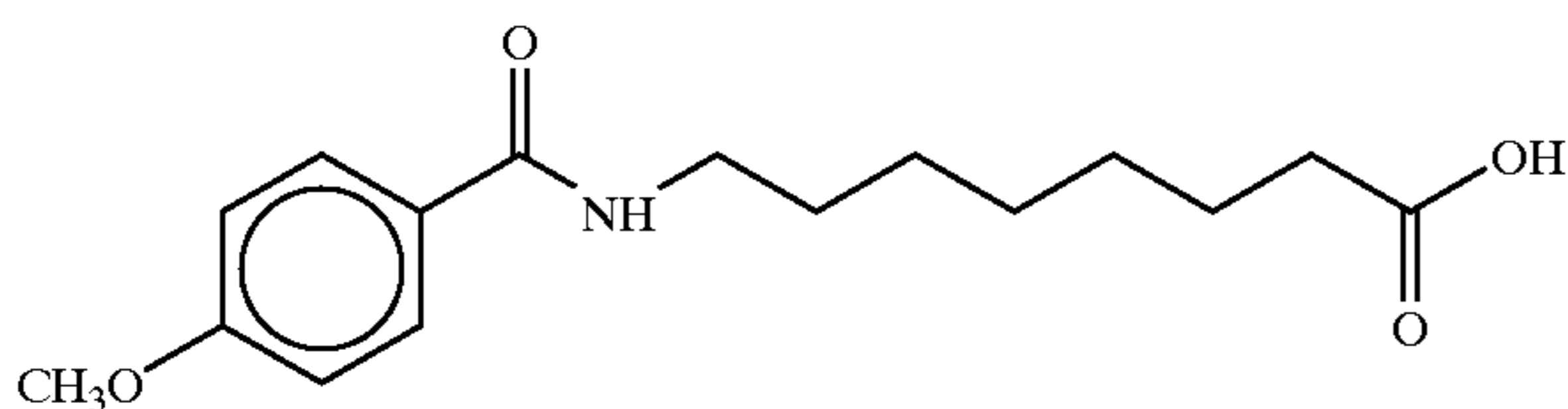
8-(p-anisoyl)aminocaprylic acid
