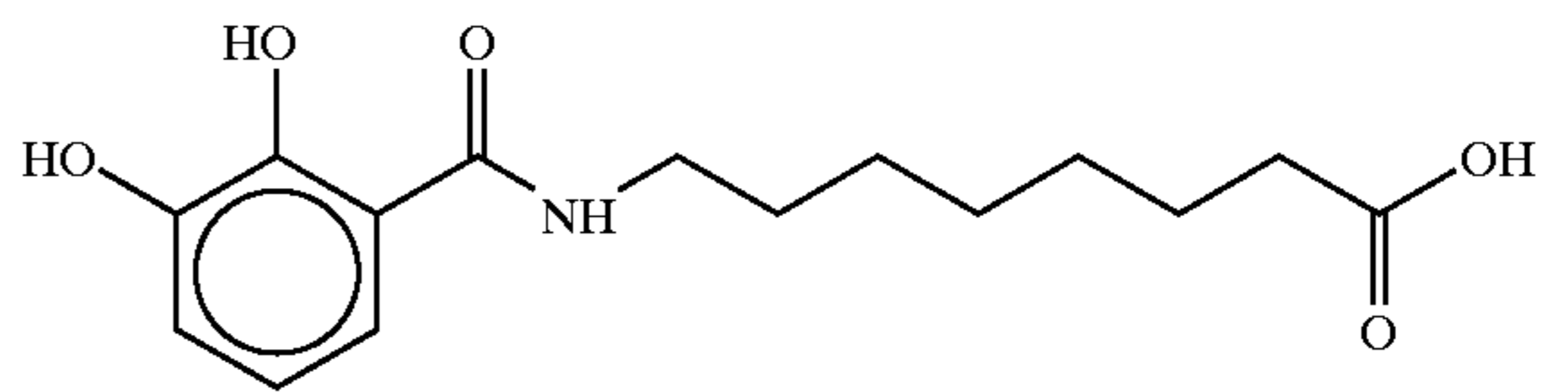
8-(N-(2,3-Dihydroxybenzoyl)aminocaprylic acid
