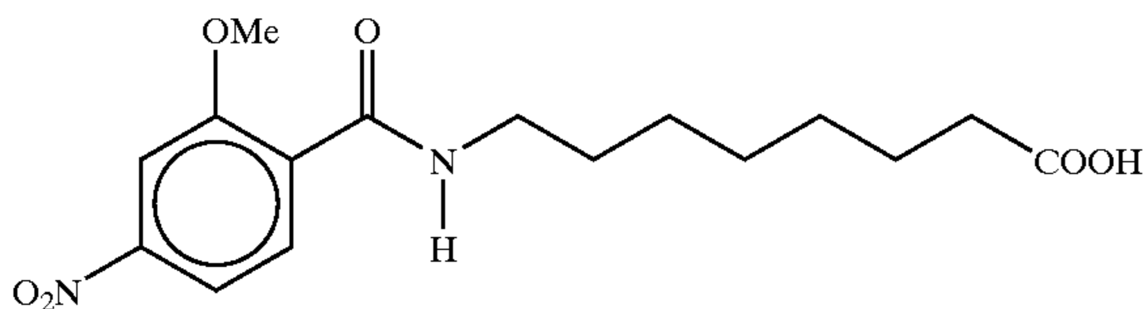
8-N-(2-methoxy-4-nitrobenzoyl)aminocaprylic acid
