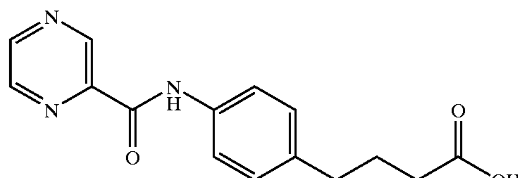
4-(4-(2-pyrazinecarbonyl)aminophenyl)butyric acid
