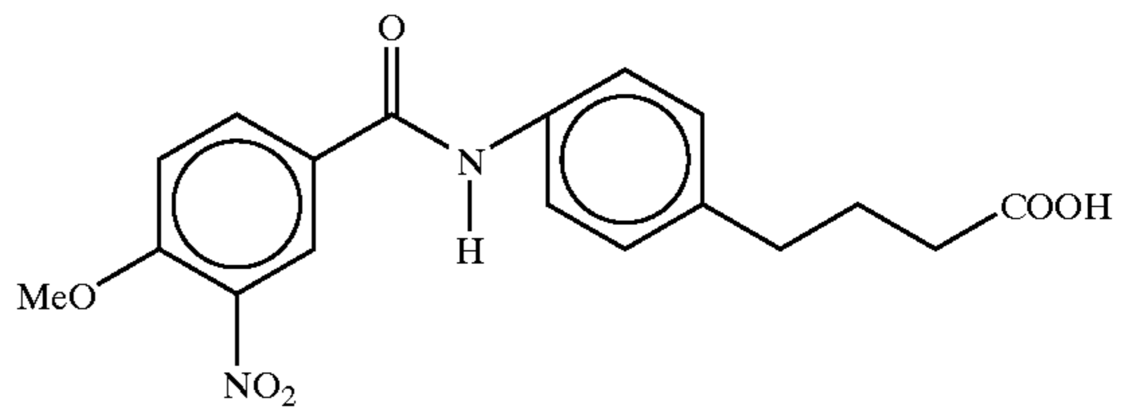
4-[4-N-(4-methoxy-3-nitrobenzoyl)aminophenyl]butyric acid
