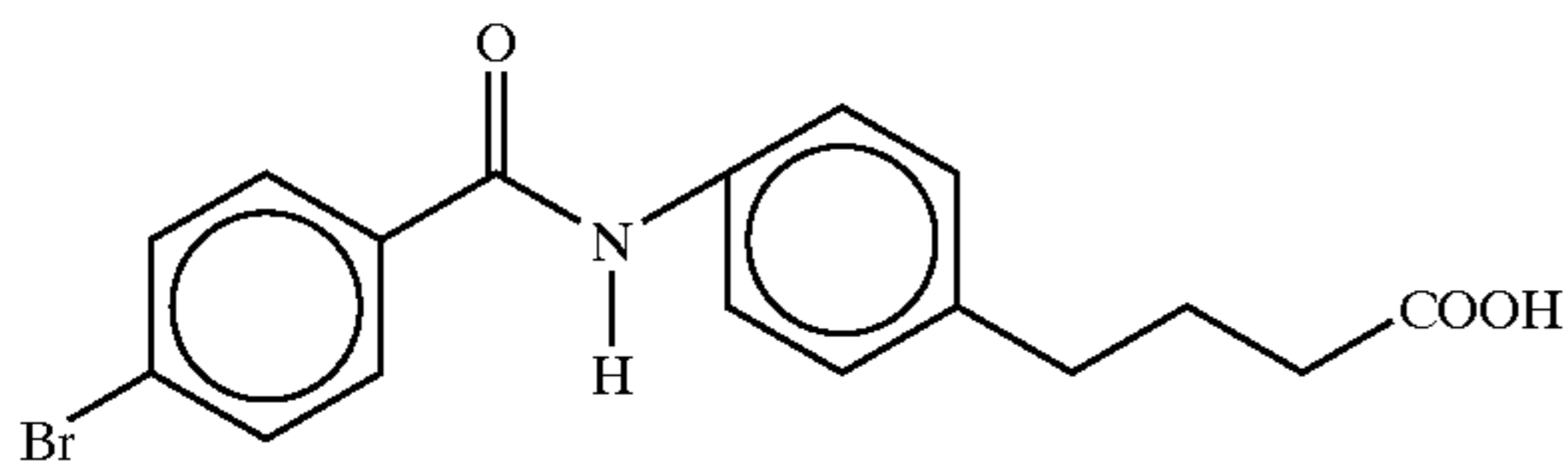
4-[4-(N-(4-bromobenzoyl)aminophenyl)]butyric acid
