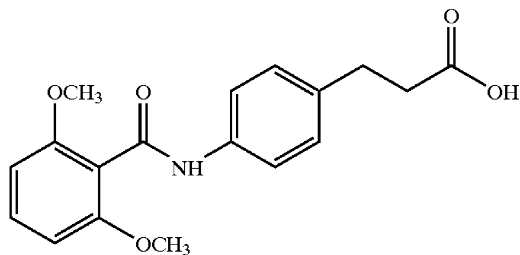
3-(4-(2,6-dimethoxybenzoyl)aminophenyl)propionic acid
