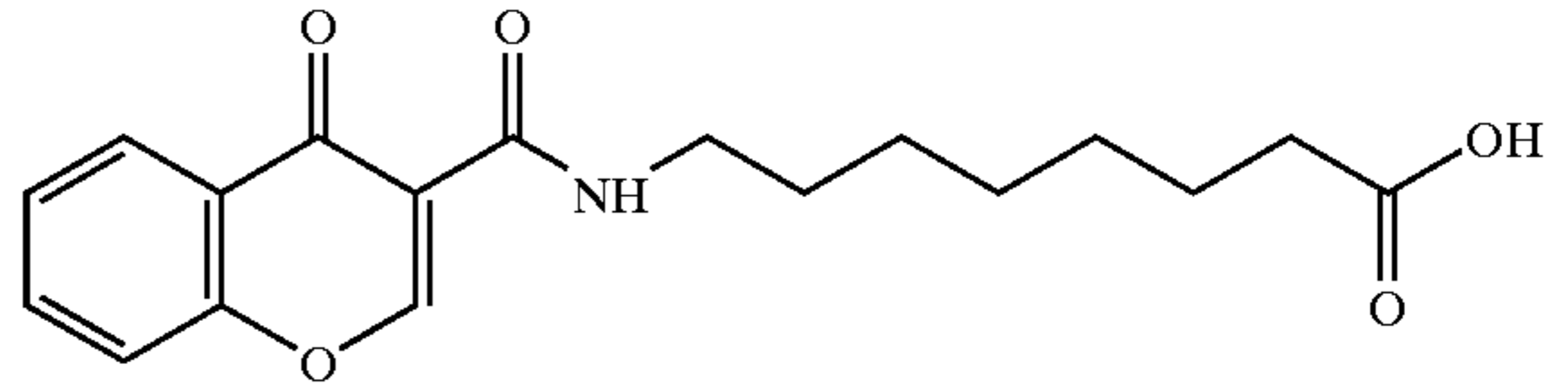
8-(chromomone-3-carbonyl) aminocaproic acid
