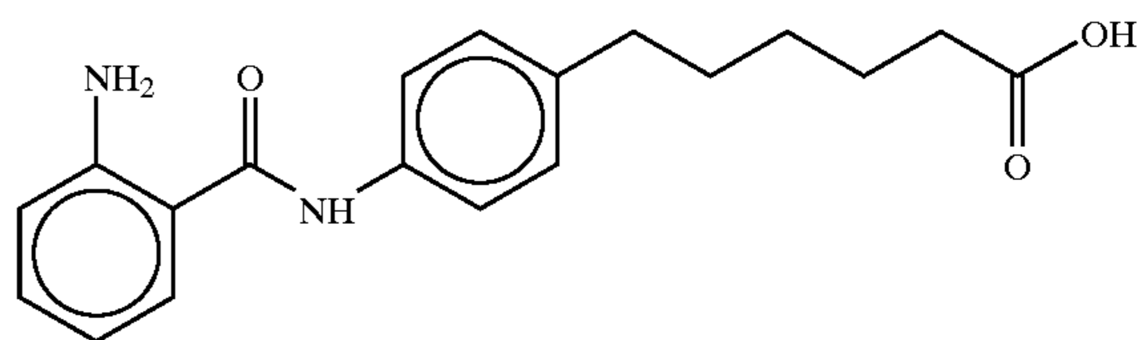
6-(4-(N-2-aminobenzoyl)aminophenyl)hexanoic acid
