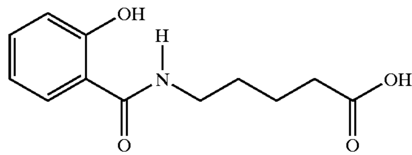
5-(N-salicyloylamino) valeric acid
