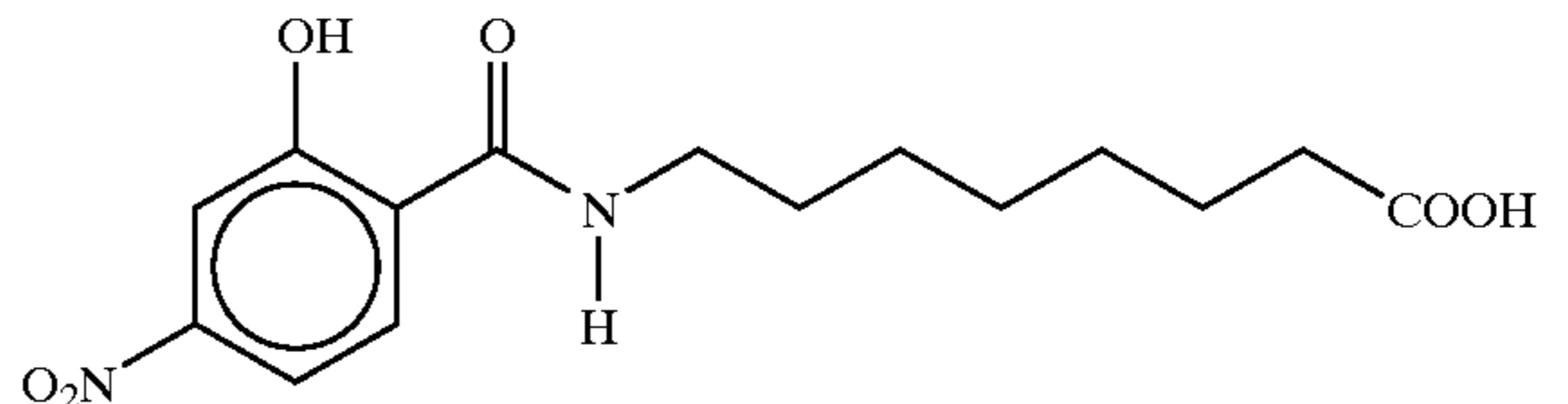
8-(N-(2-hydroxy-4-nitrobenzoyl)aminocaprylic acid
