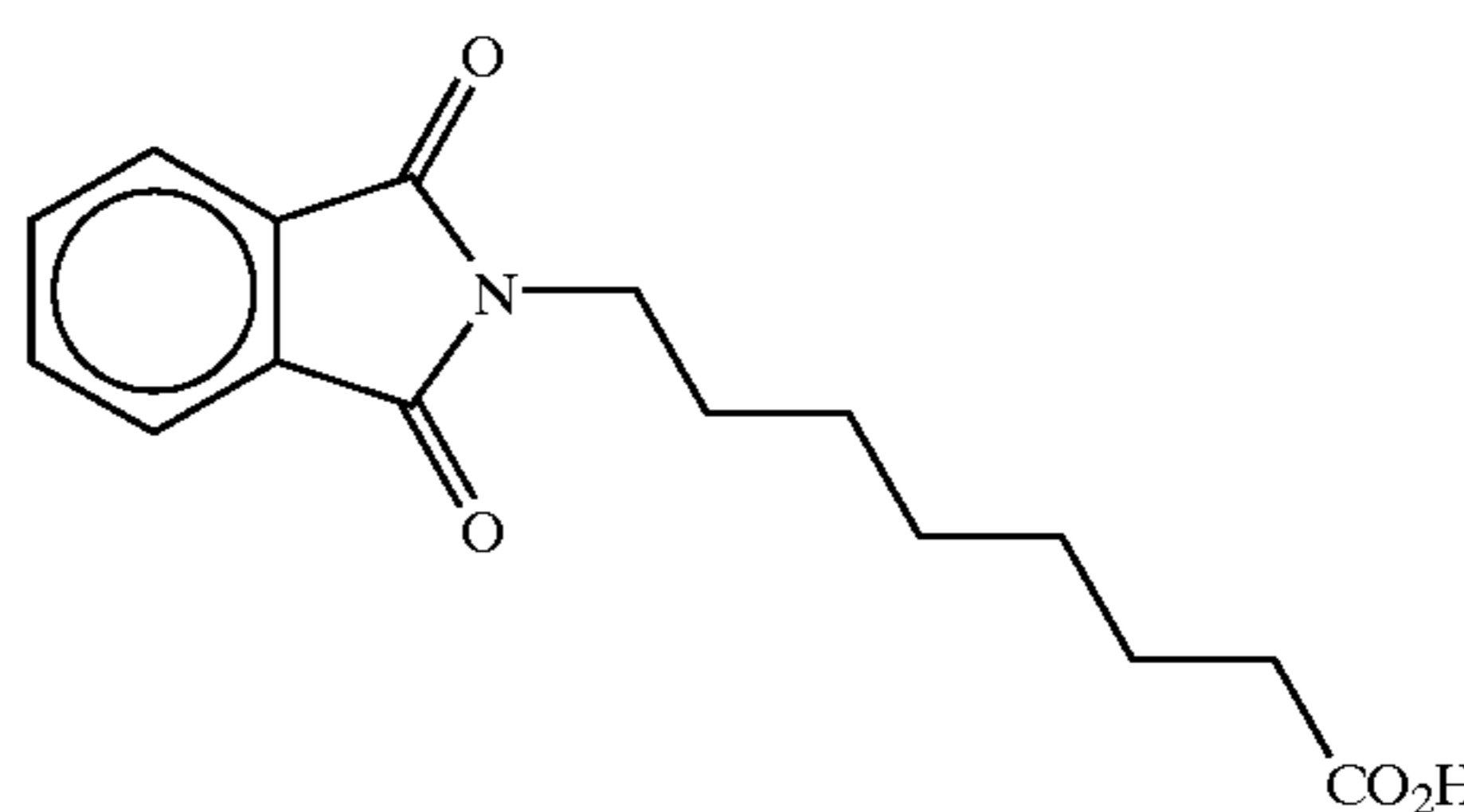
8-(phthalimido)caprylic acid
