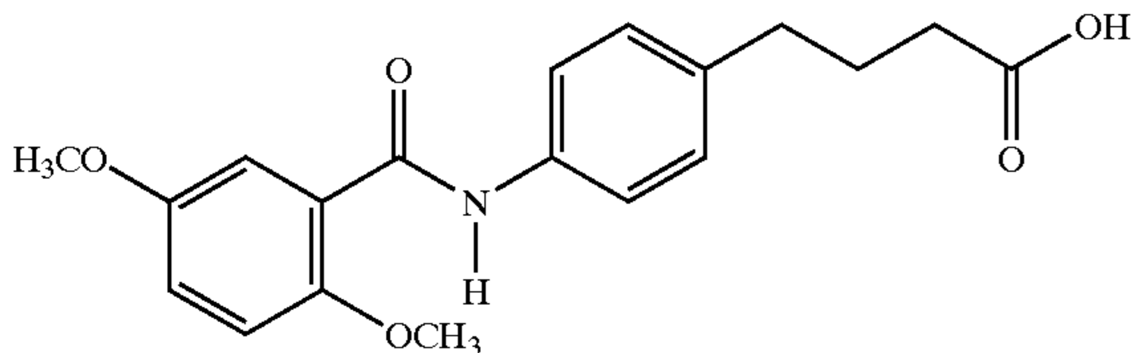
4-(4-(2,5-dimethoxybenzoyl)aminophenyl)butyric acid
