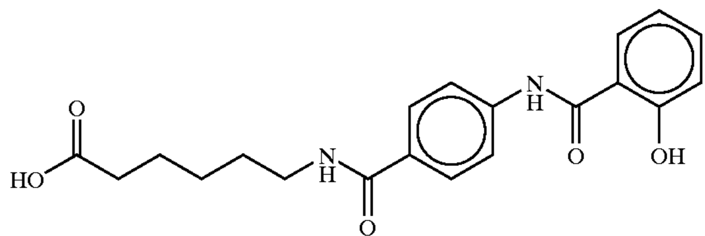
N-(4-salicyloylamino)-6-caproic acid
