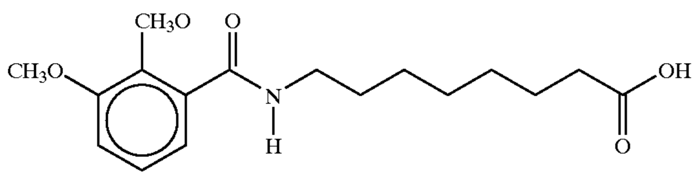
8-(N-2,3-Dimethoxybenzoyl) aminocaprylic acid
