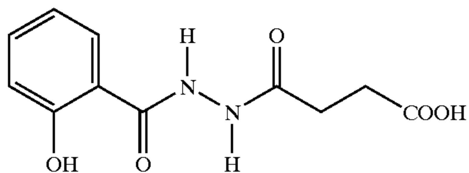
1-salicyloyl-2-succinyl hydrazide
