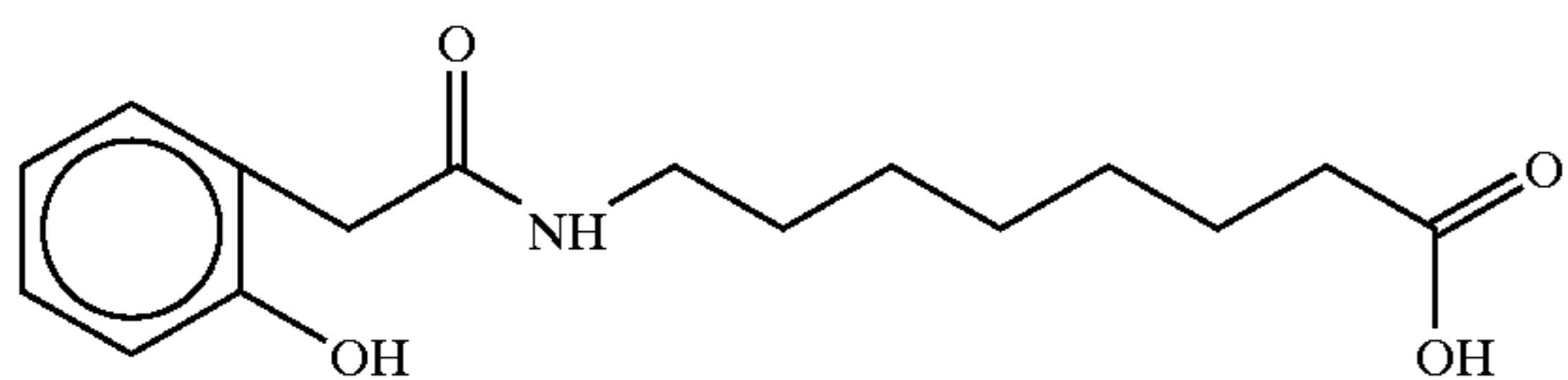
8-(2-hydroxyphenoxy)aminocaprylic acid
