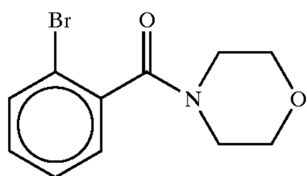
N-(2-bromobenzoyl)morpholine
