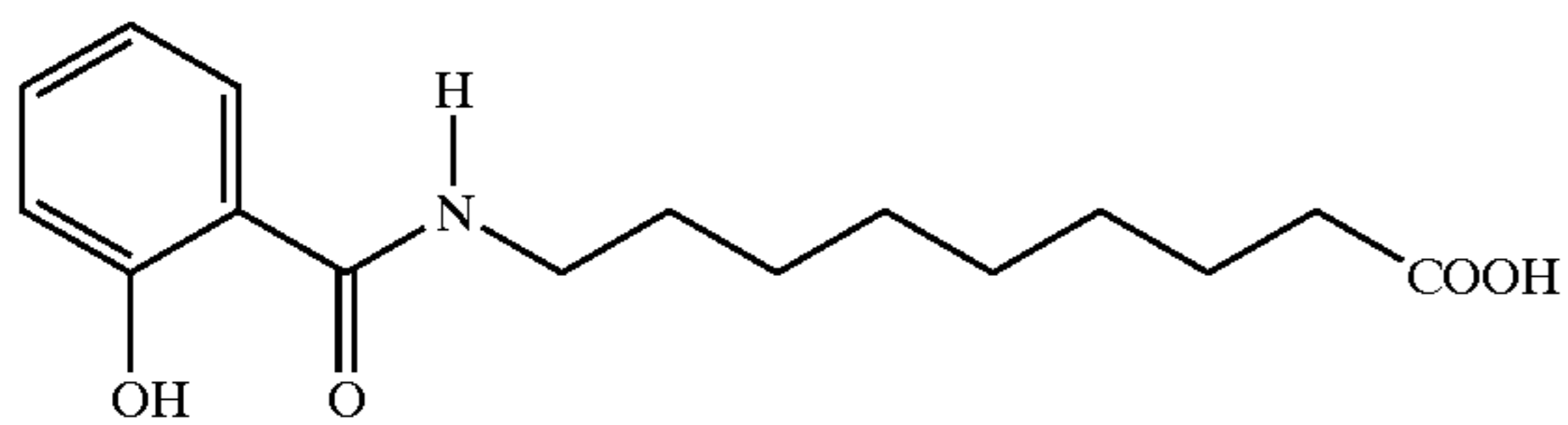
9-Salicyloylaminononanic acid
