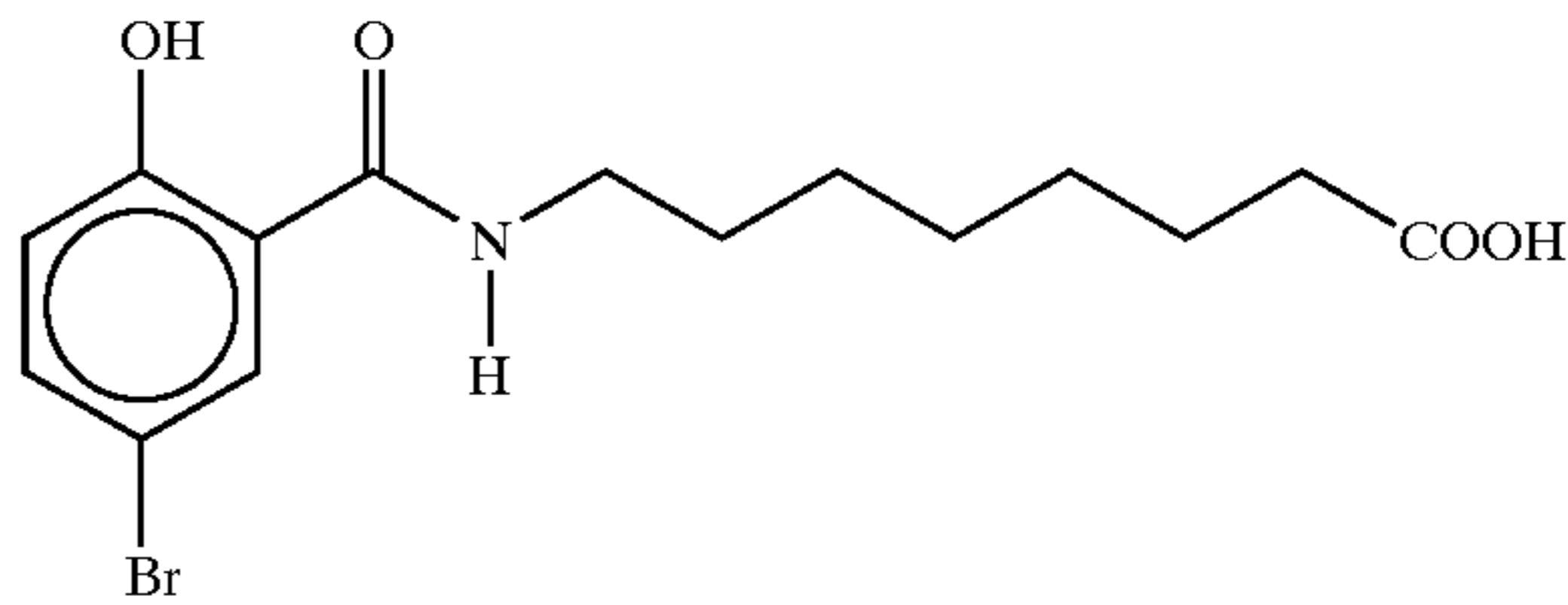
8-(N-2-hydroxy-5-bromobenzoyl)aminocaprylic acid
