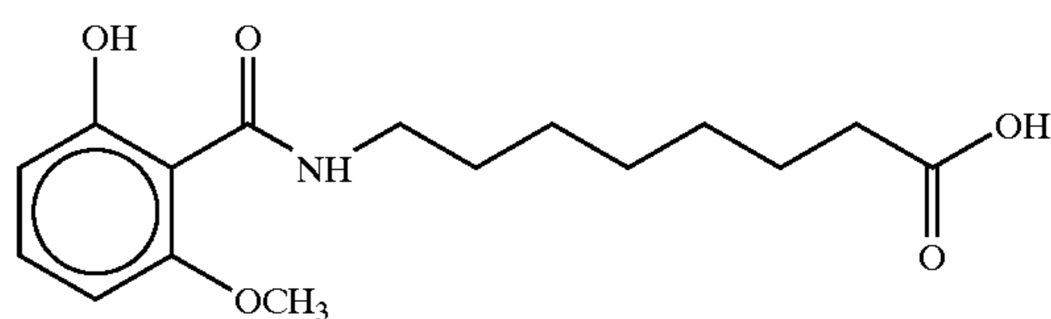
8-(N-2-Hydroxy6-methoxybenzoyl)aminocaproic acid
