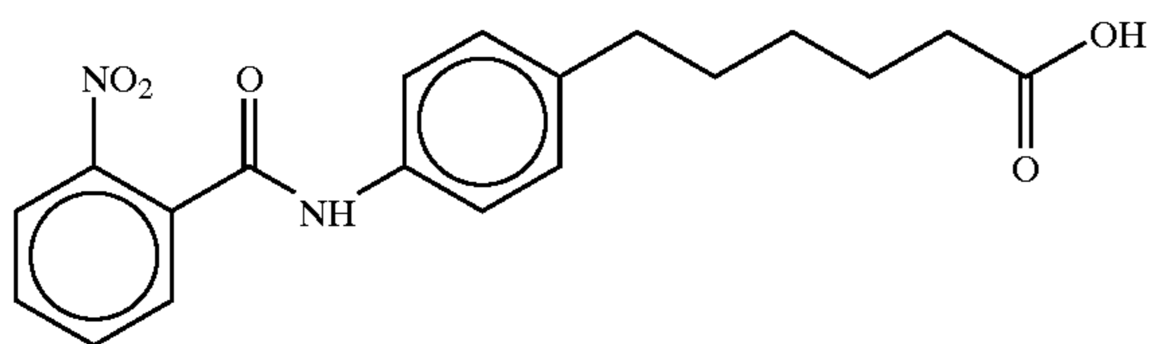
6-(4-(N-2-Nitrobenzoyl)aminophenyl)hexanoic acid
