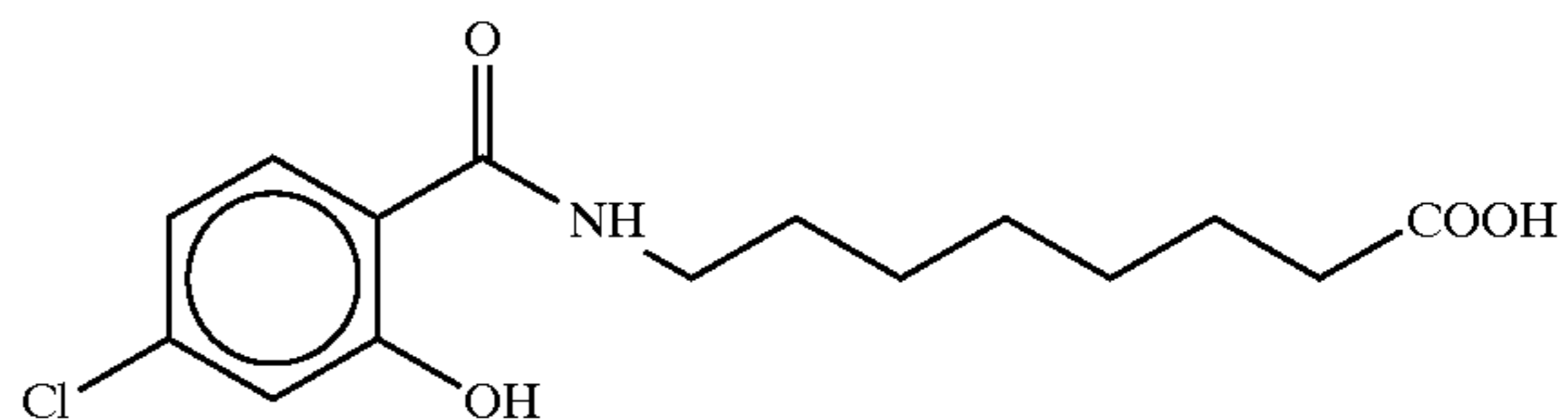
8-(2-hydroxy-4-chlorobenzoyl)aminocaproic acid
