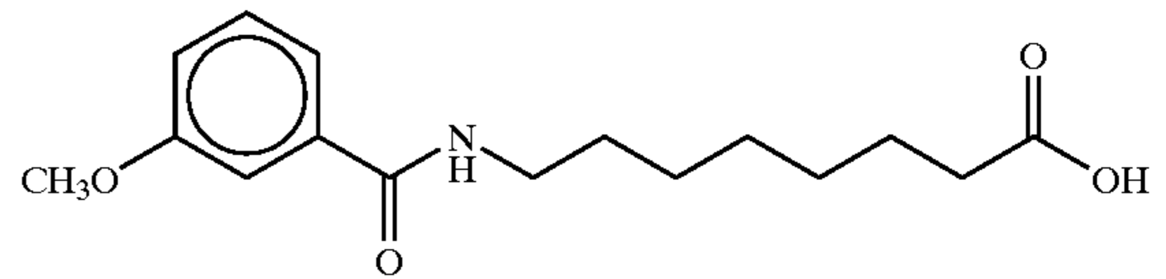
8-(3-anisoyl)aminocaprylic acid
