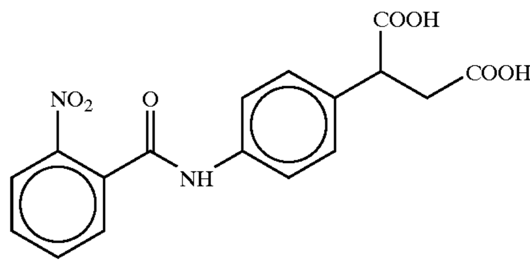
4-(2-Nitrobenzoyl)aminophenylsuccinic acid
