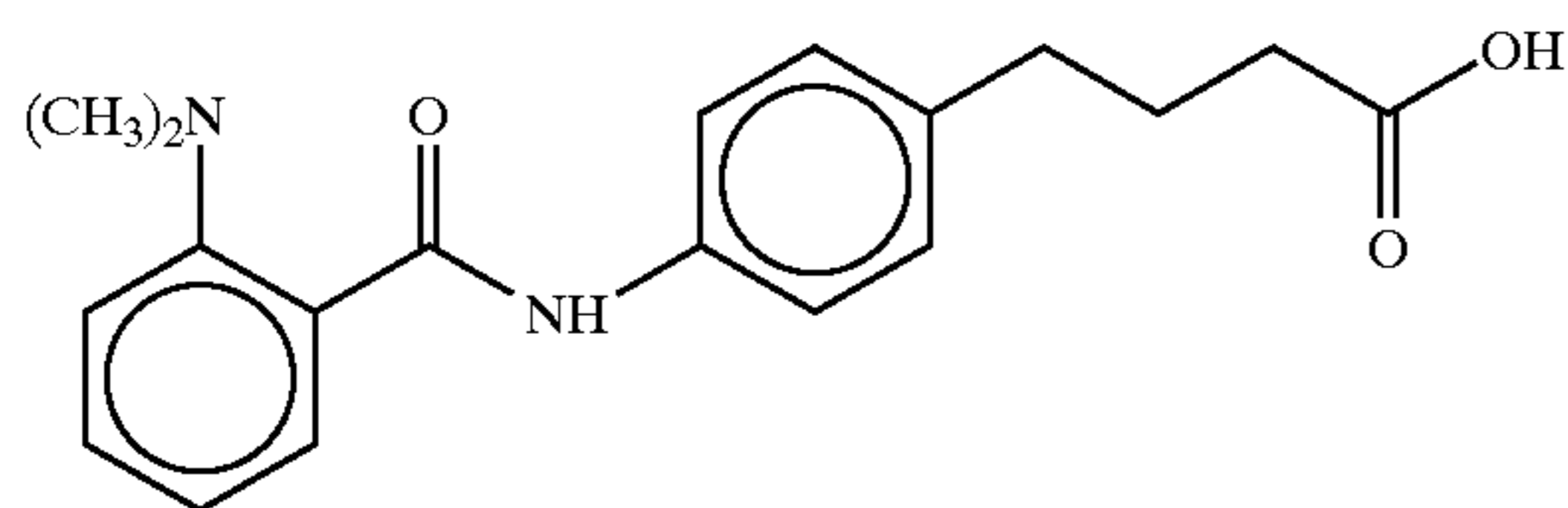
4-(4-(2-Dimethylamino benzoic)aminophenyl) butyric acid
