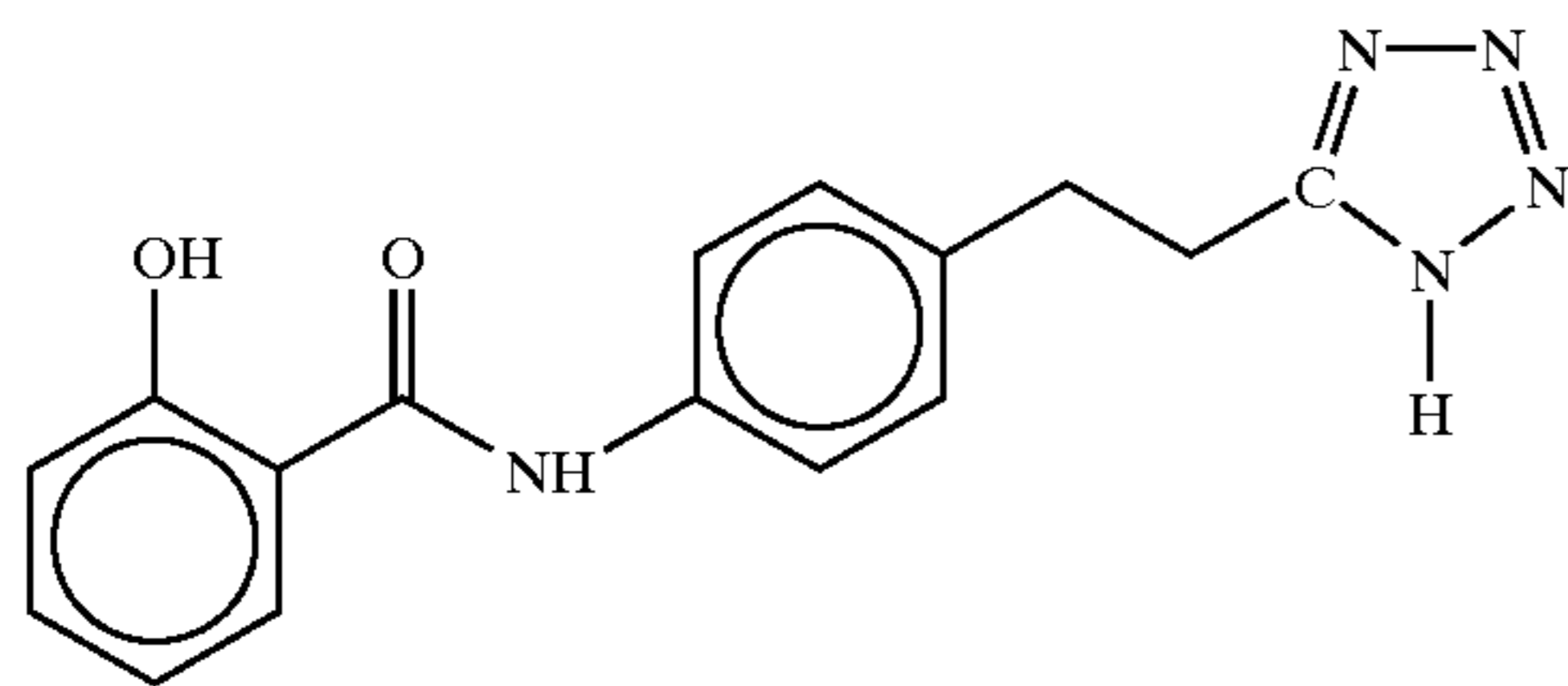
4-(Salicyloyl)amionphenylethyltetrazole
