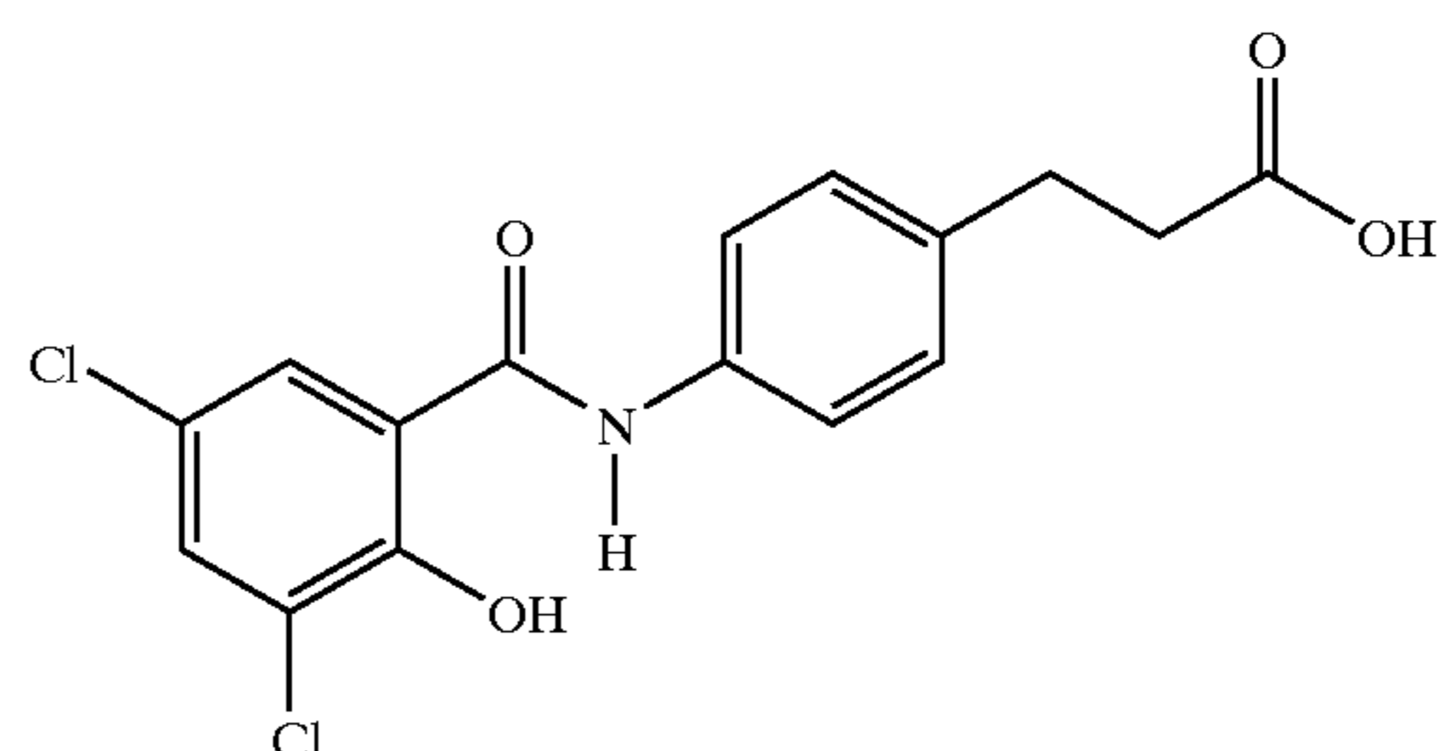
N-[3,5-dichloro-2-hydroxybenzoyl-3-(4-aminophenyl)]propionic acid
