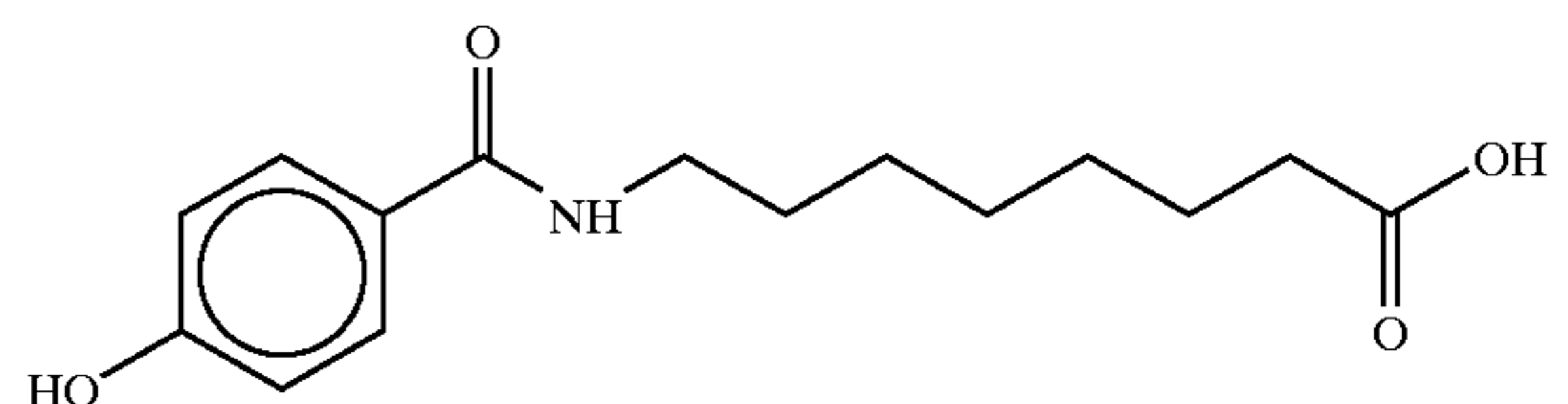
8-(4-Hydroxybenzoyl)aminocaprylic acid
