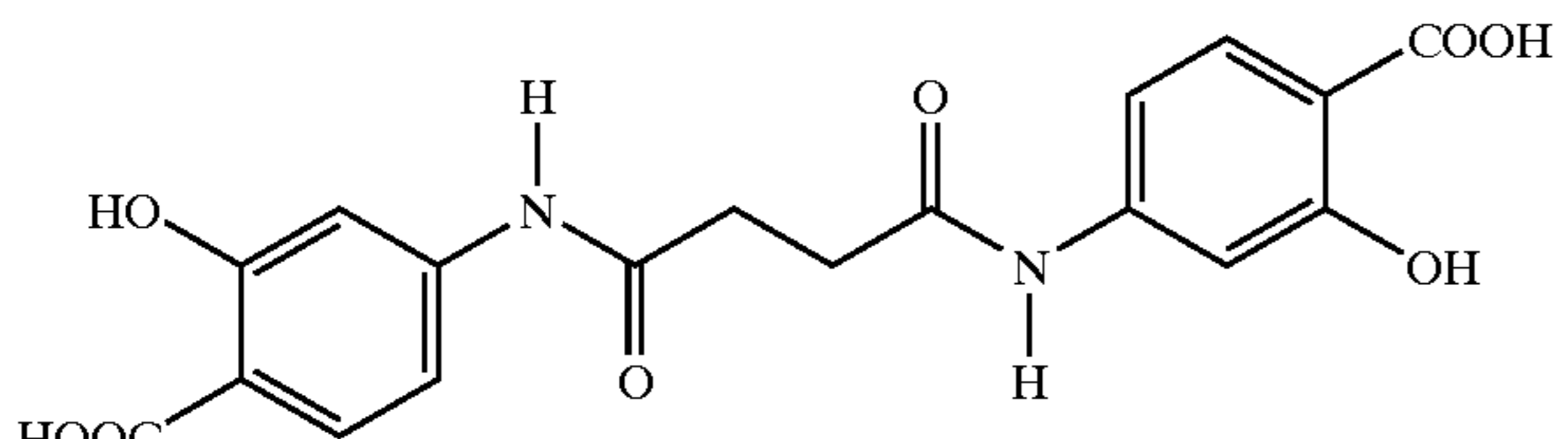
Succinyl-4-aminosalicylic acid
