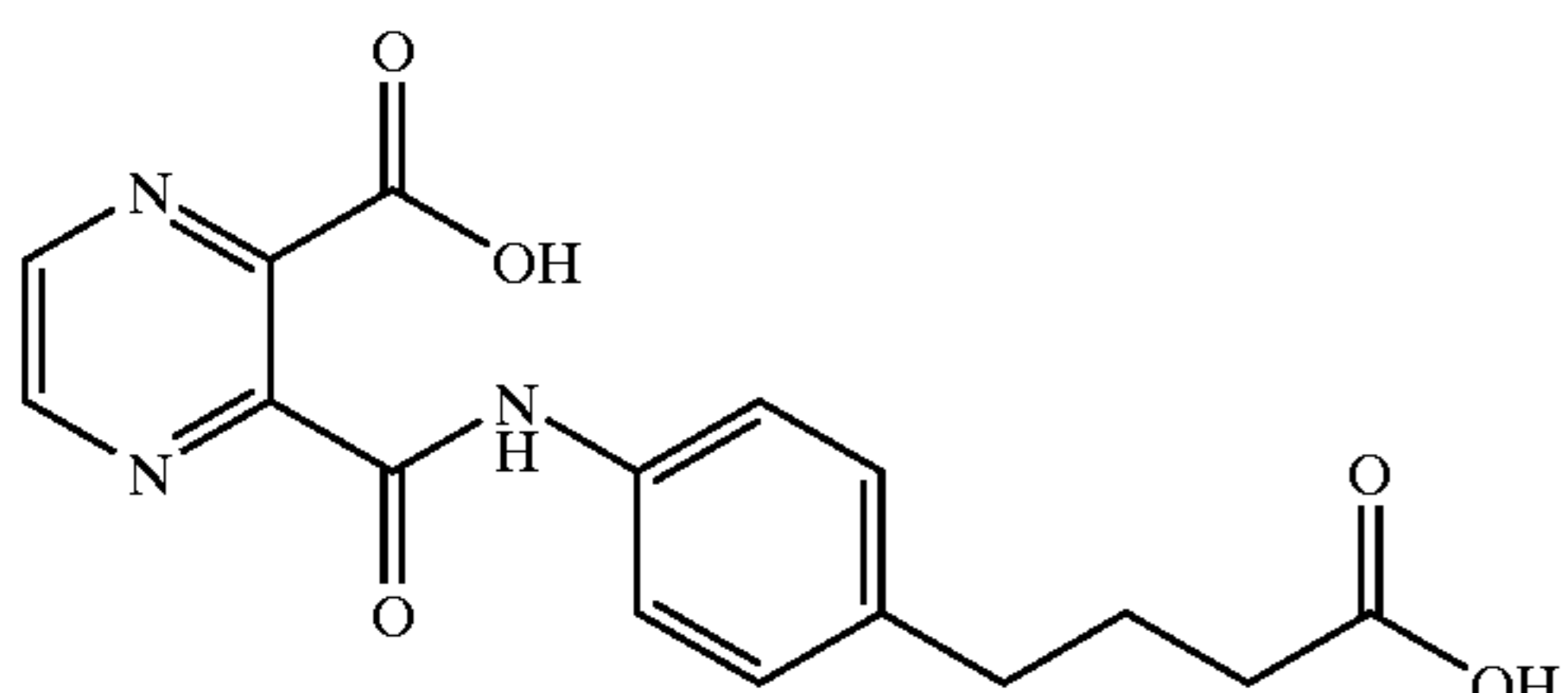
4-(4-(2-(3-carboxyl)pyrazinecarbonyl)aminophenyl)butyric acid
