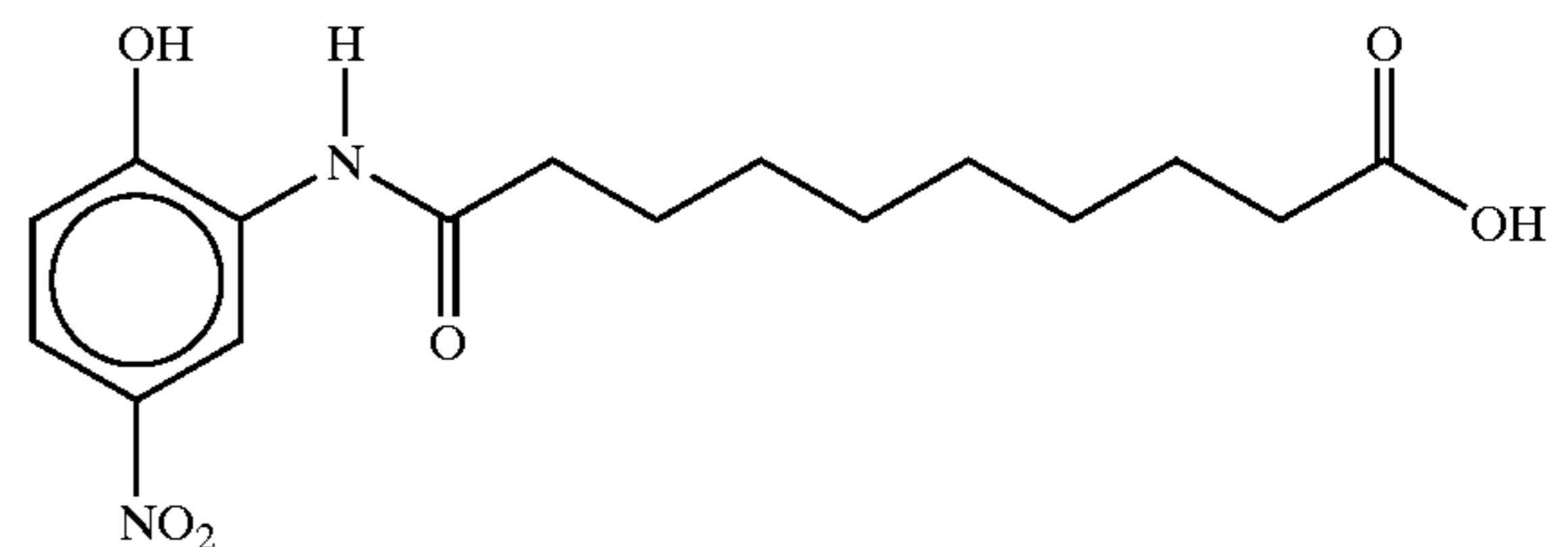
N-10-(2-hydroxy-5-nitroanilino)decanoic acid
