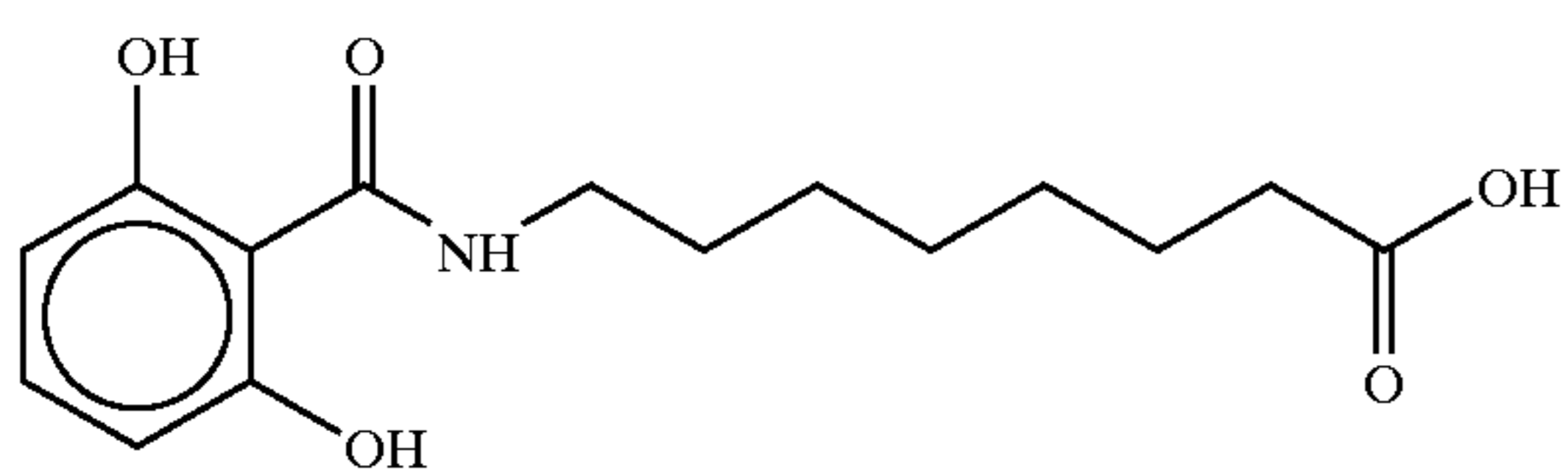
8-(N-2,6-Dihydroxybenzoyl)aminocaproic acid
