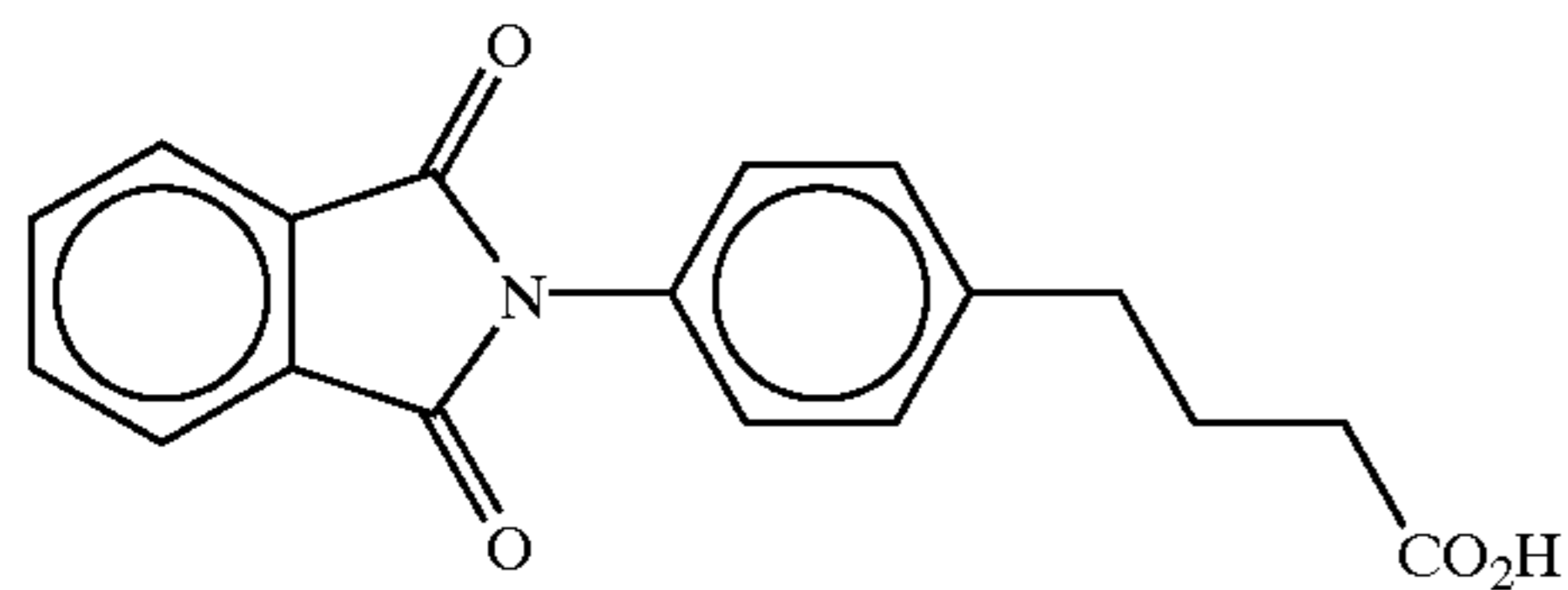
4-(4-phthalimidophenyl)butyric acid
