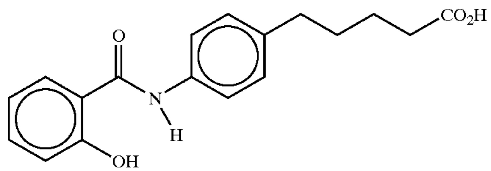
N-salicyloyl-5-(4-aminophenyl)valeric acid
