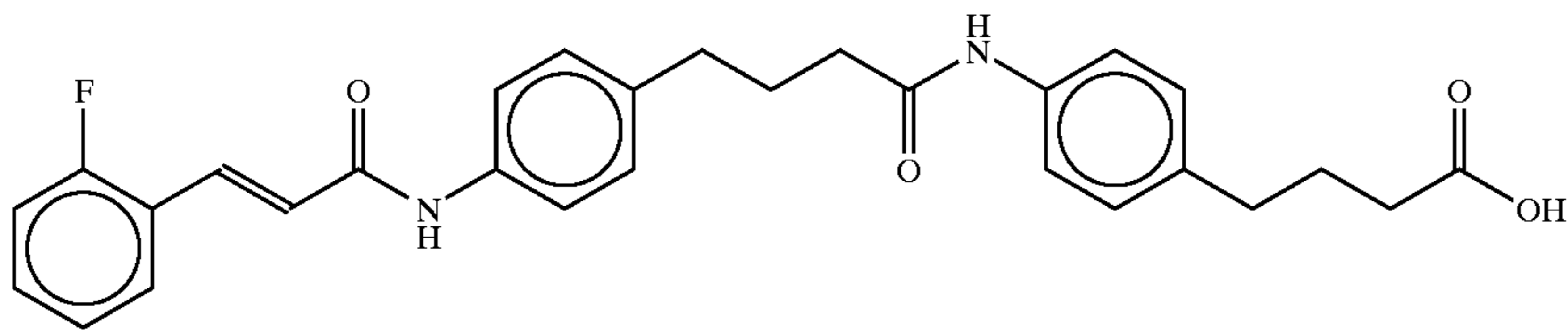
4-(4-(N-(2-Fluorocinnamoyl))aminophenyl) butyric
