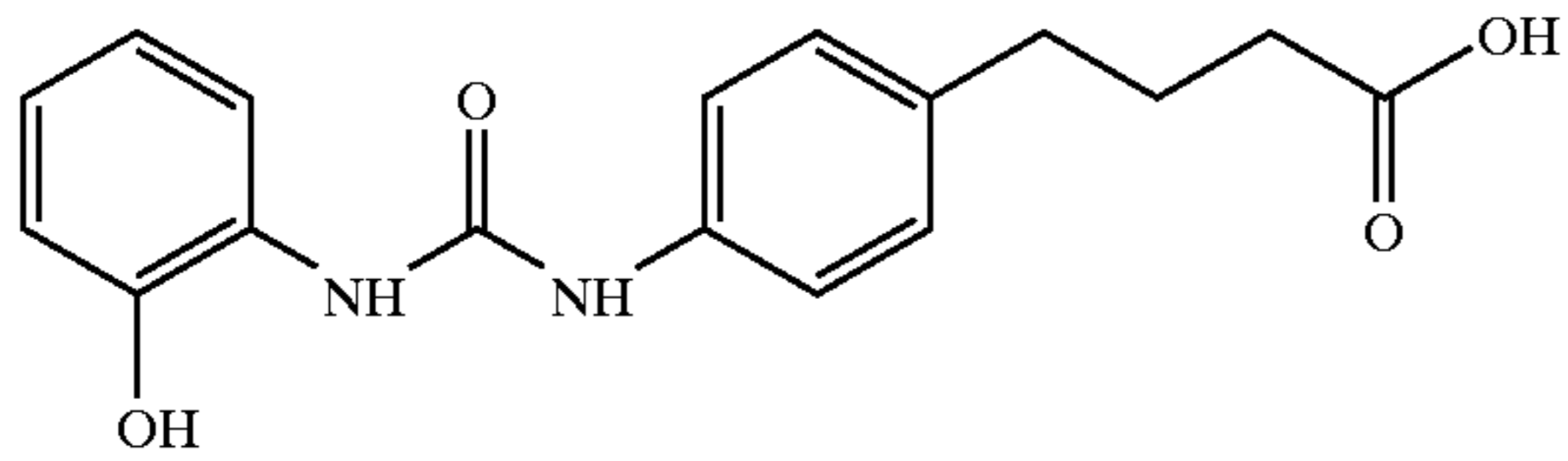
3-Indolebutyric acid
