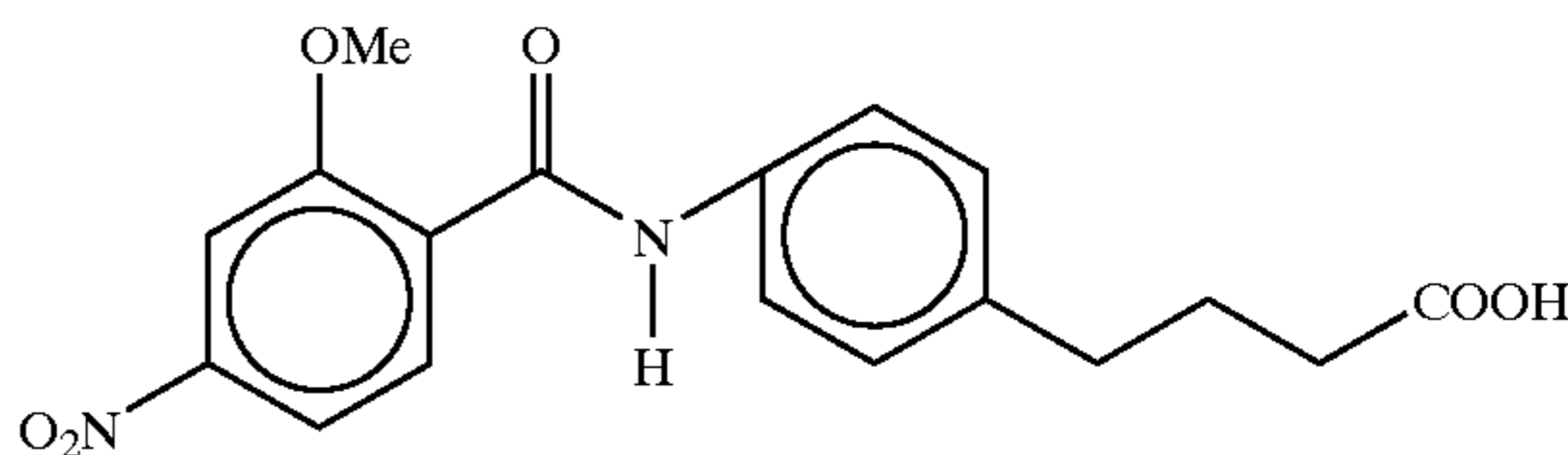
4-{N-[4-(2-methoxy-4-nitrobenzoyl)aminophenyl]}butyric acid
