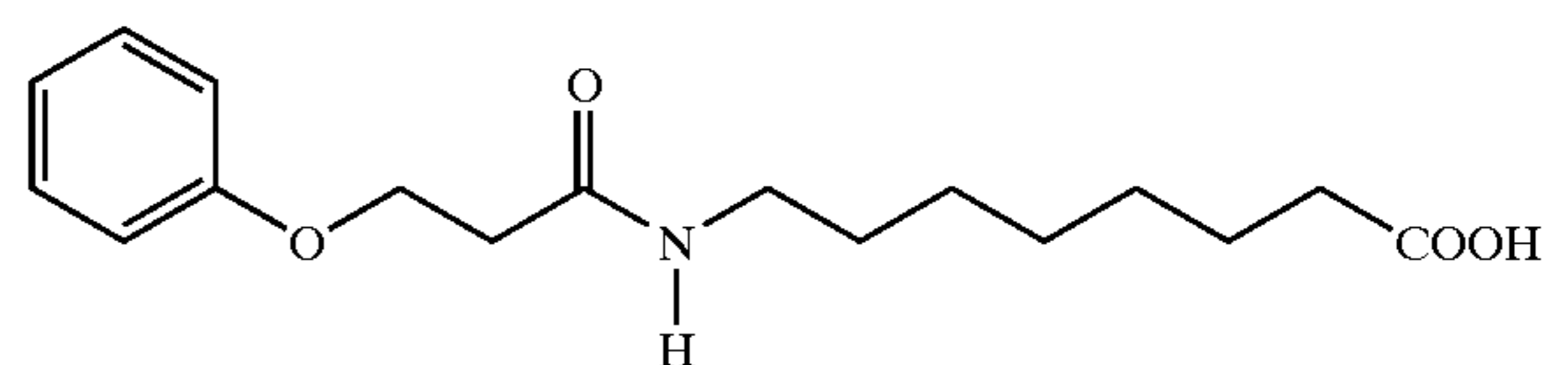
8-(3-Phenoxypropionylamino)caprylic acid
