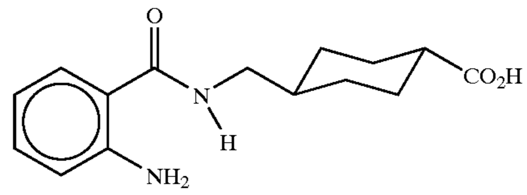
trans-4-(2-aminobenzamidomethyl)cyclohexanecarboxylic acid
