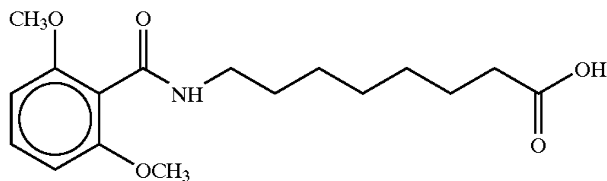
8-(N-2-6-Dimethoxybenzoyl)aminocaproic acid
