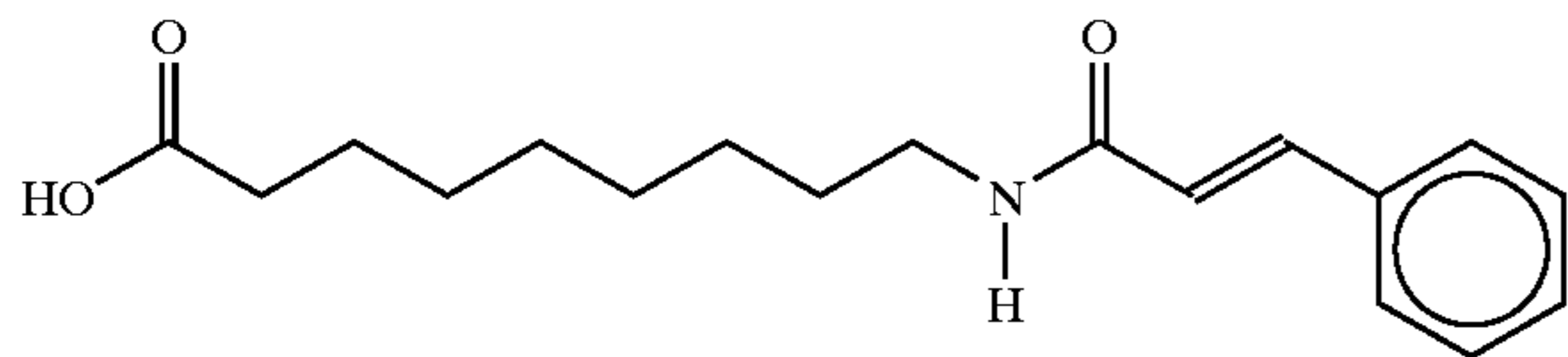
9-(cinnamoylamino)nonanoic acid
