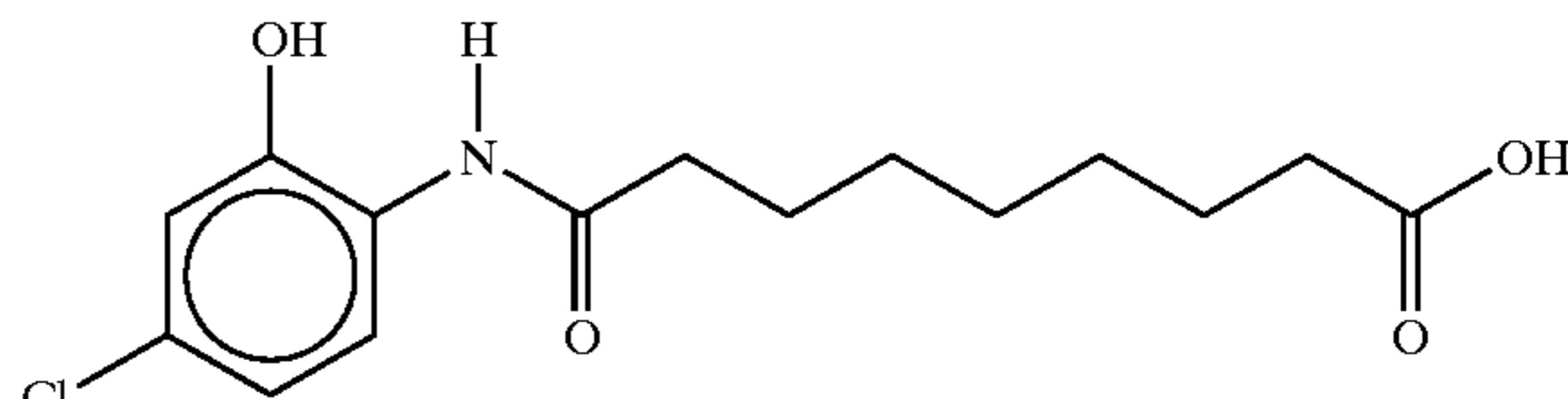
8-(2-hydroxy-5-chloroanilino)octanoic acid
