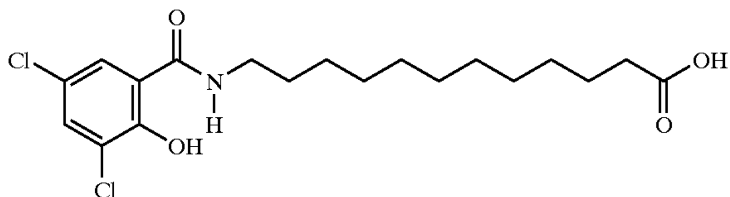
12-N-(3,5-dichloro-2-hydroxybenzoyl)aminododecanoic acid
