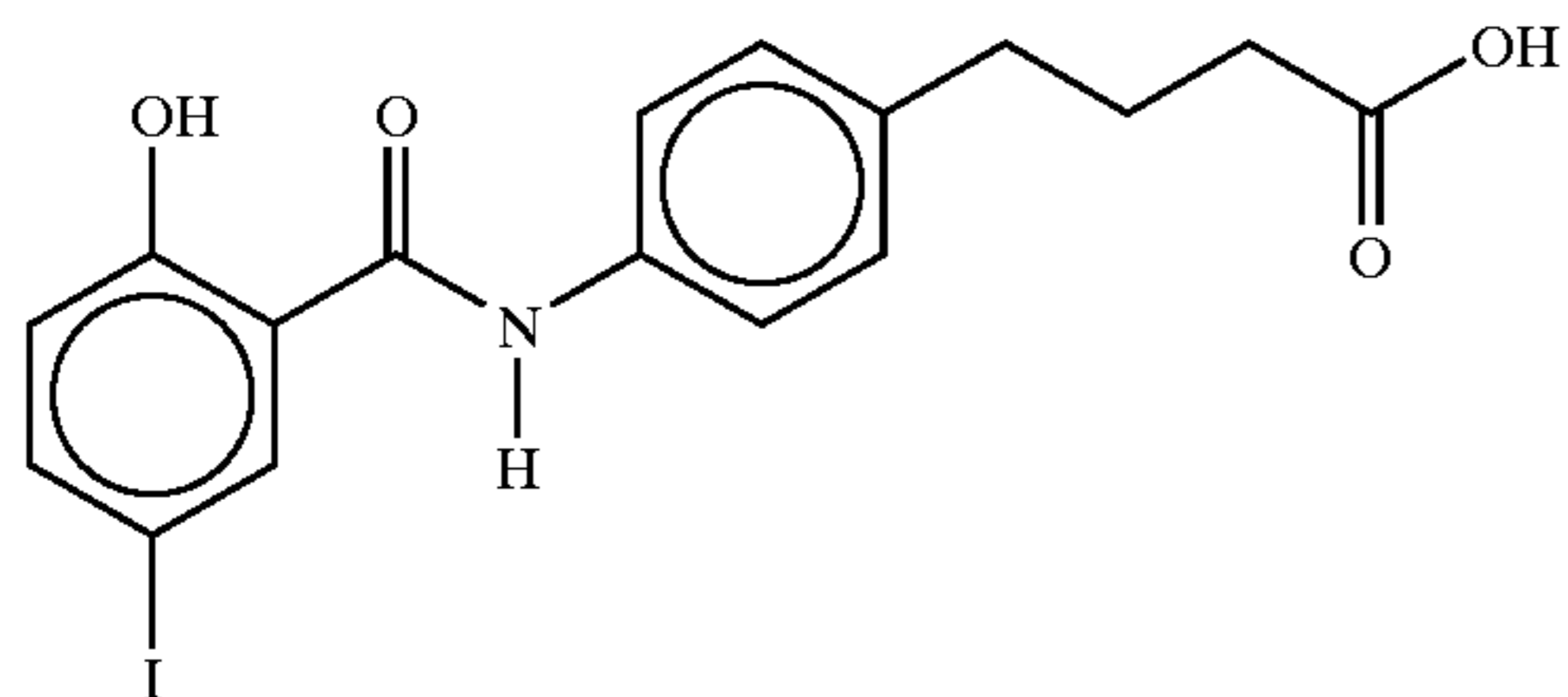
4-[N-(2-hydroxy-5-iodobenzoyl)aminophenyl]butyric acid
