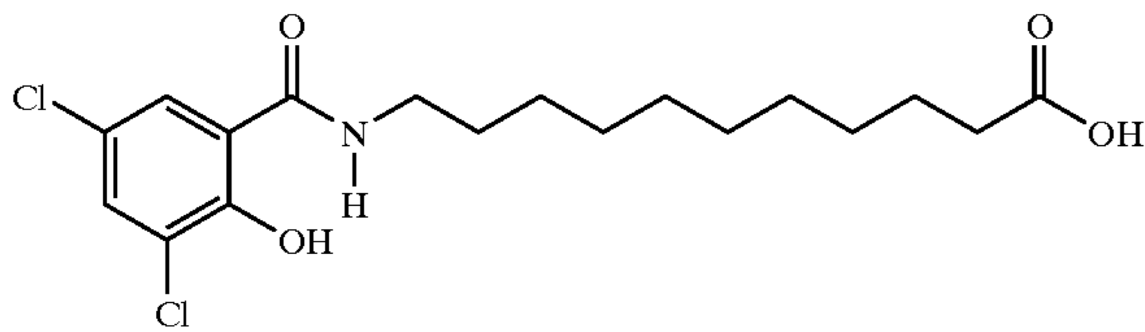
11-N-(3,5-dichloro-2-hydroxybenzoyl)aminoundecanoic acid
