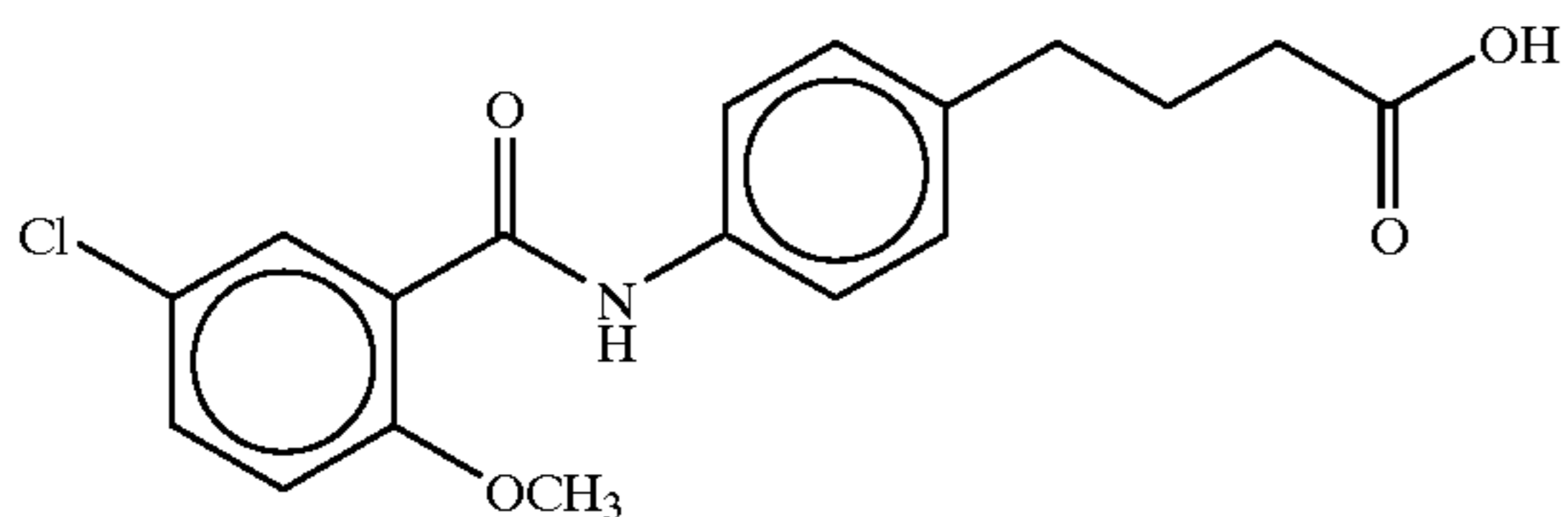
4-(4-(5-chloro-o-anisoyl)aminophenyl)butyric acid
