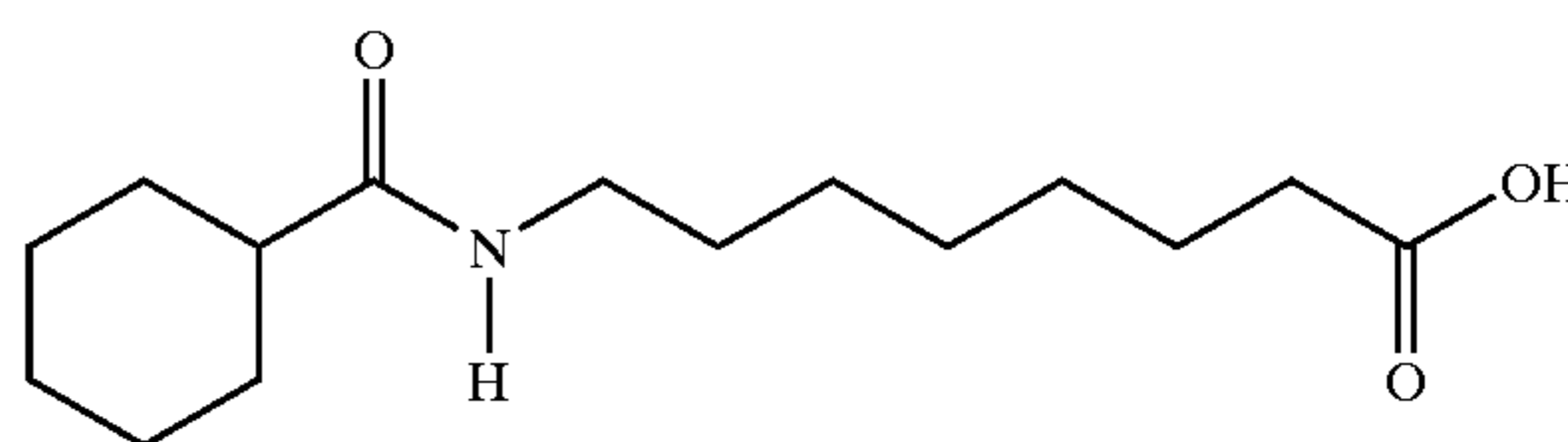
8-N-cyclohexanoylaminocaprylic acid
