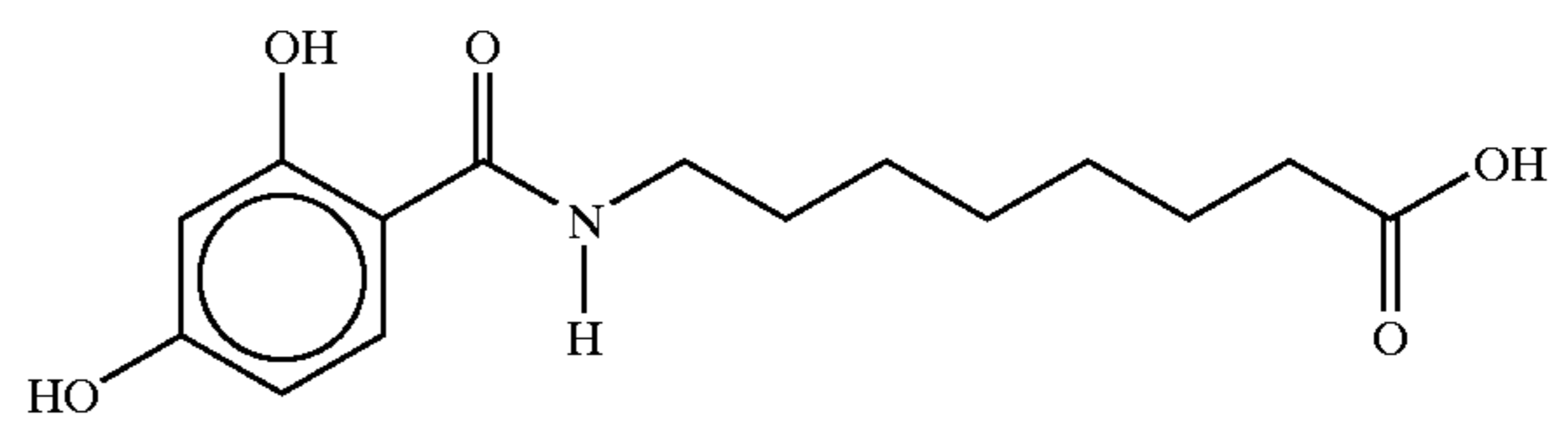
8-(N-2,4-Dihydroxybenzoyl) aminocaprylic acid
