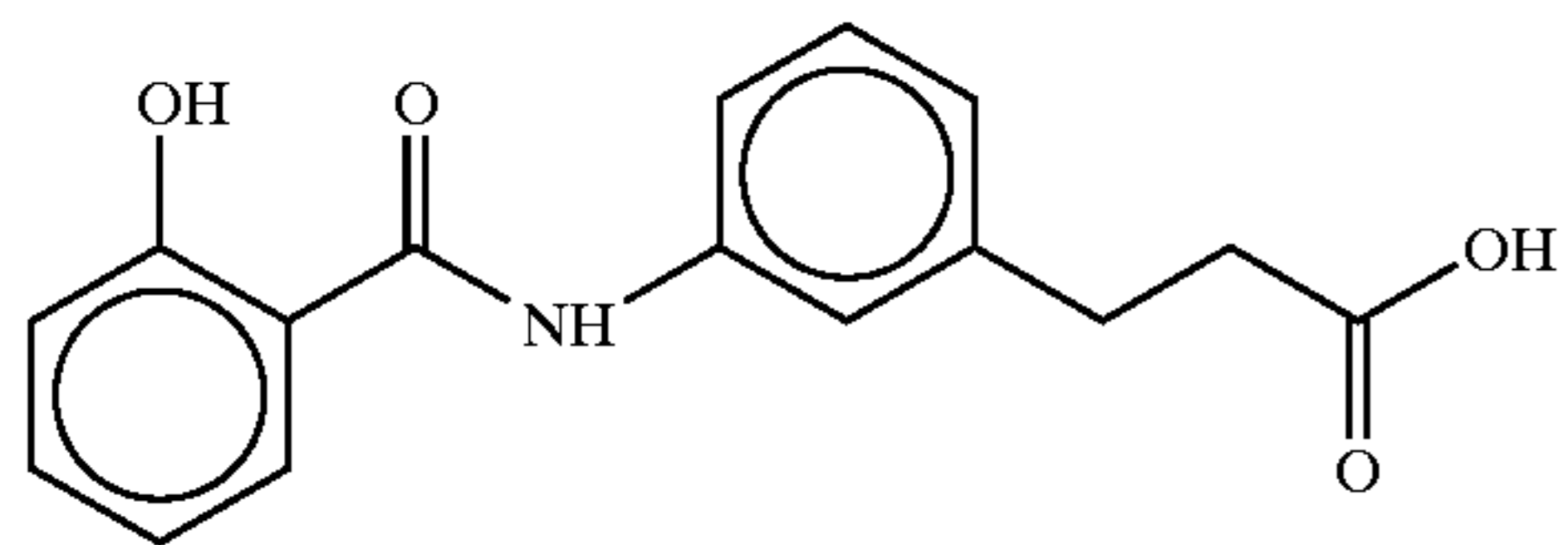
3-(3-(salicyloyl)aminophenyl) propionic acid
