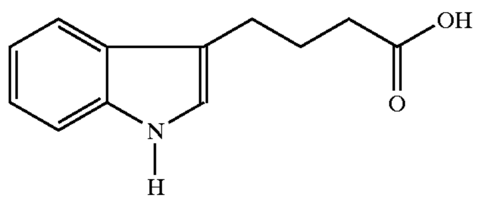
3-Indolebutyric acid
