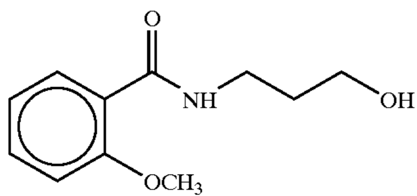
3-(2-methoxybenzoylamino)- 1-propanol
