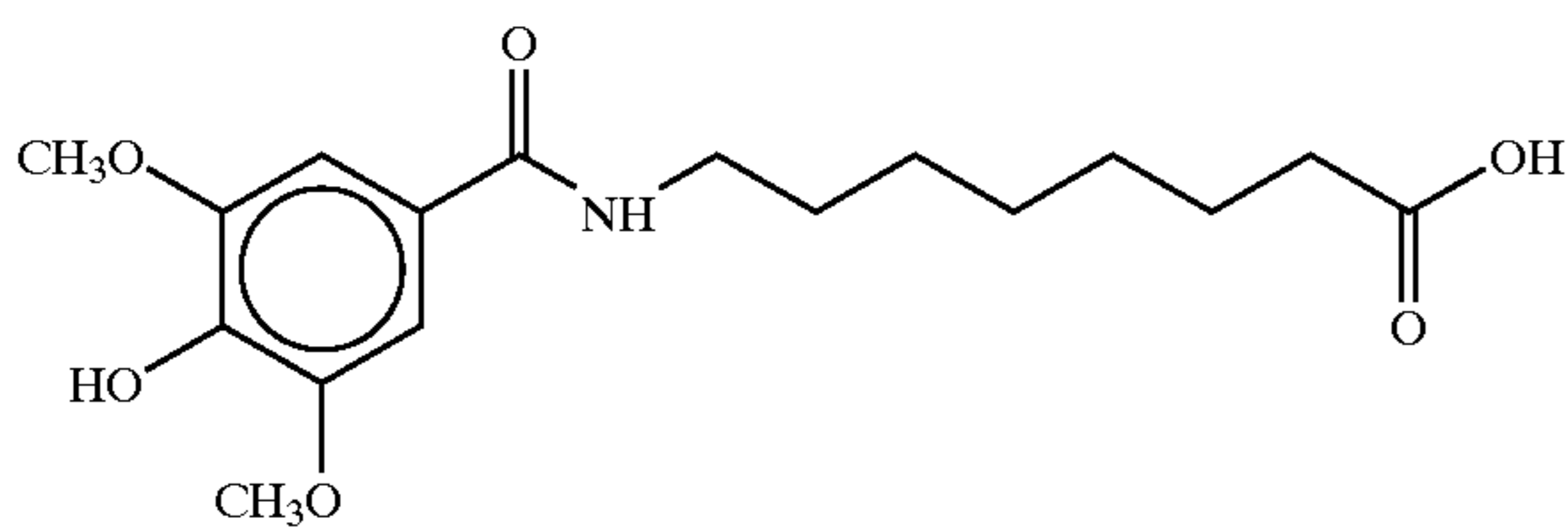
8-(N-3,5-Dimethoxy 4-hydroxybenzoyl)aminocaproic acid
