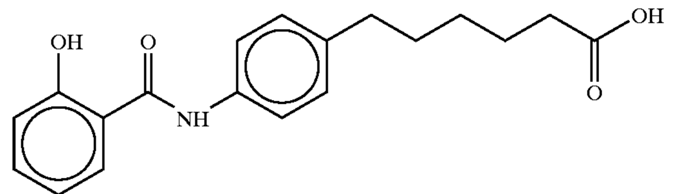
6-(4-(salicyloyl)aminophenyl) hexanoic acid
