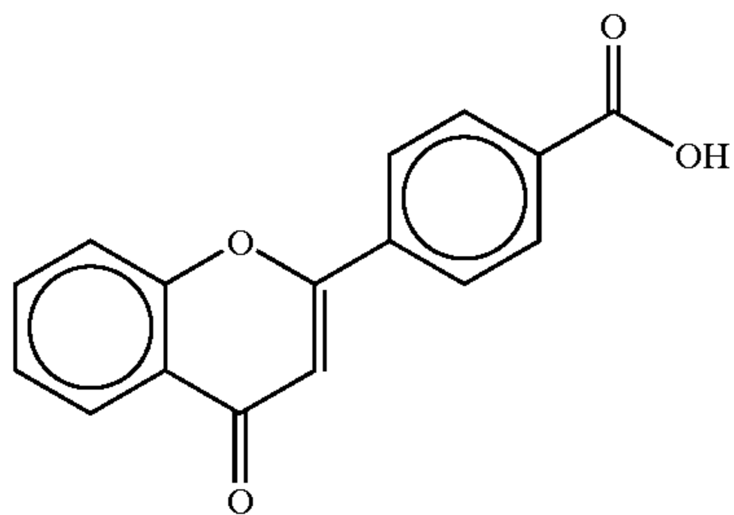
4'-flavonic acid
