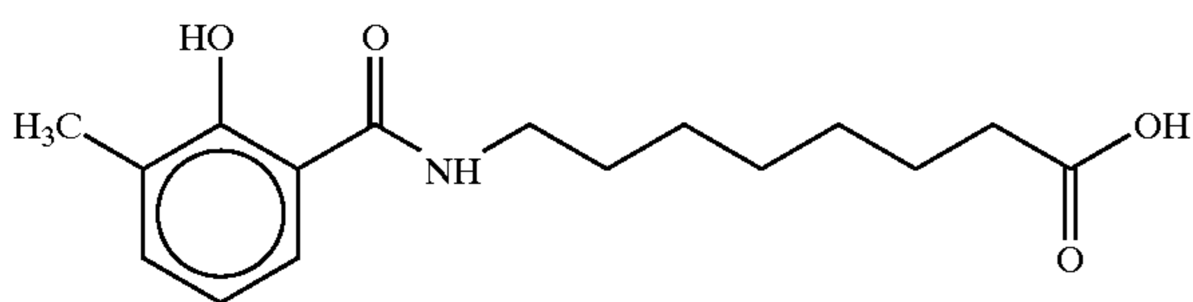
8-(N-(3-methylsalicyloyl)aminocaprylic acid
