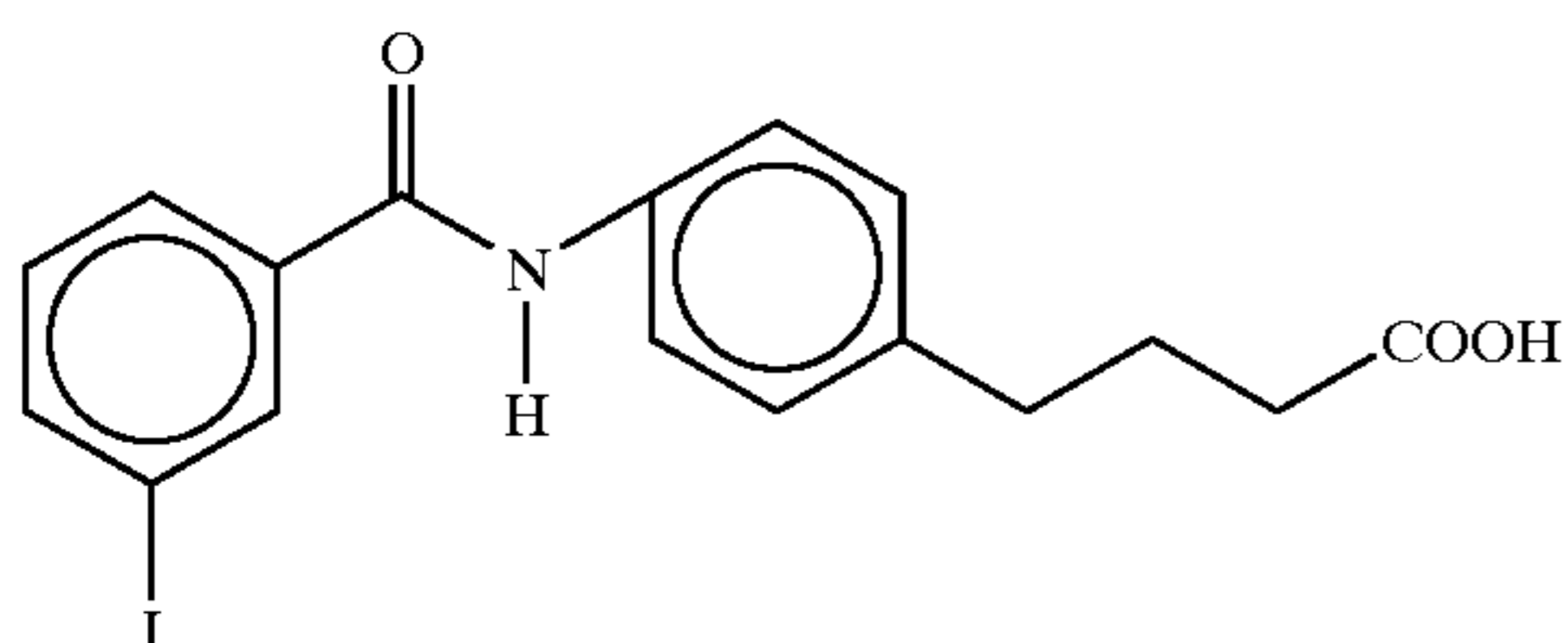
4-{N-[4-(3-iodobenzoyl)aminophenyl]}butyric acid
