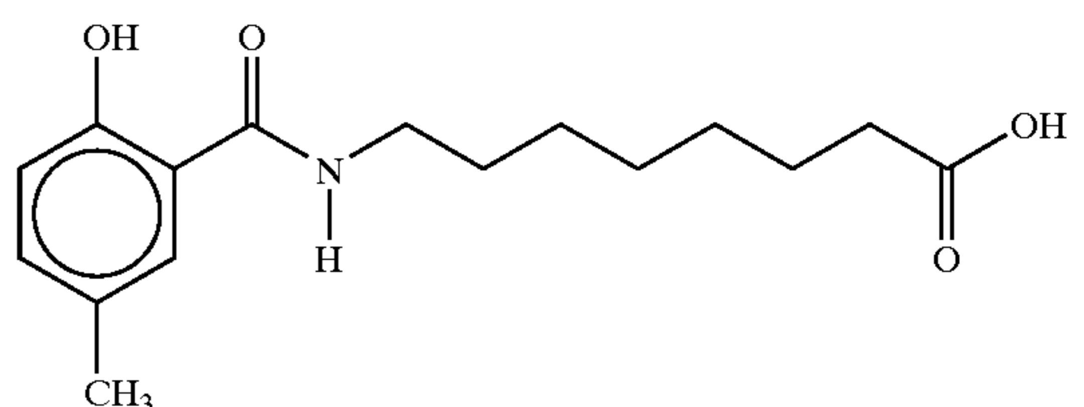
8-(N-(5-methylsalicyloyl)aminocaprylic acid
