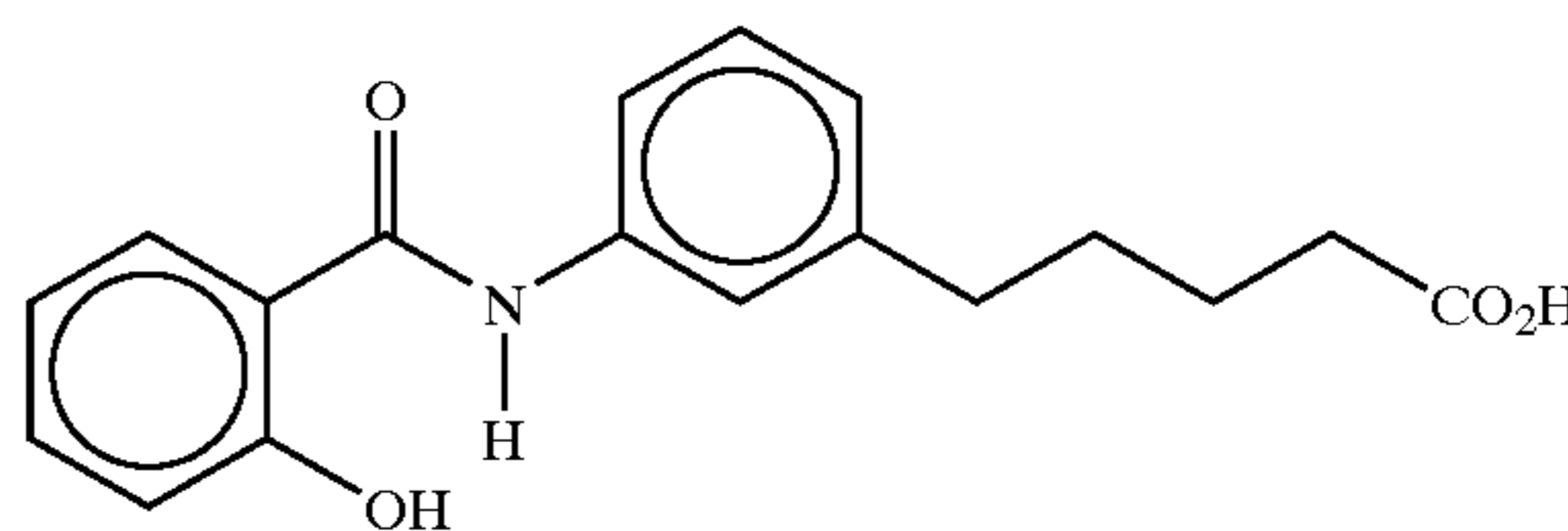
N-Salicyloyl-5-(3-aminophenyl)valeric acid
