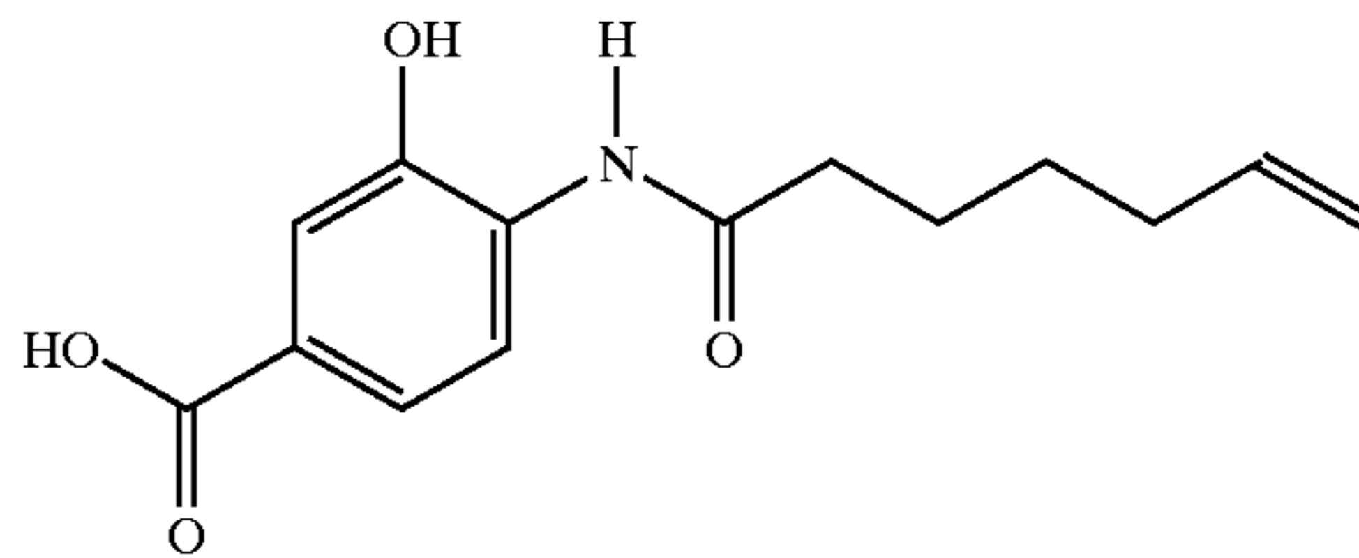
N-(2-hydroxy-4-carboxy)-6-heptenamide
