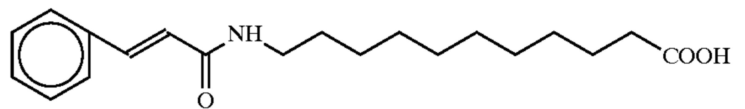
11-cinnamoylaminoundecanoic acid
