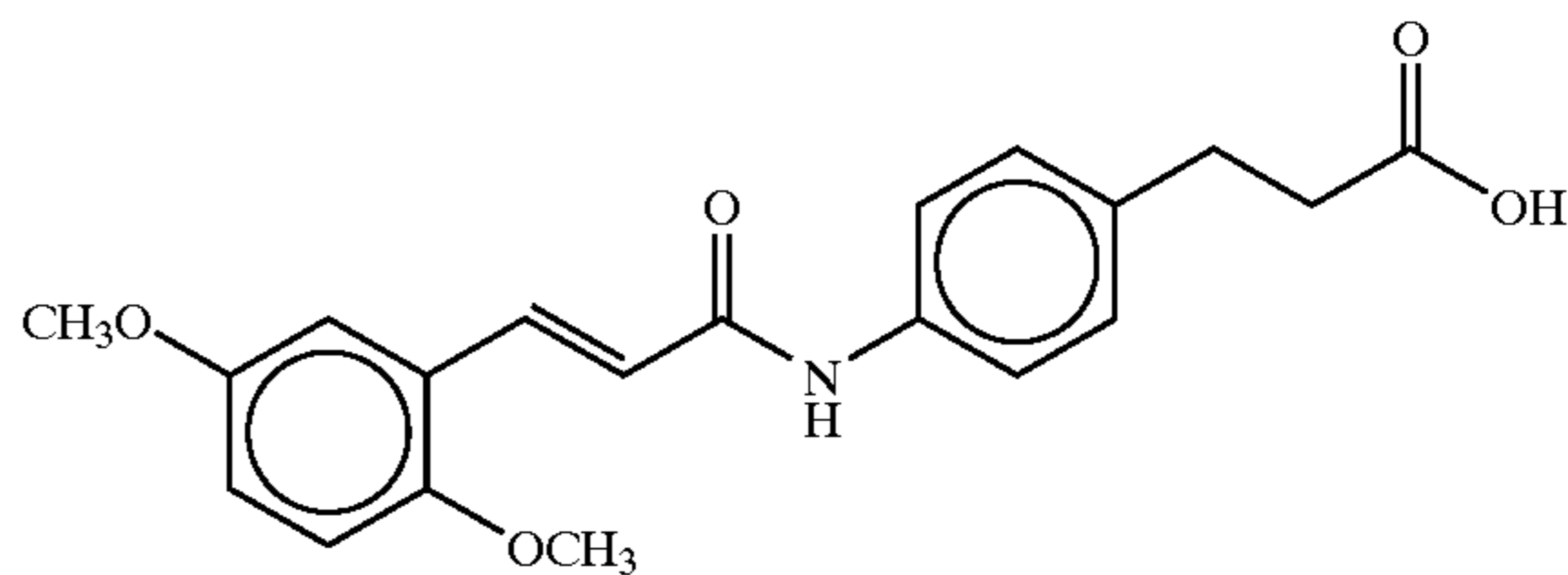
3-(4-(2,5-dimethoxycinnamoyl)aminophenyl)propionic acid
