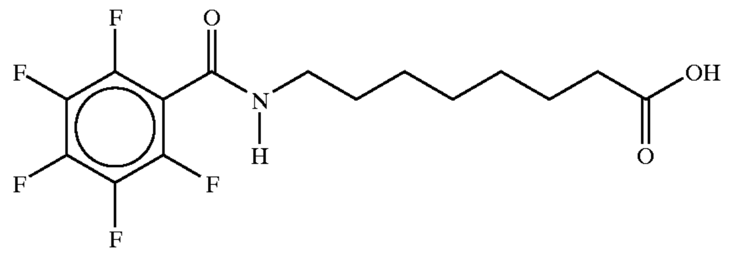
8-(pentafluorobenzoyl)aminocaprylic acid
