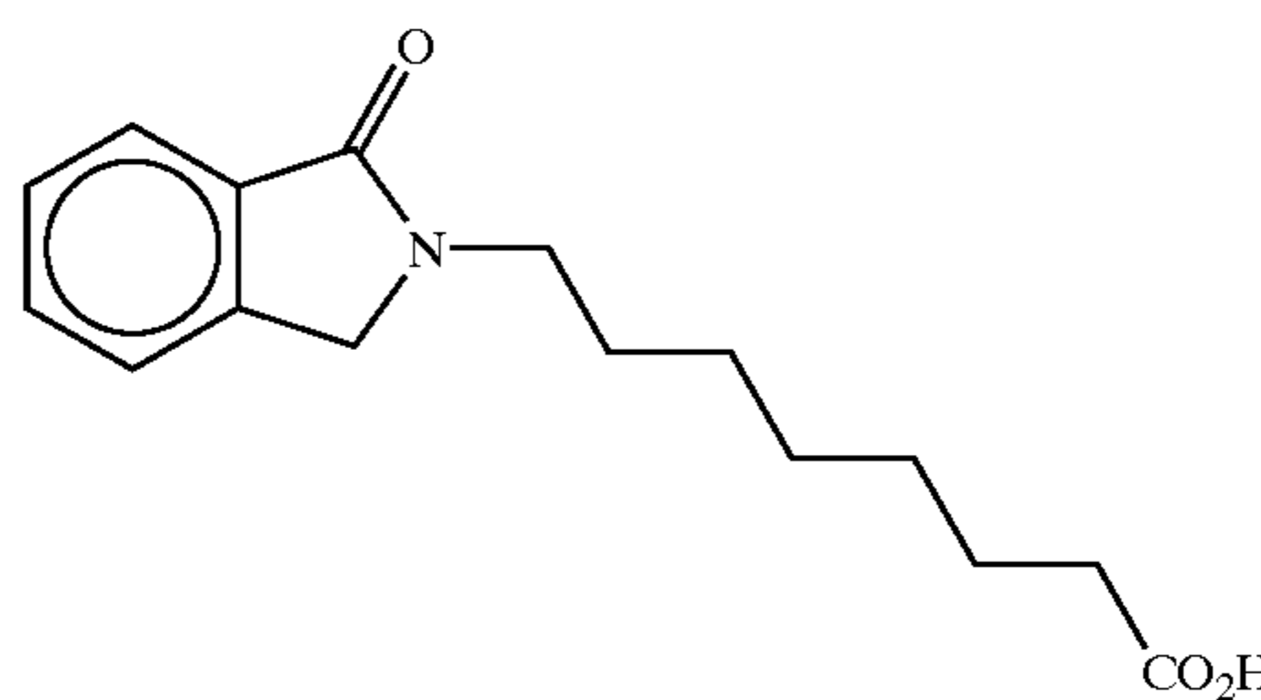
8-(2-(1,2-dihydroisindole-1-one))octanoic acid
