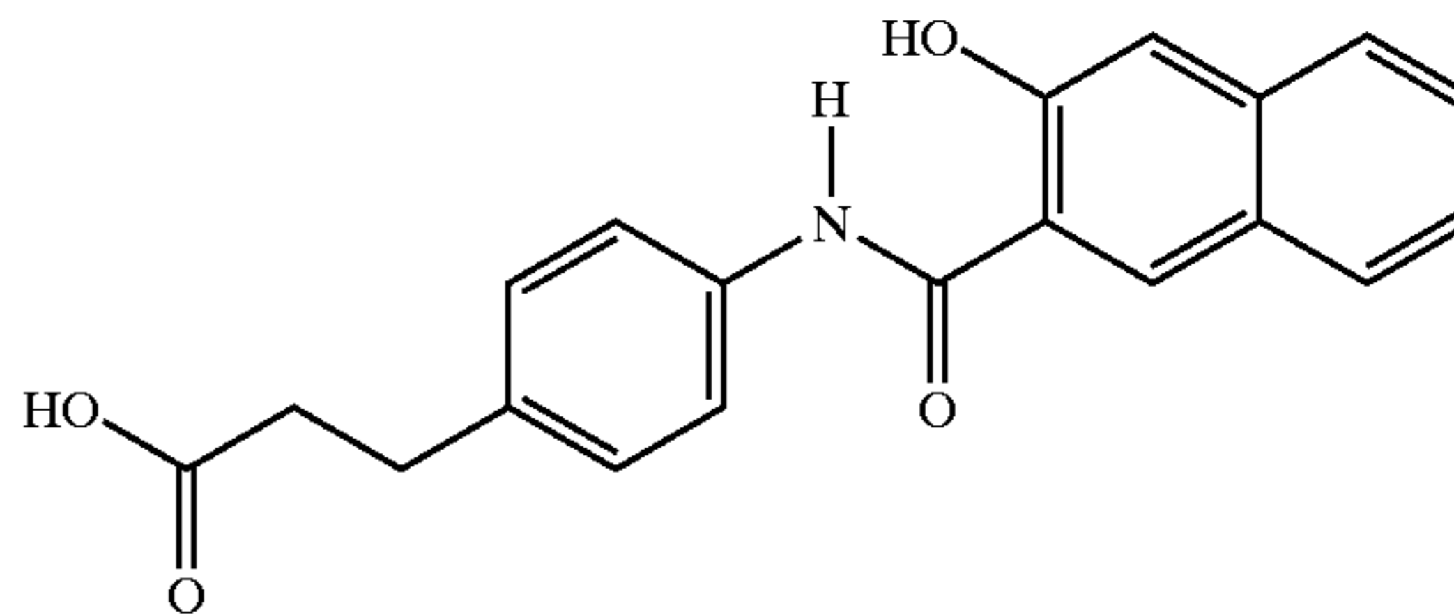
4-{4-[N-(3-hydroxy-2-naphthoyl)aminophenyl]}propanoic acid
