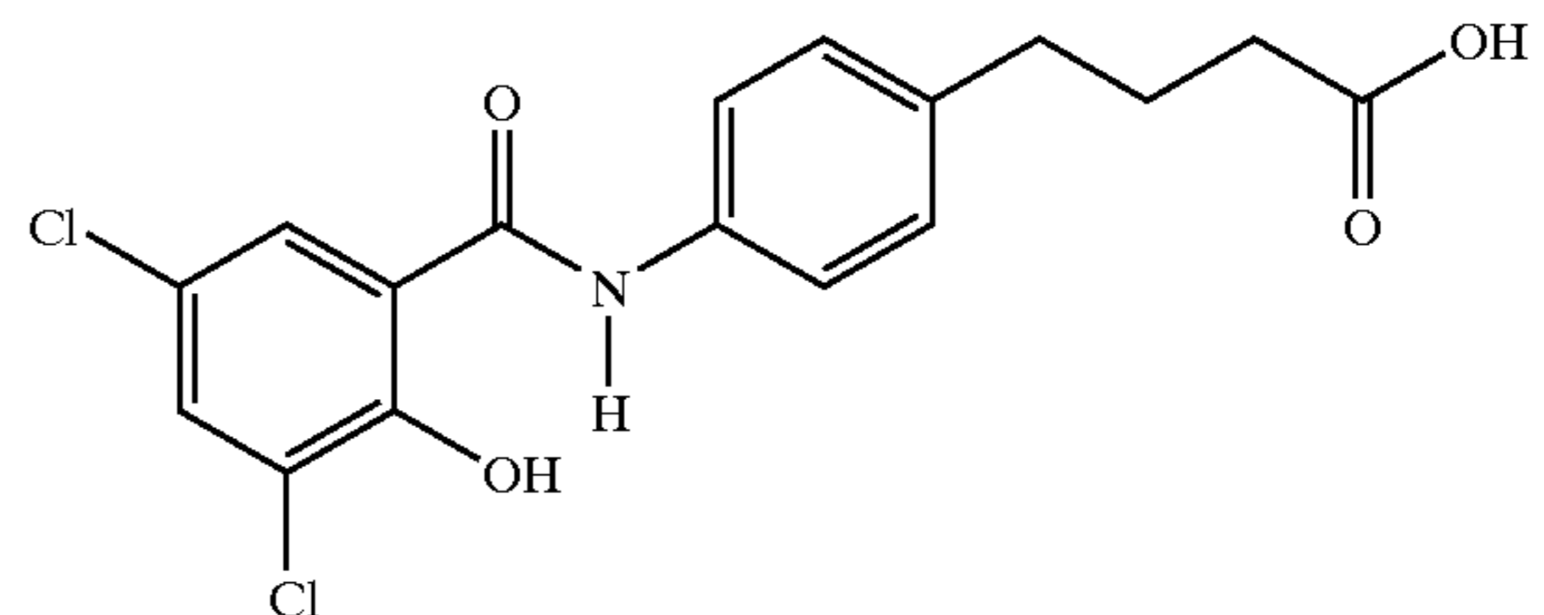
N-[3,5-dichloro-2-hydroxybenzoyl-4(4-aminophenyl)]butyric acid
