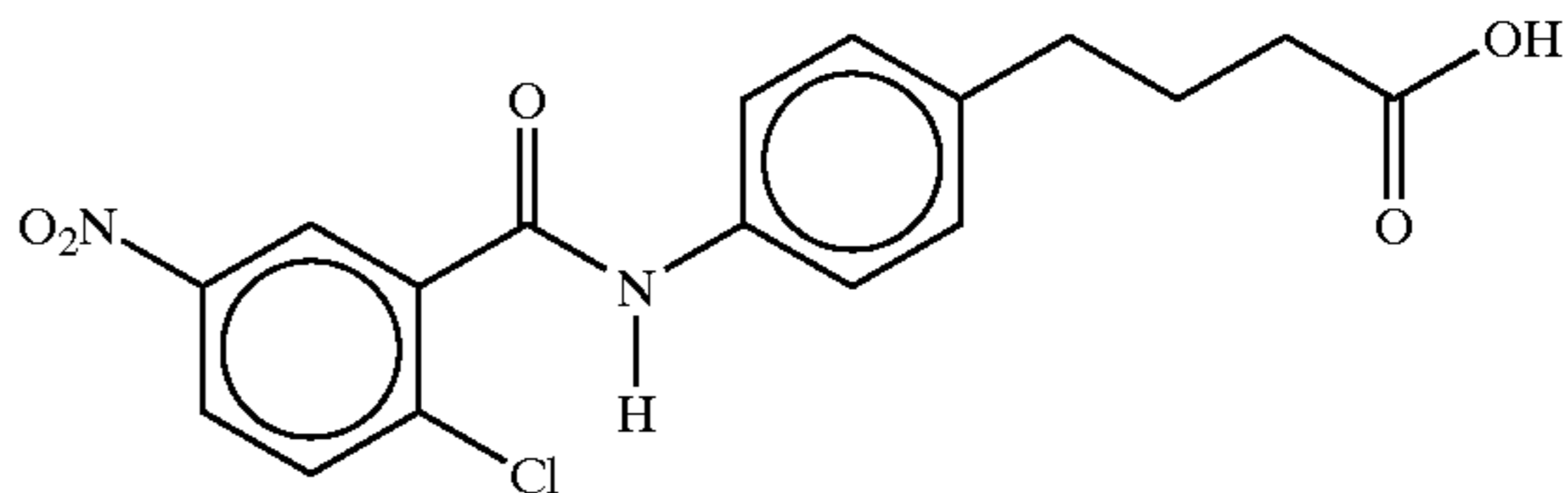
4-[4-(2-chloro-5-nitrobenzoyl)aminophenyl]butyric acid
