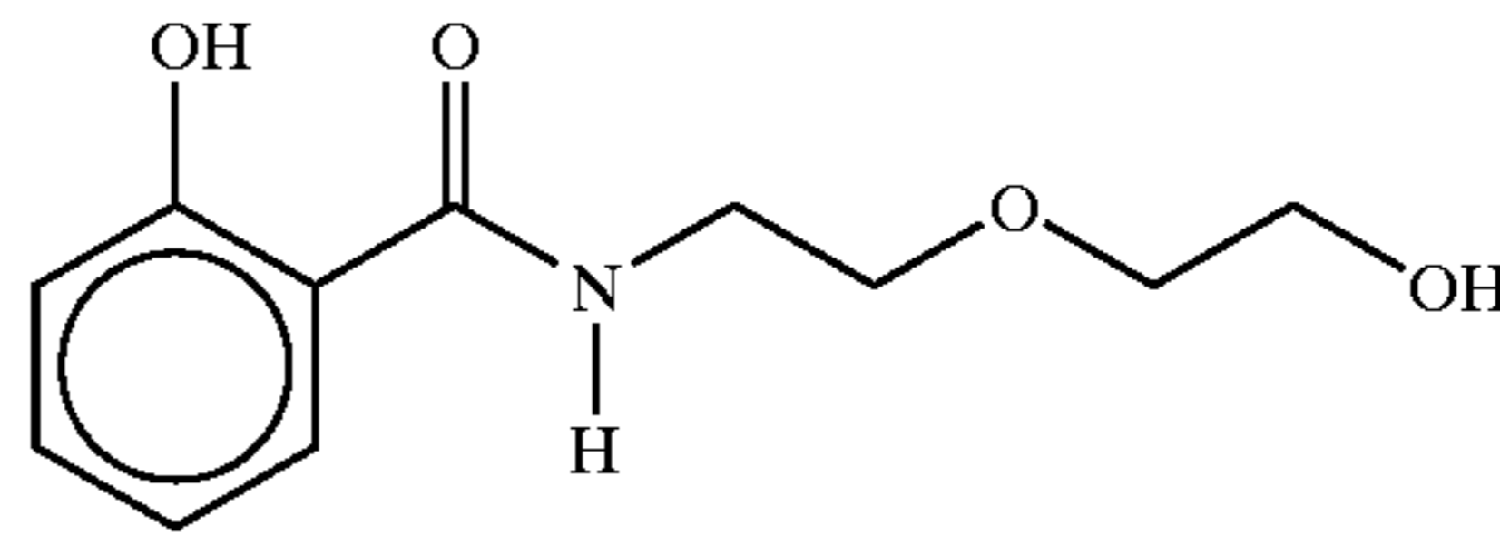
2-[N-(2-hydroxybenzoylamino)ethoxy]ethanol
