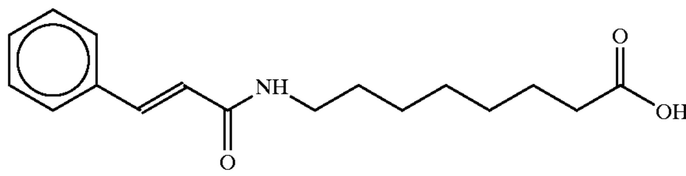
8-cinnamoylaminocaproic acid
