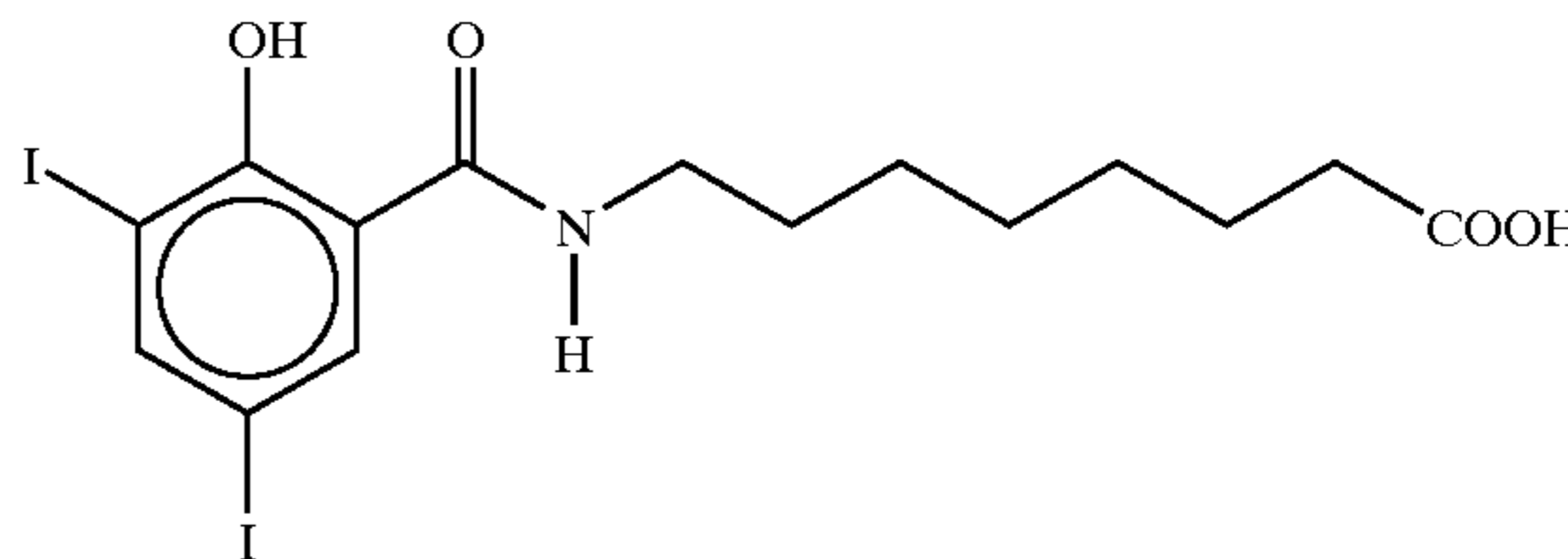
8-(N-2-hydroxy-3,5-diiodobenzoyl)aminocaprylic acid
