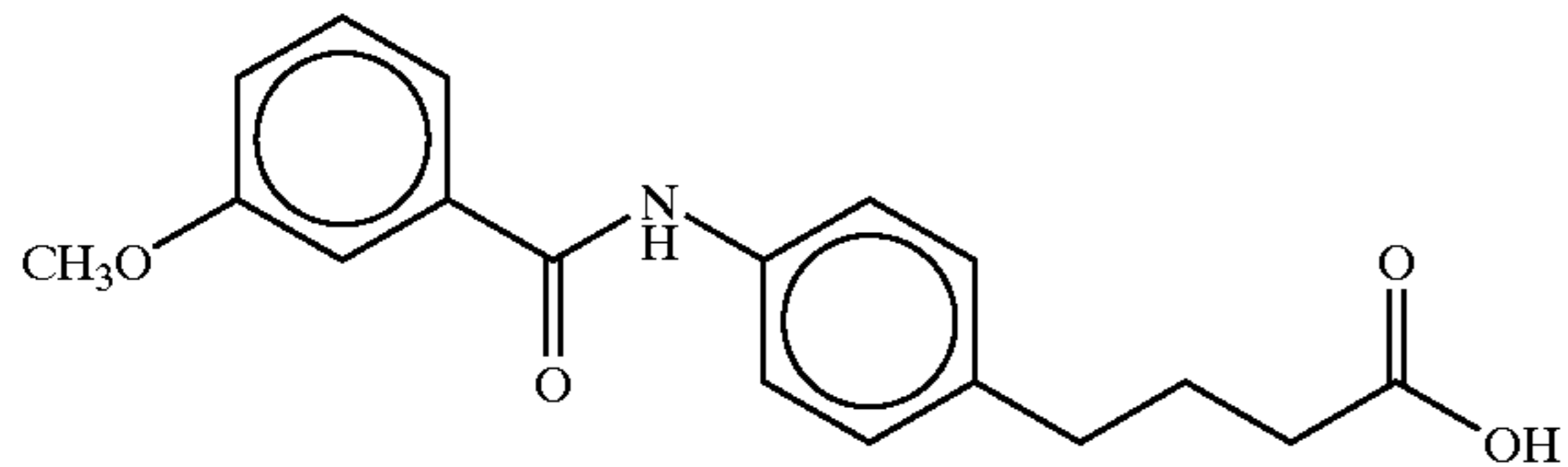
4-(4-(3-anisoyl)aminophenyl) butyric acid
