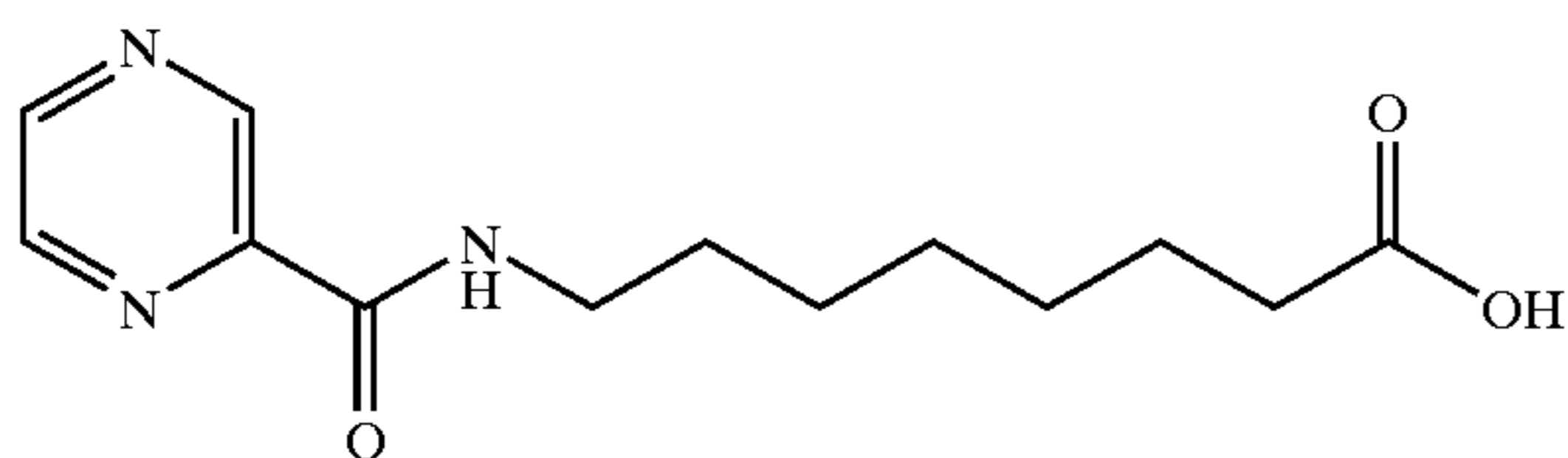
8-(2-pyrazinecarbonyl)aminocaproic acid
