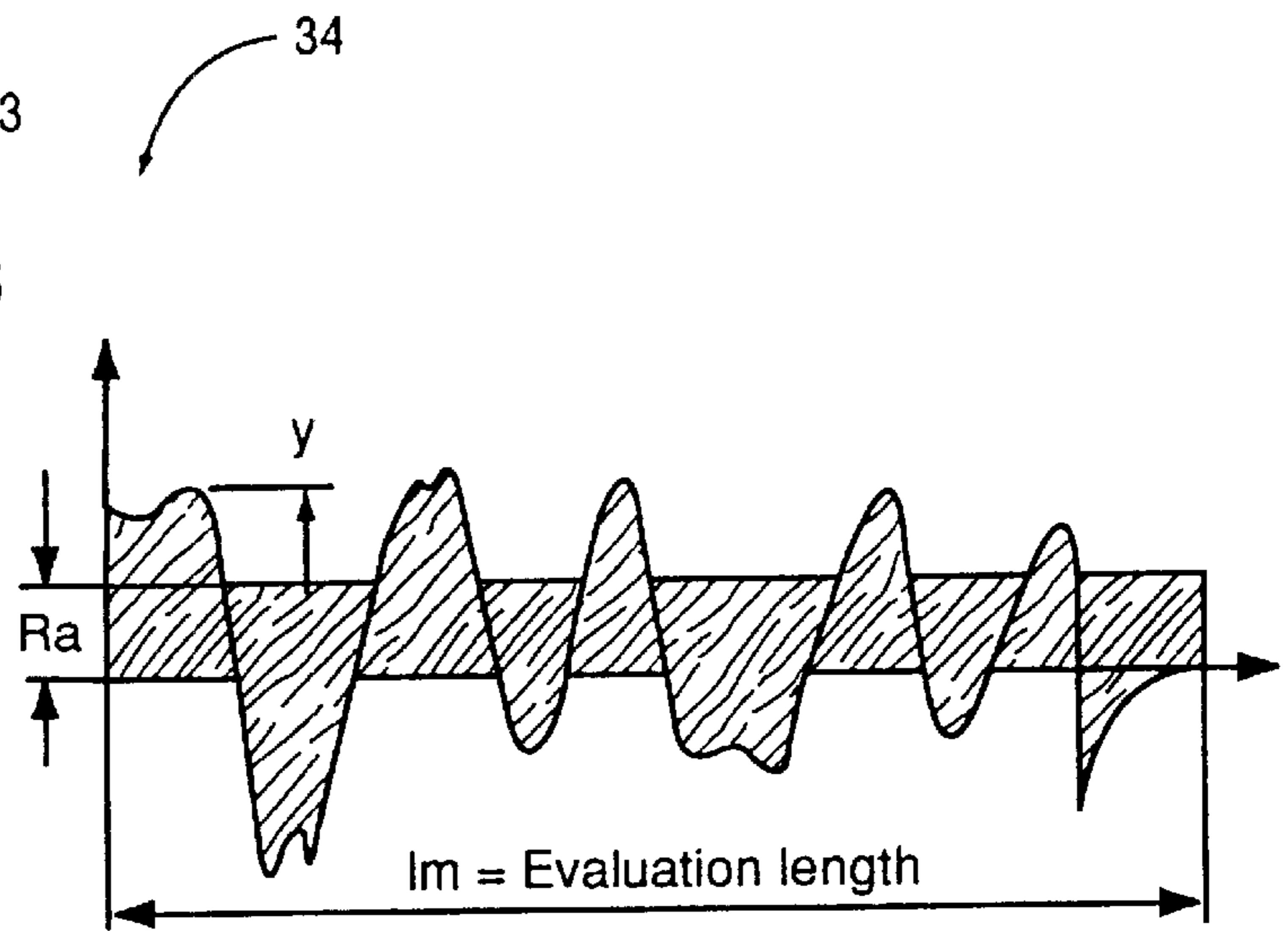
FIG. 3 PRIOR ART
