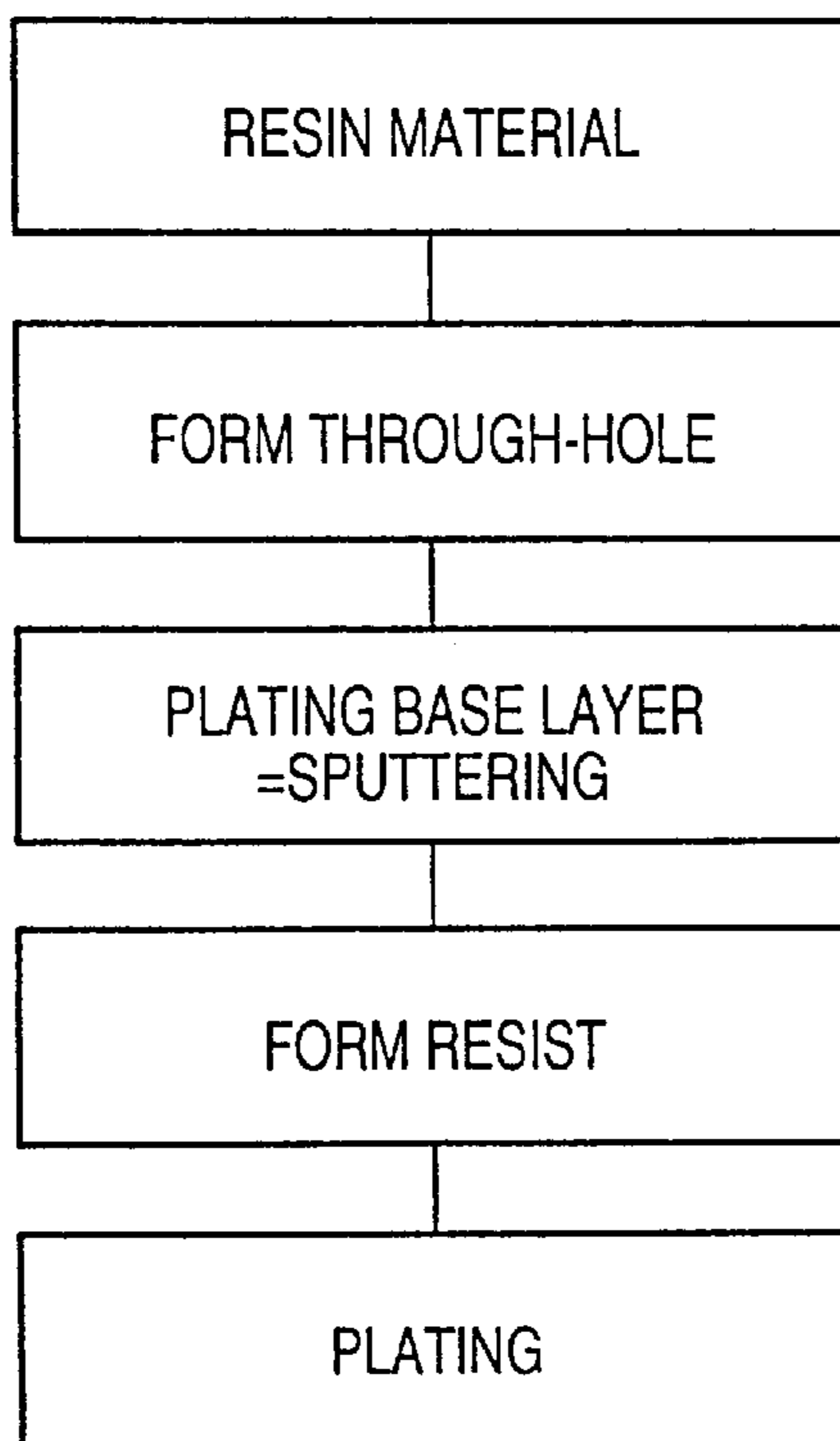
Fig. 2 PRIOR ART
