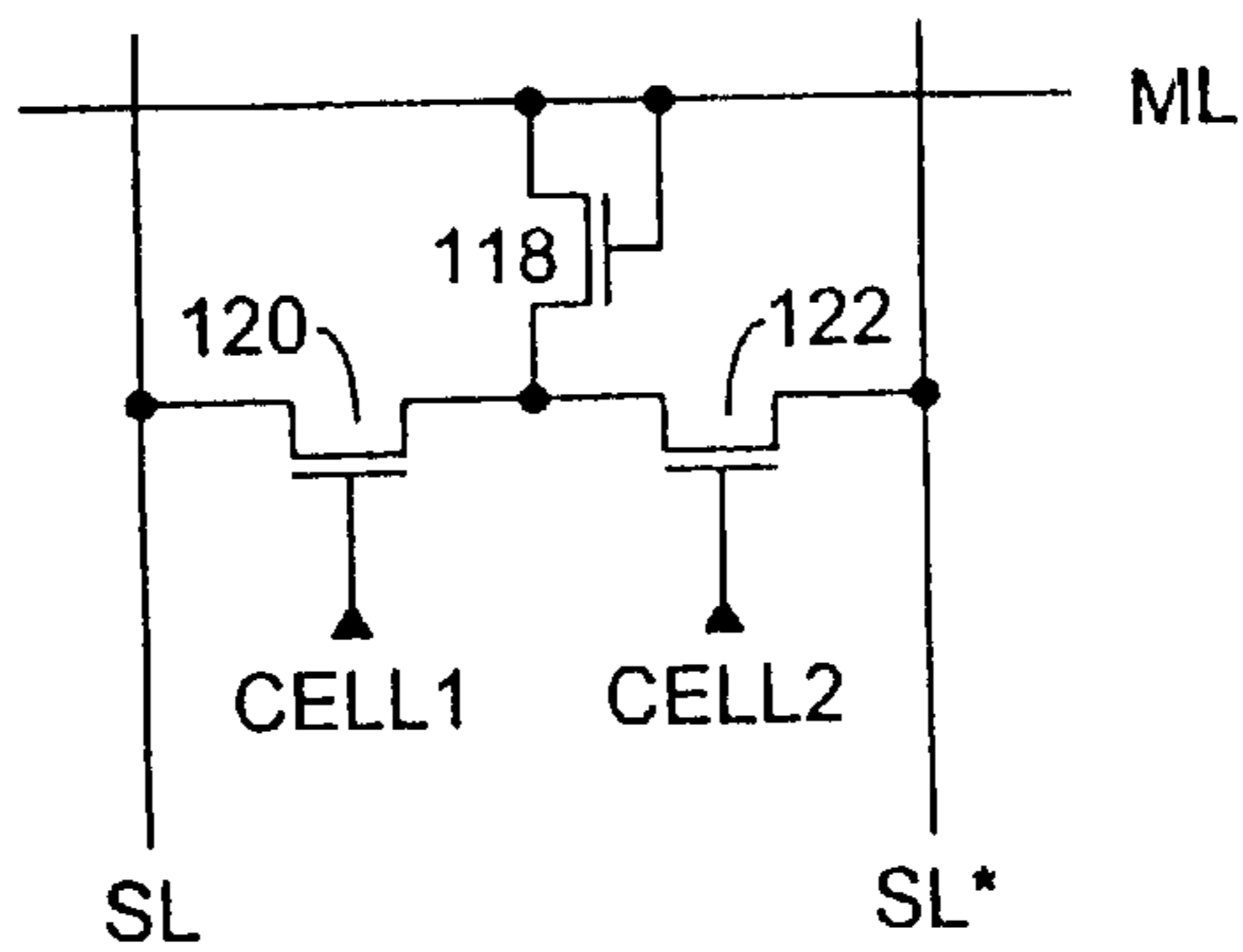
Fig. 4 (prior art)
