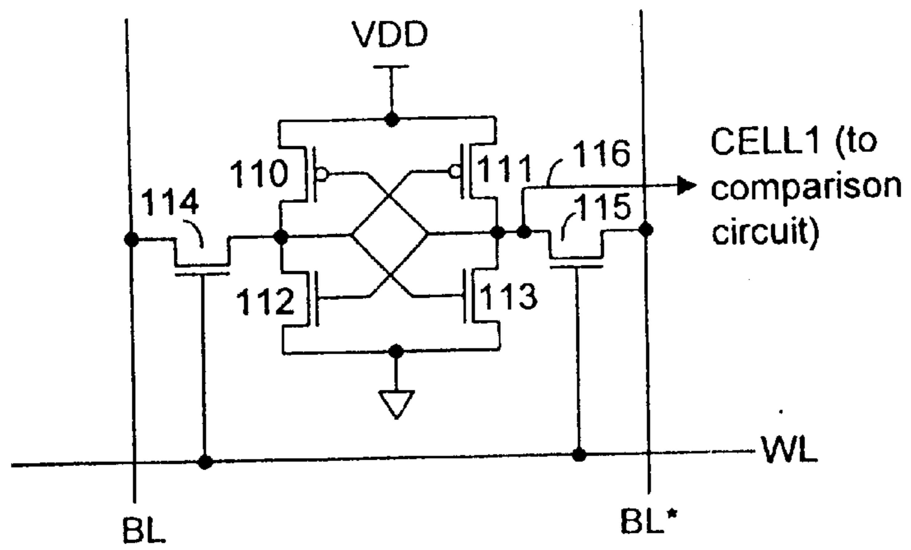
Fig. 3 (prior art)
