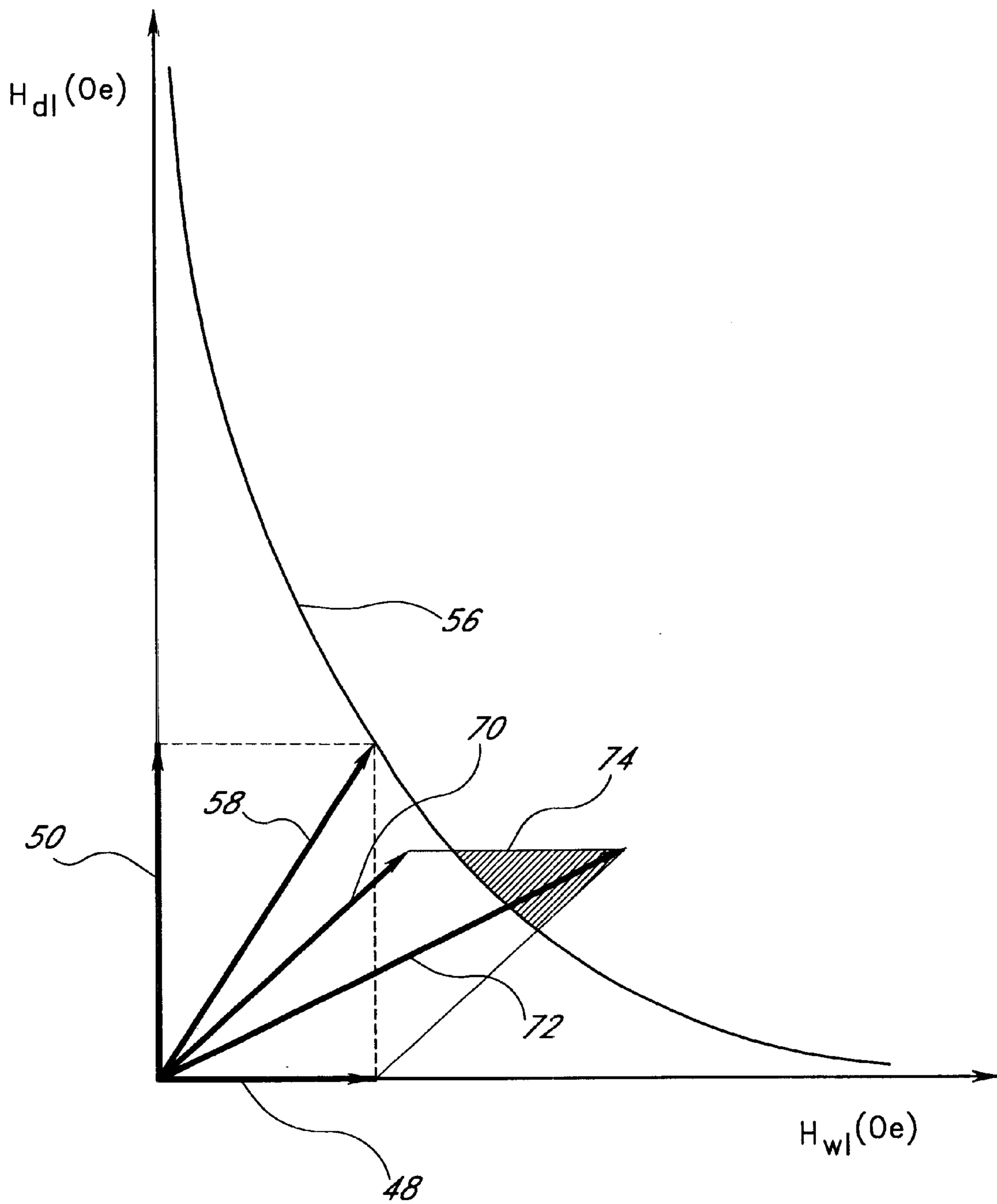
FIG. 2 (PRIOR ART)
