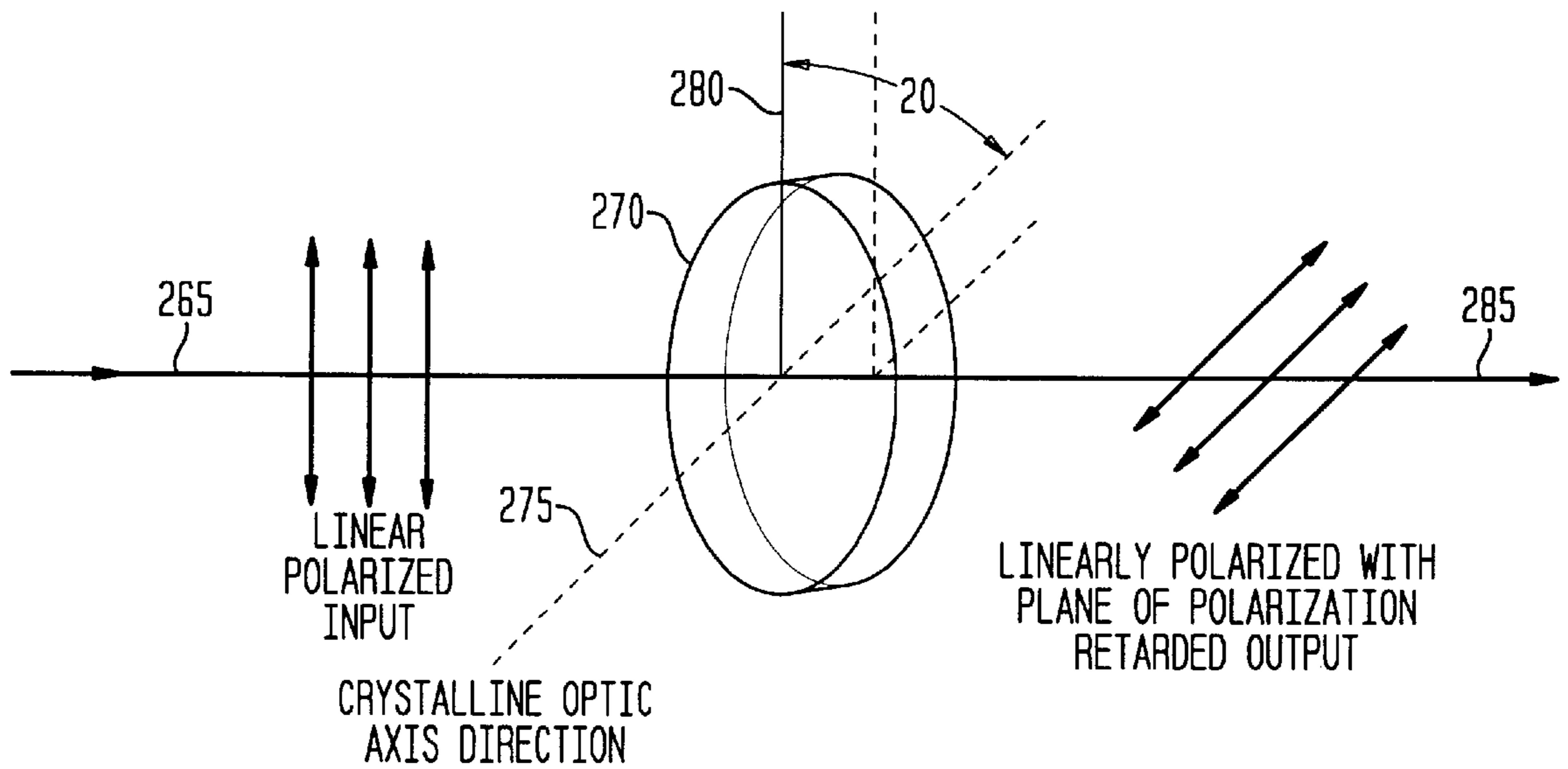
FIG. 2C \lambda/2 WAVEPLATE
