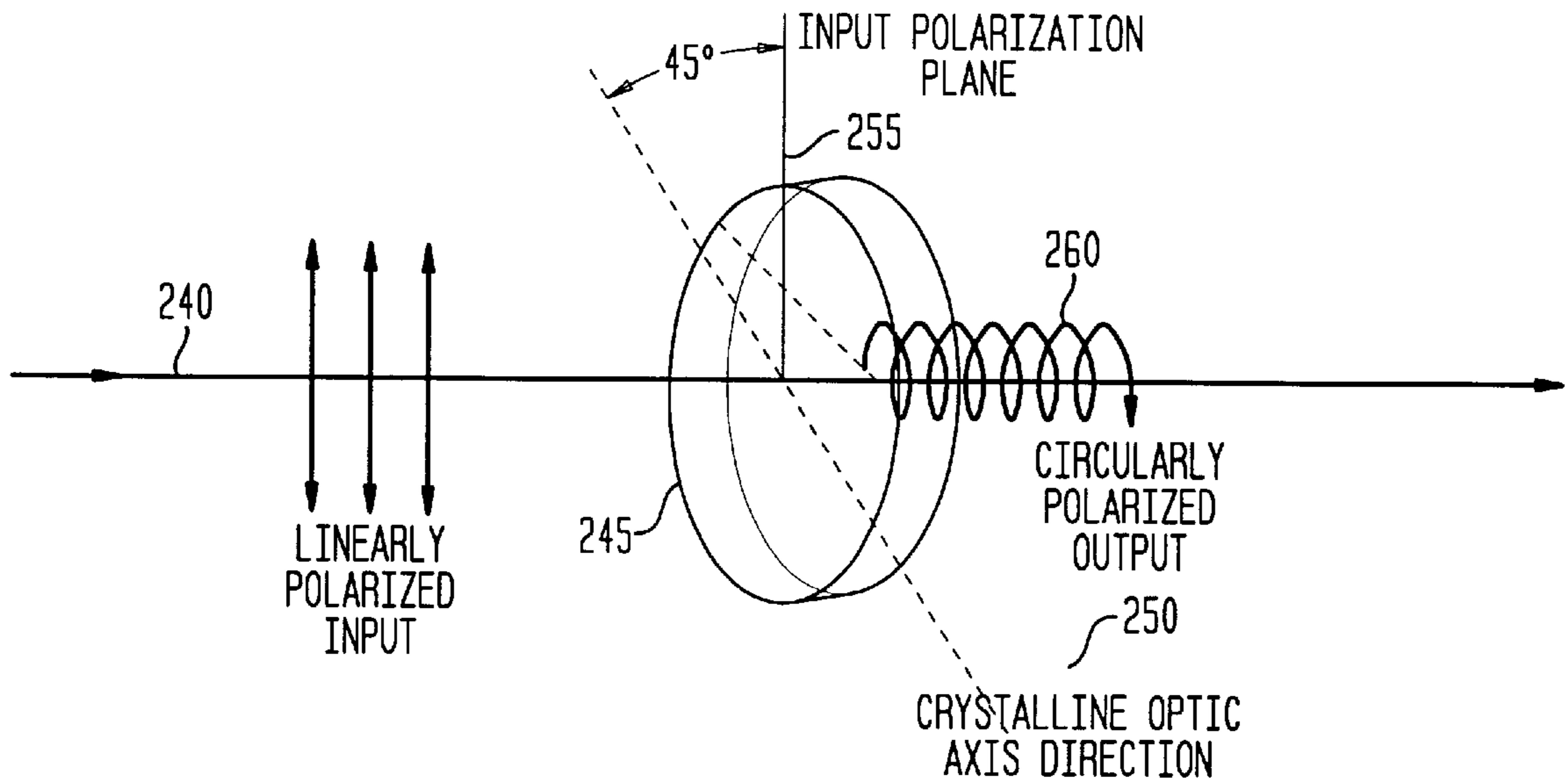
FIG. 2B \lambda/4 WAVEPLATE
