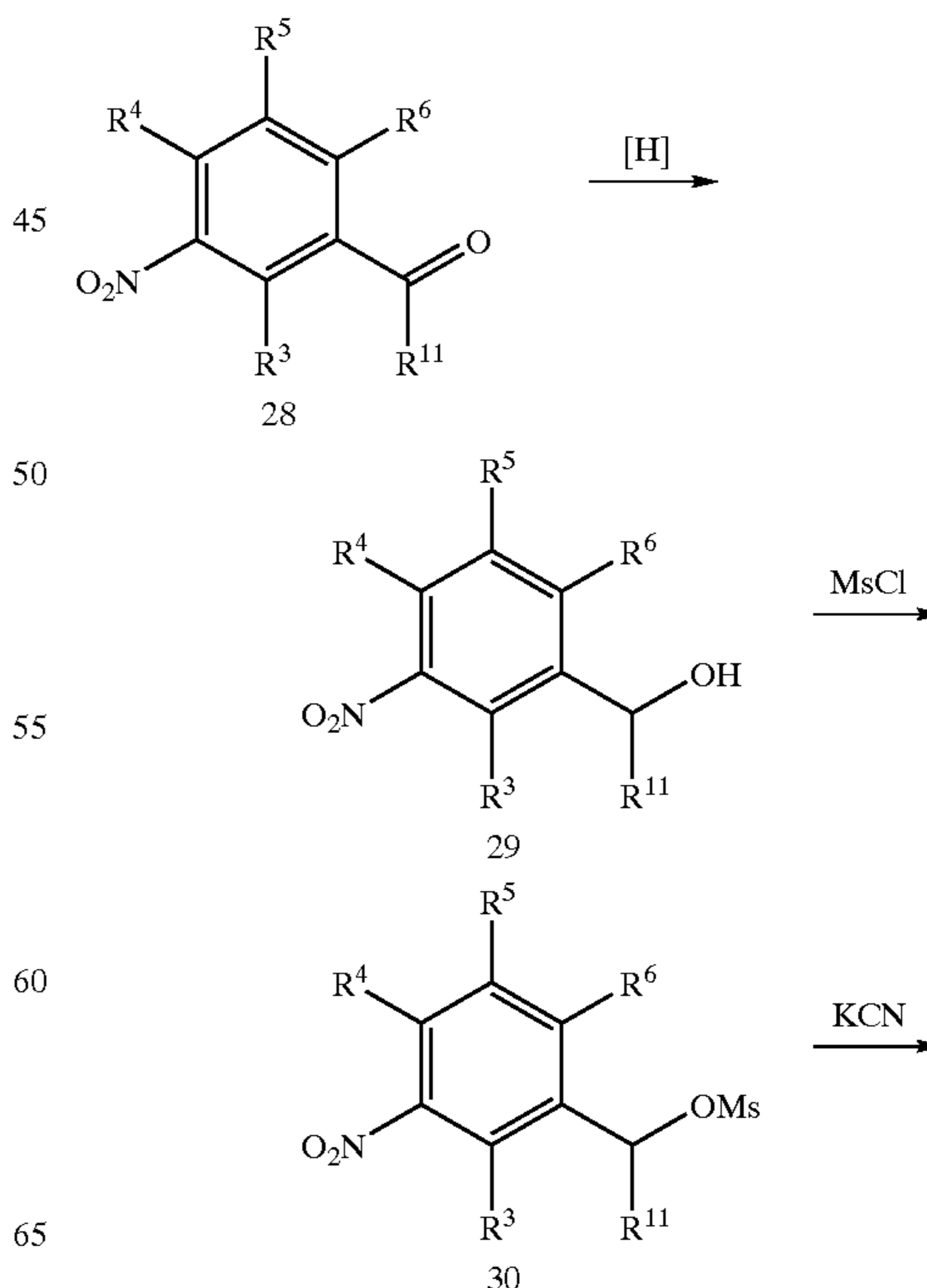
Scheme 6
