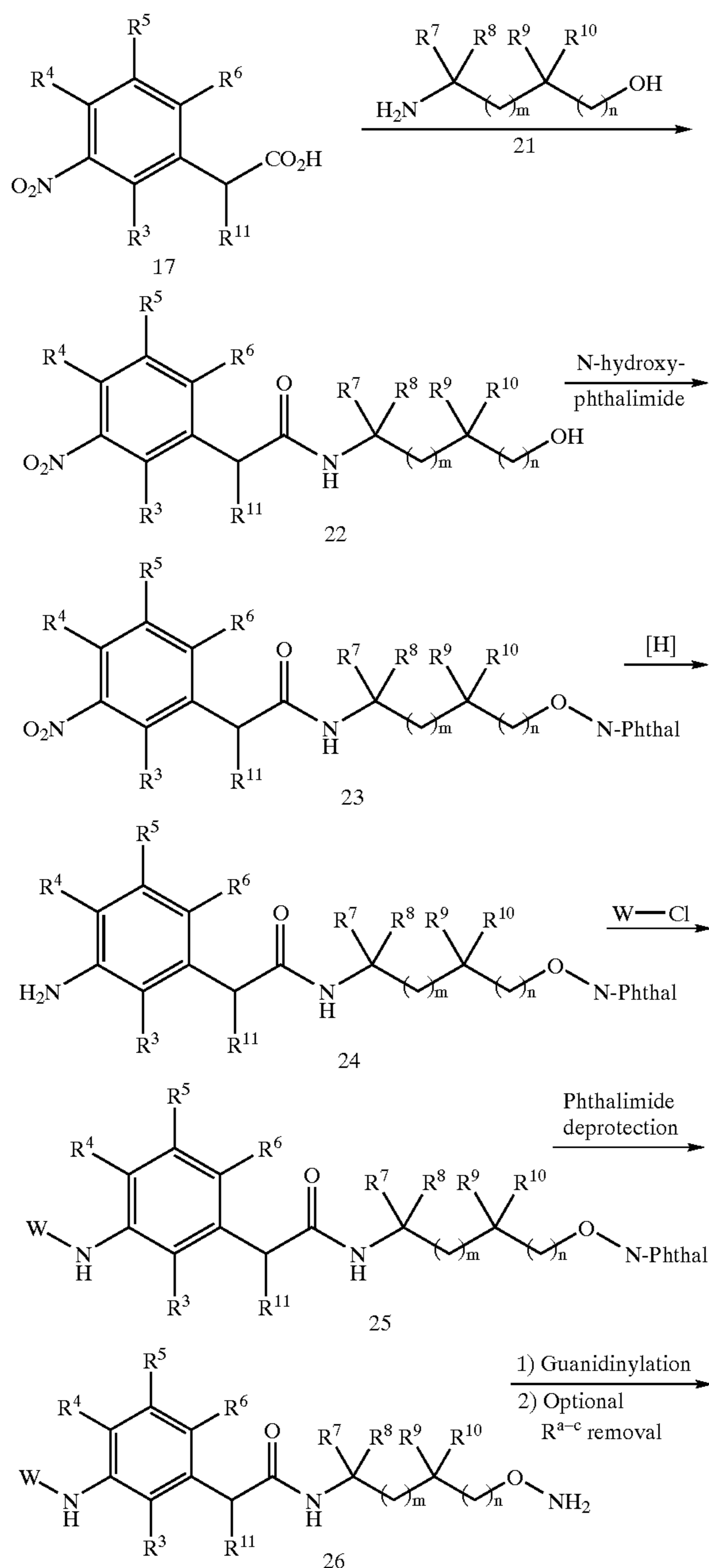
Scheme 5
