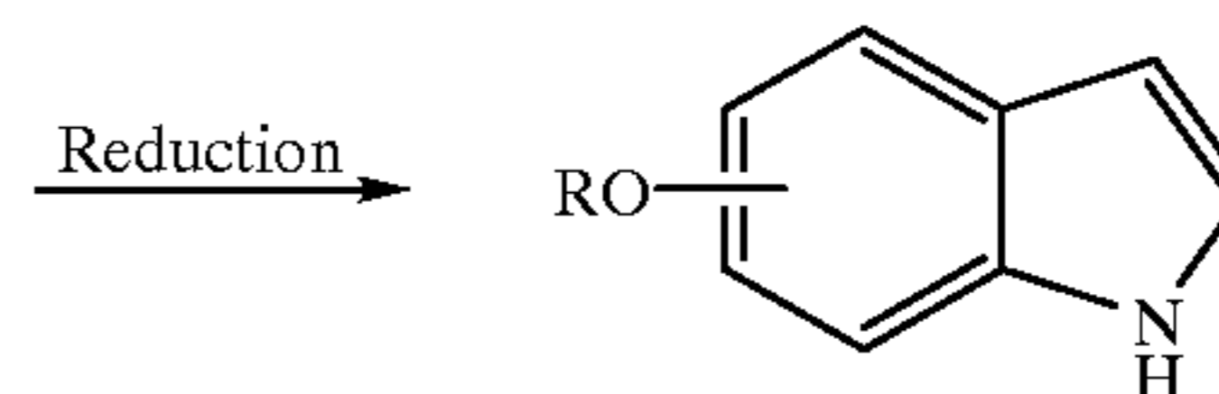
Scheme J
