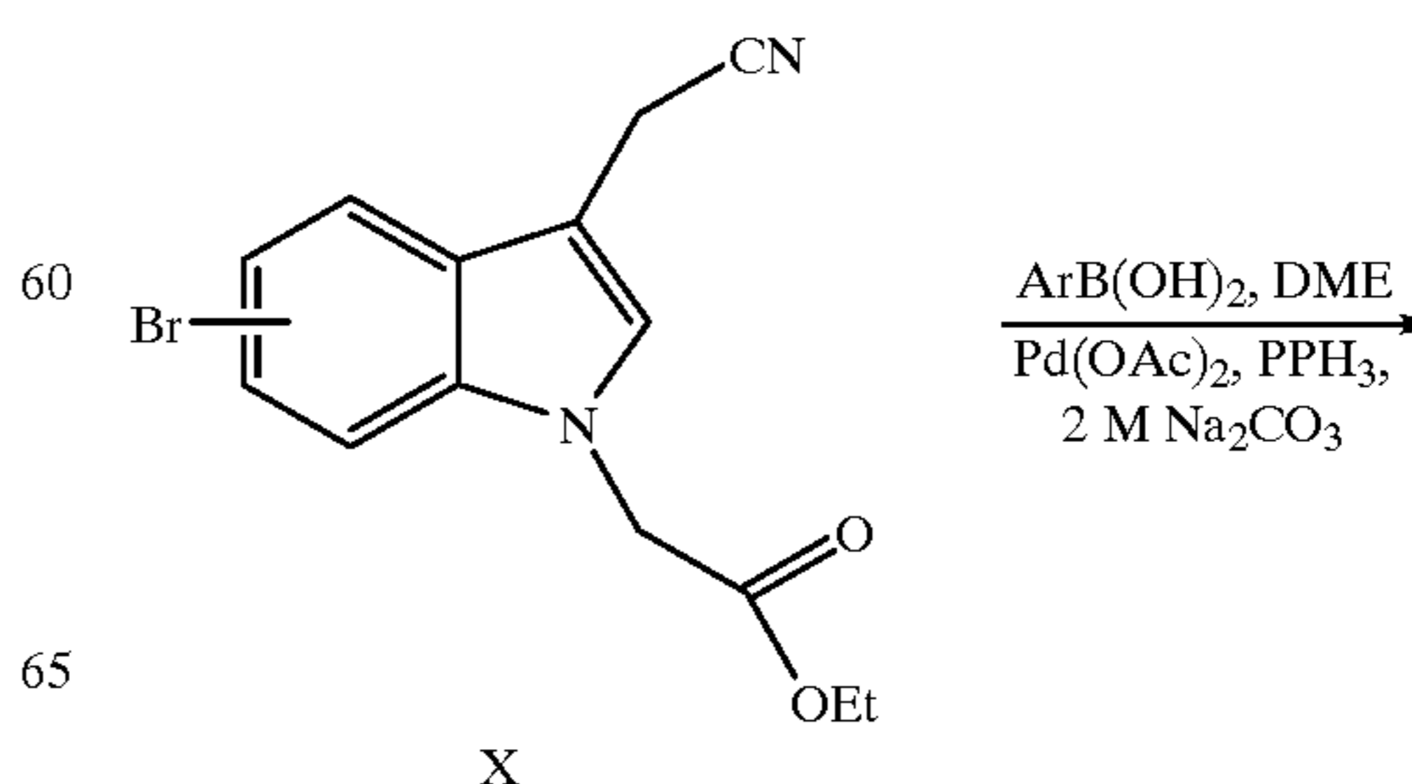
Scheme E
