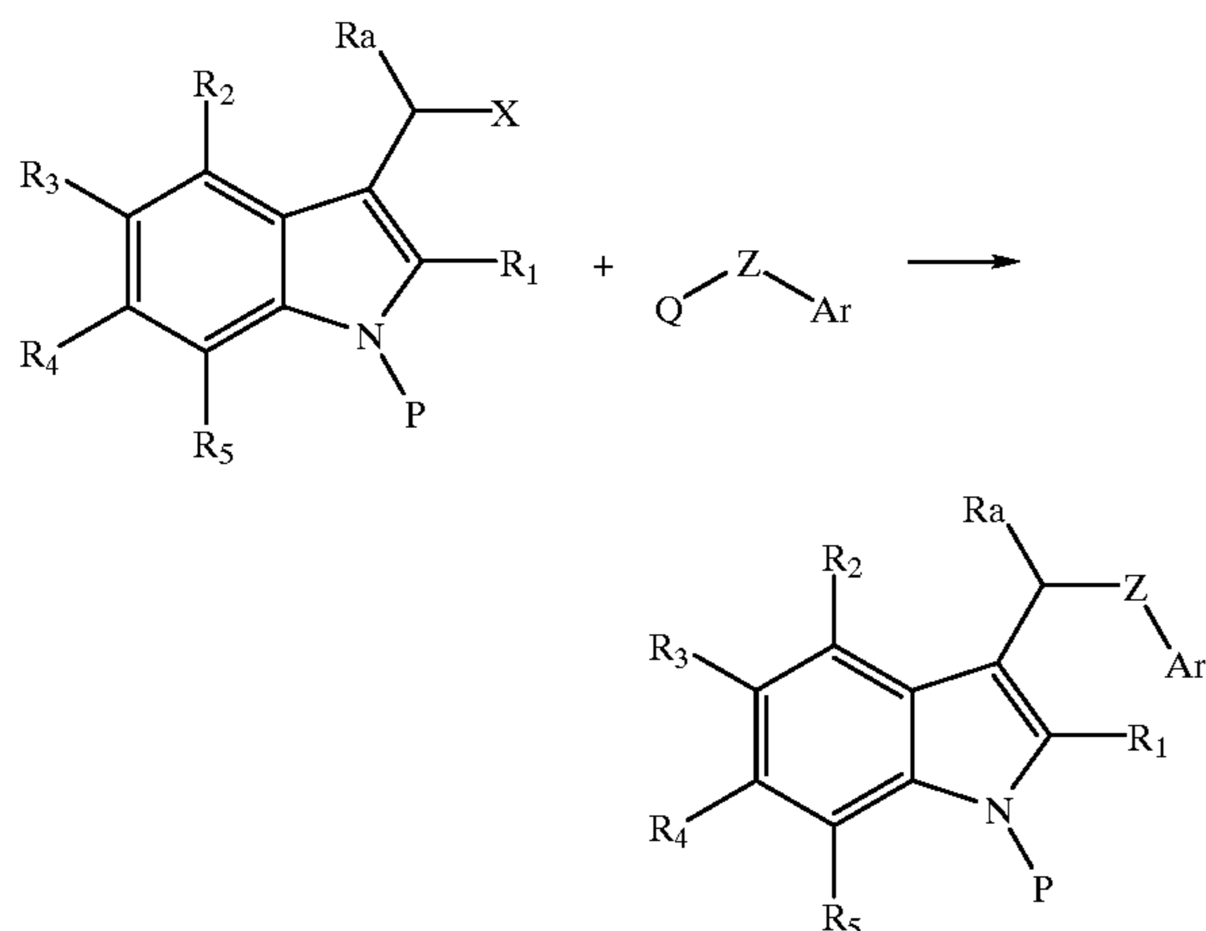
Scheme C
