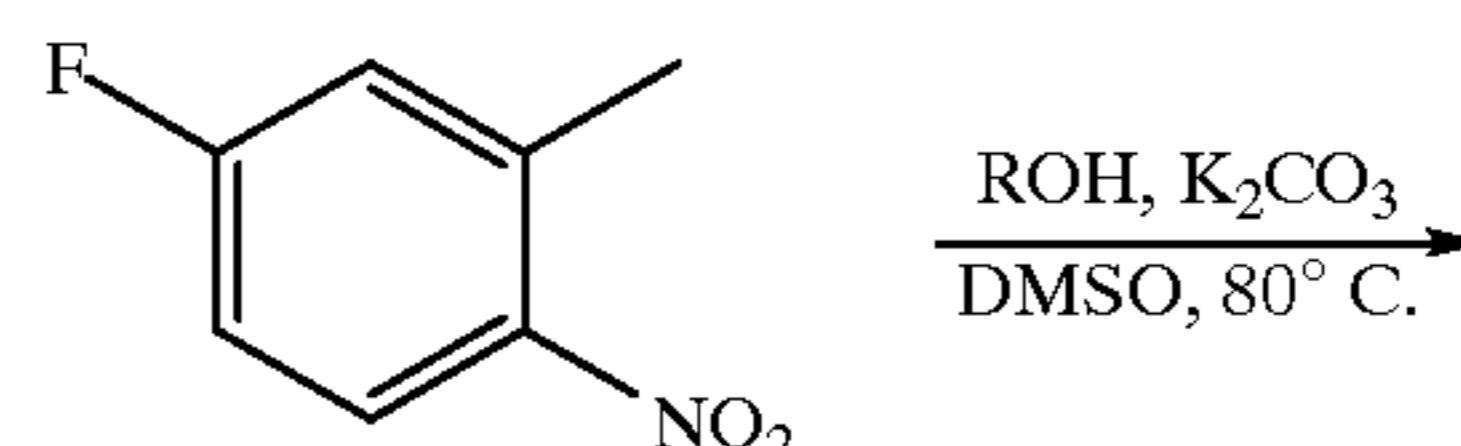
Scheme G
