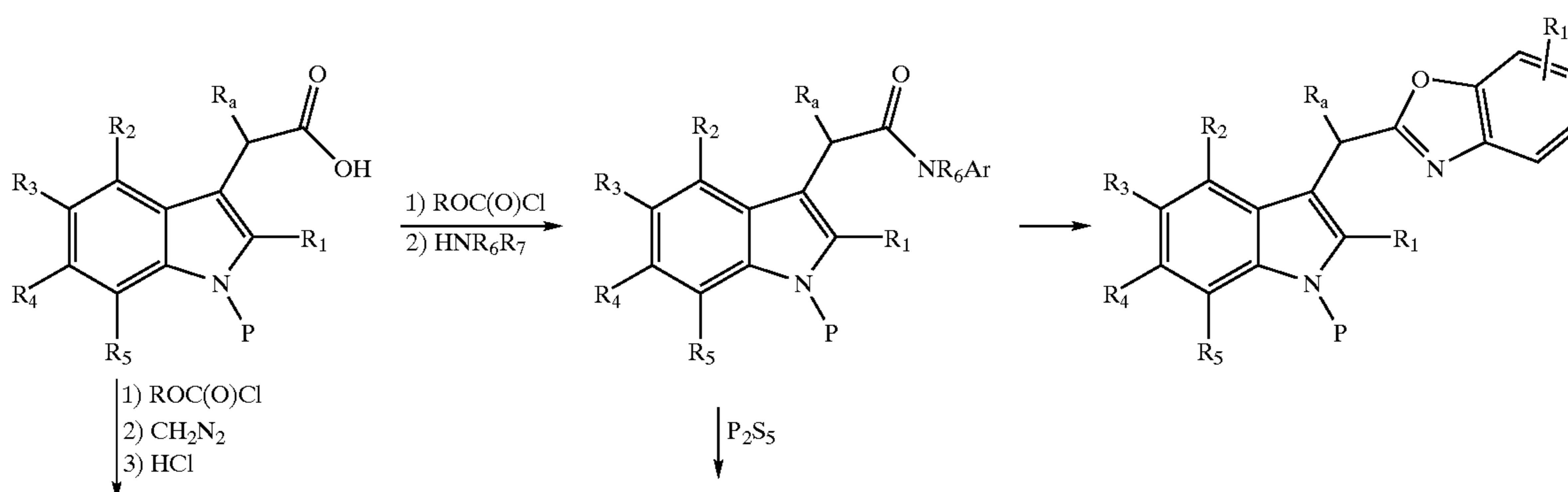
Scheme I
