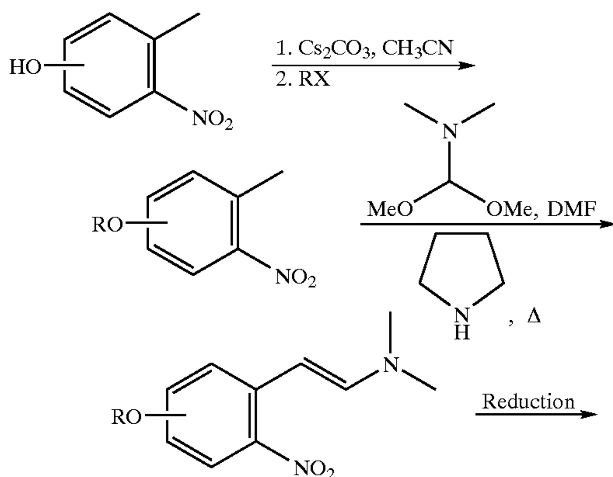
Scheme H
