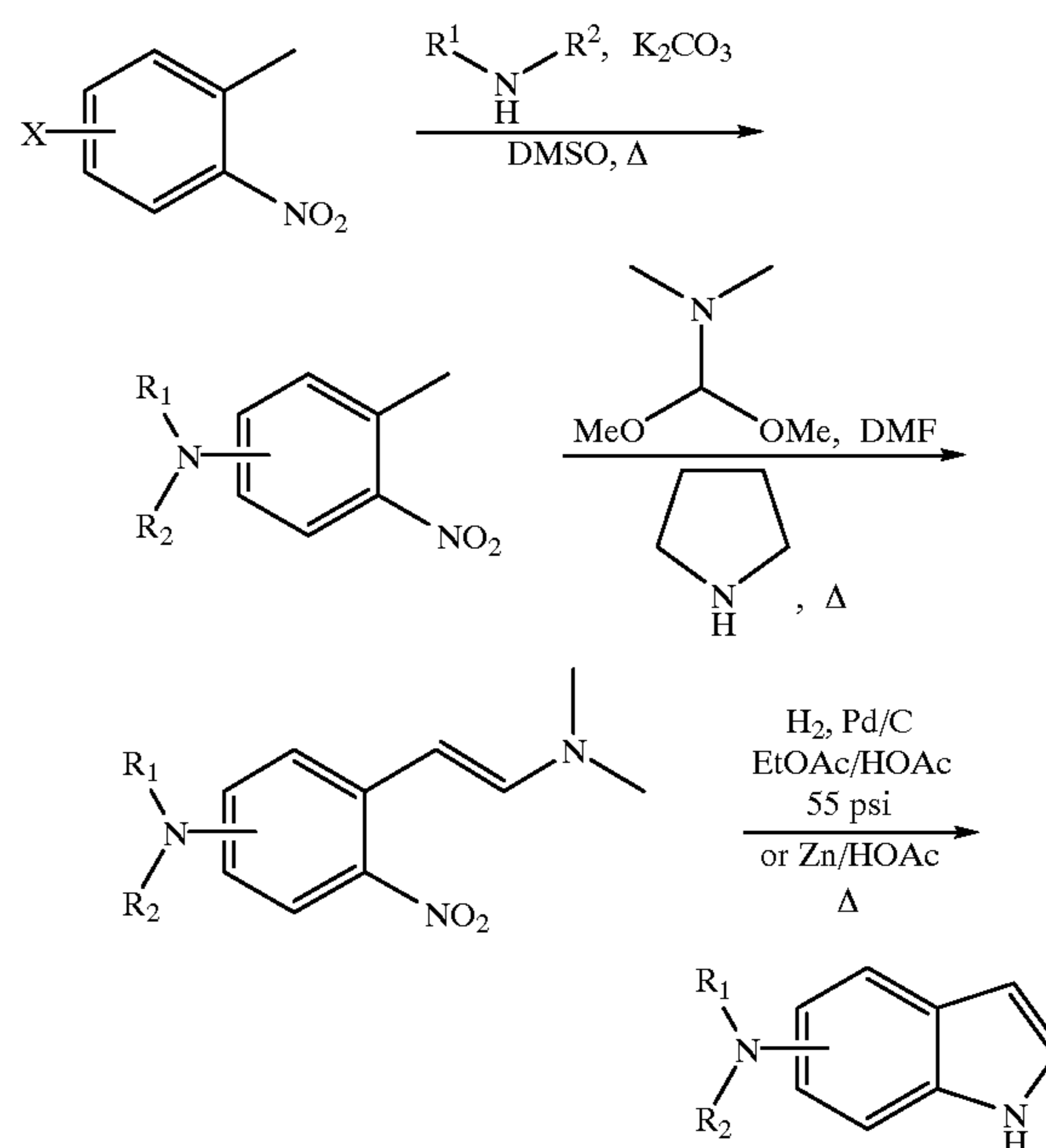
Scheme F
