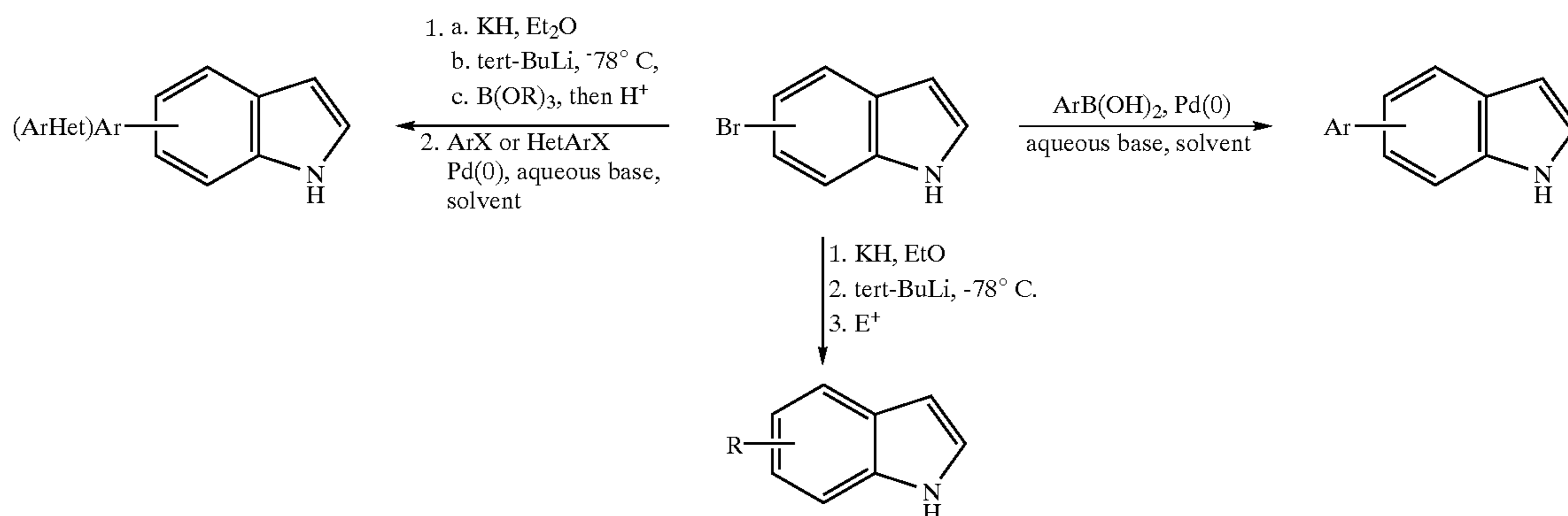
Scheme D
