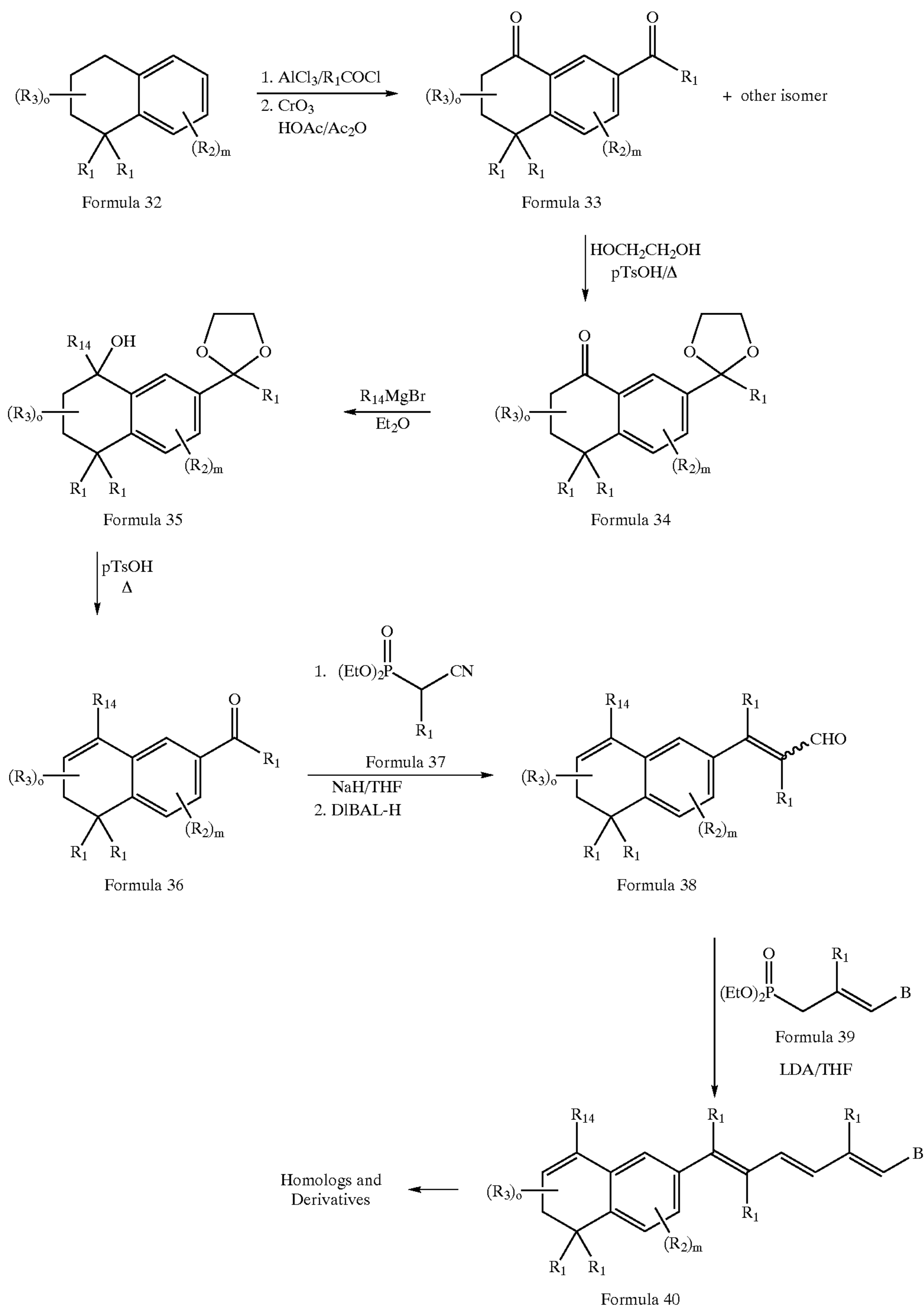
Reaction Scheme 4
