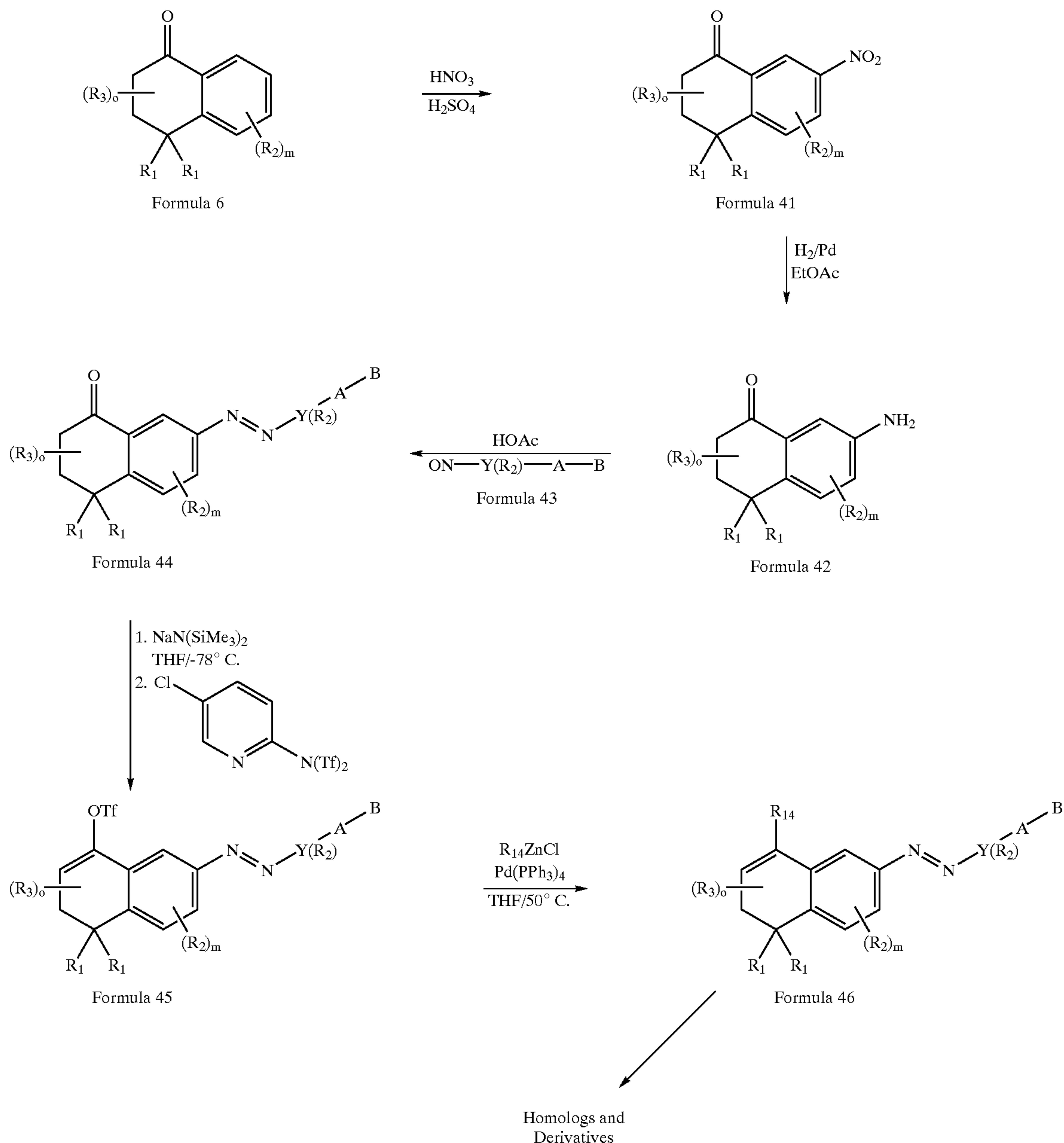
Reaction Scheme 5
