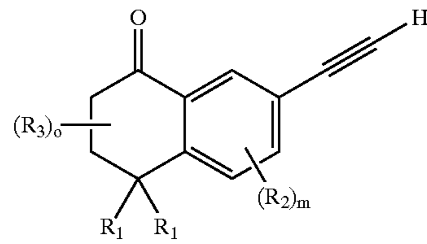
Formula 9
