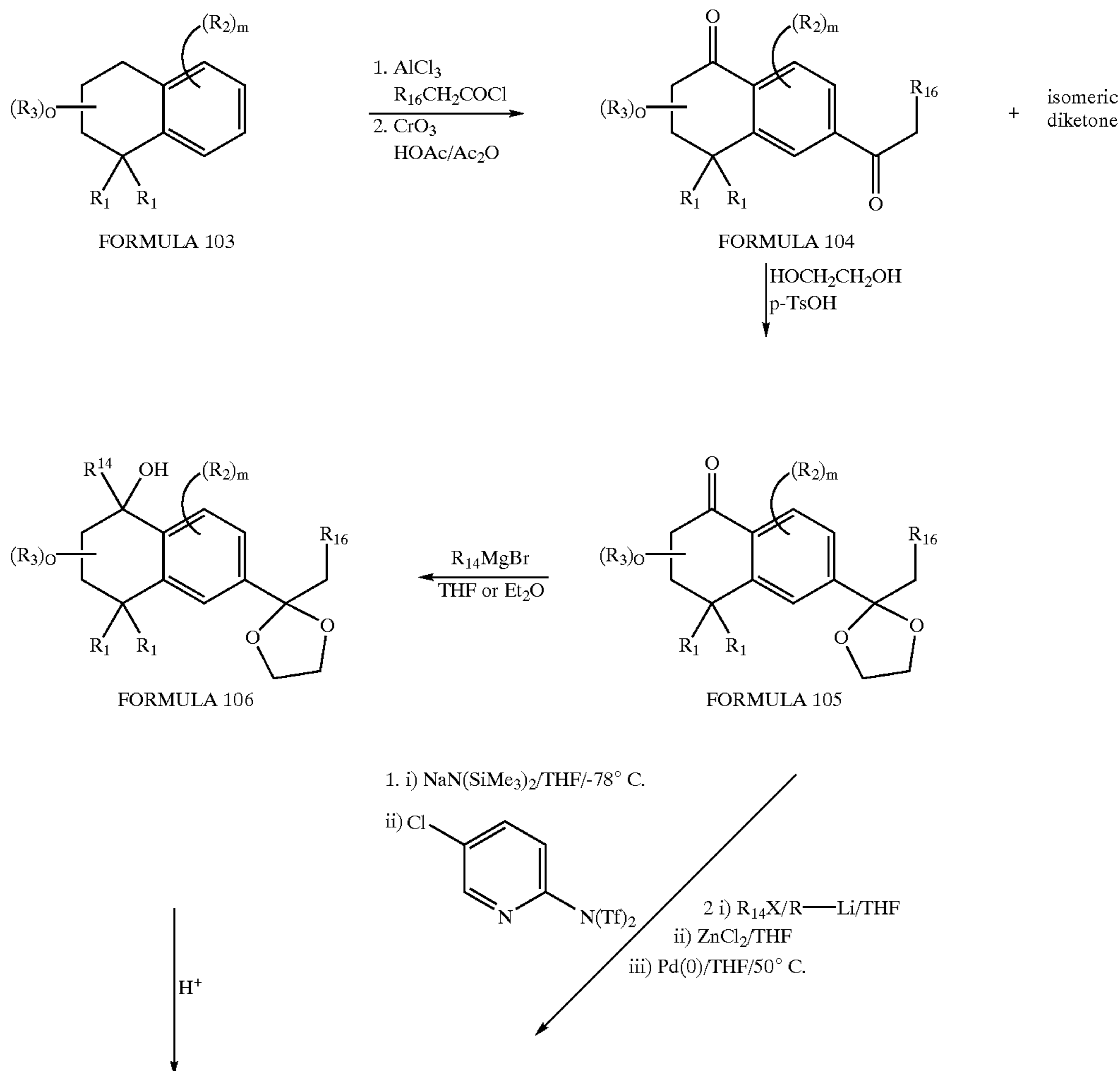
Reaction Scheme 101
