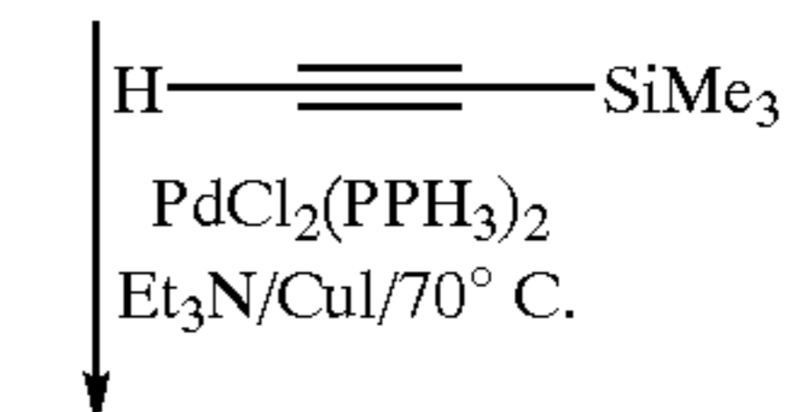
Formula 7
