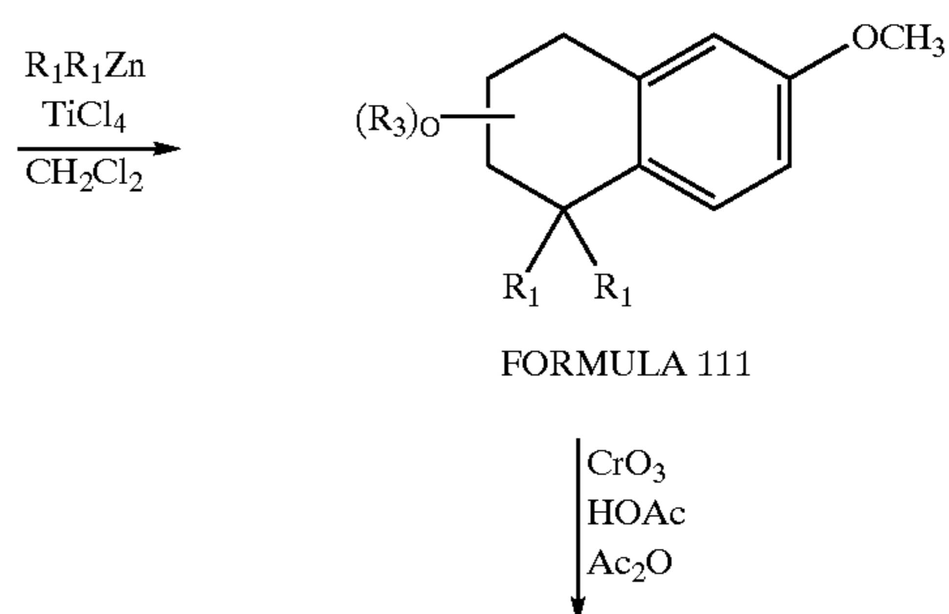
Reaction Scheme 102
