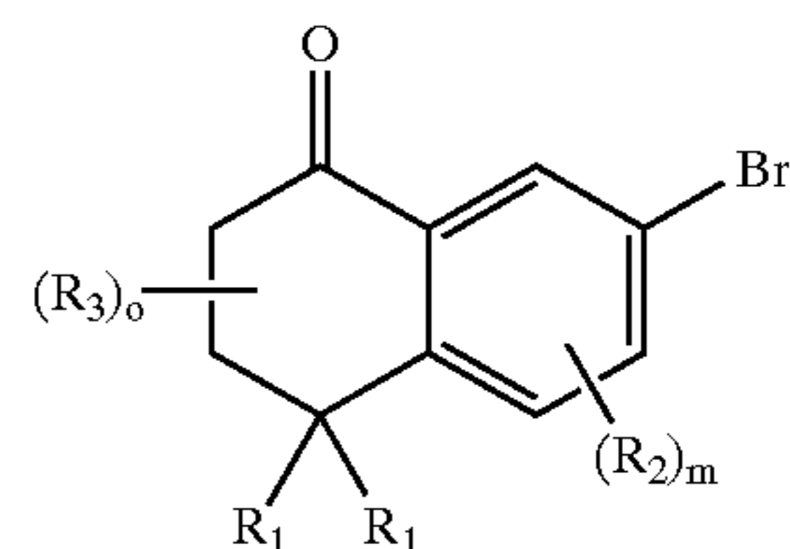
Formula 7
