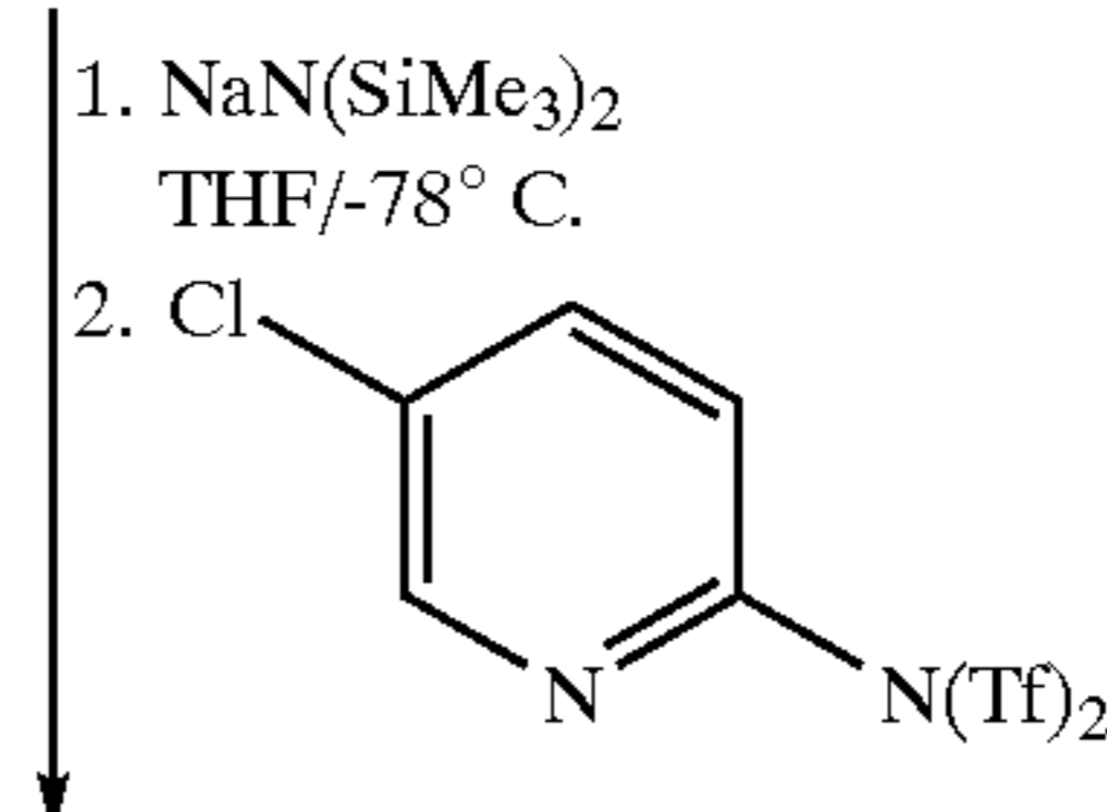
Formula 23
