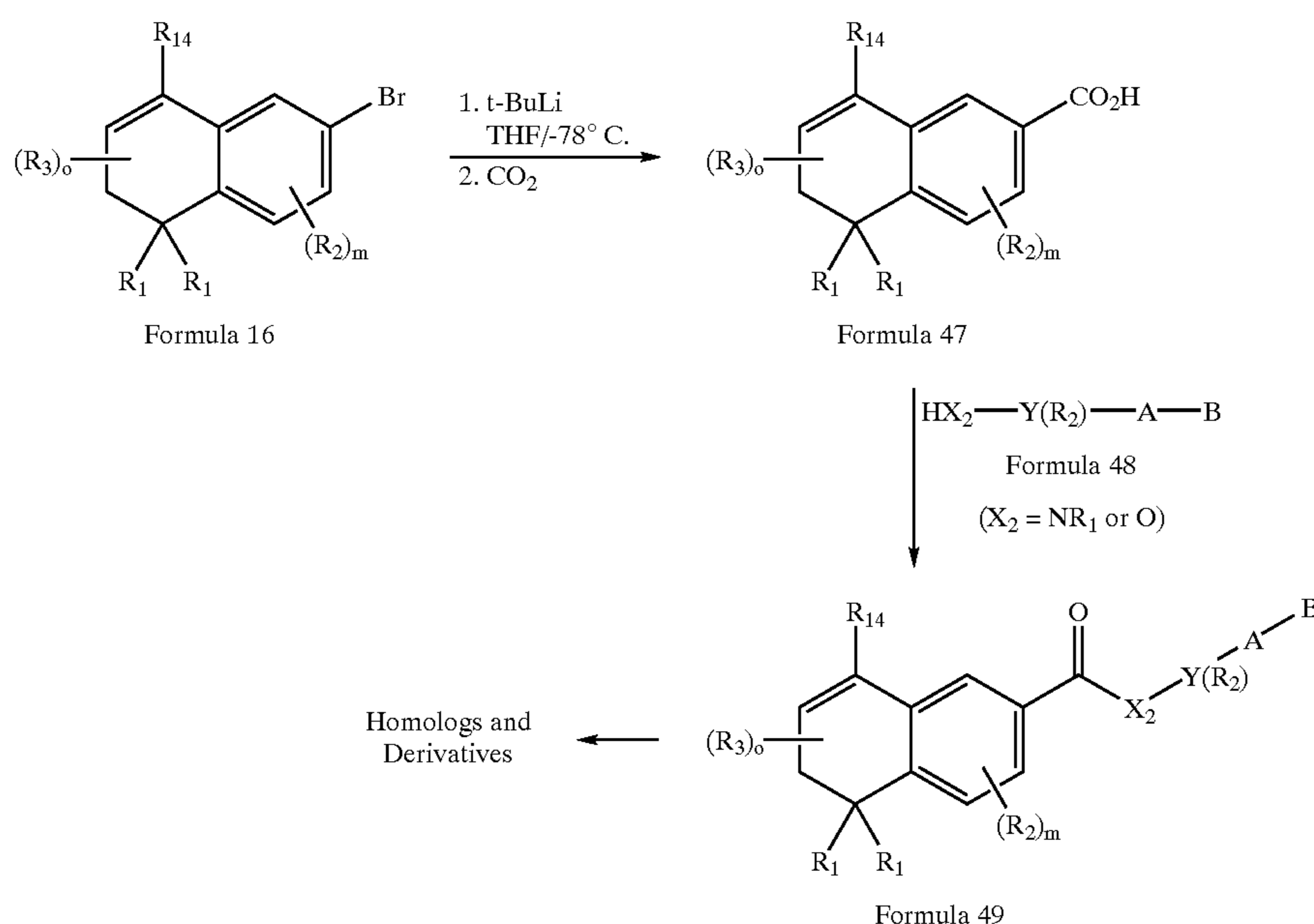
Reaction Scheme 6
