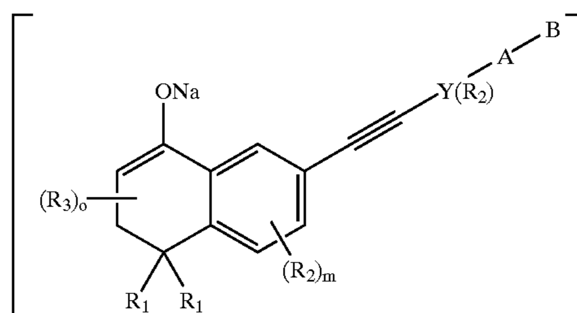
Formula 12
