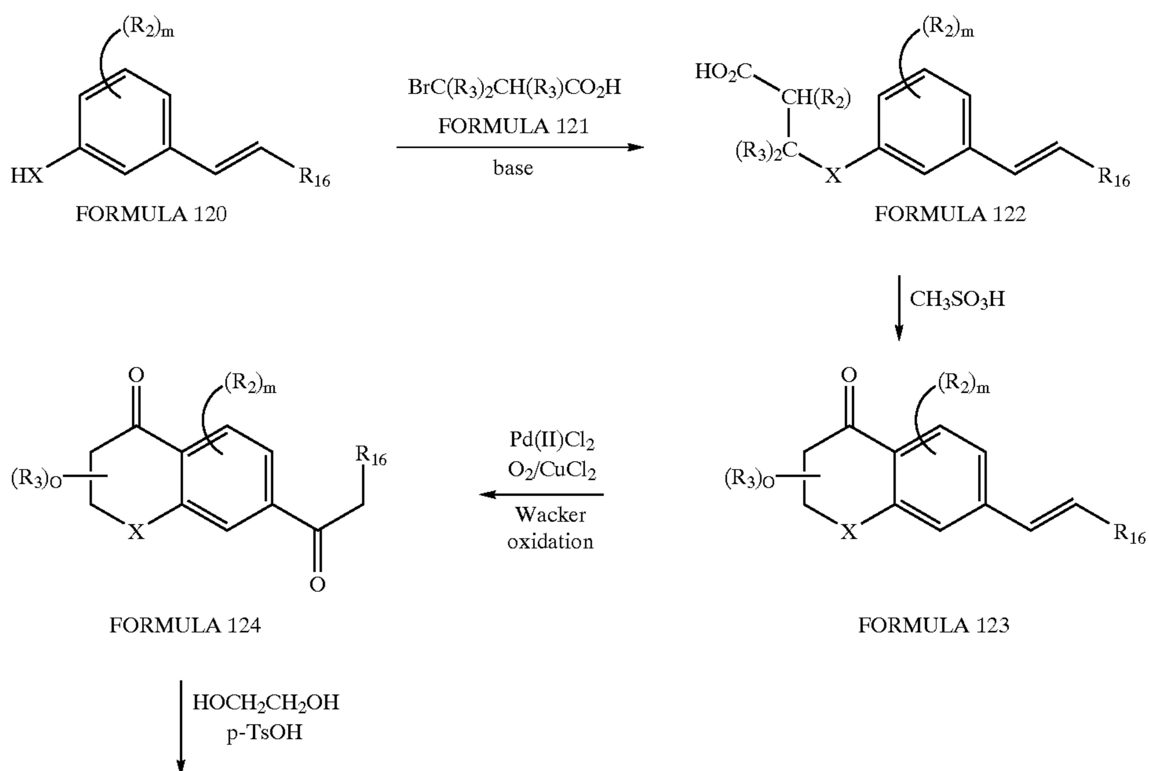
Reaction Scheme 103
