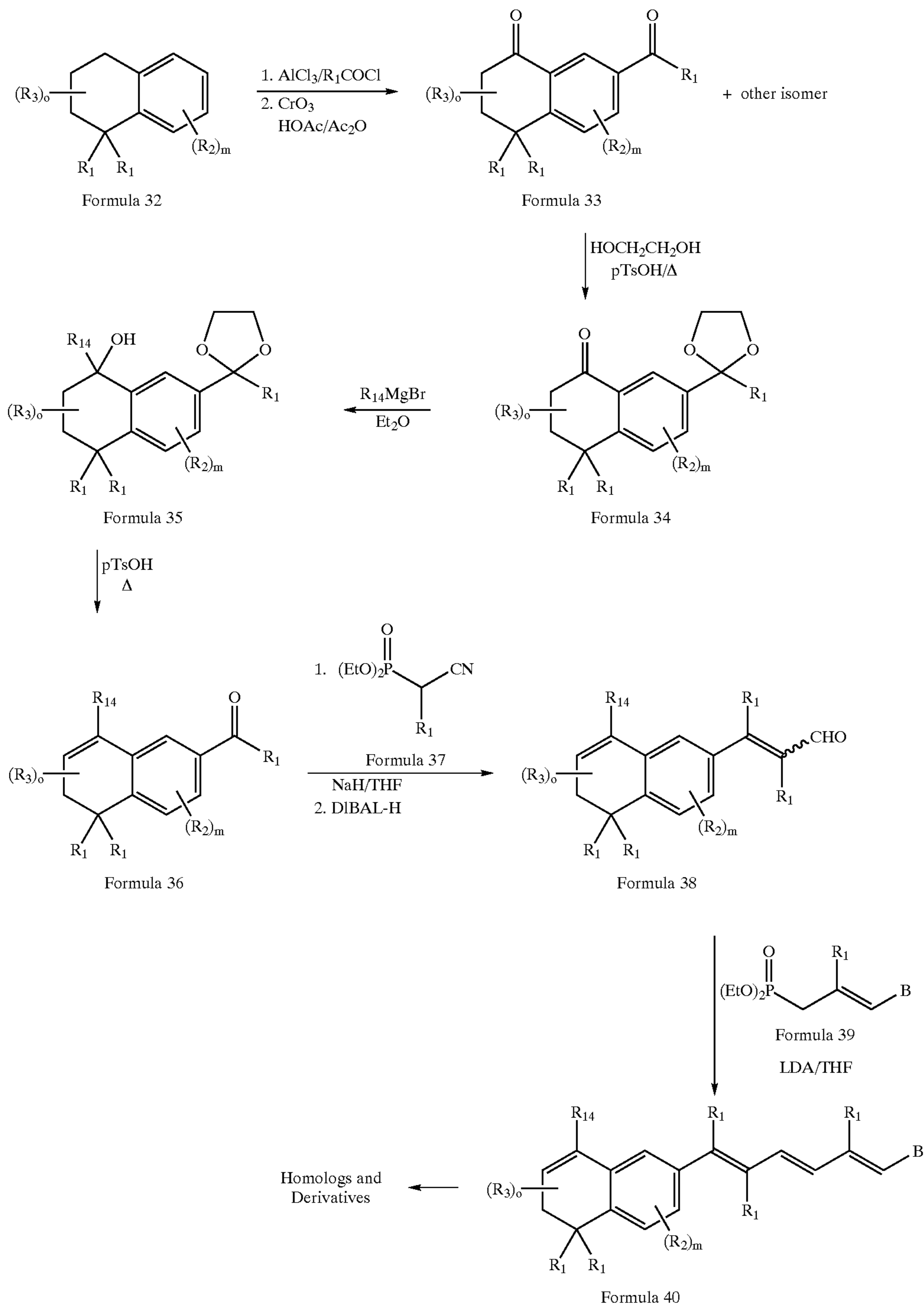
Reaction Scheme 4
