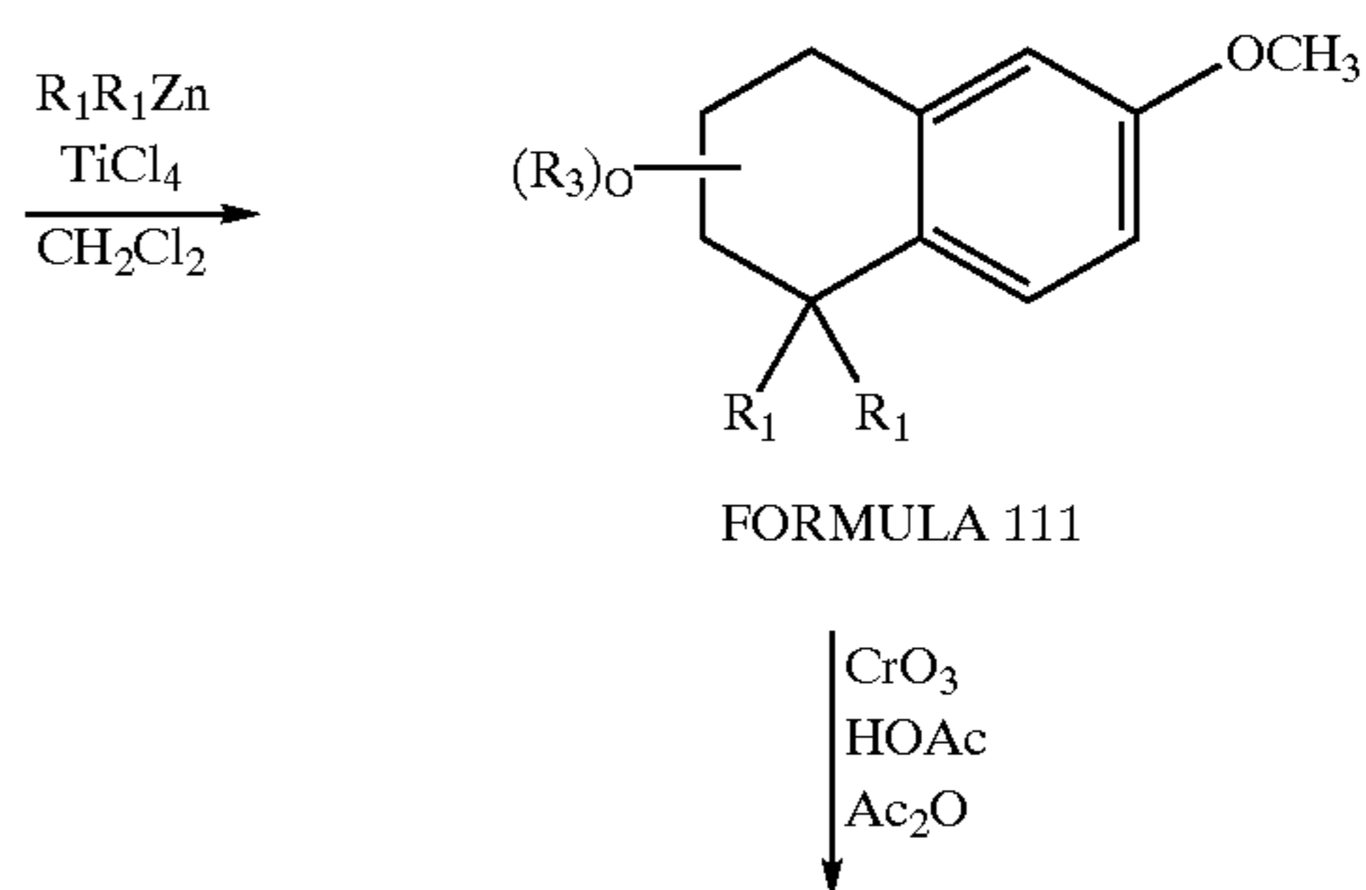
Reaction Scheme 102
