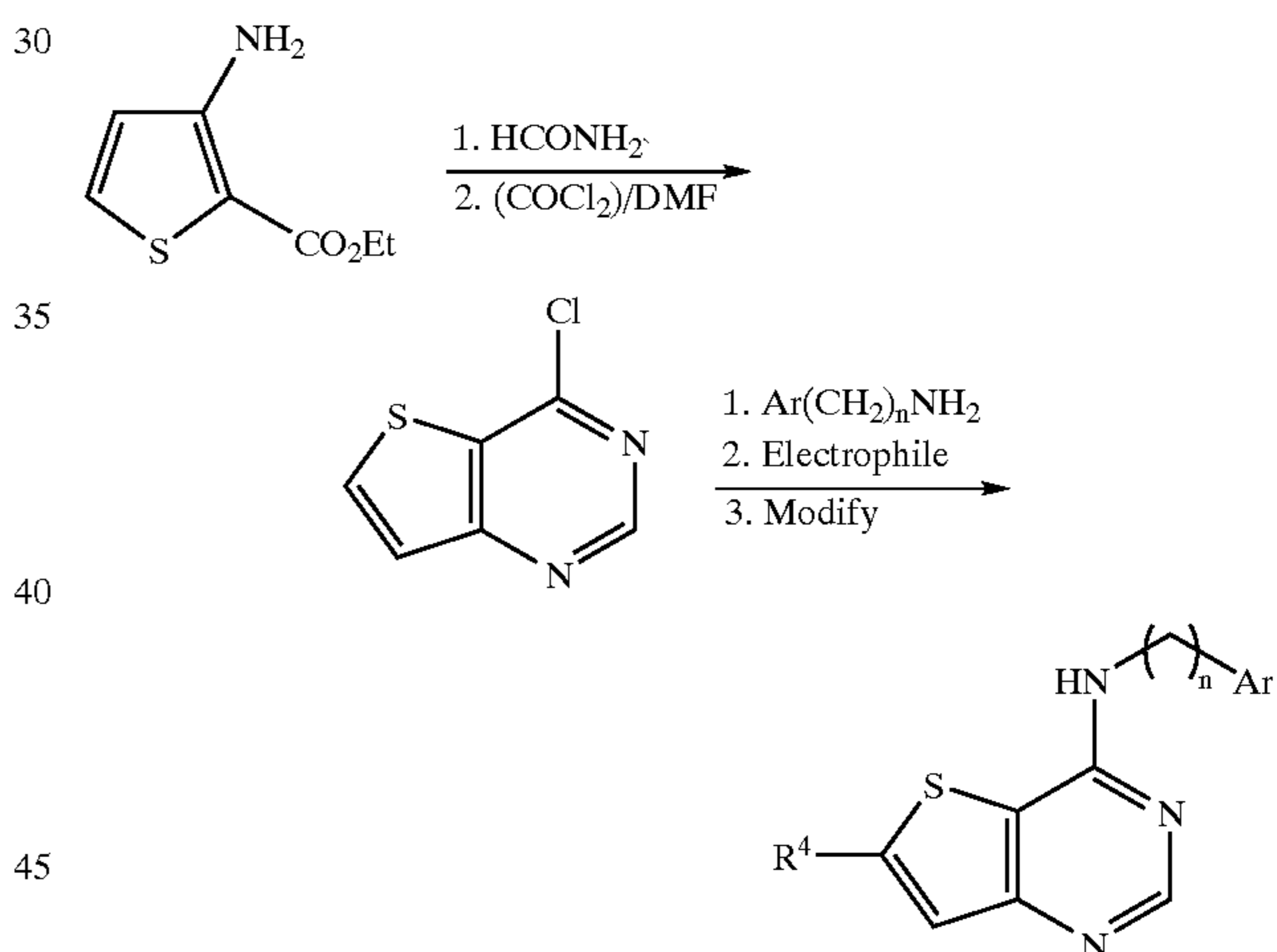
Scheme 17 Synthesis of Preferred Group 41; [3,2-d] ring fusion
