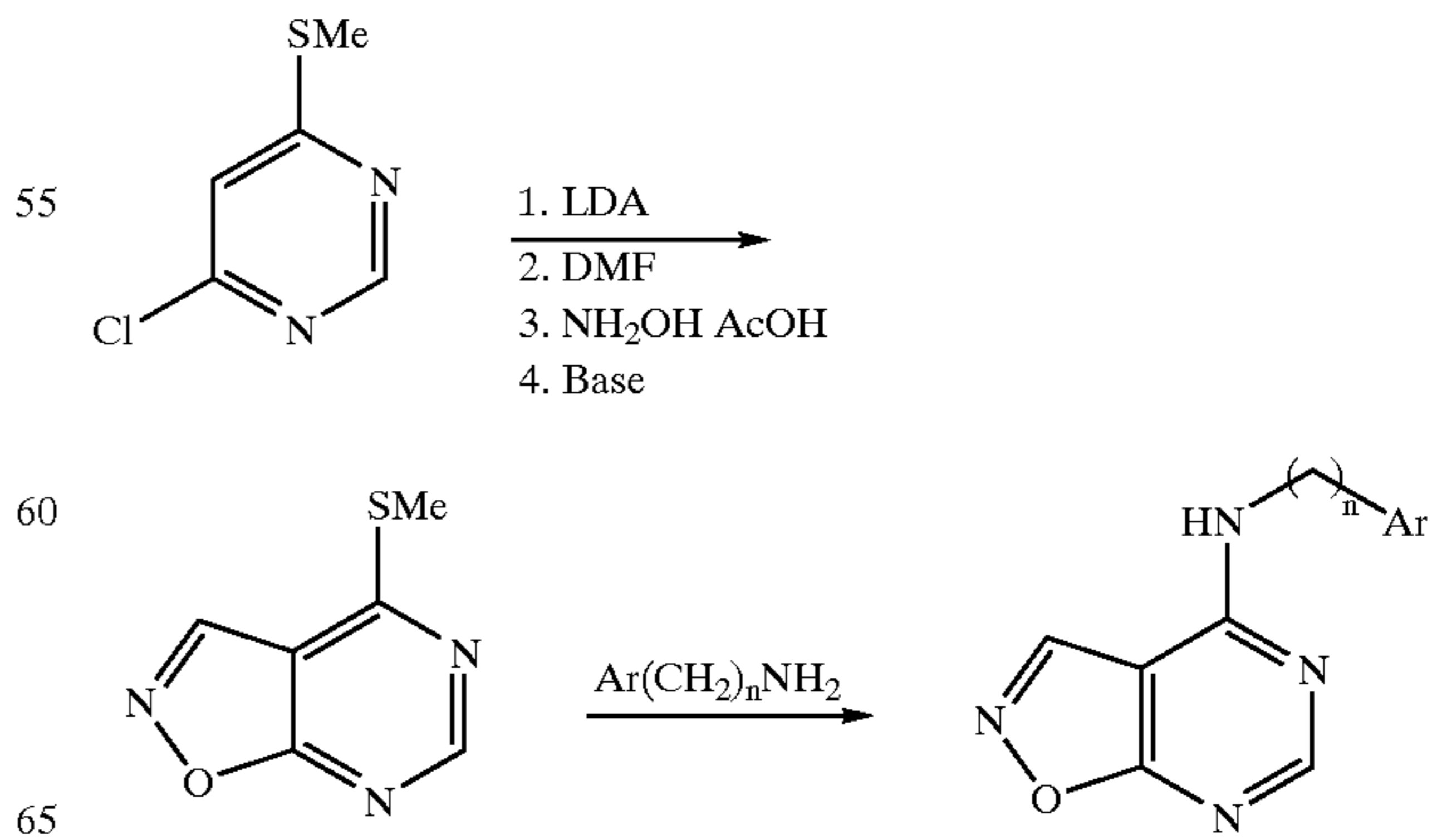
Scheme 28. Synthesis of Preferred Group 47: [5,4-d] ring fusion.
