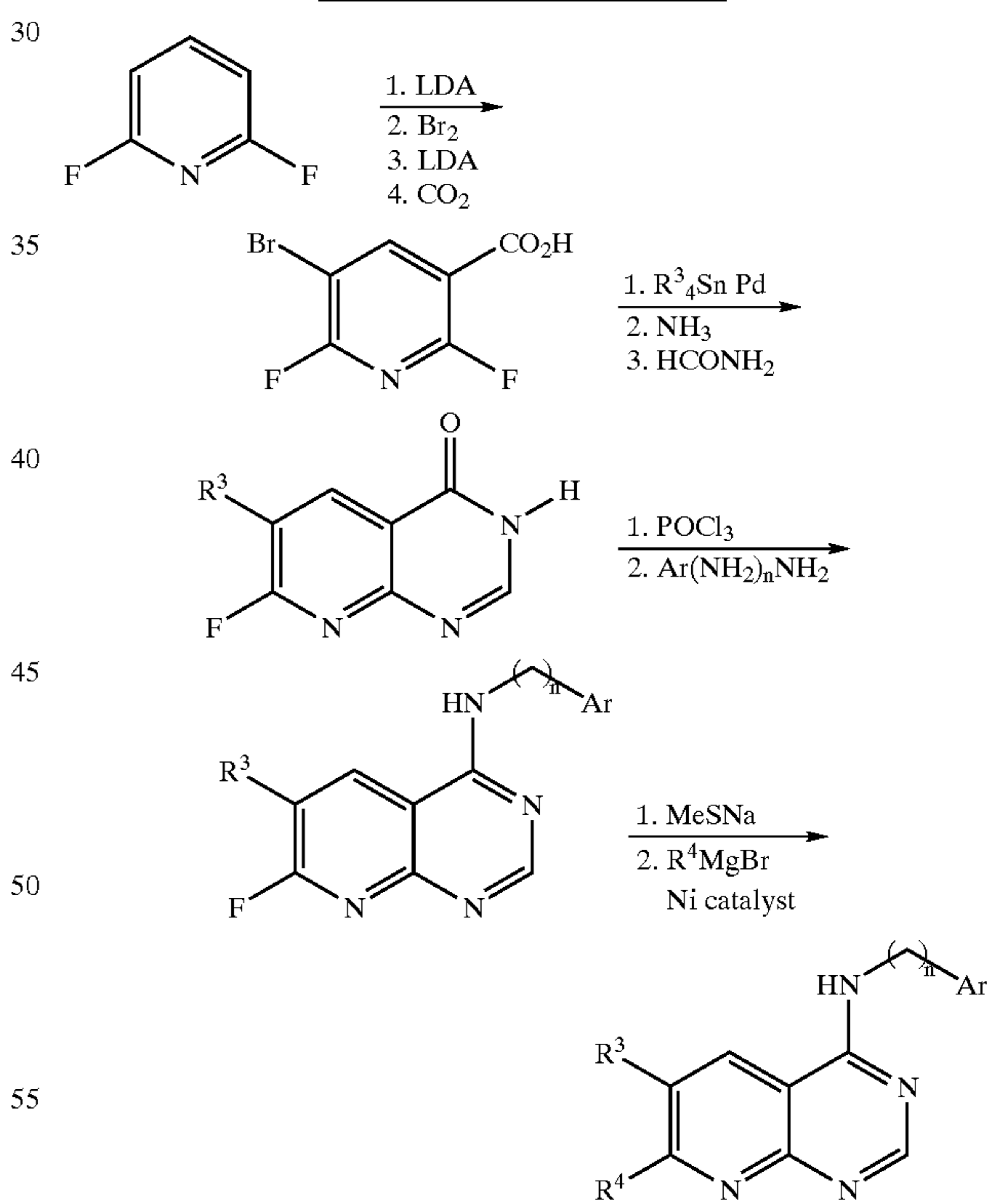
Scheme 12
