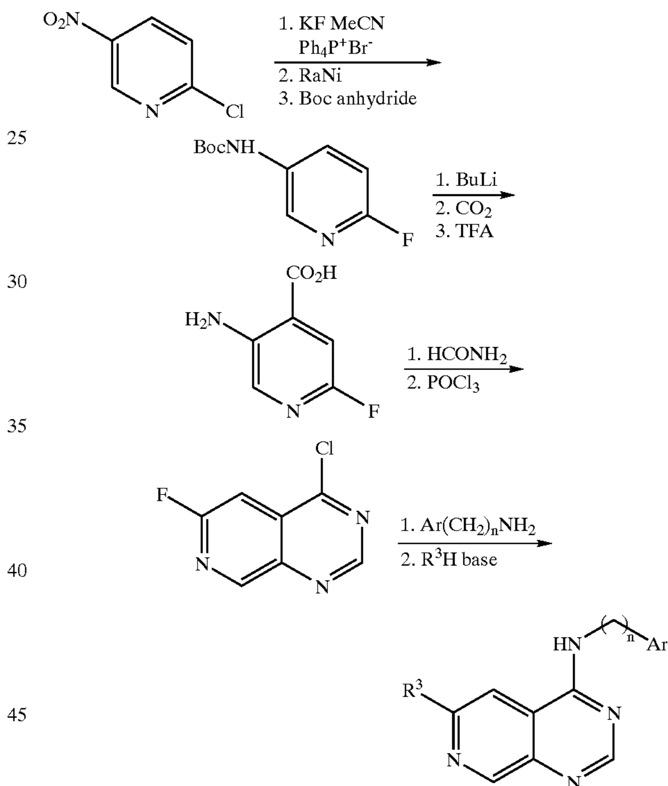
Scheme 8 Synthesis of Preferred Groups 17-21.
