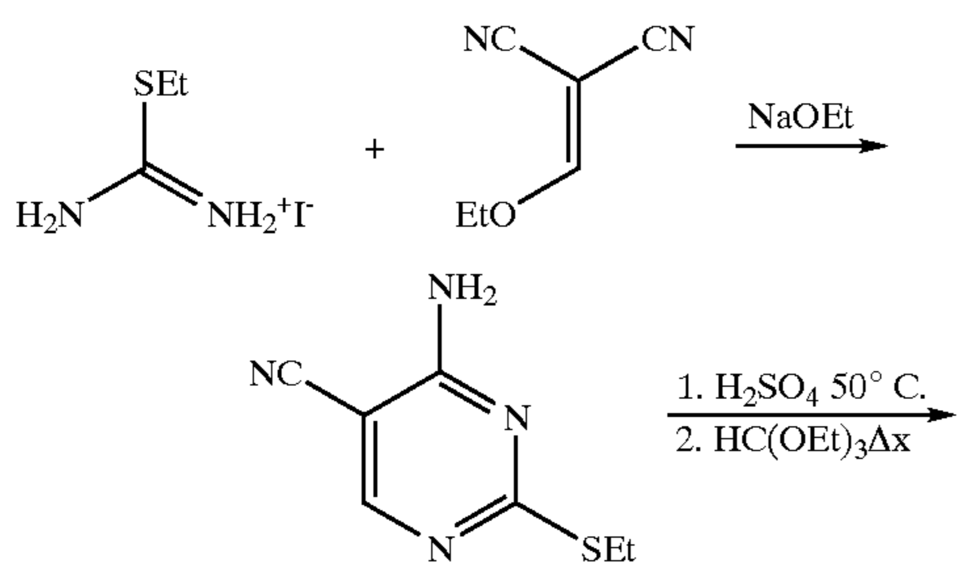
Scheme 15 Synthesis of Preferred Groups 33-36
