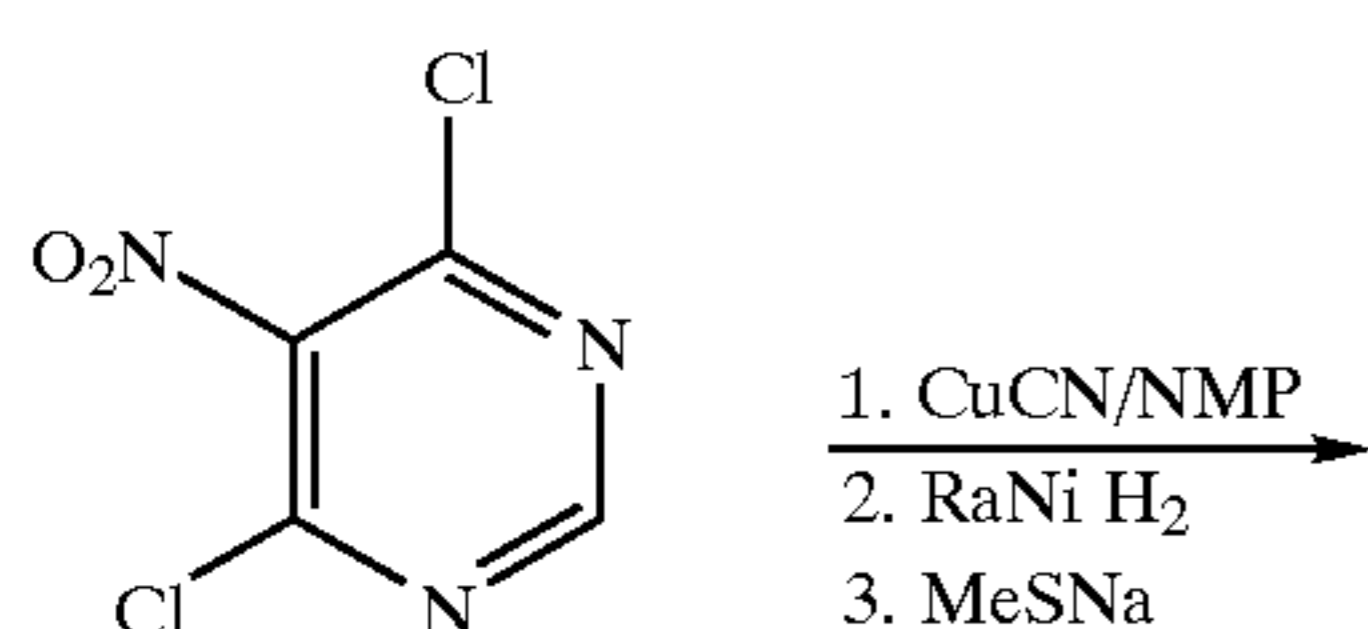
Scheme 31. Synthesis of Preferred Group 48: [4,5-d] ring fusion.
