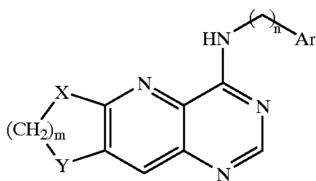
Scheme 6 Preferred Group 11.
