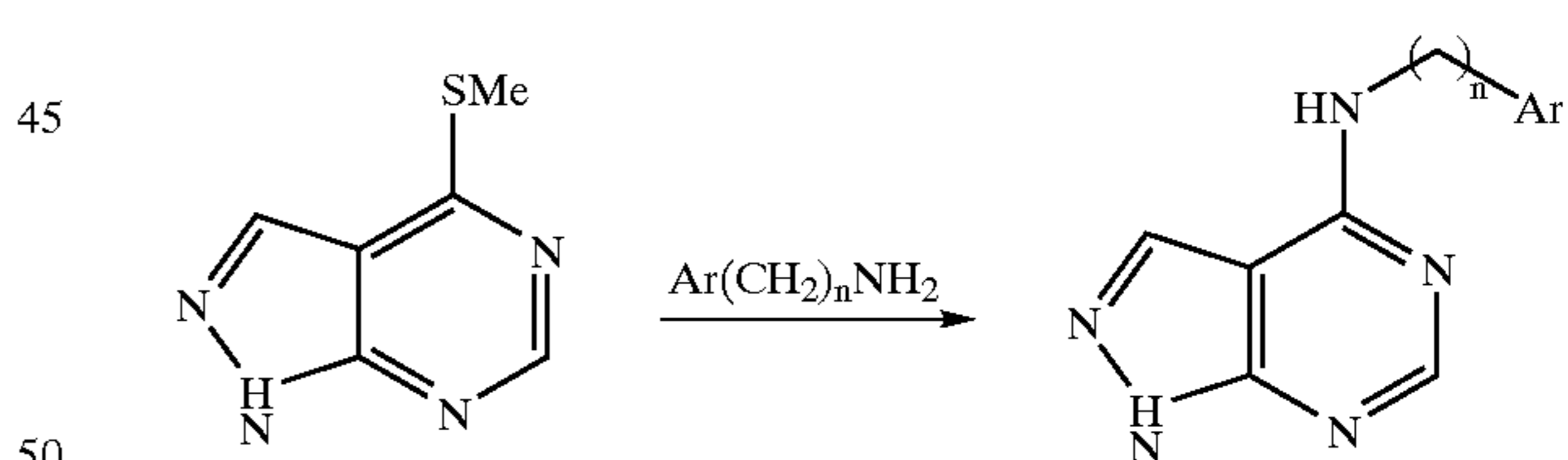
Scheme 33. Synthesis of Preferred Group 49: [4,3-d] ring fusion.
