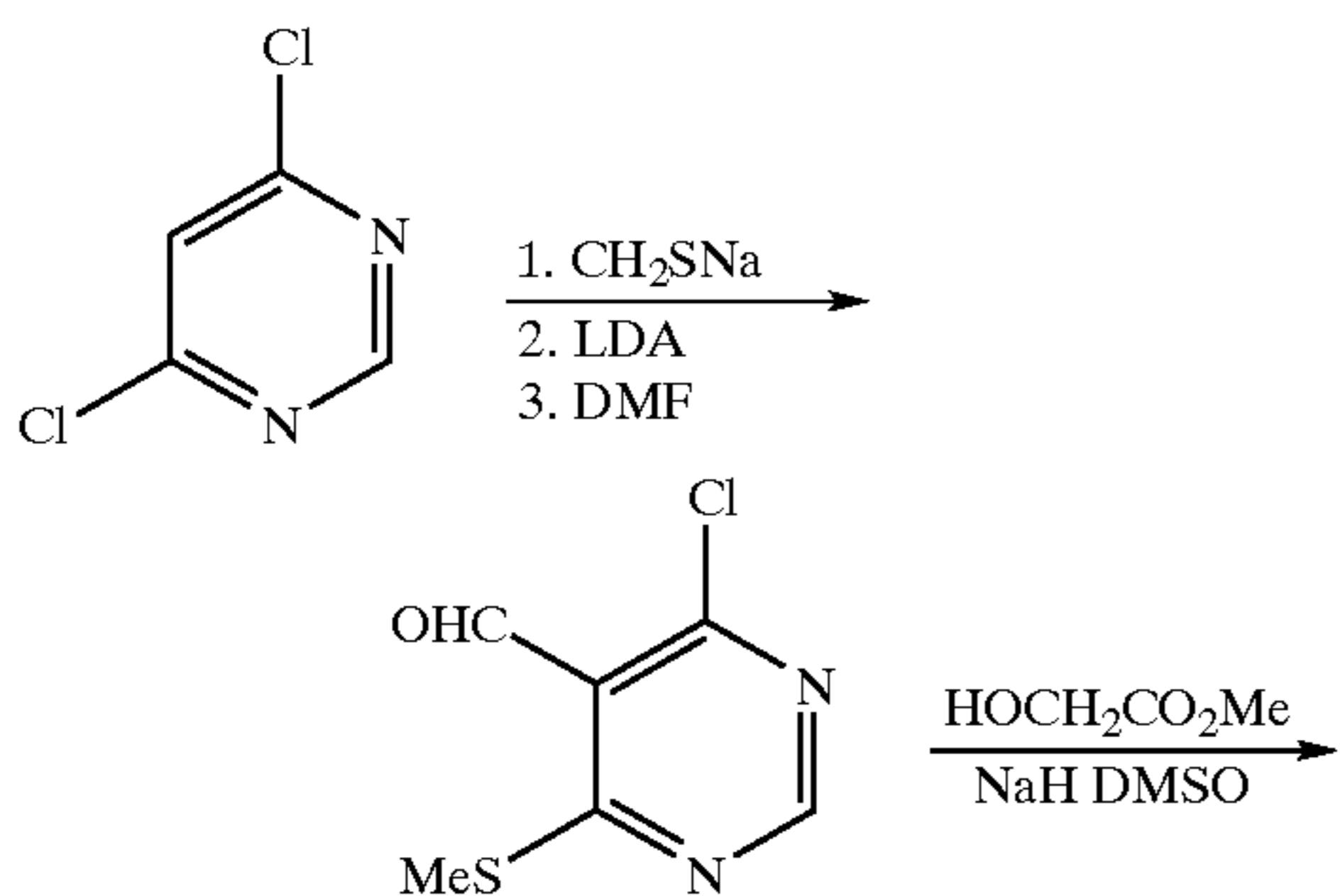
Scheme 20 Synthesis of Preferred Group 42; [2,3-d] ring fusion
