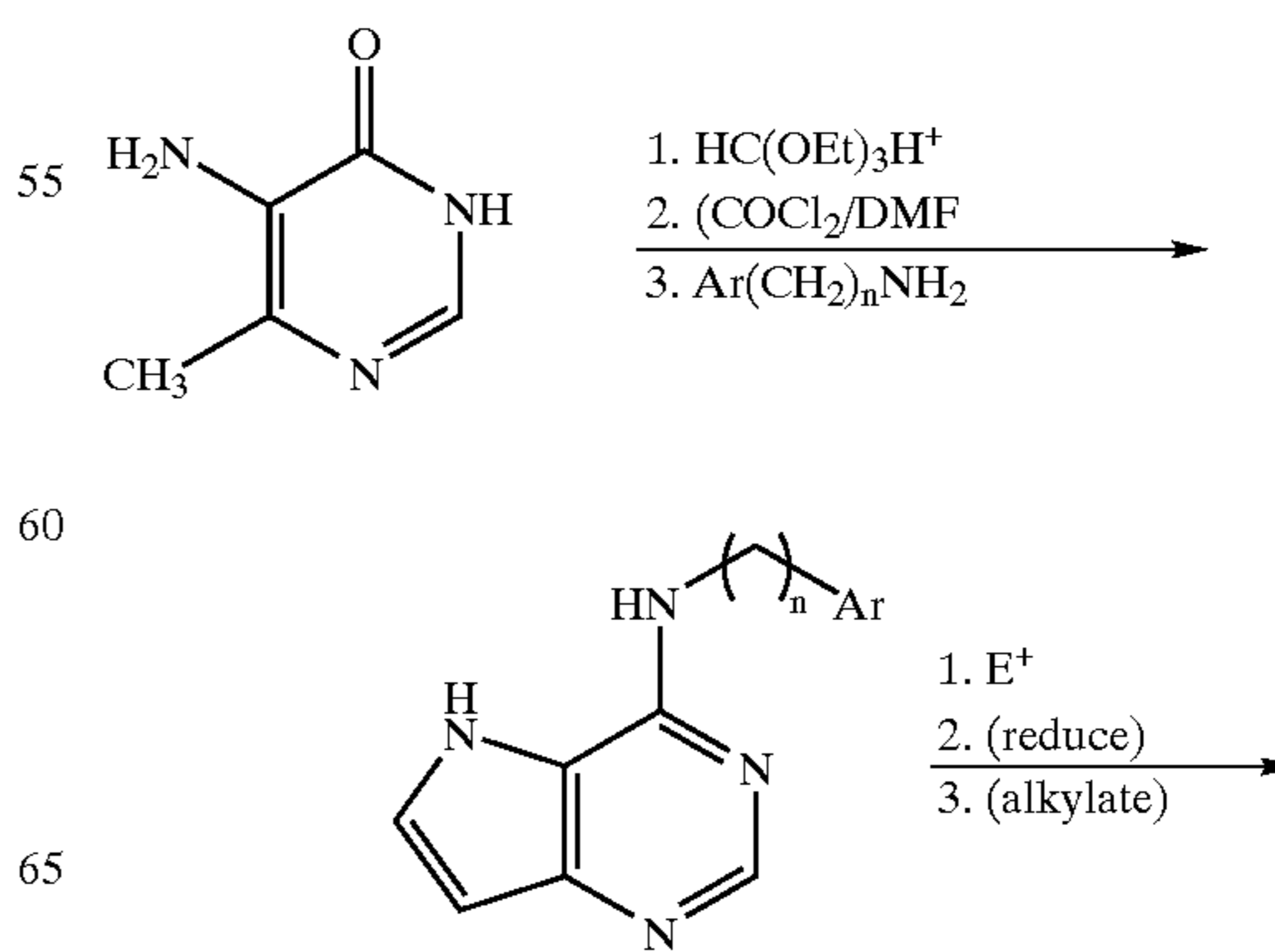
Scheme 22 Synthesis of Preferred Group 43; [3,2-d] ring fusion
