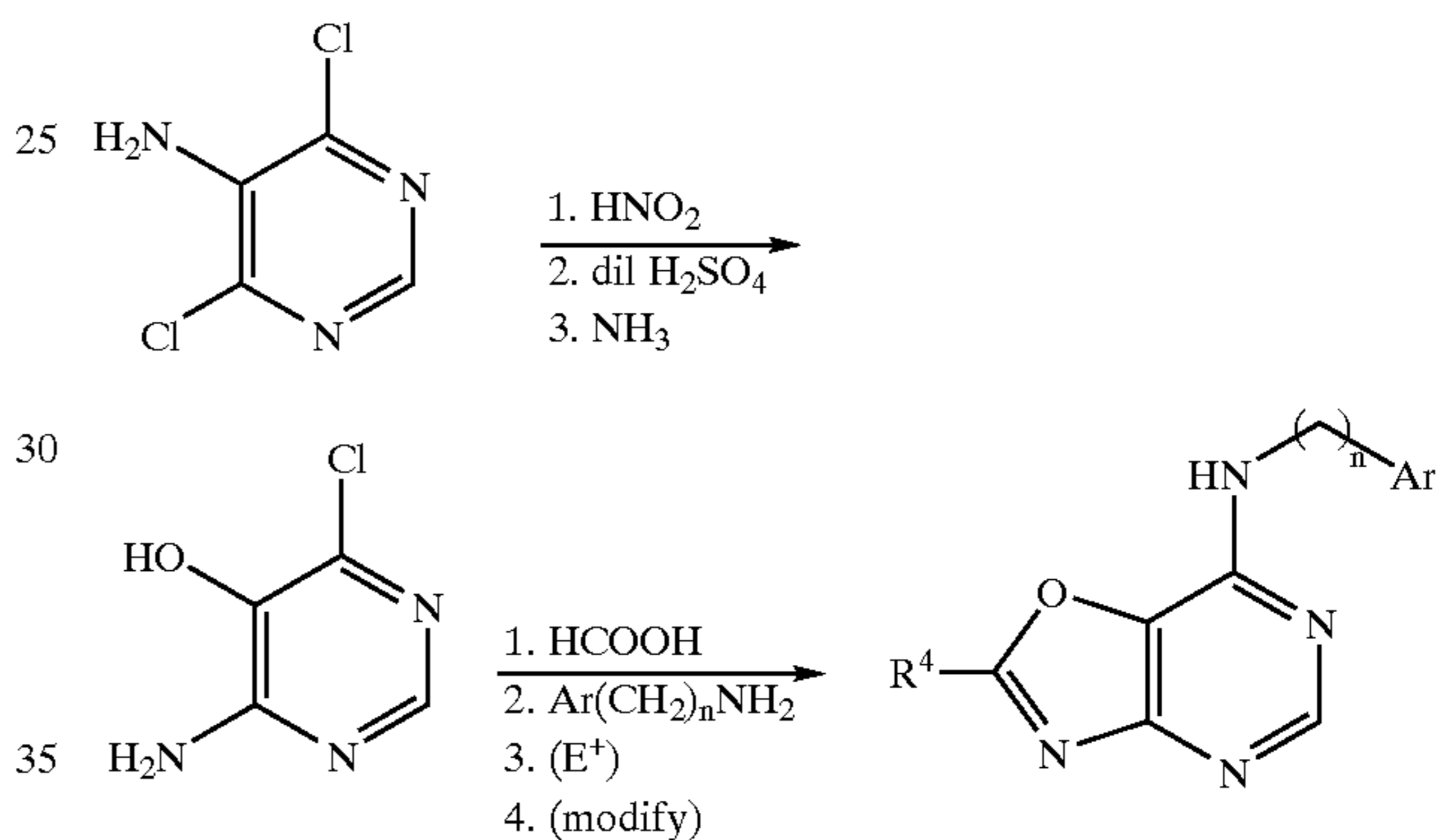
Scheme 26. Synthesis of Preferred Group 45: [4,5-d] ring fusion.
