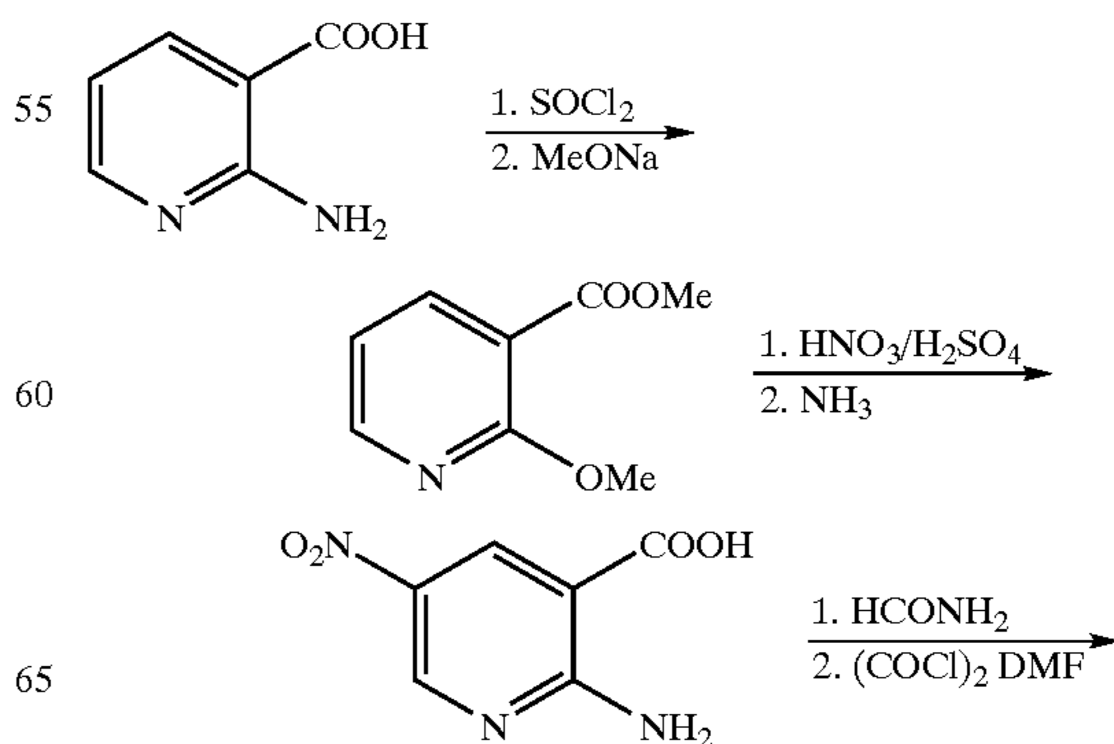
Scheme 9 Synthesis of Preferred Groups 22-26: R 4 = H.
