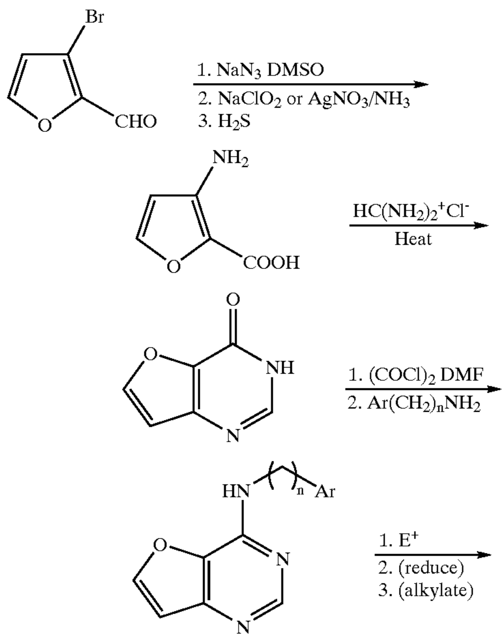
Scheme 19 Synthesis of Preferred Group 42; [3,2-d] ring fusion
