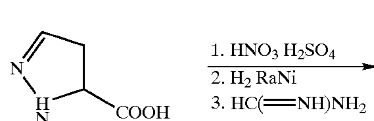
Scheme 33. Synthesis of Preferred Group 49: [4,3-d] ring fusion.
