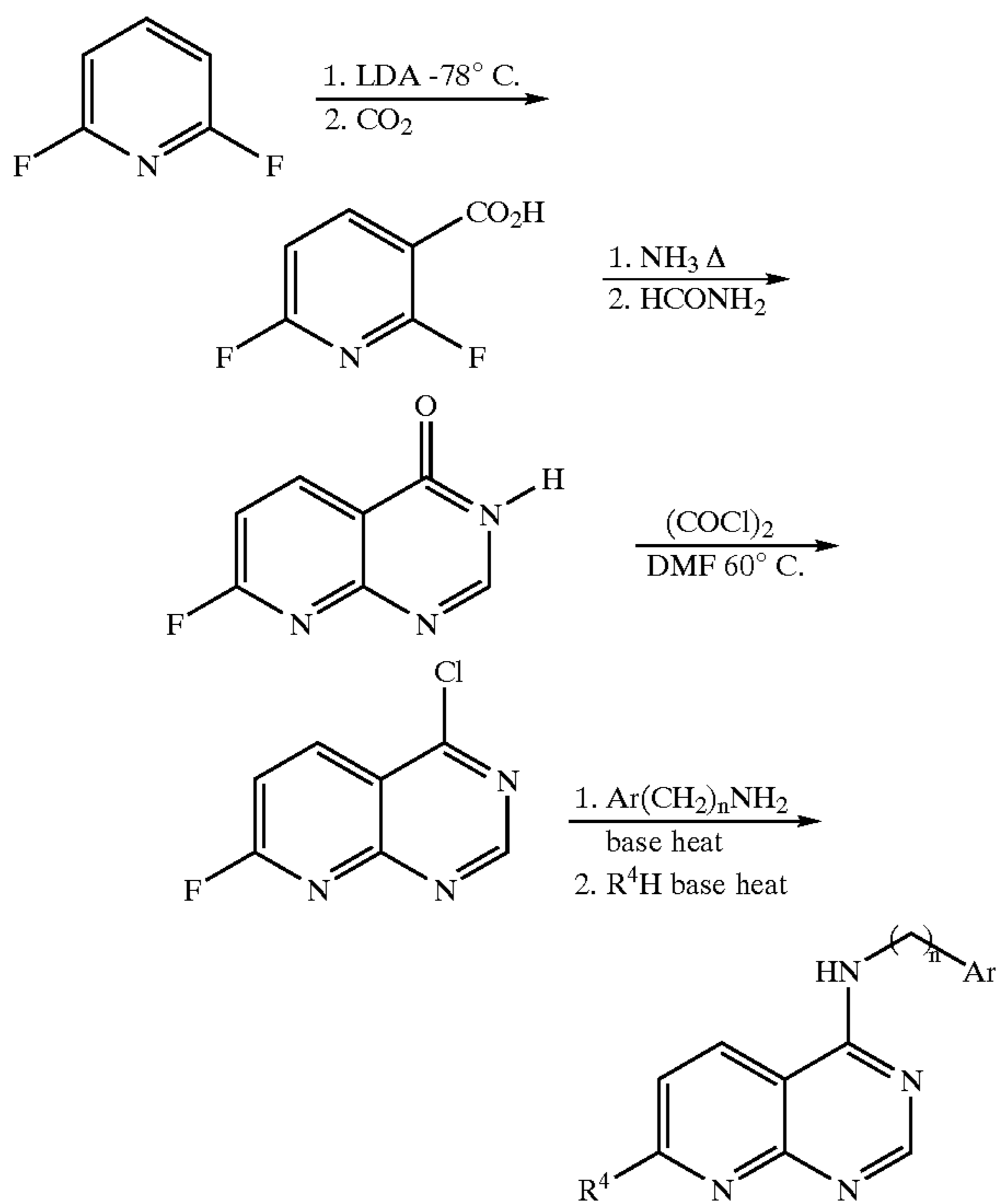
Scheme 10
