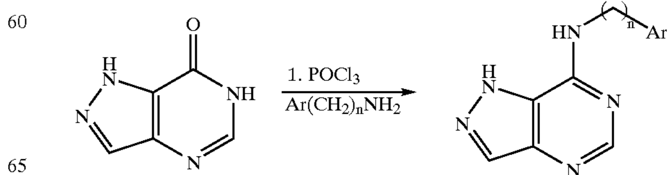
Scheme 31. Synthesis of Preferred Group 48: [4,5-d] ring fusion.
