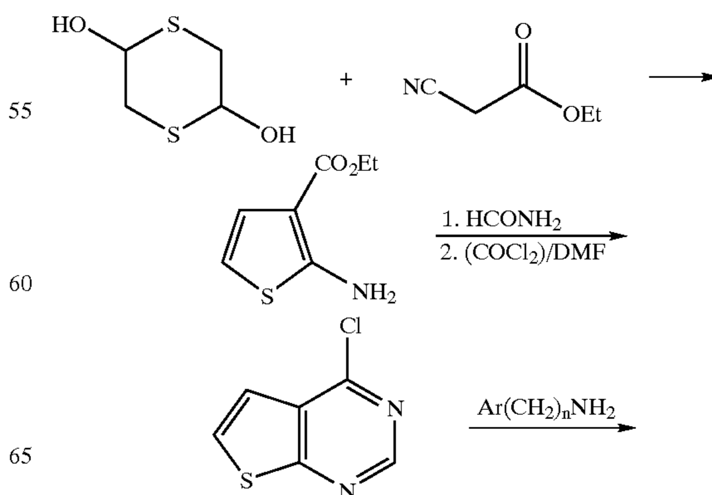
Scheme 18 Synthesis of Preferred Group 41; [2,3-d] ring fusion
