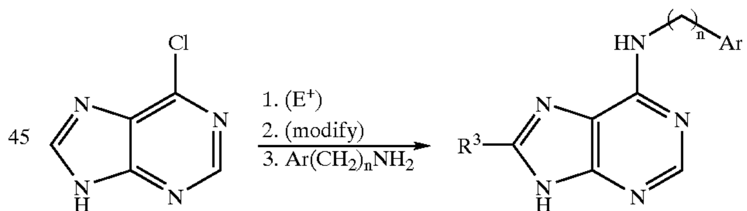
Scheme 27. Synthesis of Preferred Group 46.
