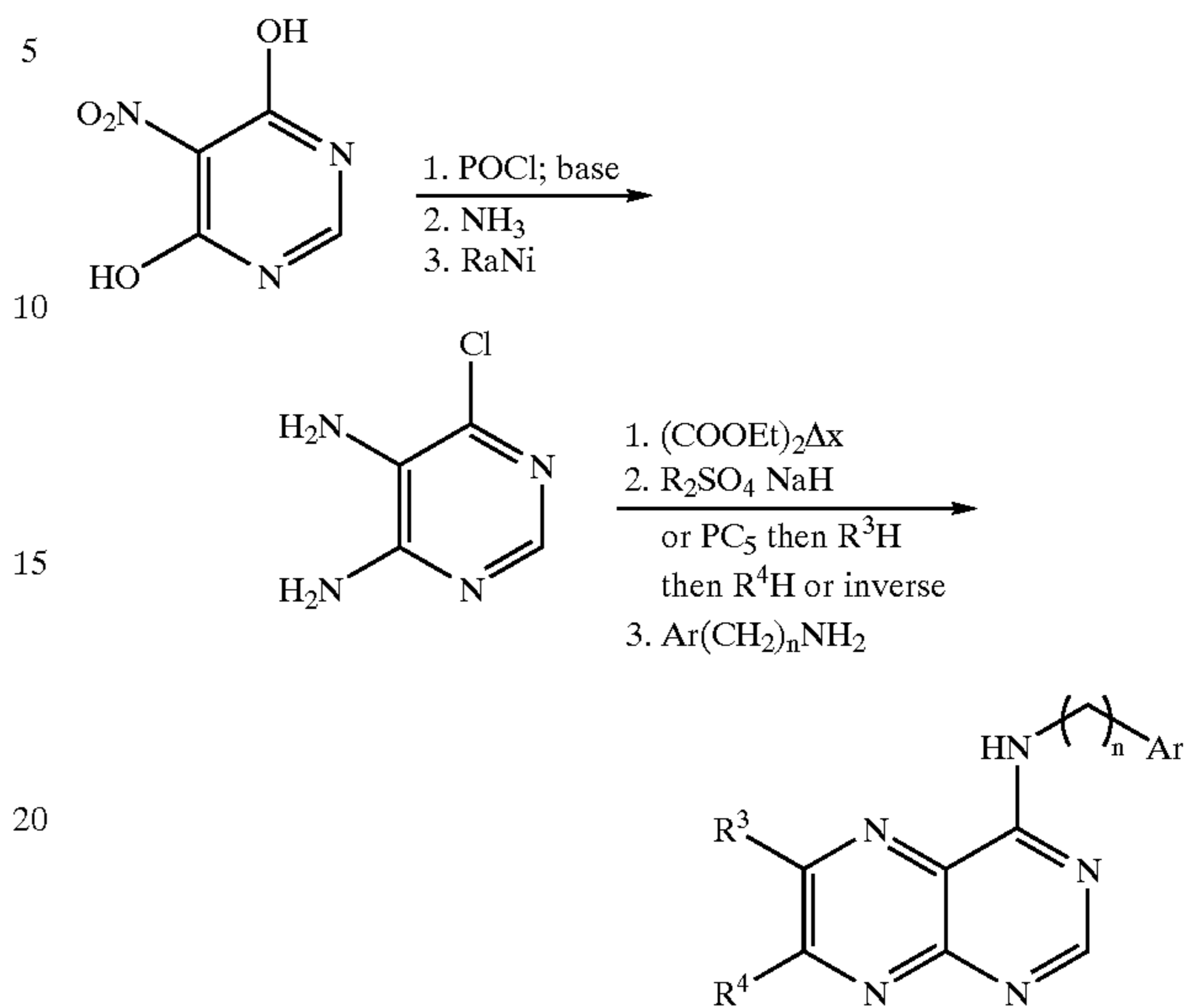
Scheme 16 Synthesis of Preferred Groups 37-40
