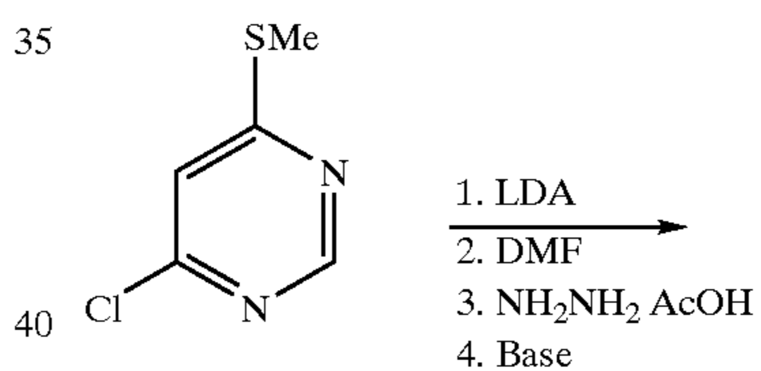
Scheme 32. Synthesis of Preferred Group 49: [3,4-d] ring fusion.
