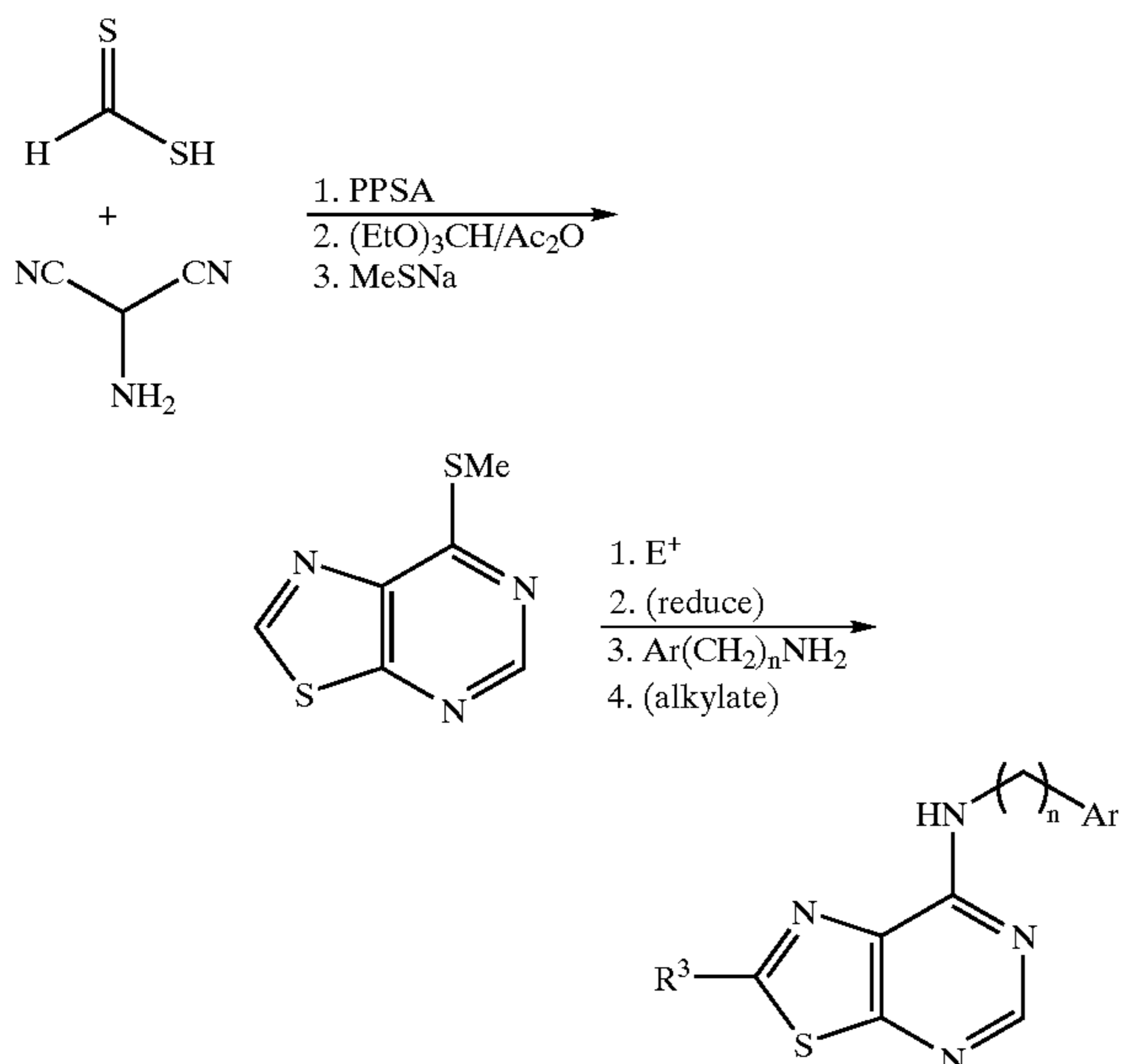
Scheme 23 Synthesis of Preferred Group 44; [5,4-d] ring fusion
