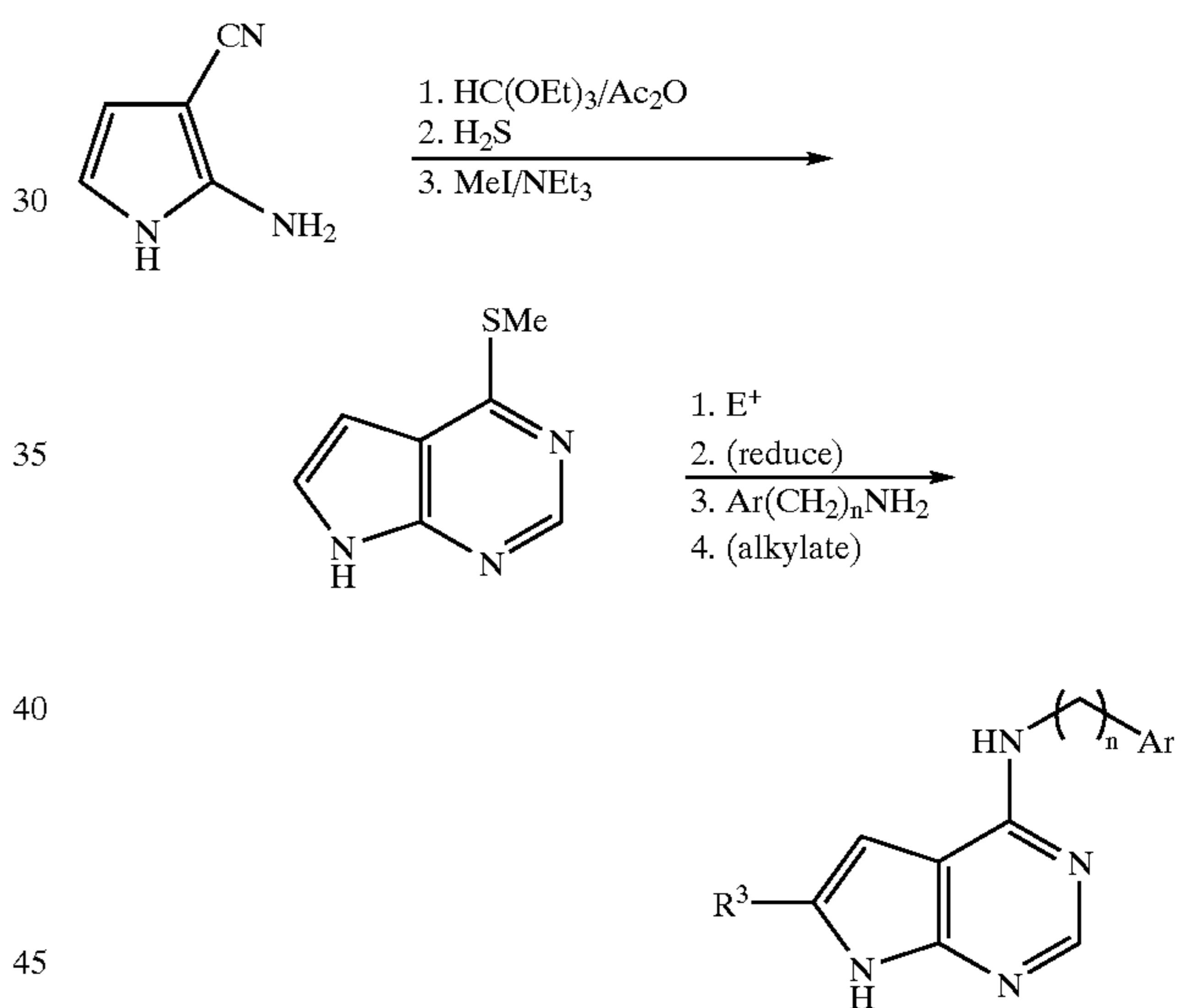
Scheme 21 Synthesis of Preferred Group 43; [2,3-d] ring fusion
