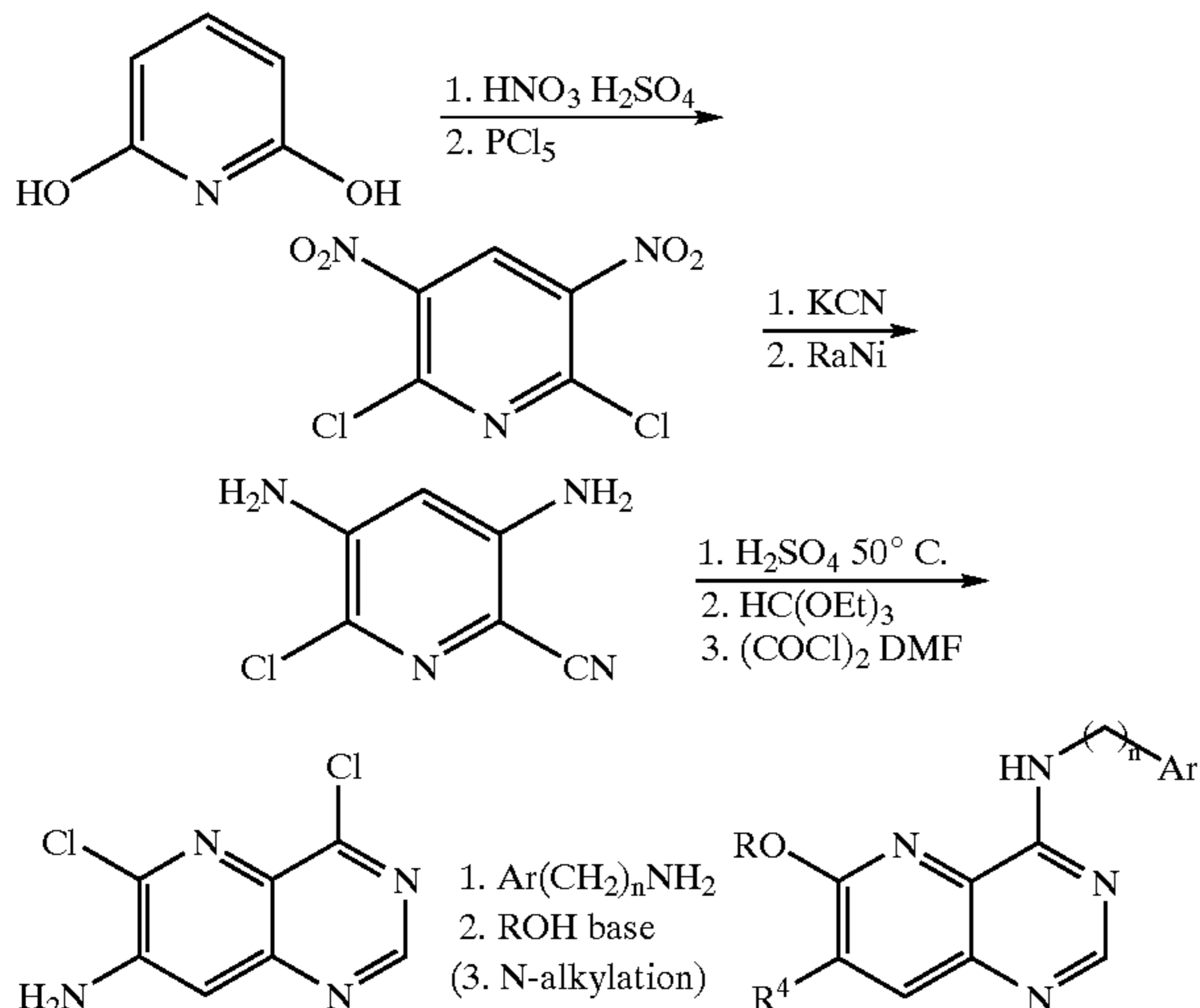
Scheme 5 Synthesis of Preferred Groups 8 & 9: R 3 = OR.
