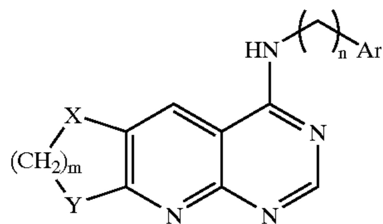
Scheme 14 Preferred Group 32
