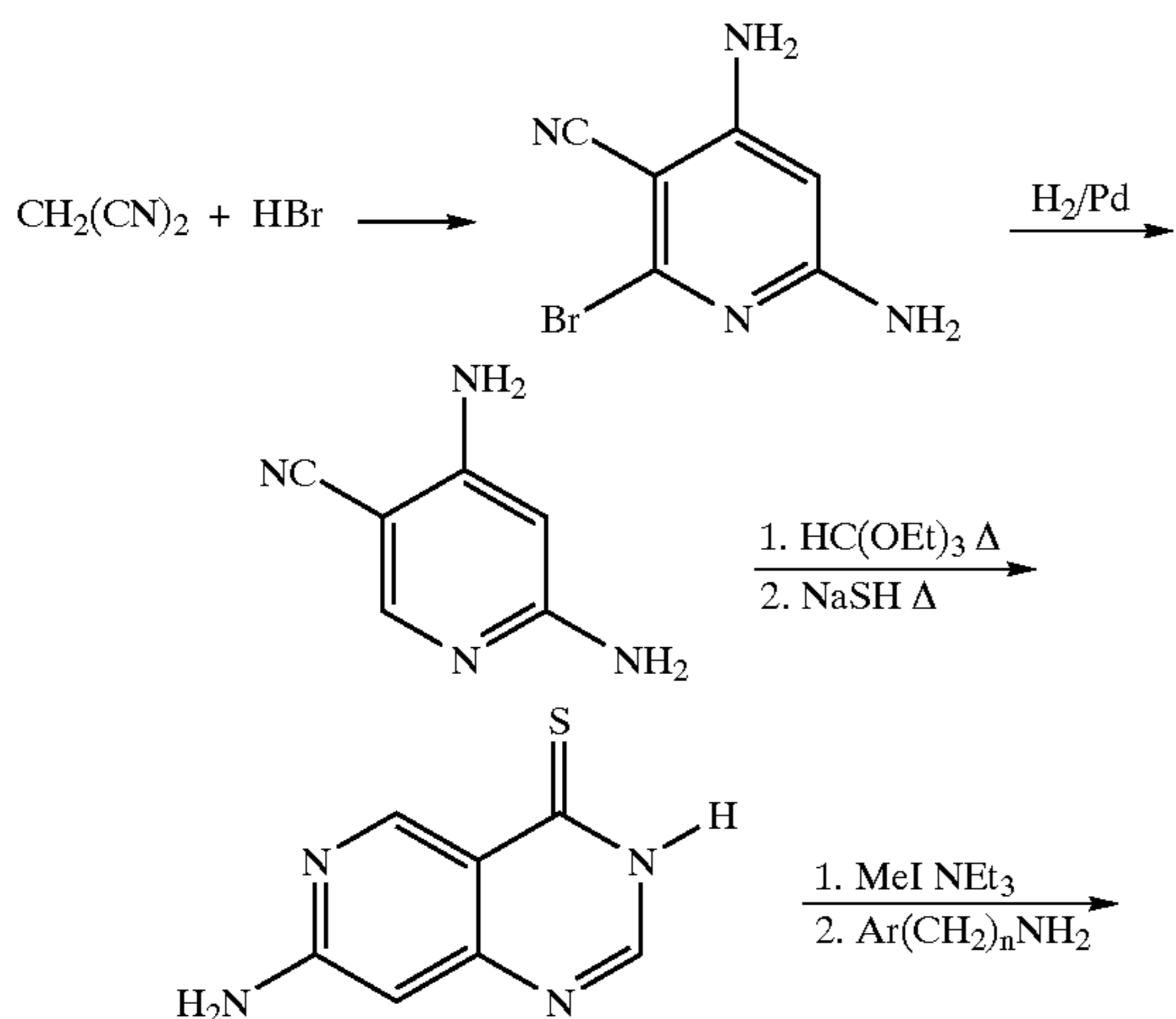
Scheme 7 Synthesis of Preferred Groups 12-16.
