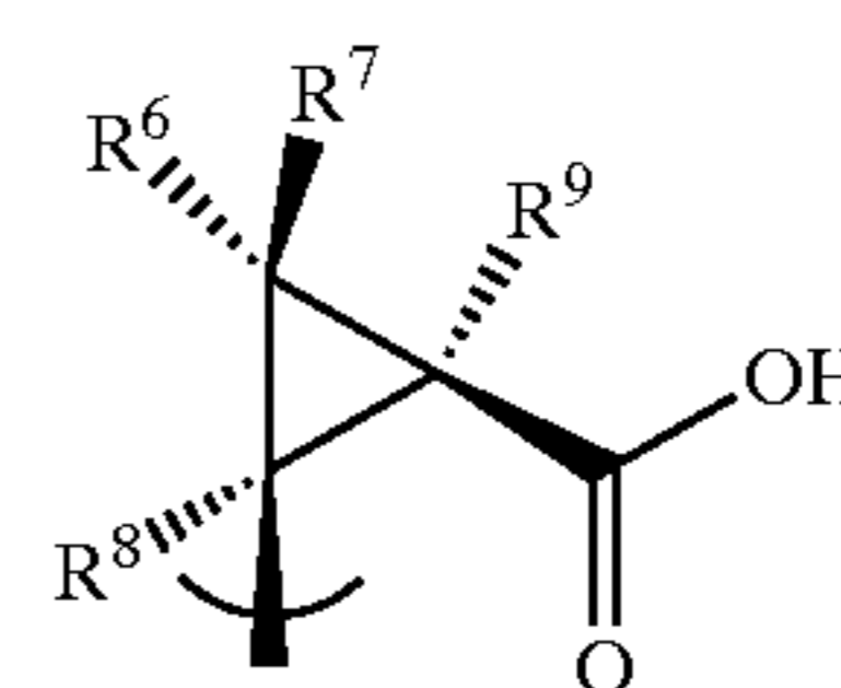
“cis-cyclopropanoic acid”
