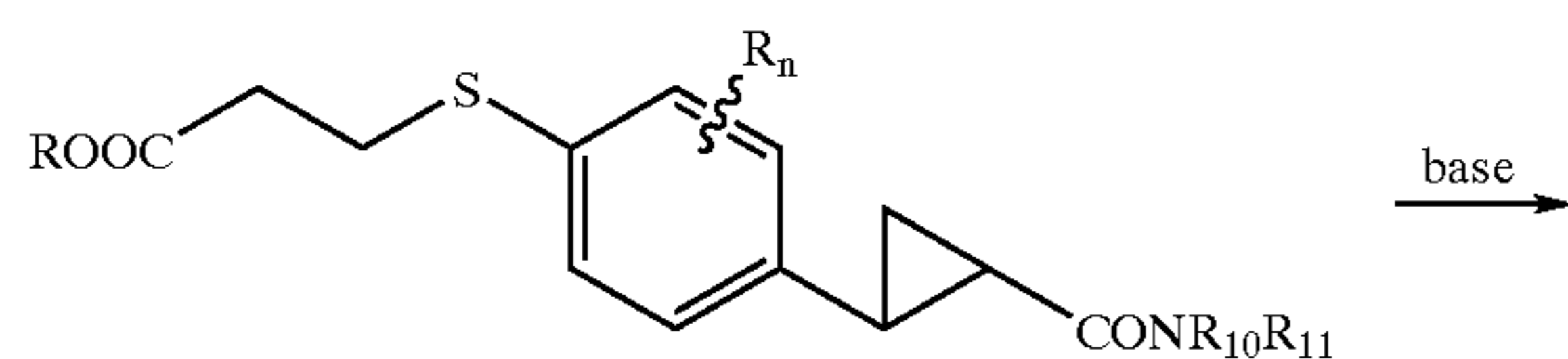
Scheme 5
