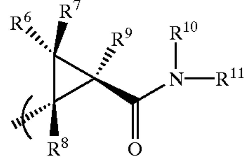
"trans-cyclopropanamide";
