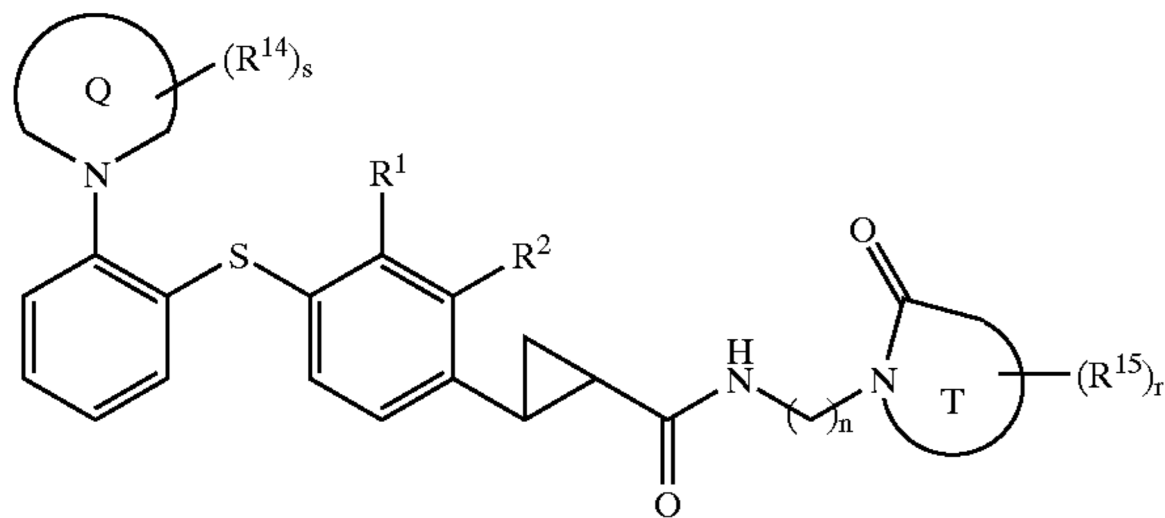
Formula III
