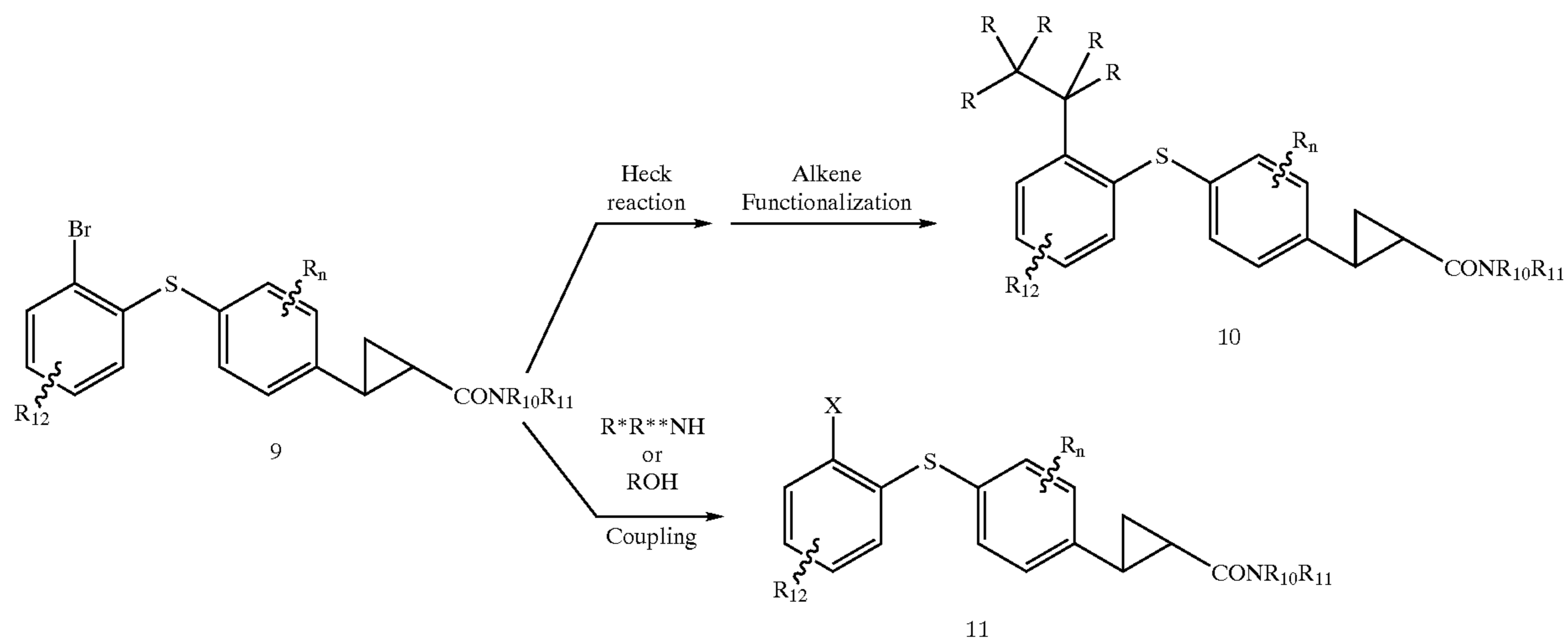
Scheme 3
