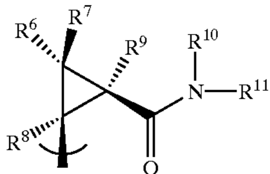
"cis-cyclopropanamide"
