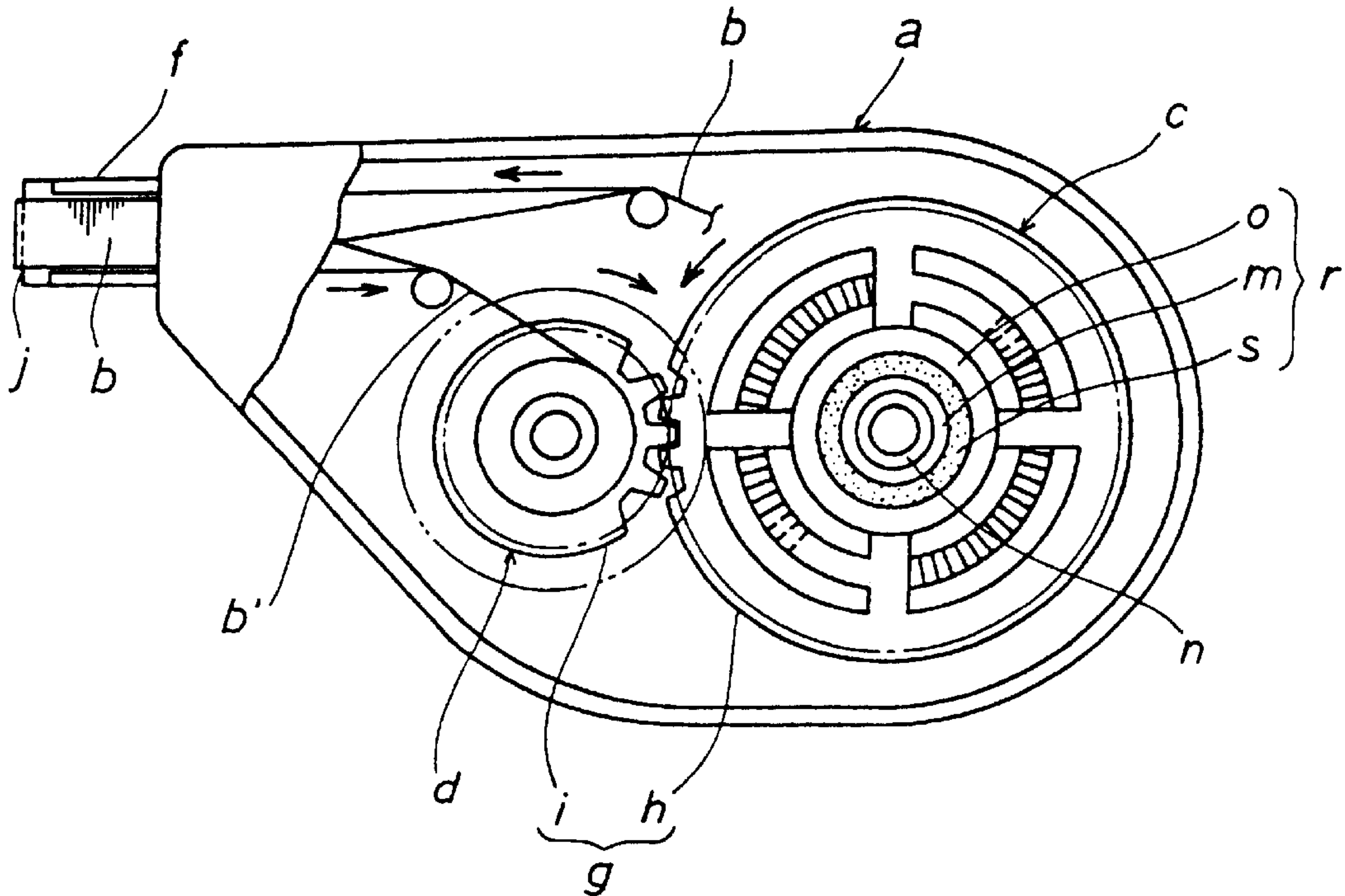
FIG.22(a) PRIOR ART
