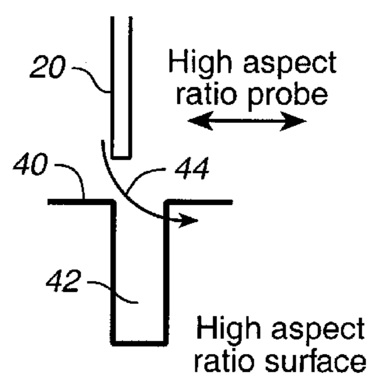
FIG. 1C (PRIOR ART)
