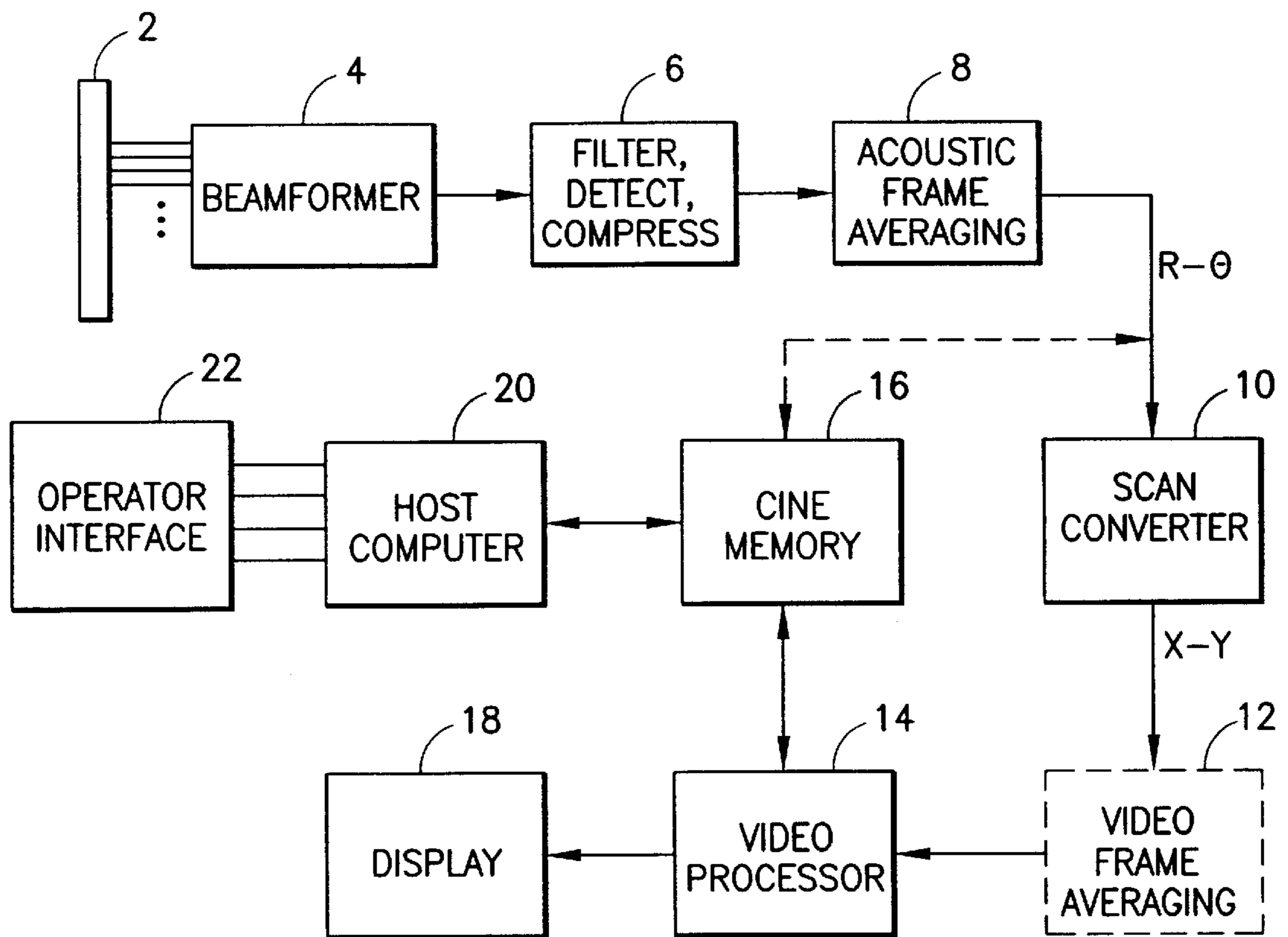
FIG. 1 PRIOR ART
