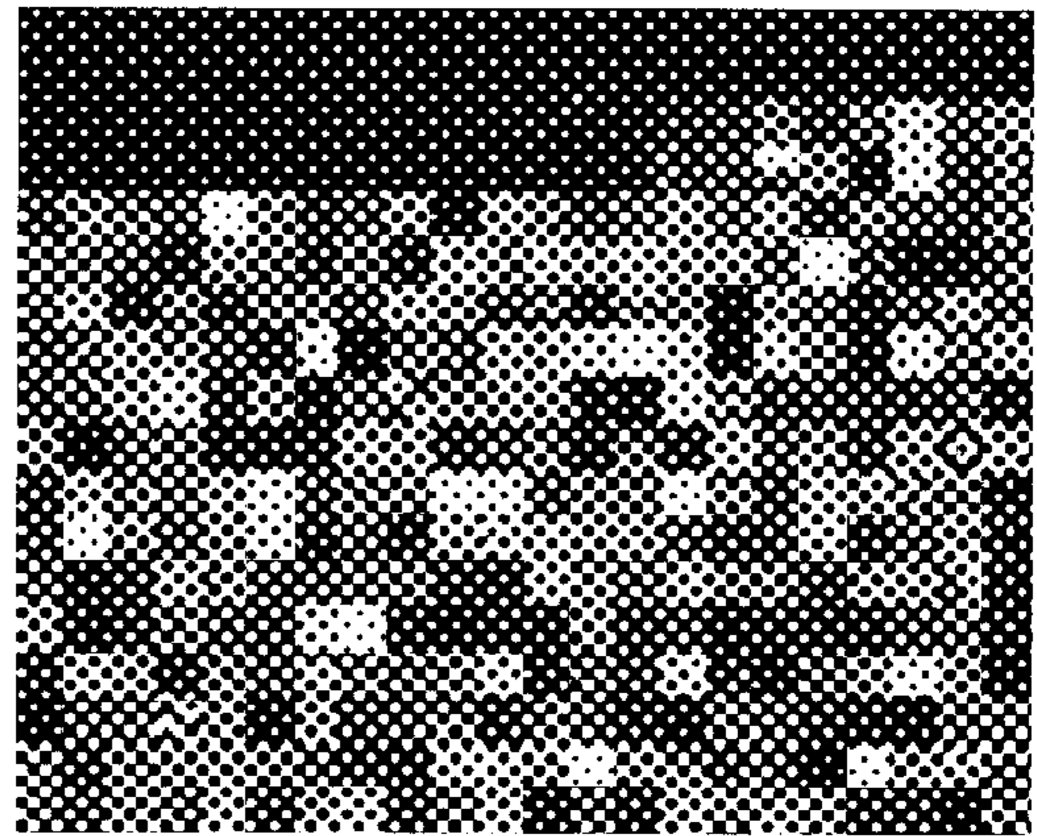
Without Segmentation
