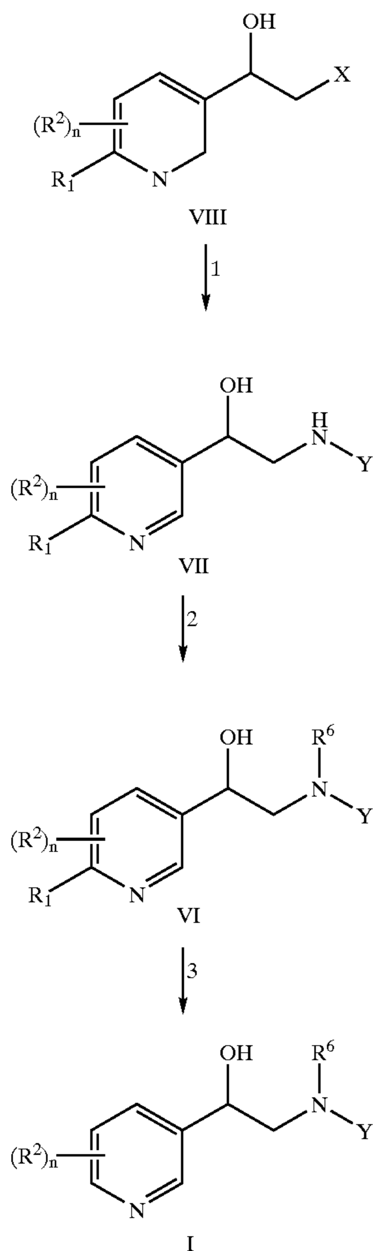
Scheme 2
