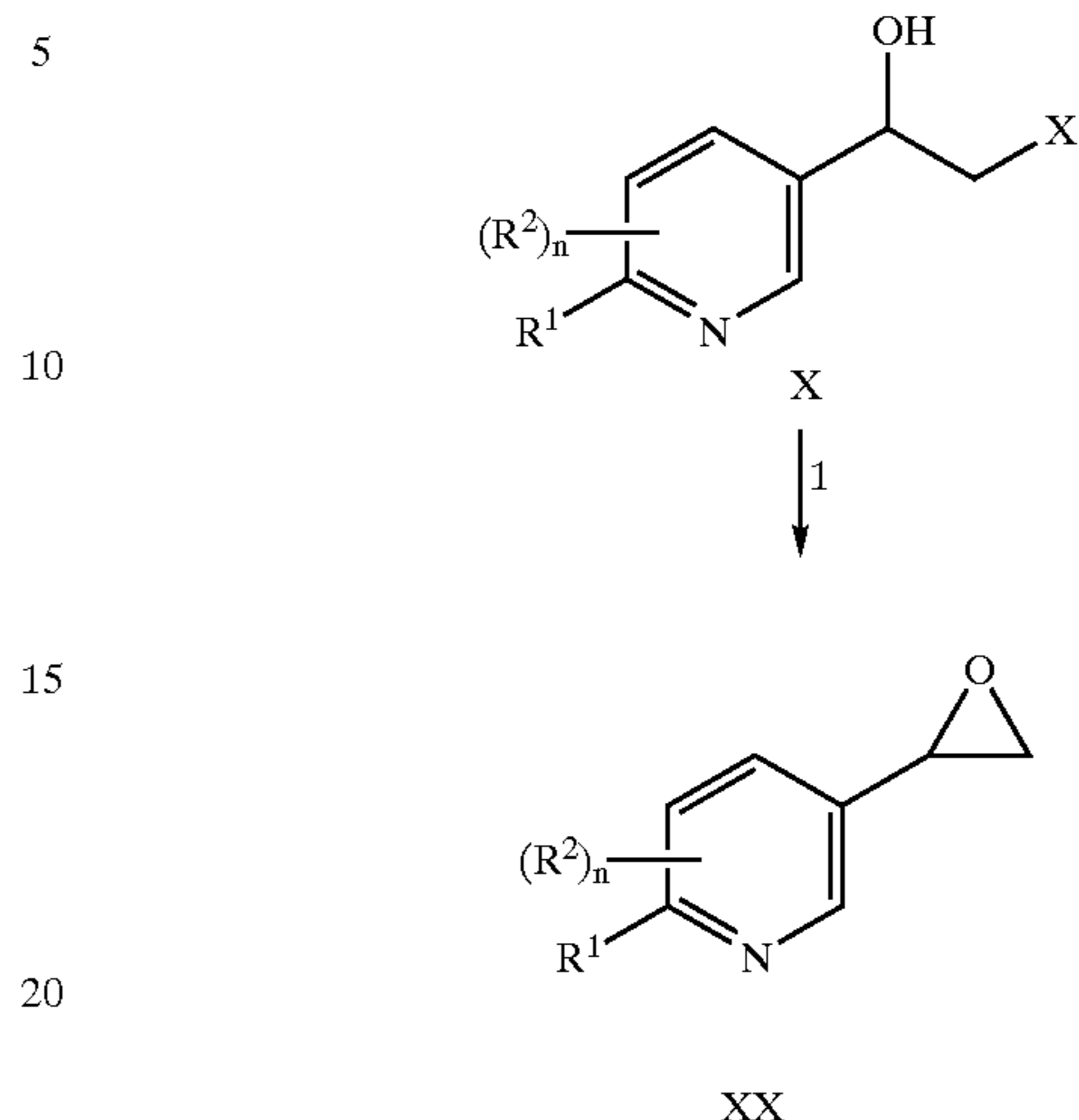
Scheme 3
