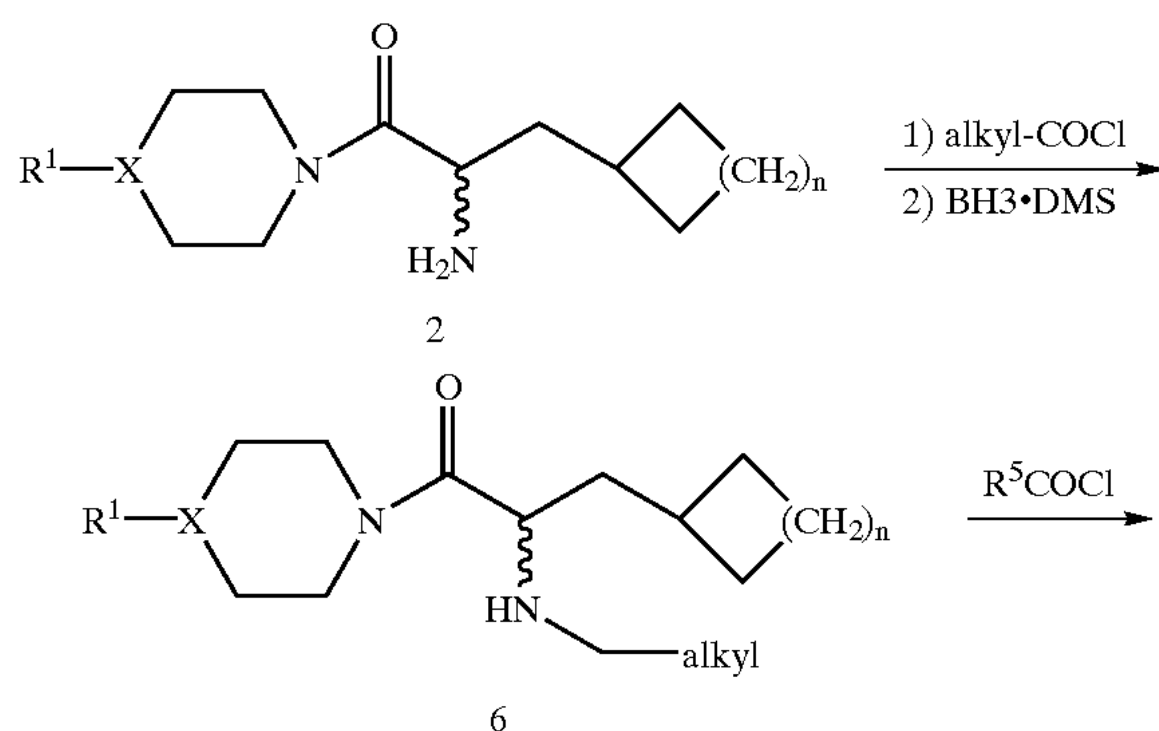
Scheme 3
