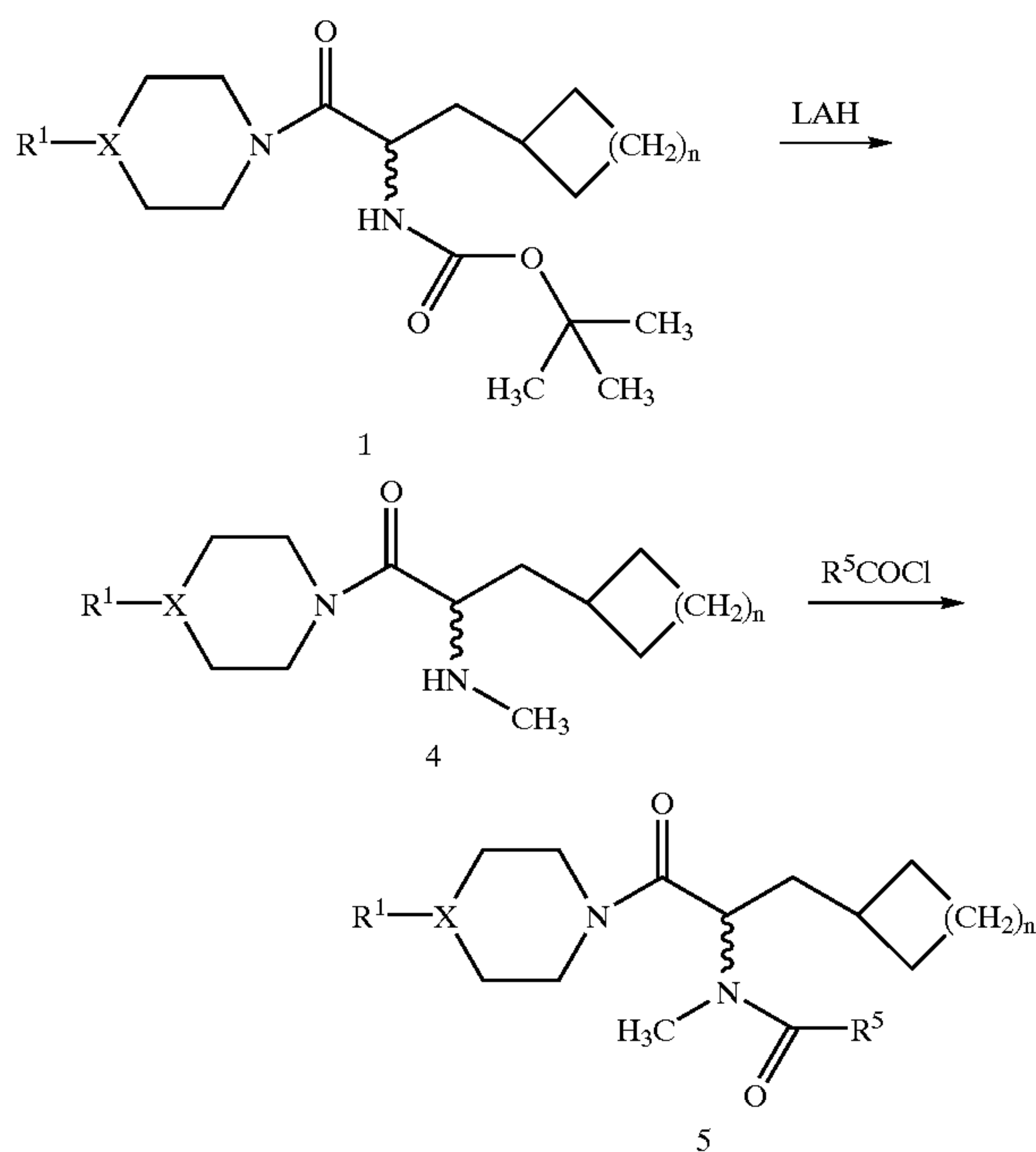
Scheme 2
