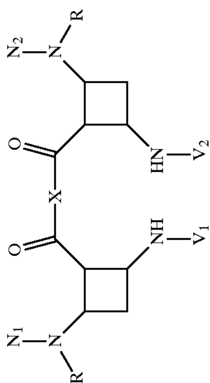
C-C COMPOUNDS
