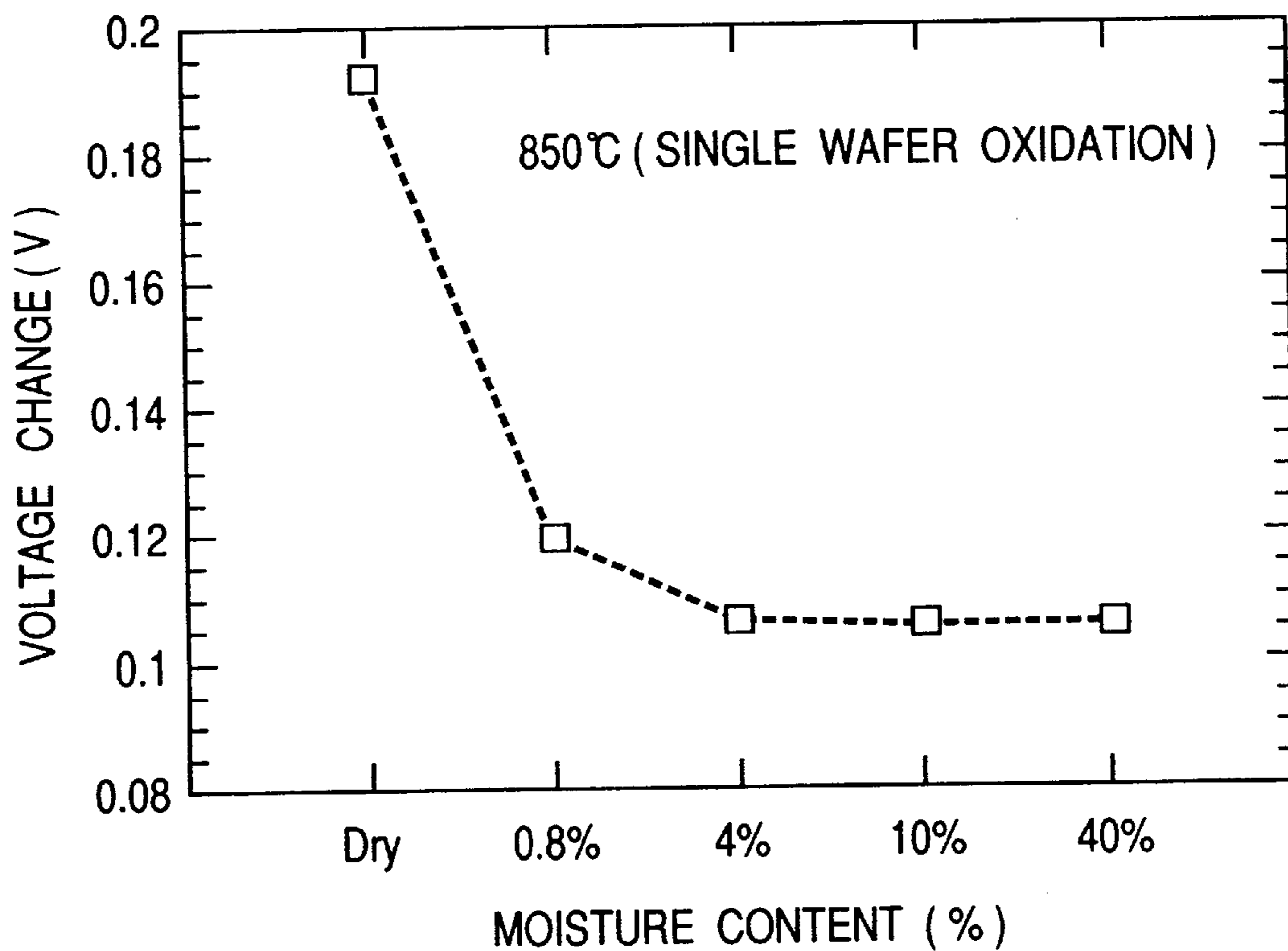
OXIDATION CONDITION DEPENDENCY OF VOLTAGE CHANGE
