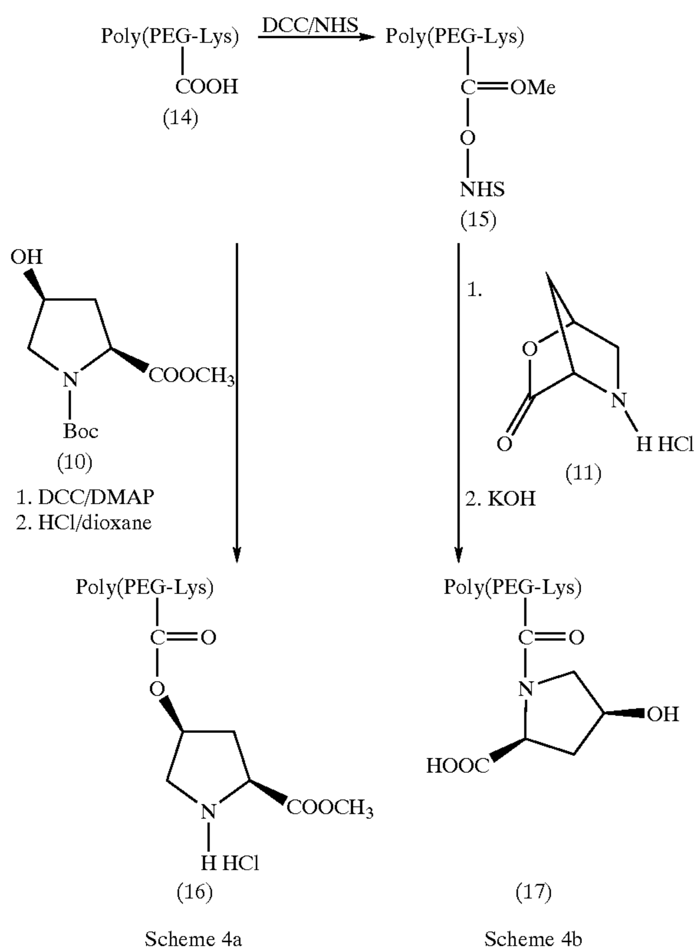
Scheme 4 Preparation of poly(PEG-Lys)-cis-Hyp copolymers
