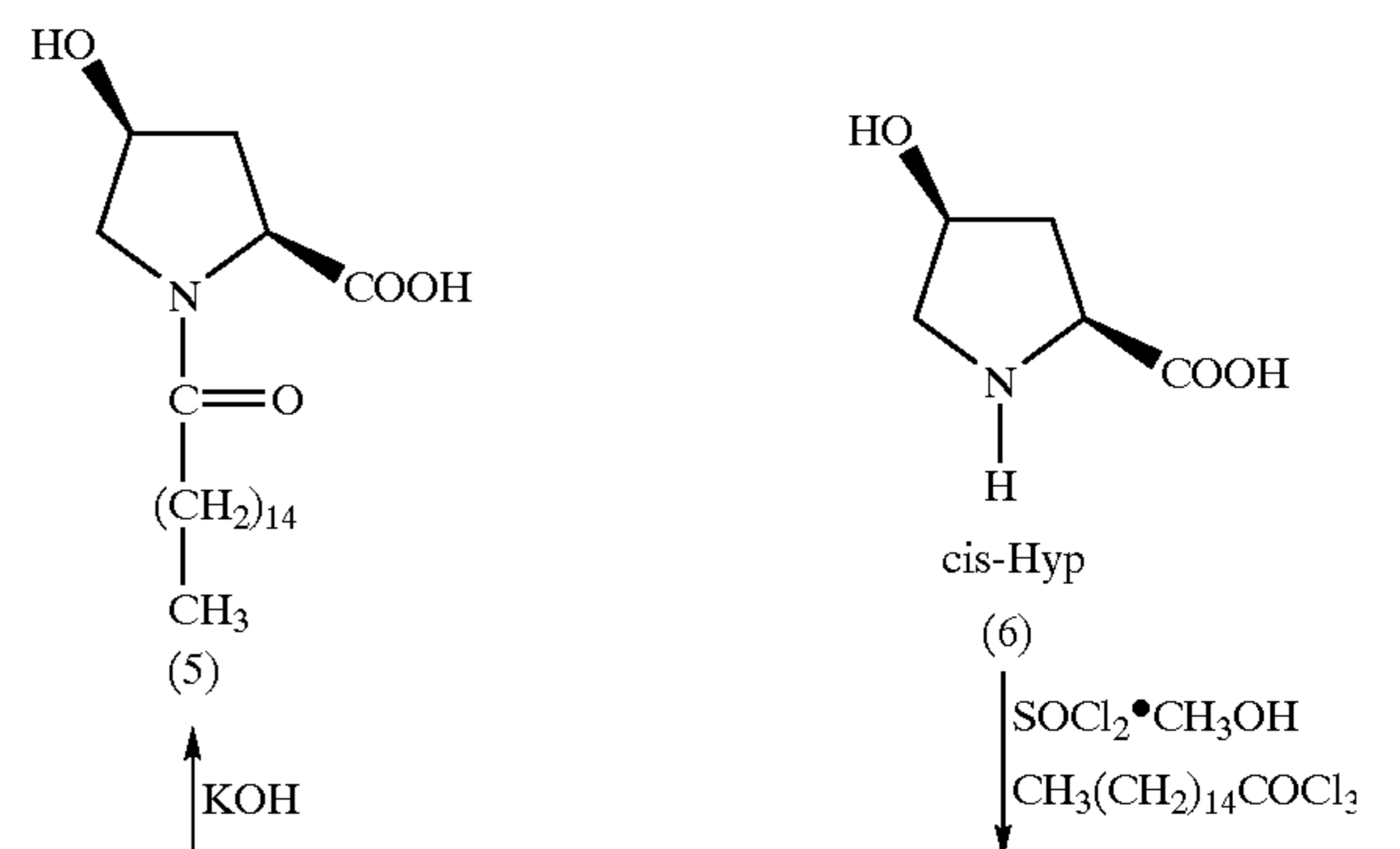
Scheme 2 Preparation of poly (cis-N-Pal-Hyp ester)
