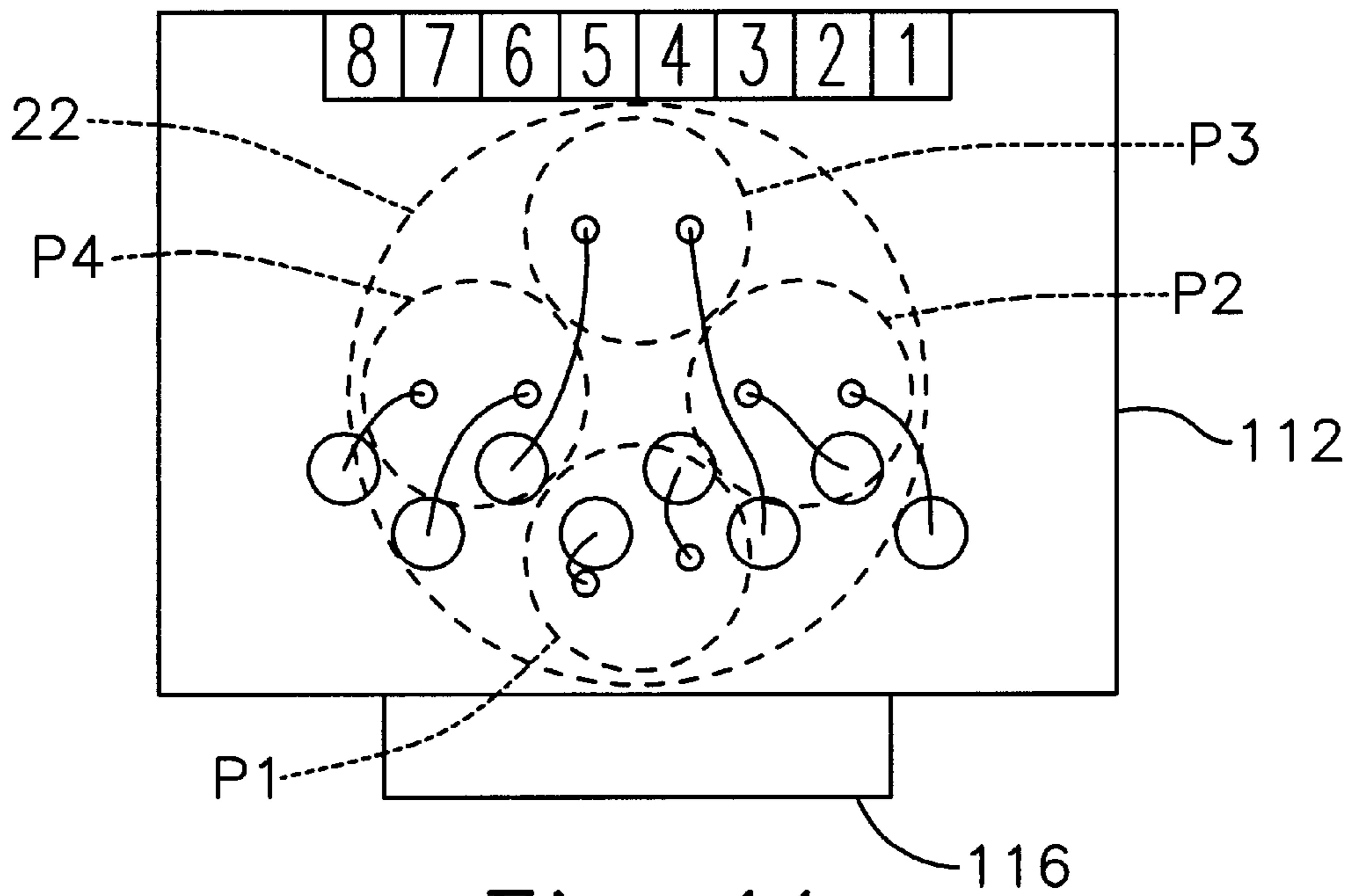
Fig. 11 Prior Art
