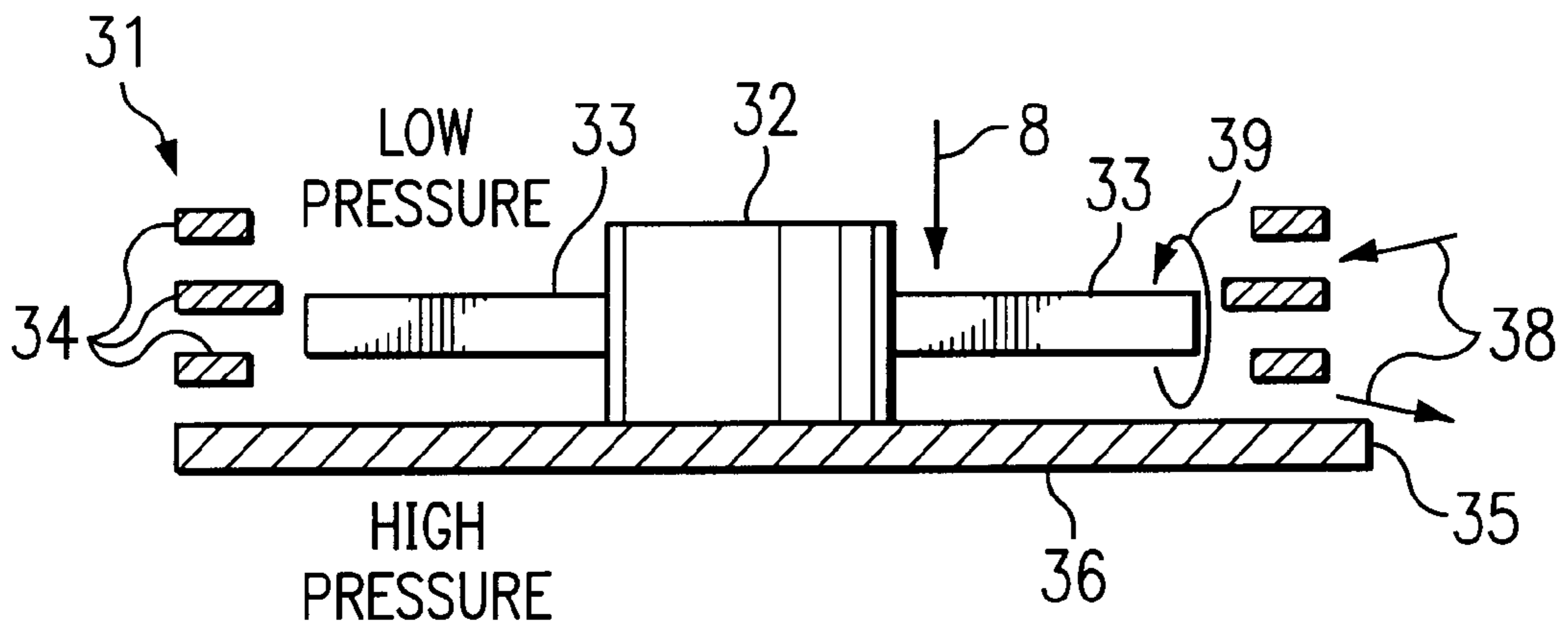
FIG. 3 (PRIOR ART)
