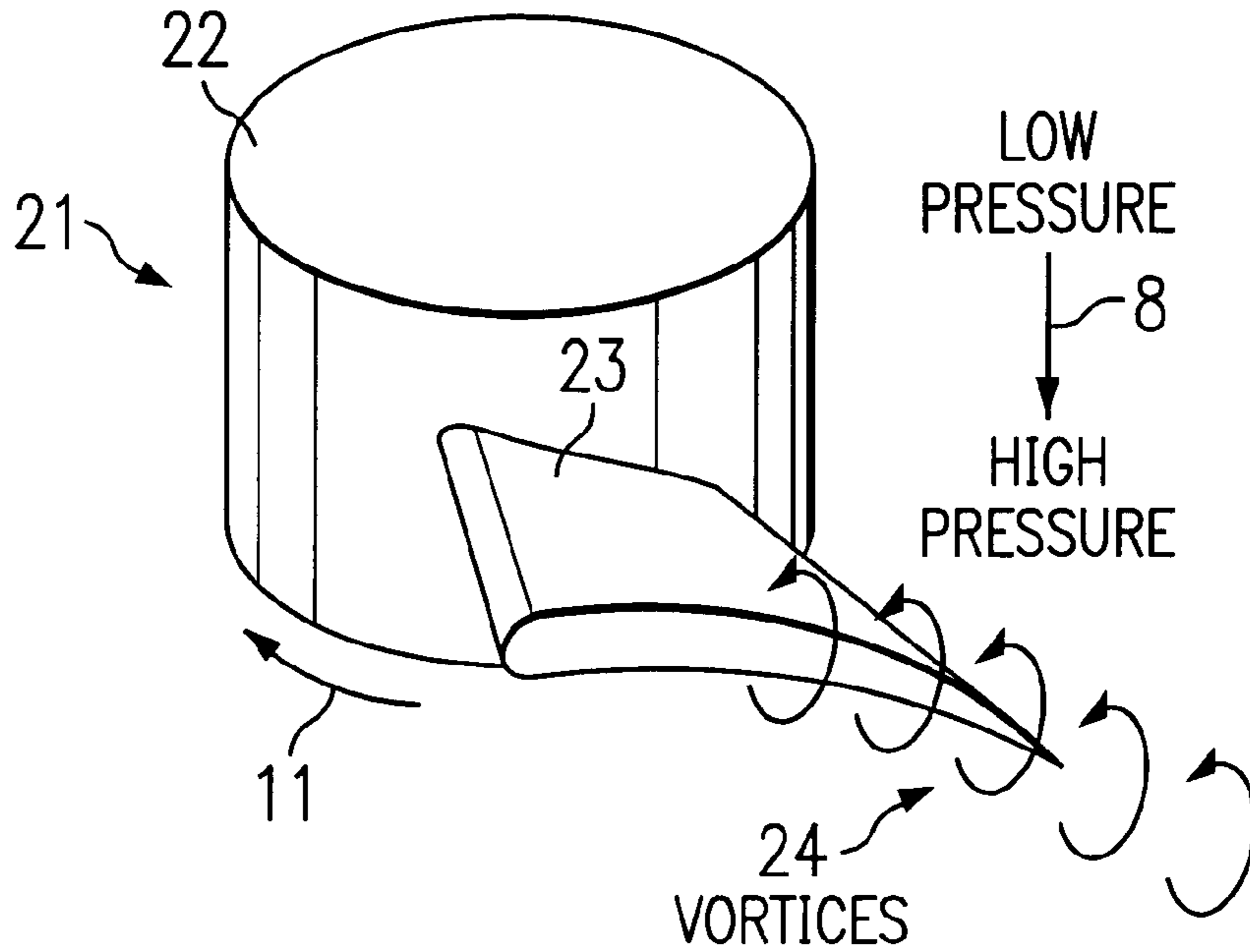
FIG. 2 (PRIOR ART)
