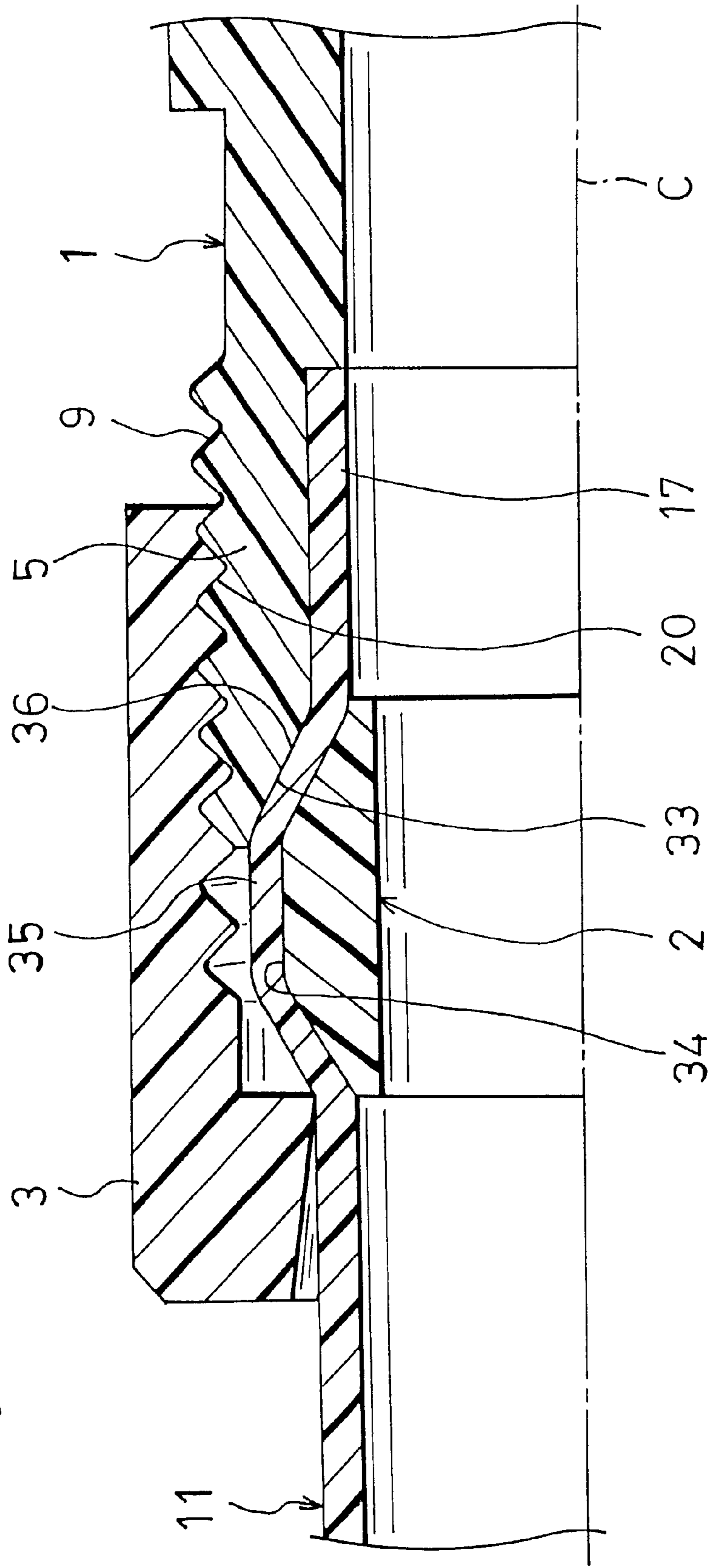
Fig. 6 (PRIOR ART)
