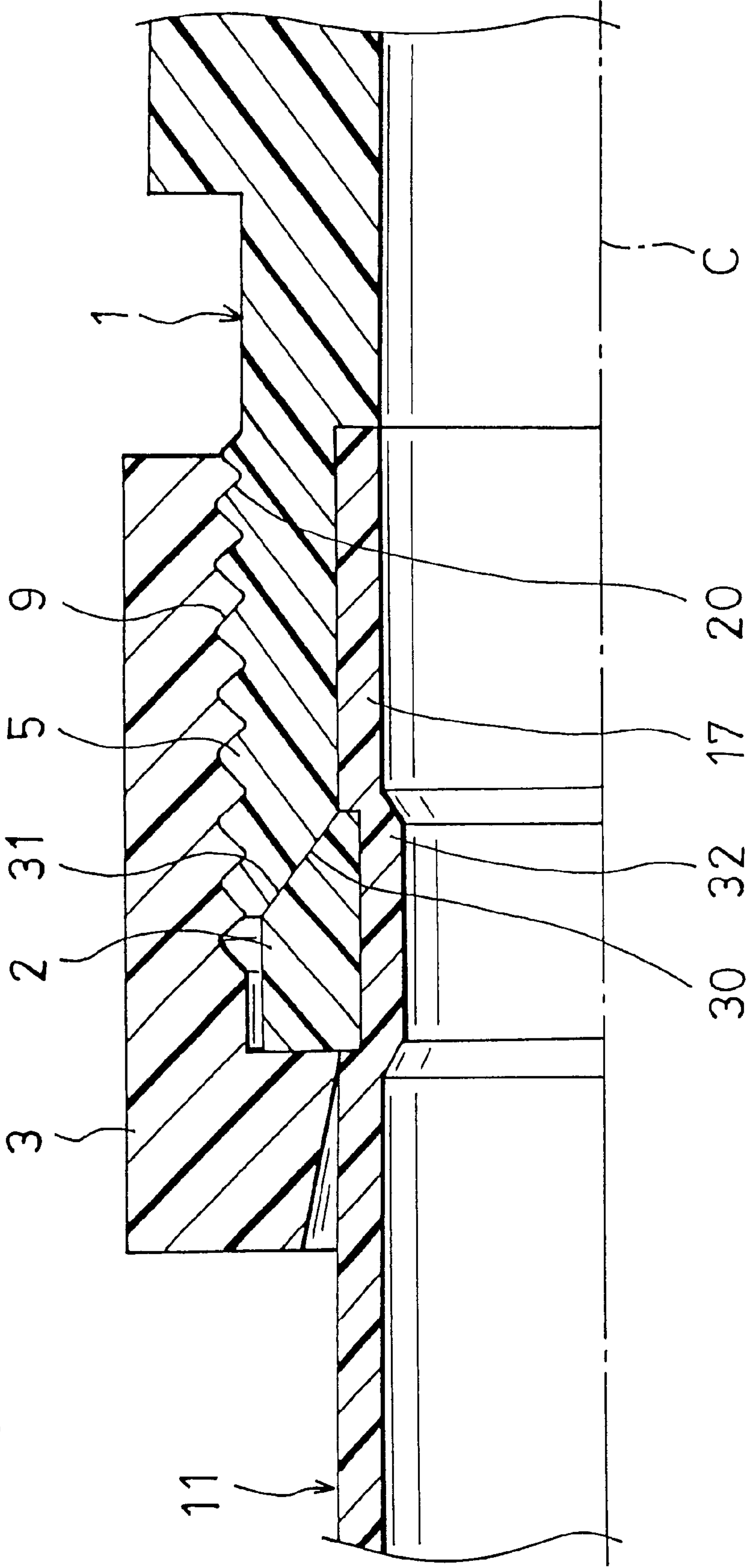
Fig. 5 (PRIOR ART)
