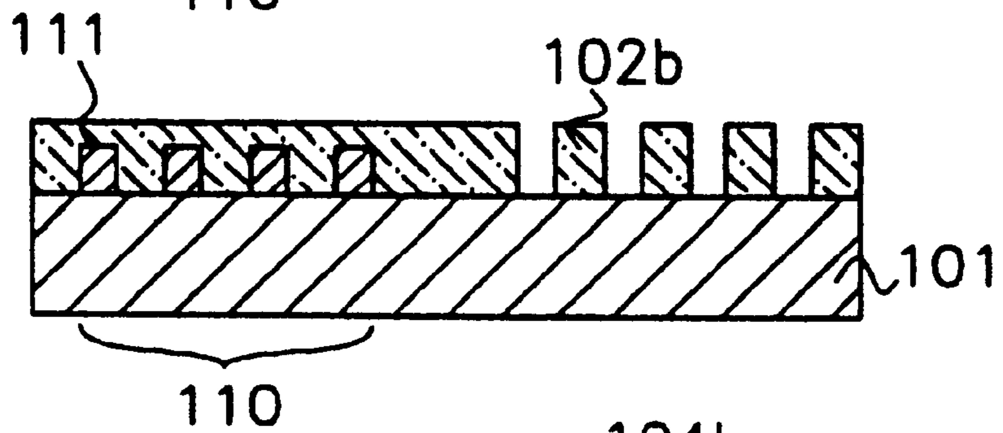
FIG. 6C PRIOR ART
