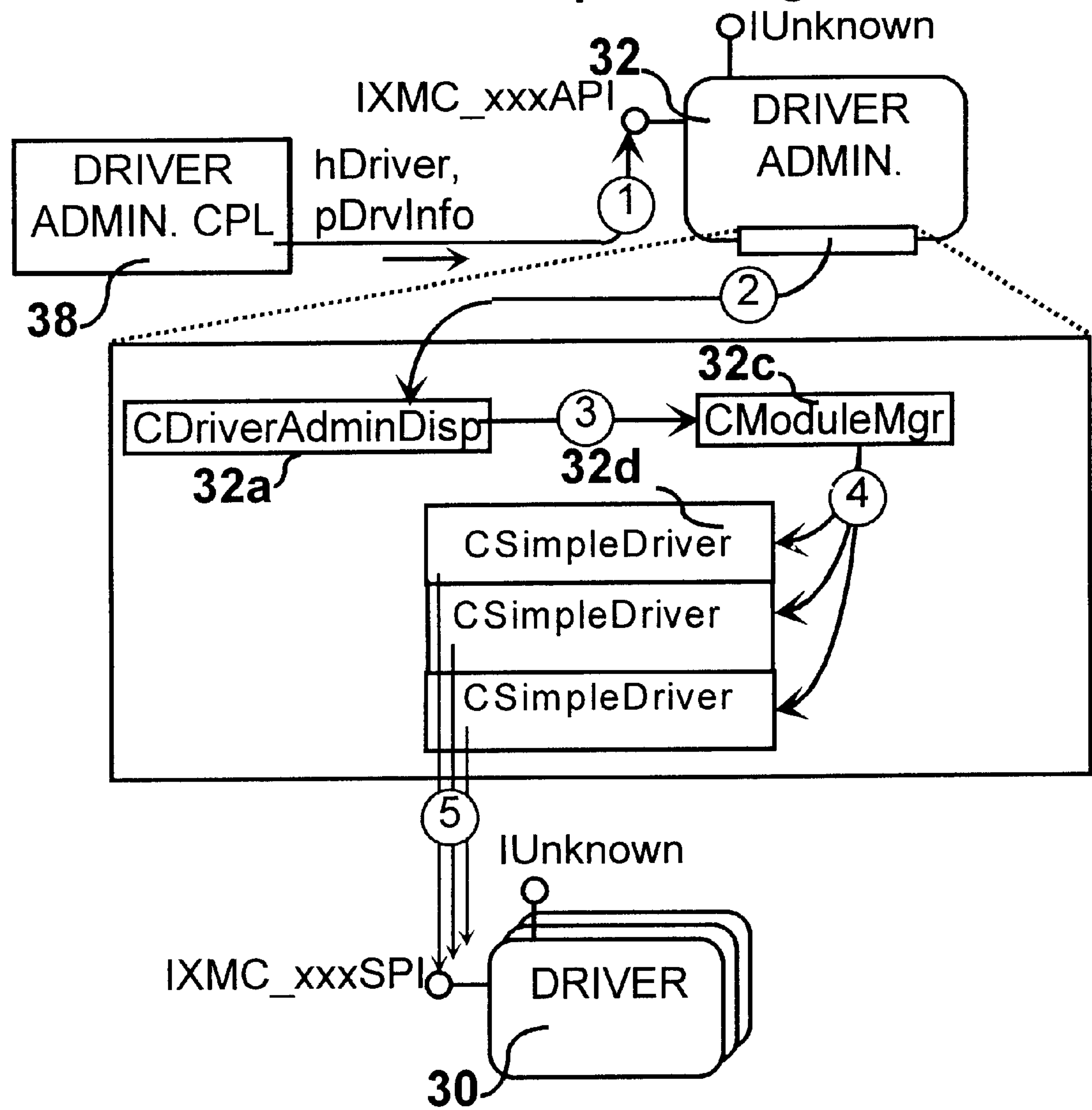
FIG. 45 Scenario-Map - Setting Driver Info.
