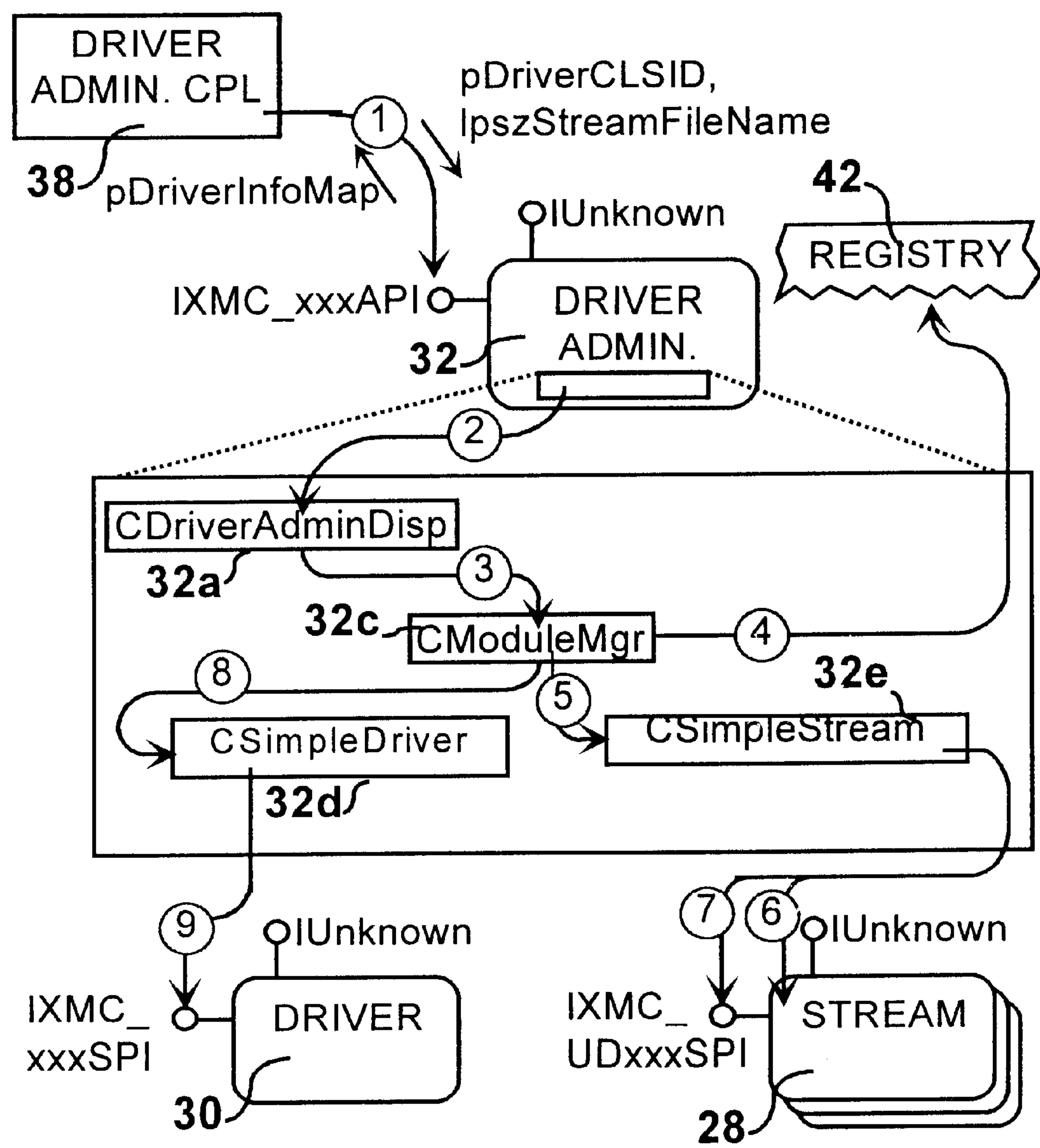
FIG. 44 Scenario-Map - Registering a Stream
