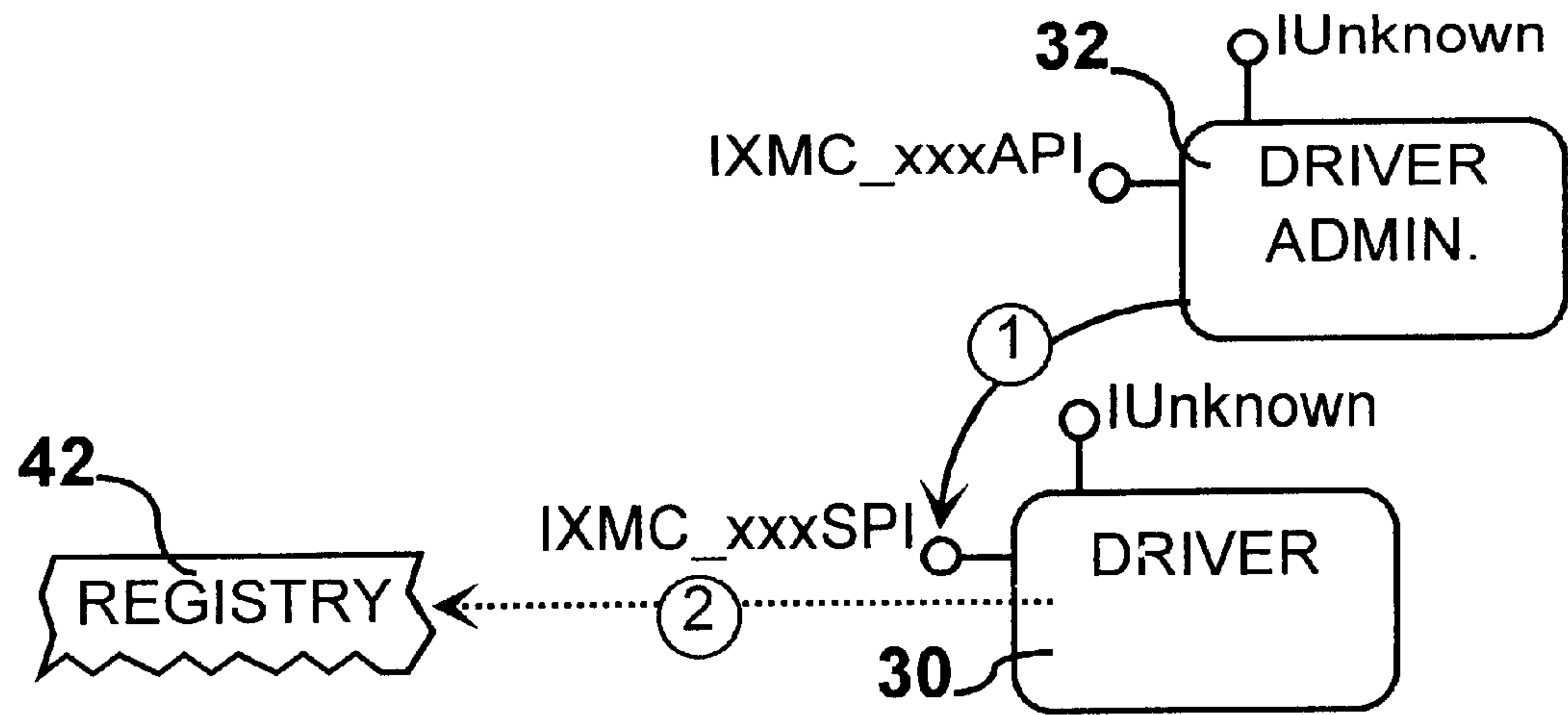
FIG. 13 Scenario-Map - Registration
