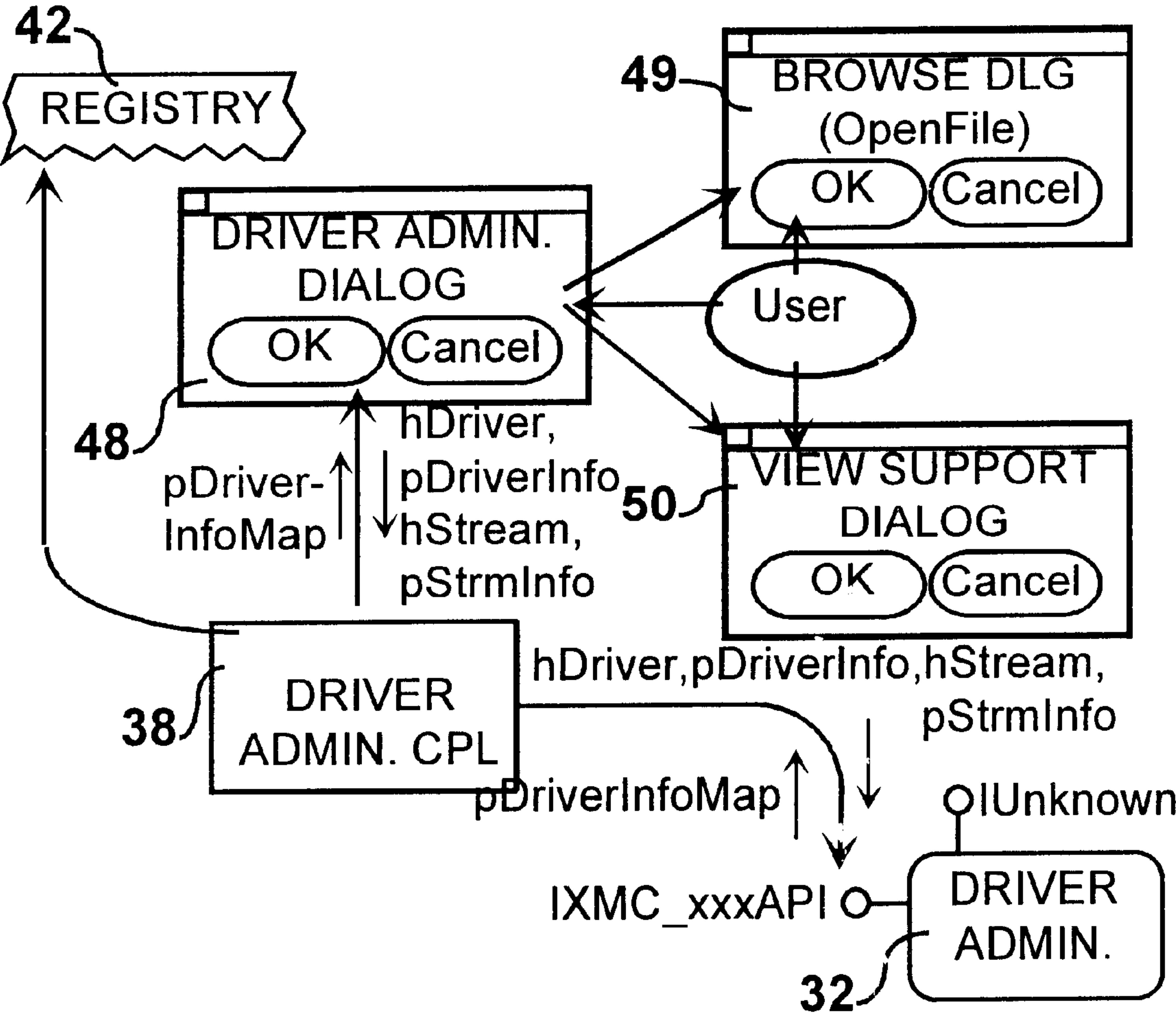
FIG. 51 Module Interaction-Map
