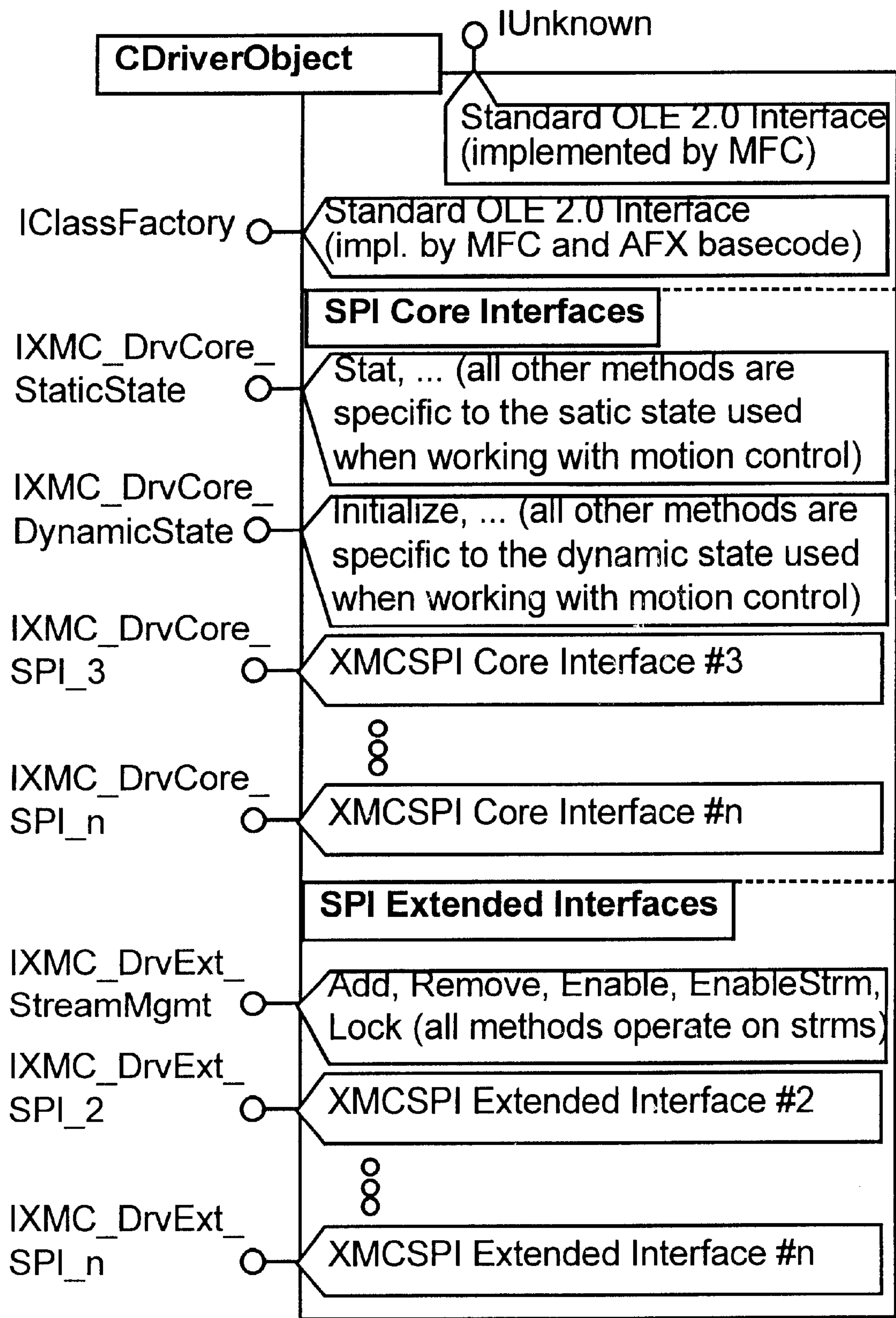
FIG. 21 Interface-Map
