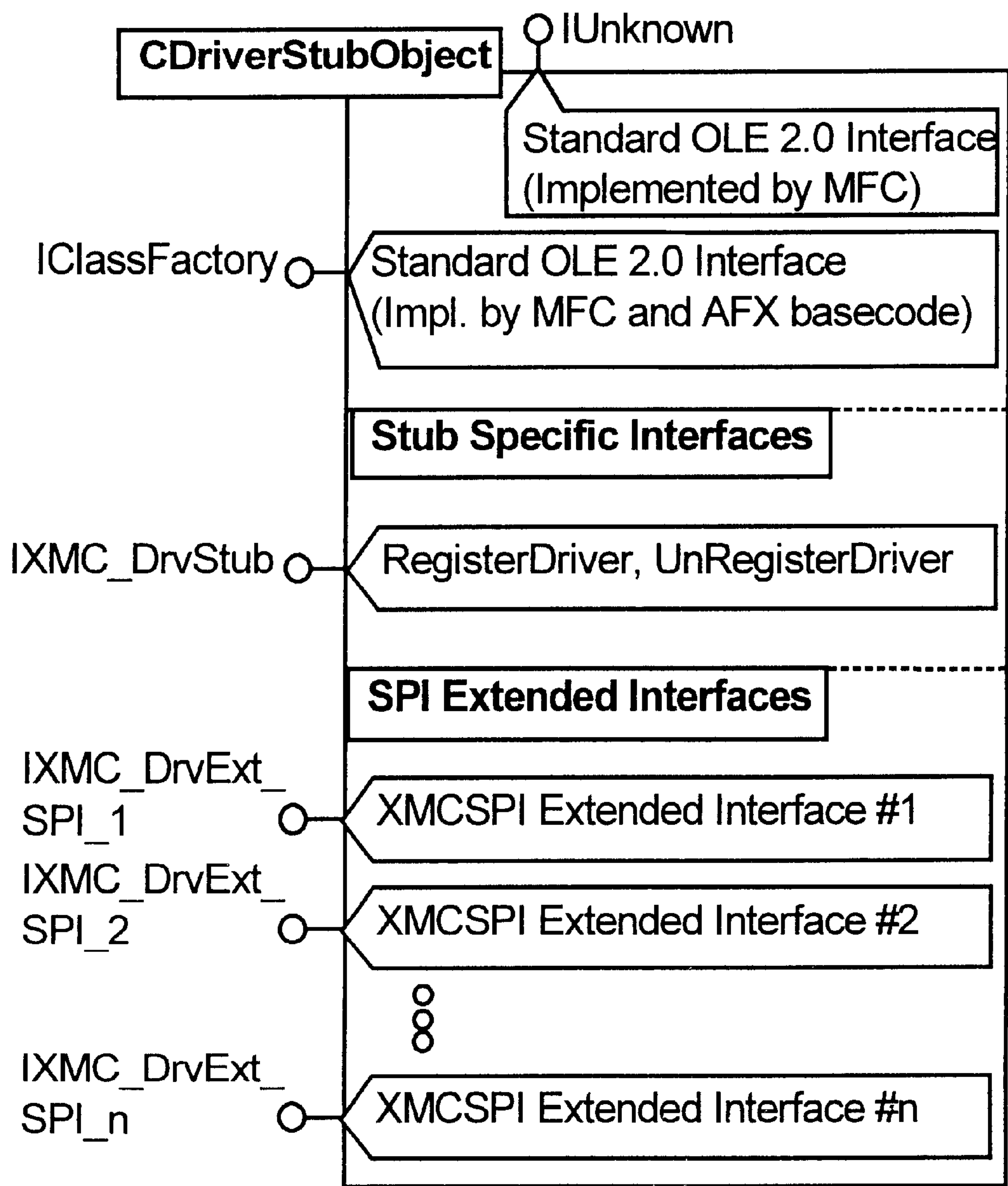
FIG. 39 Interface-Map
