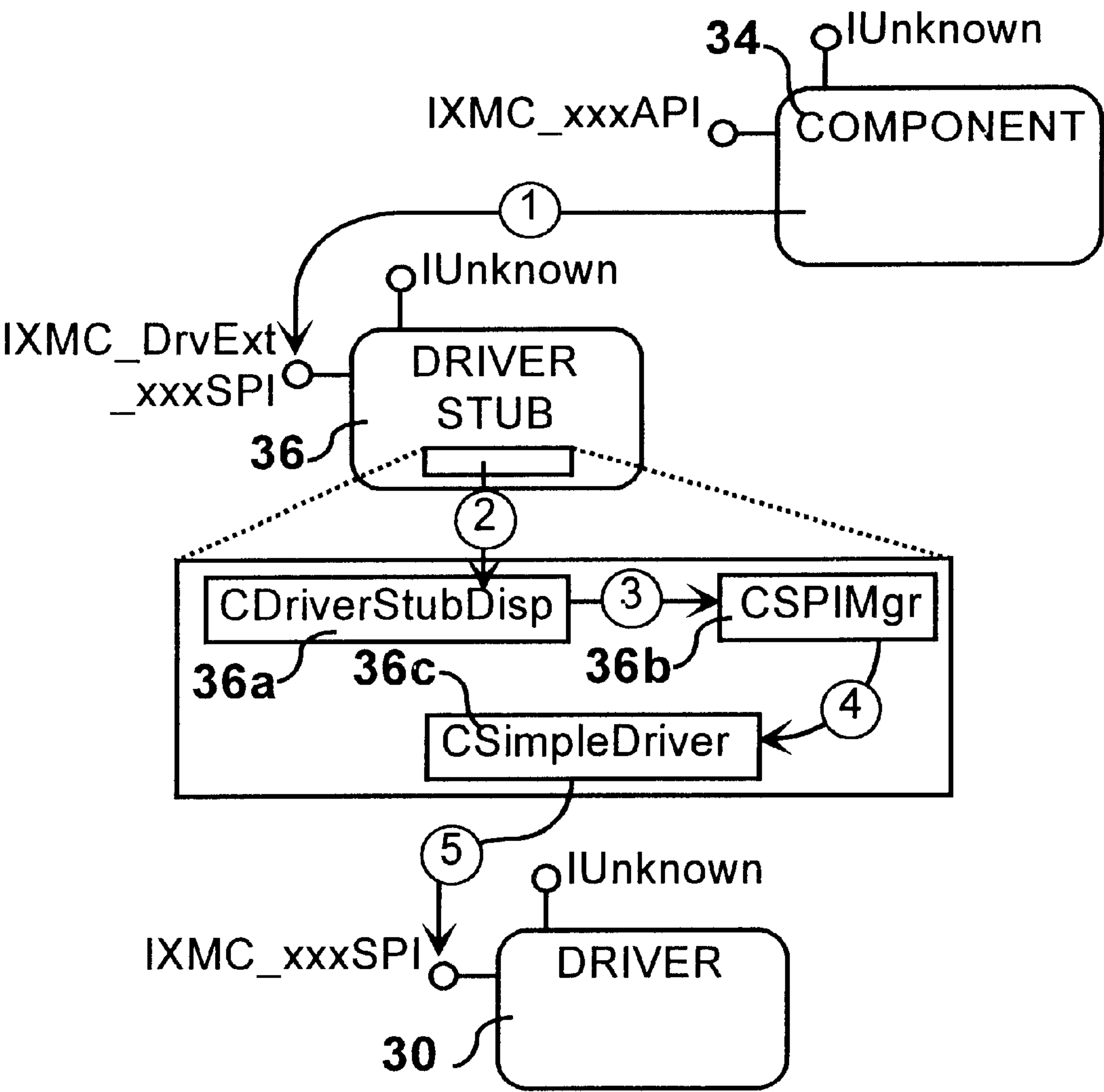
FIG. 37 Scenario-Map - Operations
