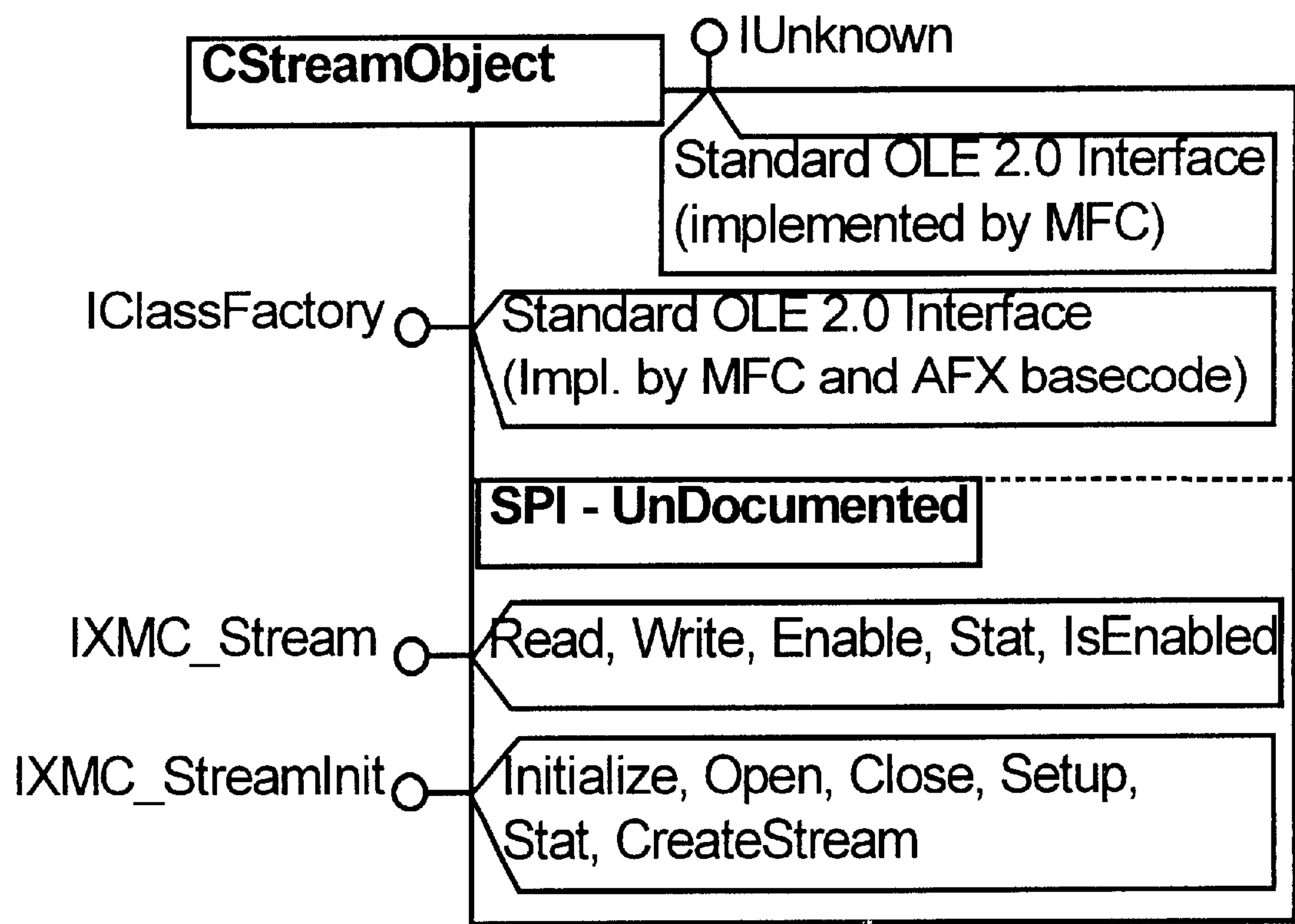
FIG. 33 Interface-Map
