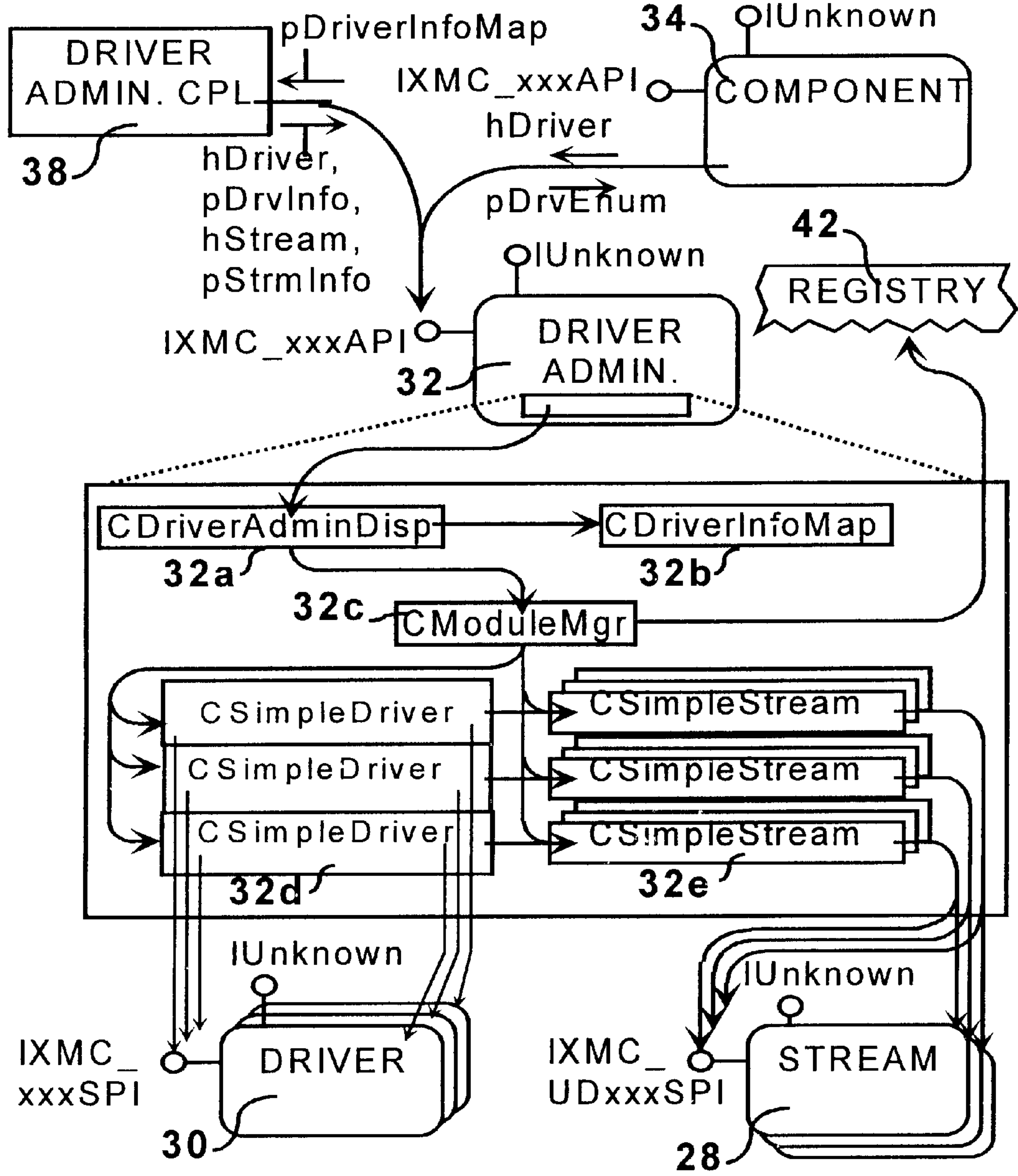
FIG. 41 Object Interaction-Map
