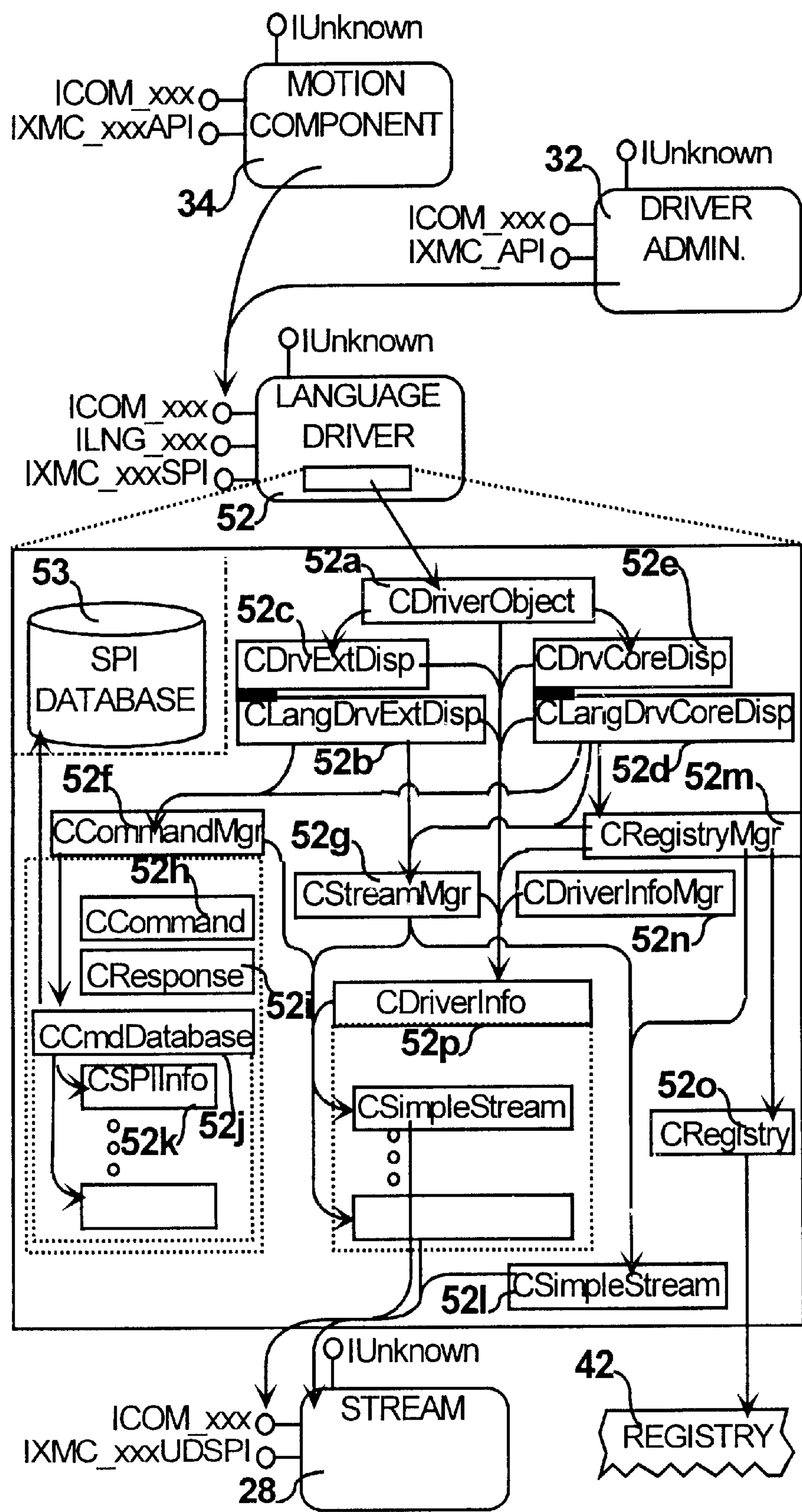
FIG. 59 Object Interaction-Map
