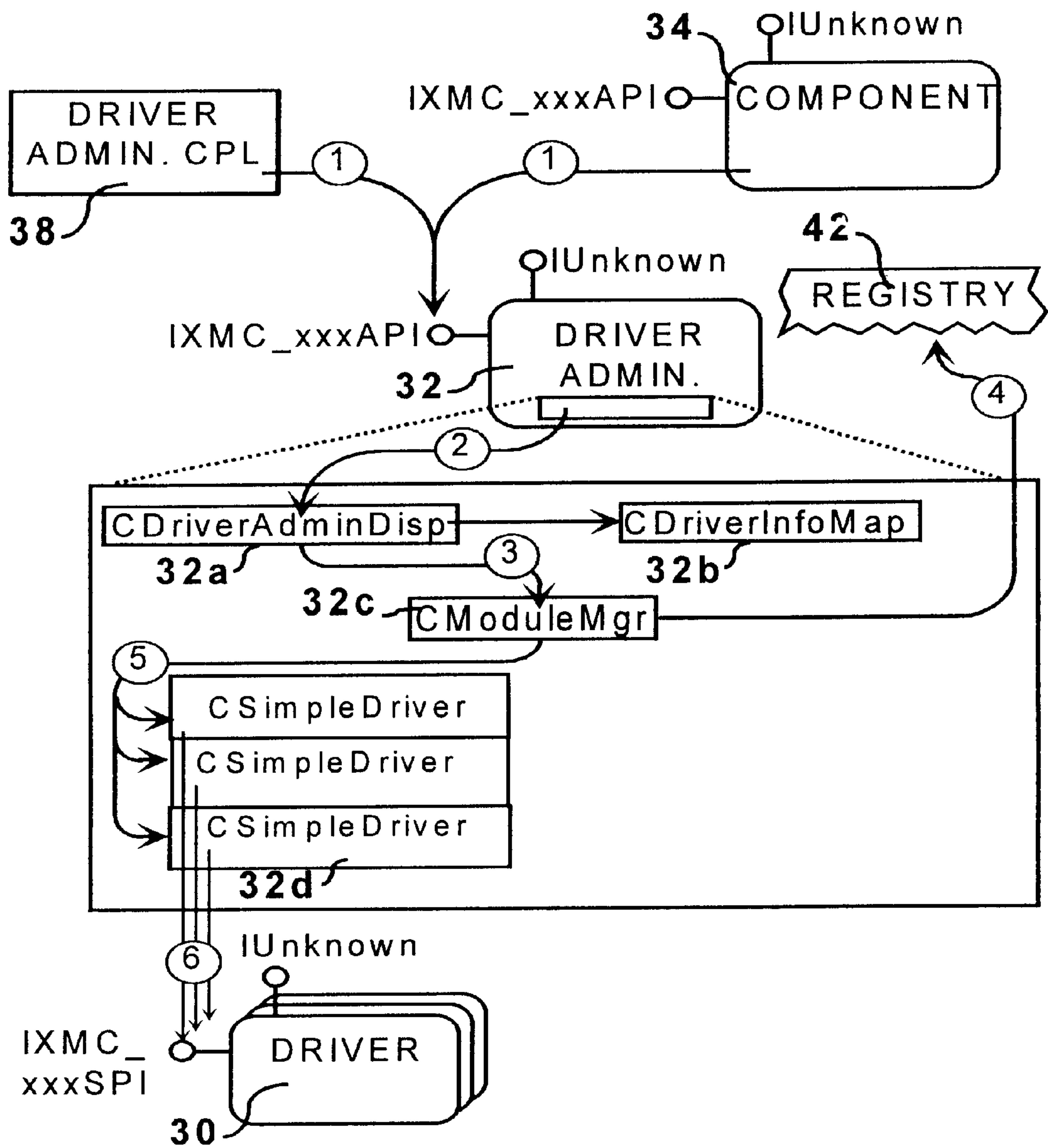
FIG. 42 Scenario-Map - Initialization
