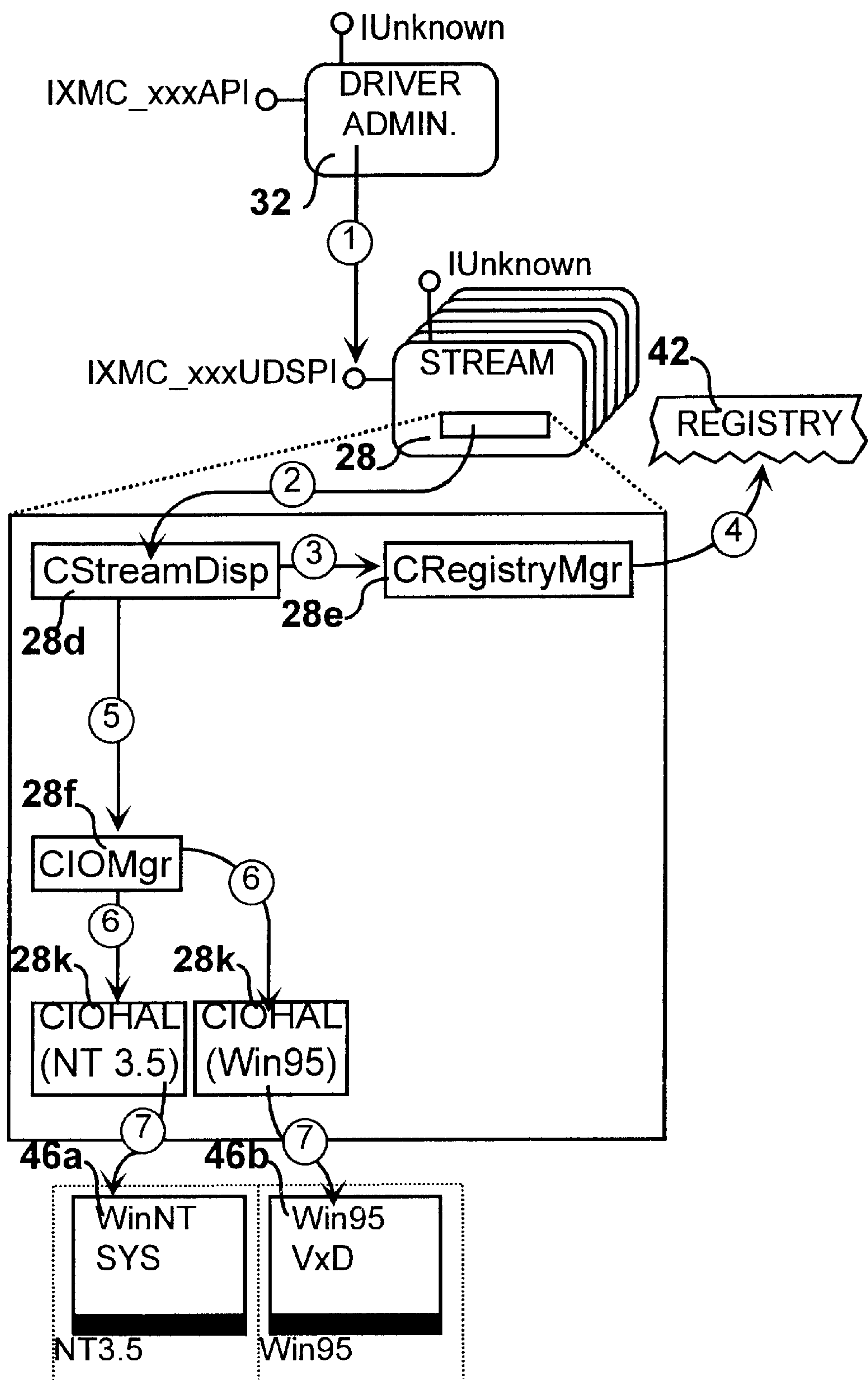
FIG. 24 Scenario-Map - Initialization
