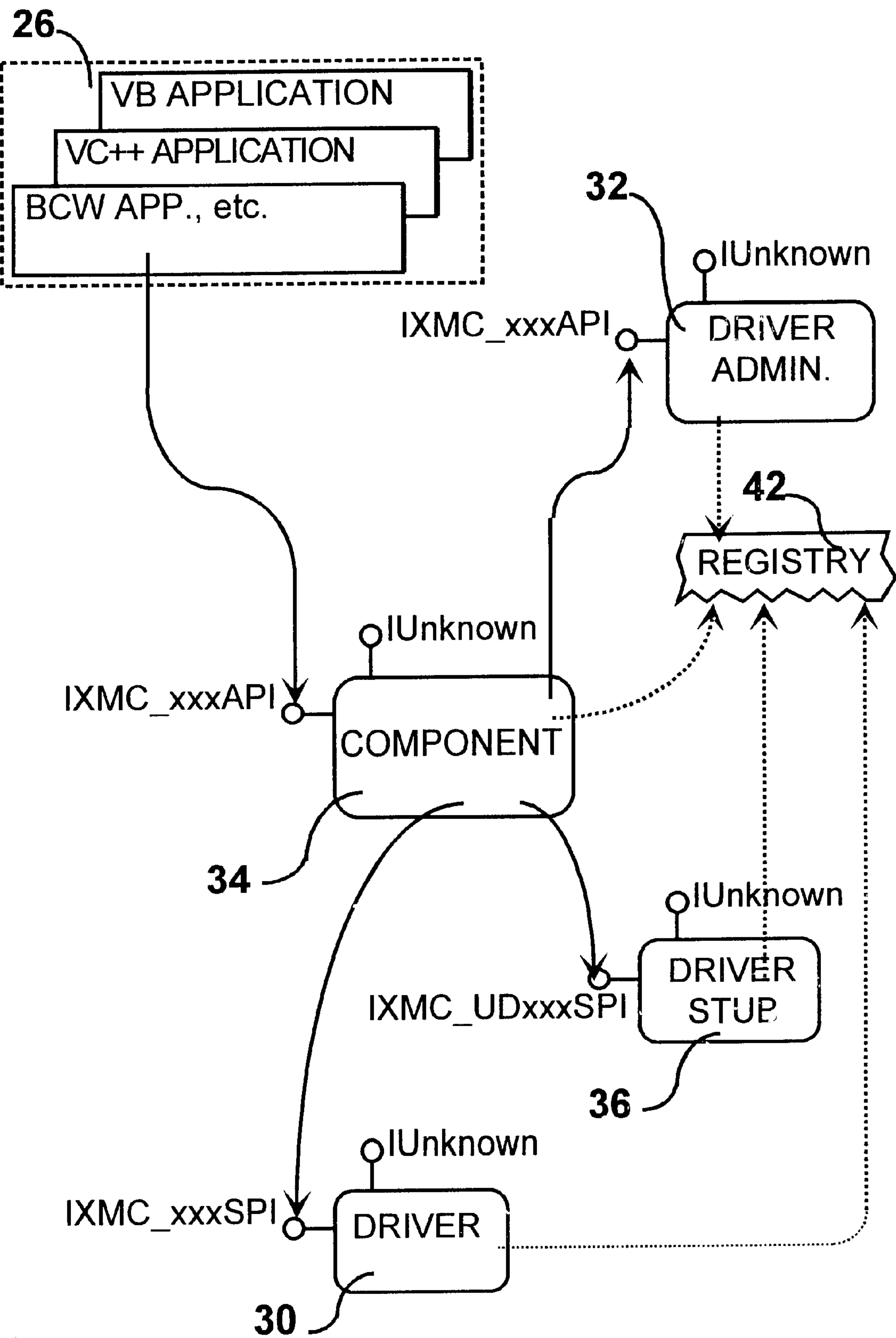
FIG. 2 Module Interaction-Map
