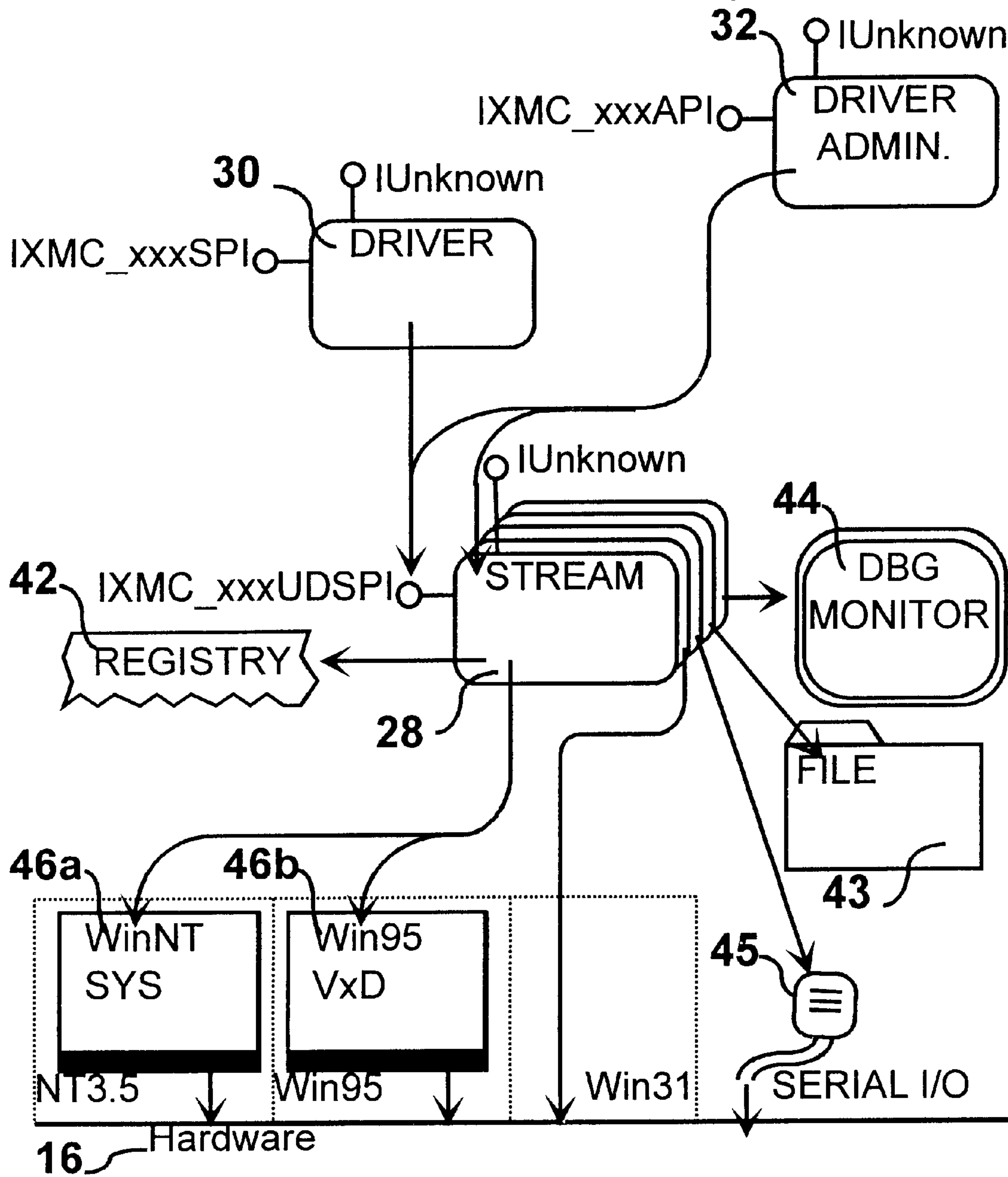
FIG. 22 Module Interaction-Map
