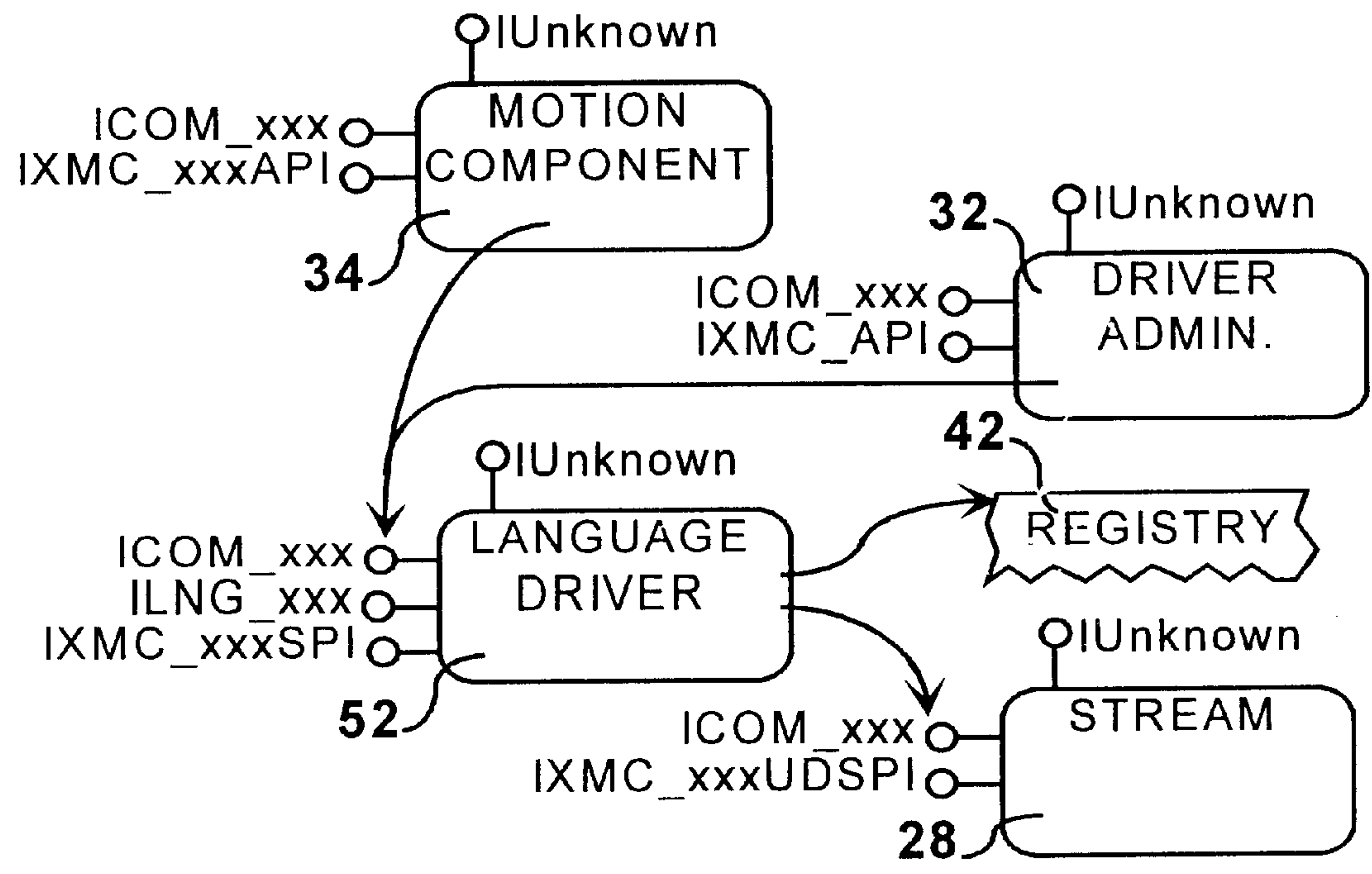
FIG. 58 Module Interaction-Map
