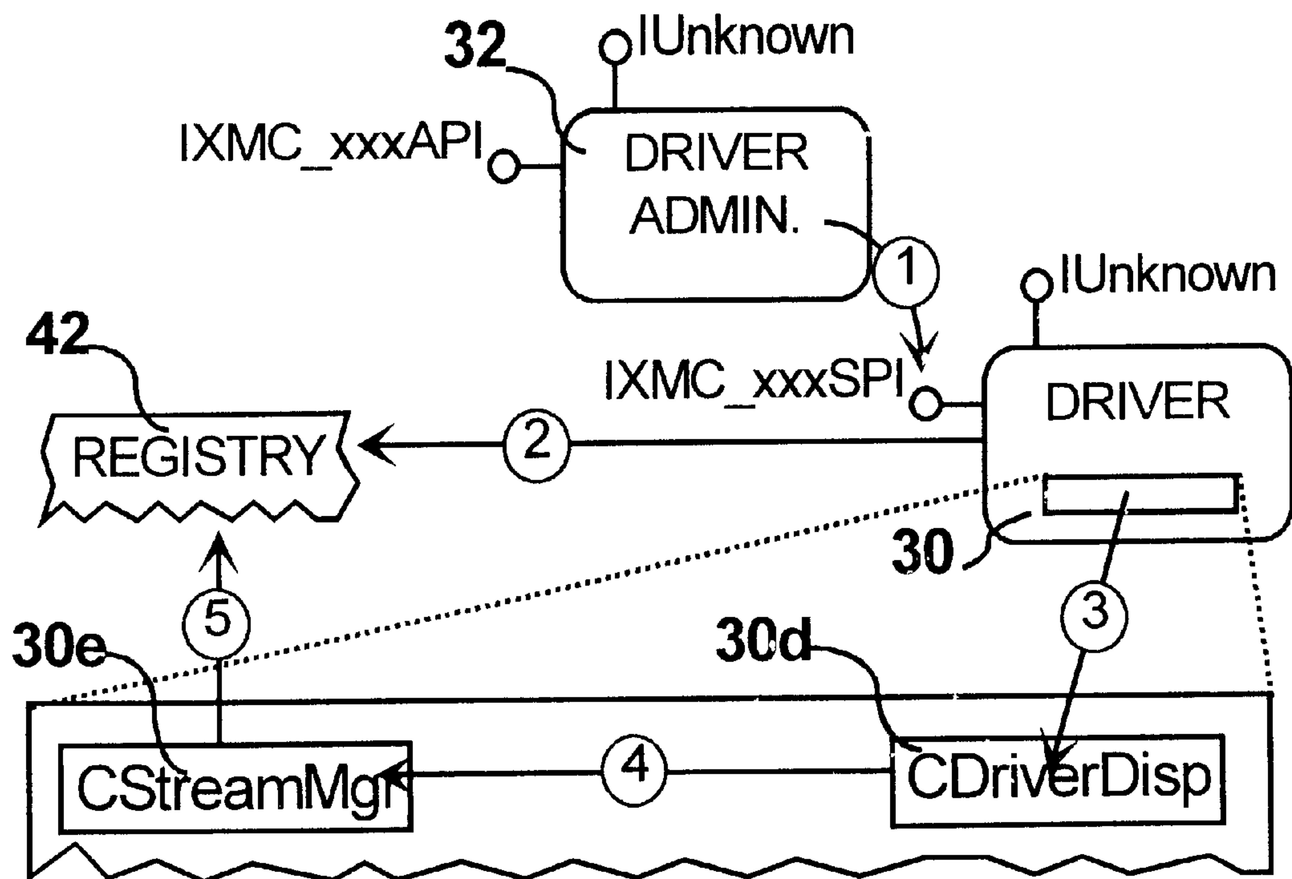
FIG. 14 Scenario-Map - Init. by Driver Admin.
