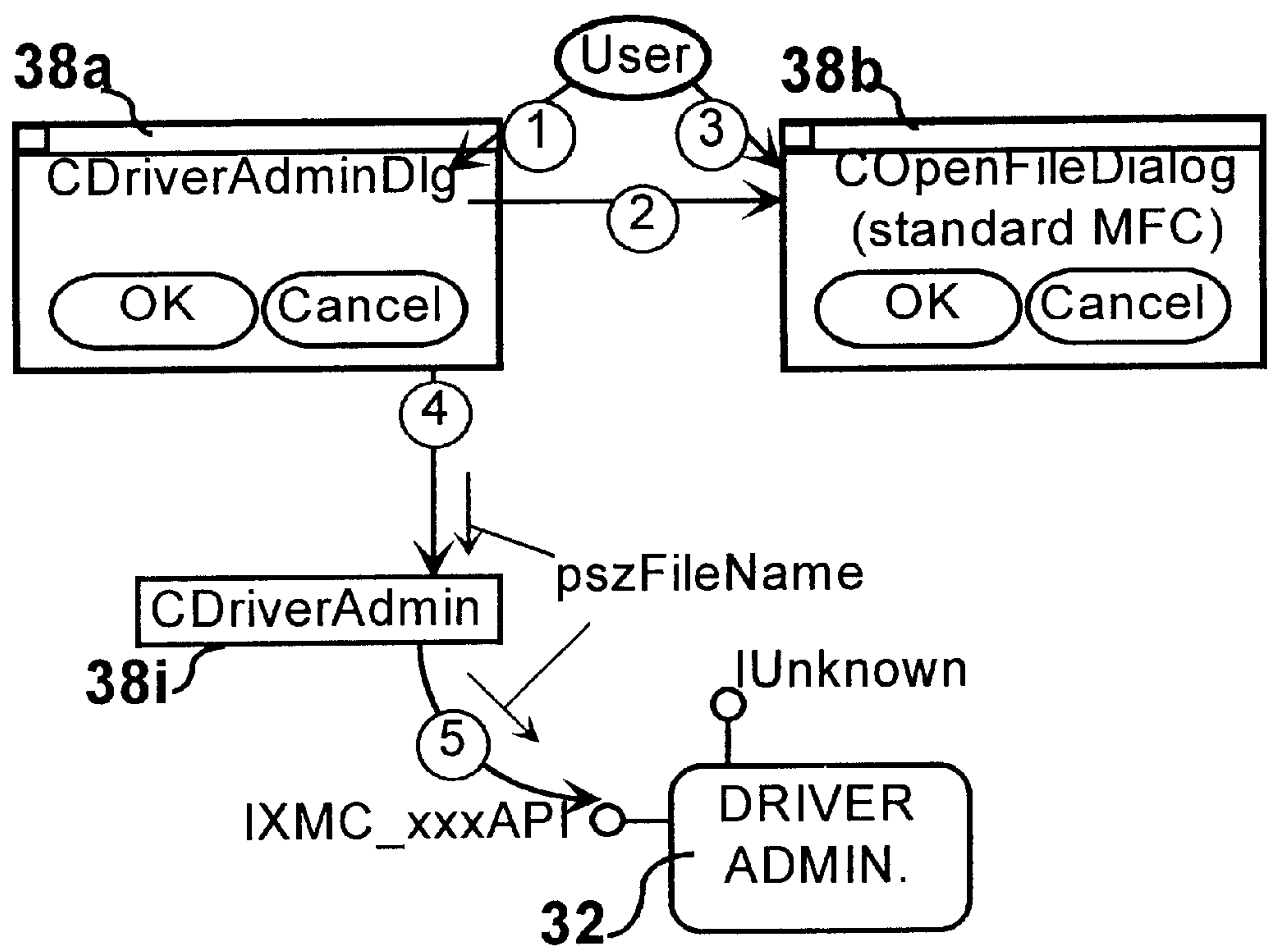
FIG. 55 Scenario-Map - Adding a Driver
