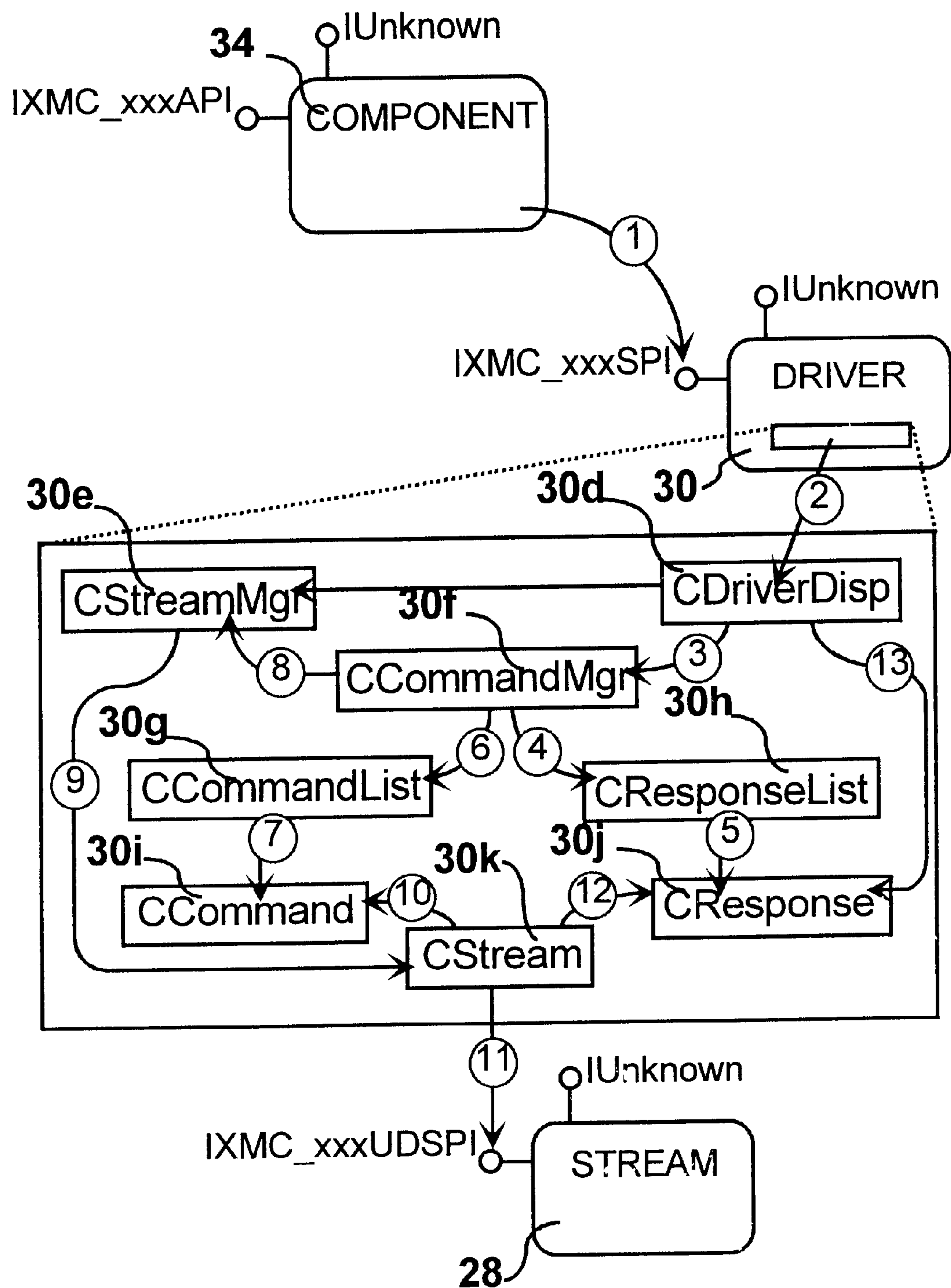
FIG. 19 Scenario-Map - Command Operations
