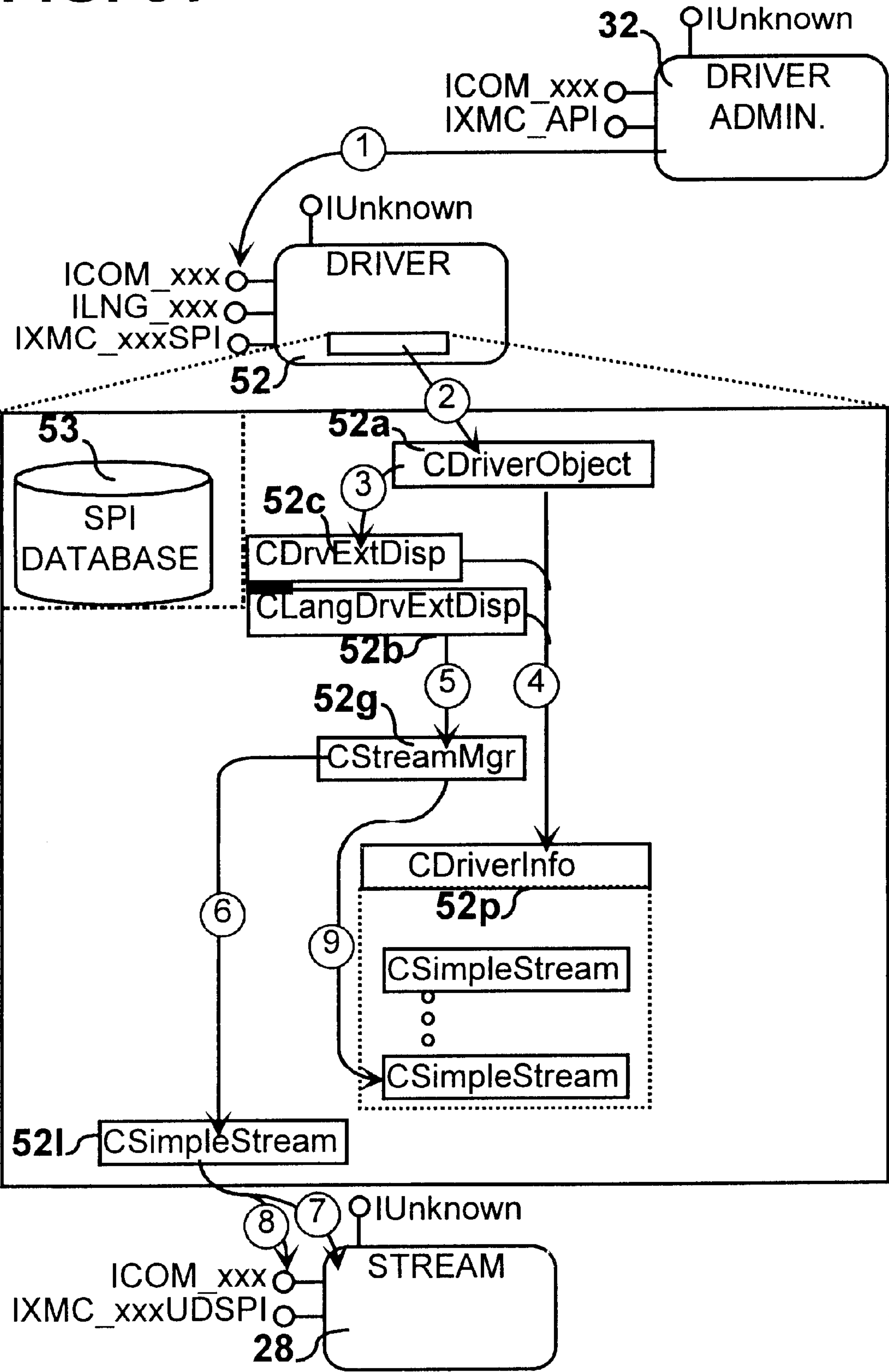
FIG. 61 Scenario-Map - Adding a Stream
