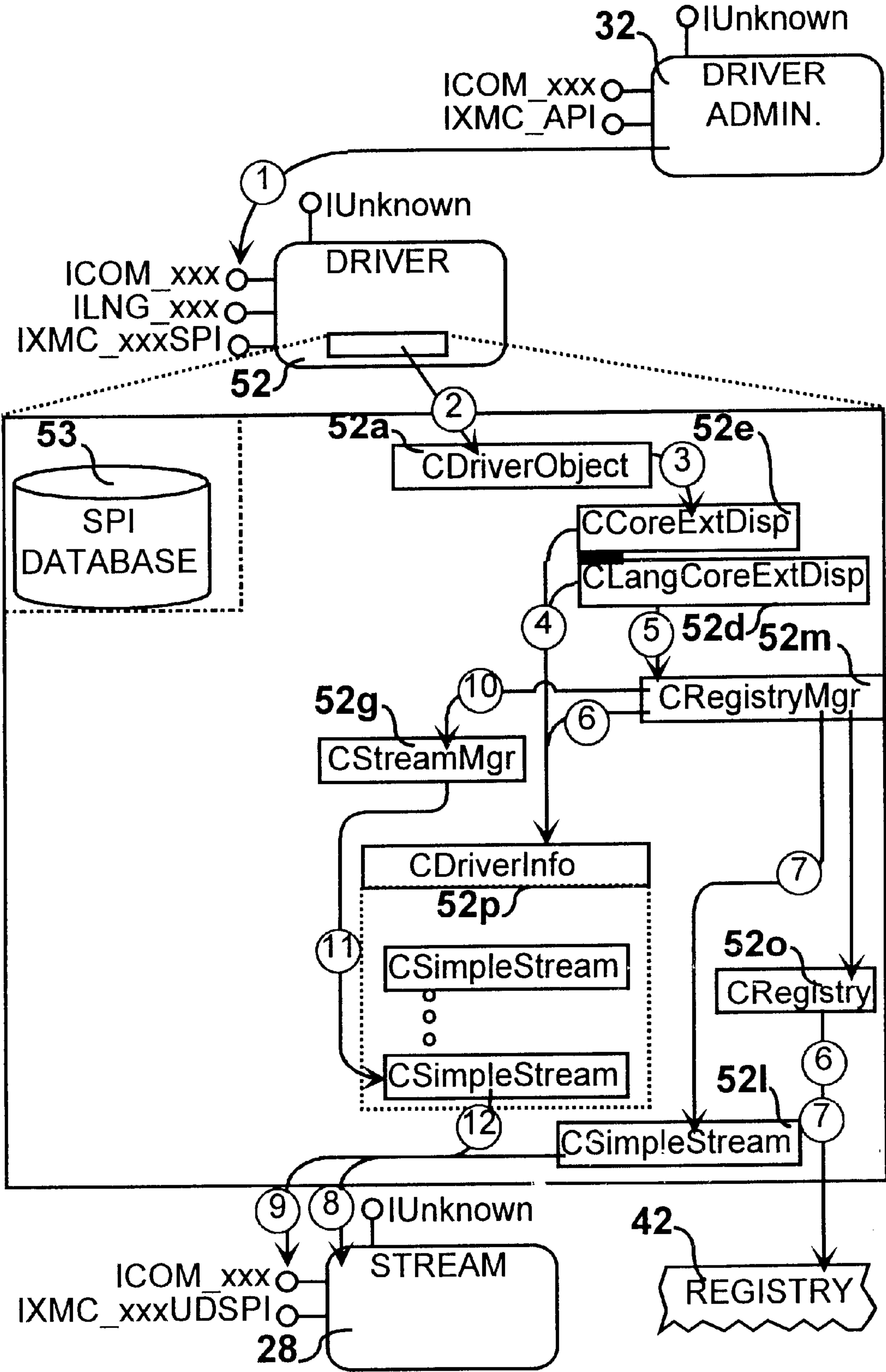
FIG. 63 Scenario-Map - Registration loading
