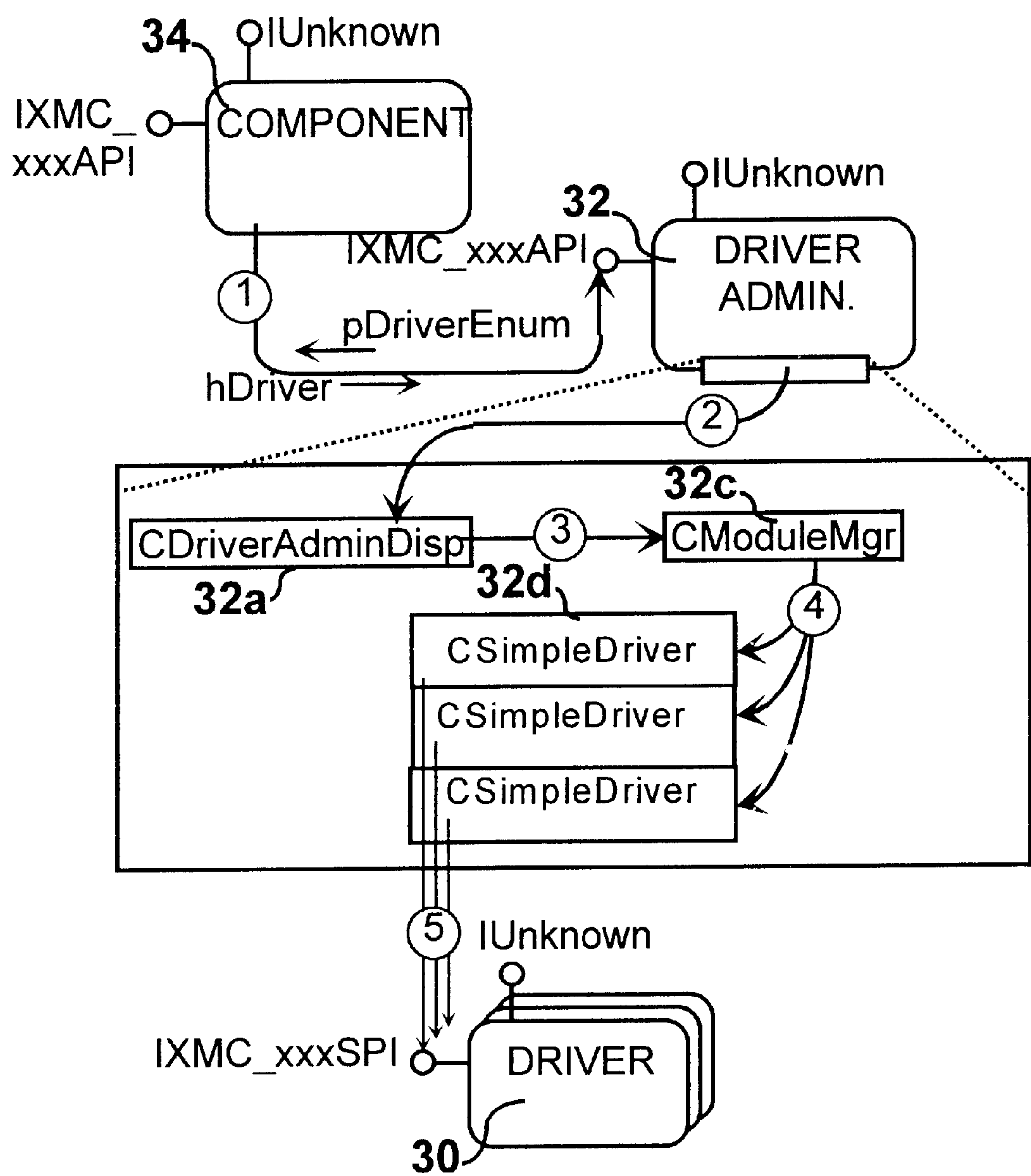
FIG. 47 Scenario-Map - Querying Driver Enum.
