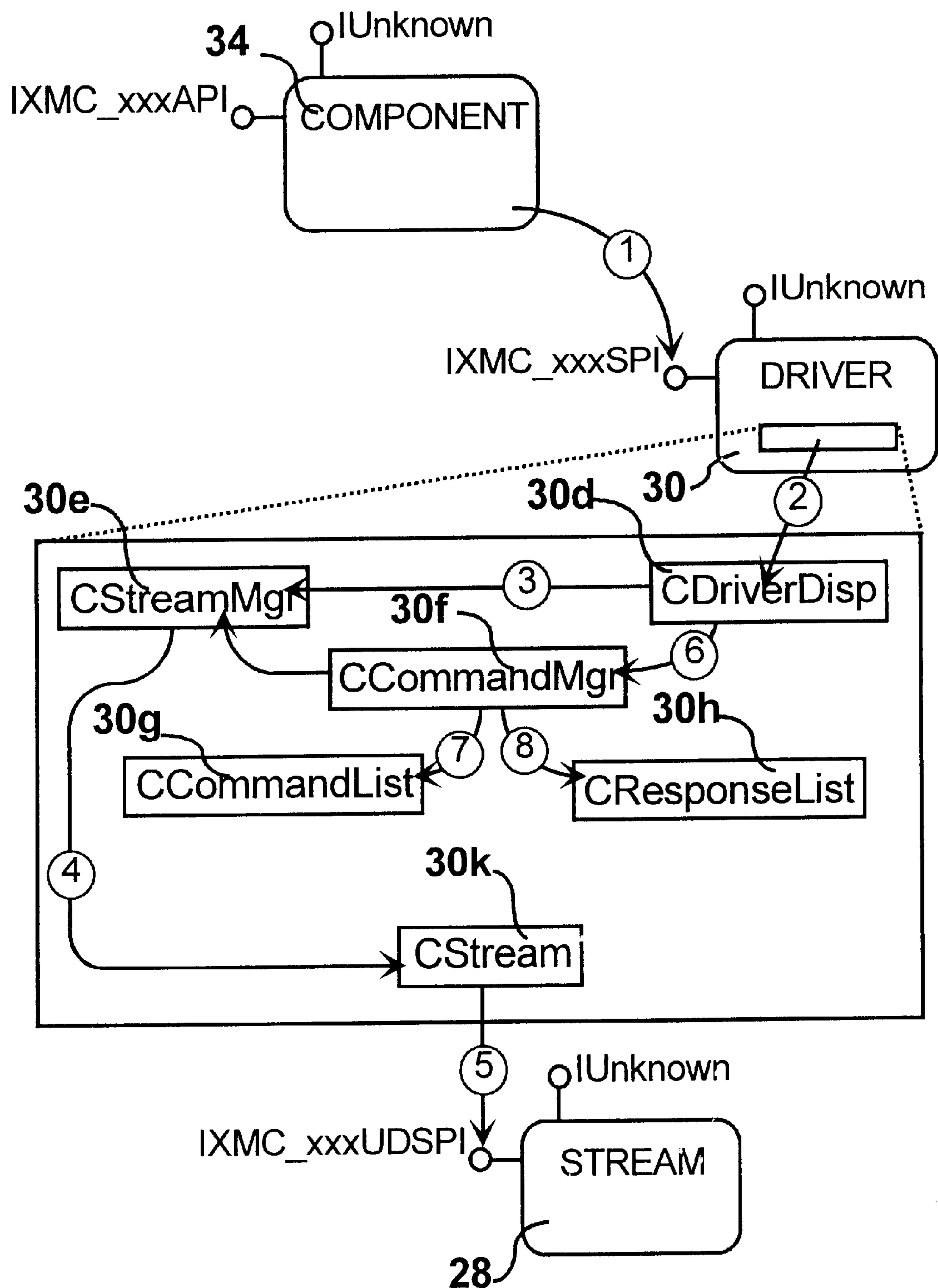
FIG. 20 Scenario-Map - Clean-up by Component
