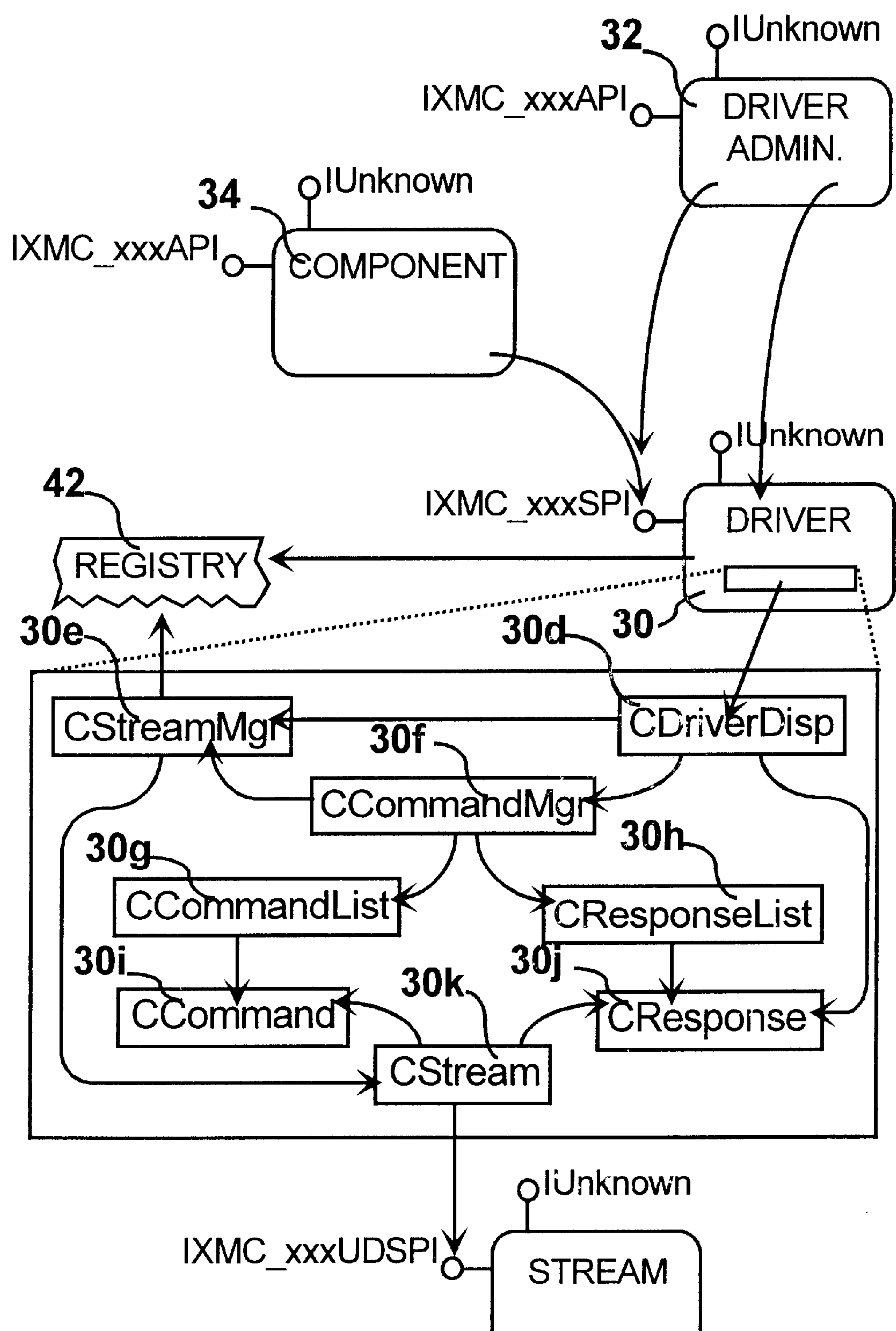
FIG. 12 Object Interaction-Map
