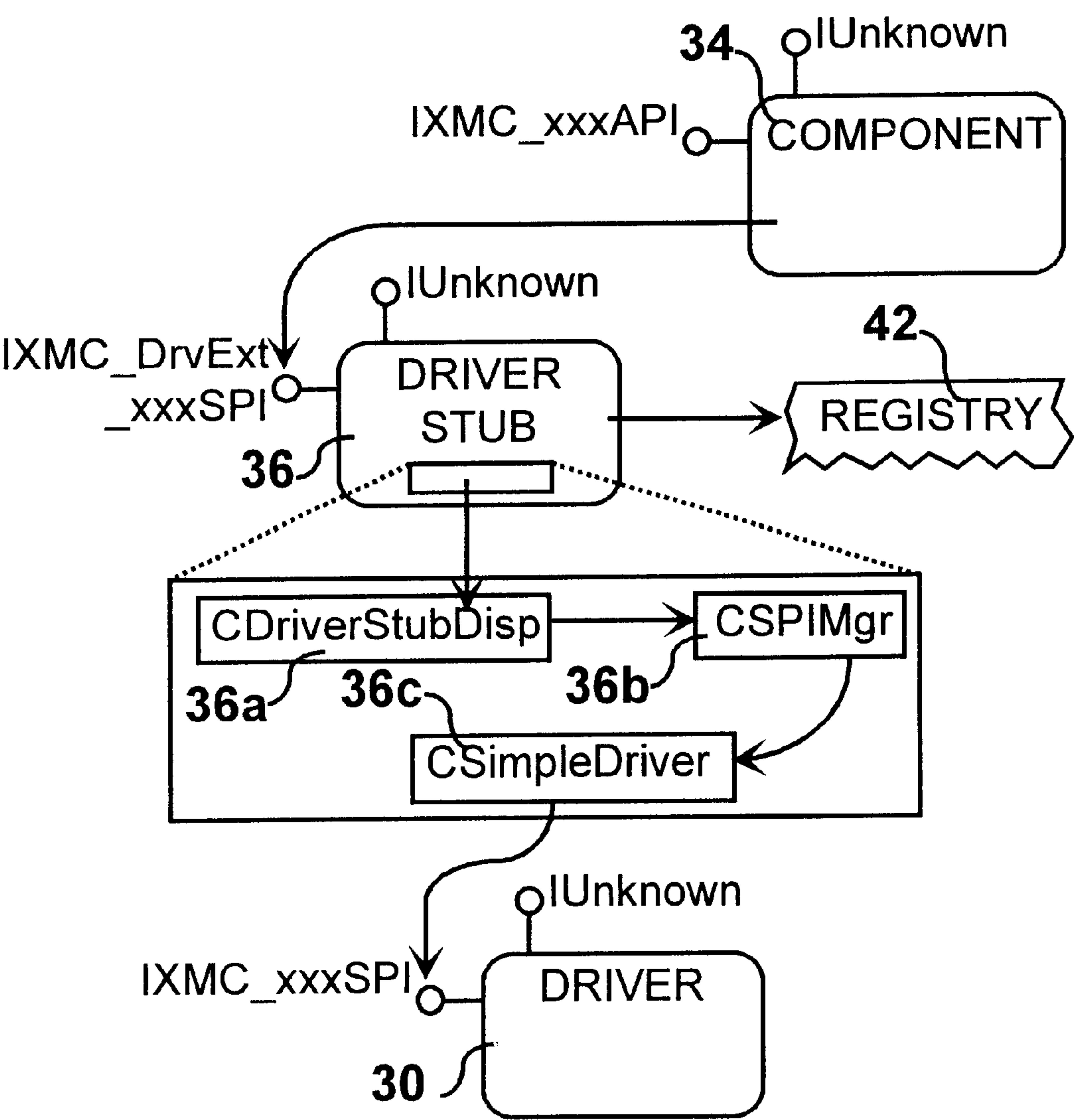
FIG. 35 Object Interaction-Map
