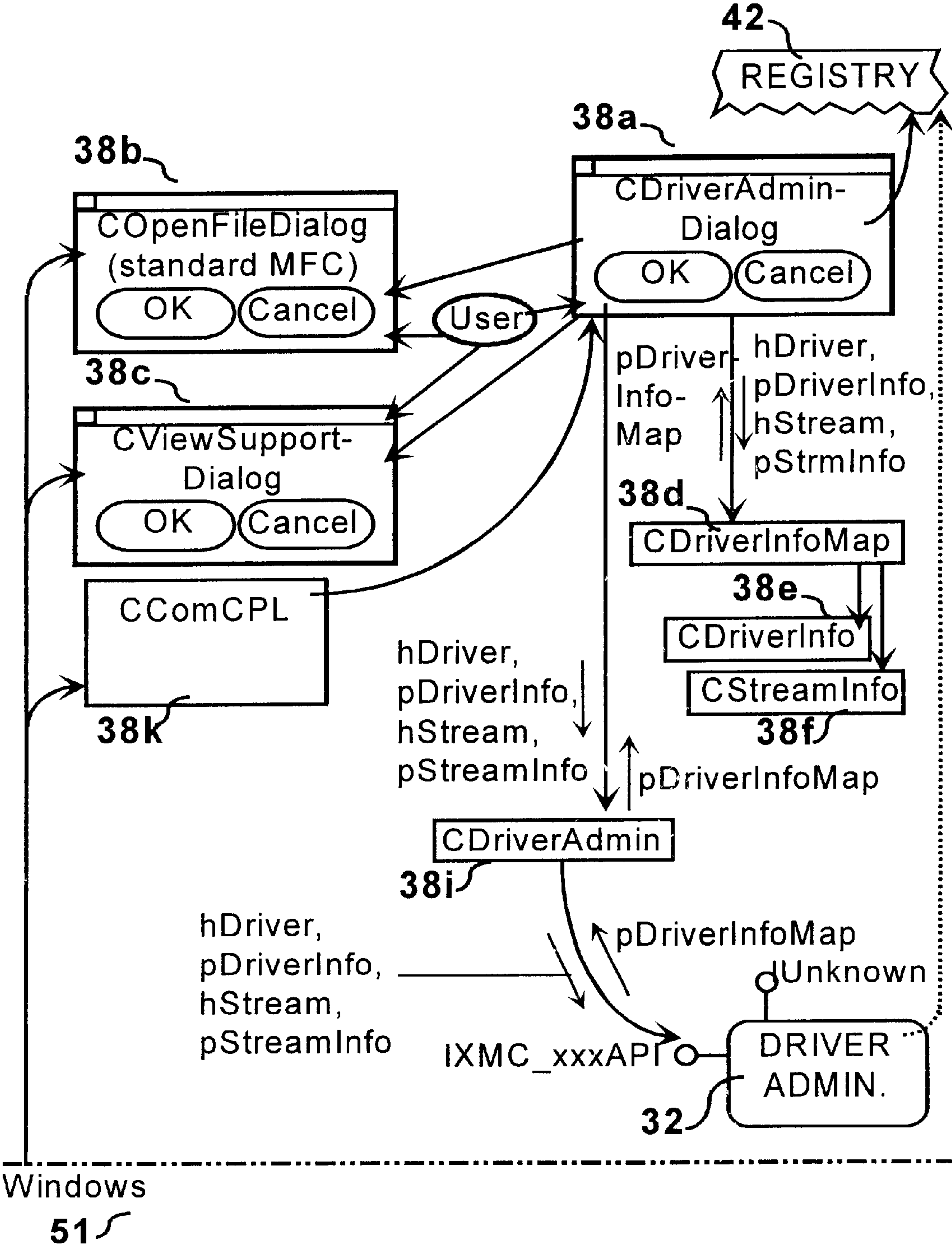
FIG. 52 Object Interaction-Map
