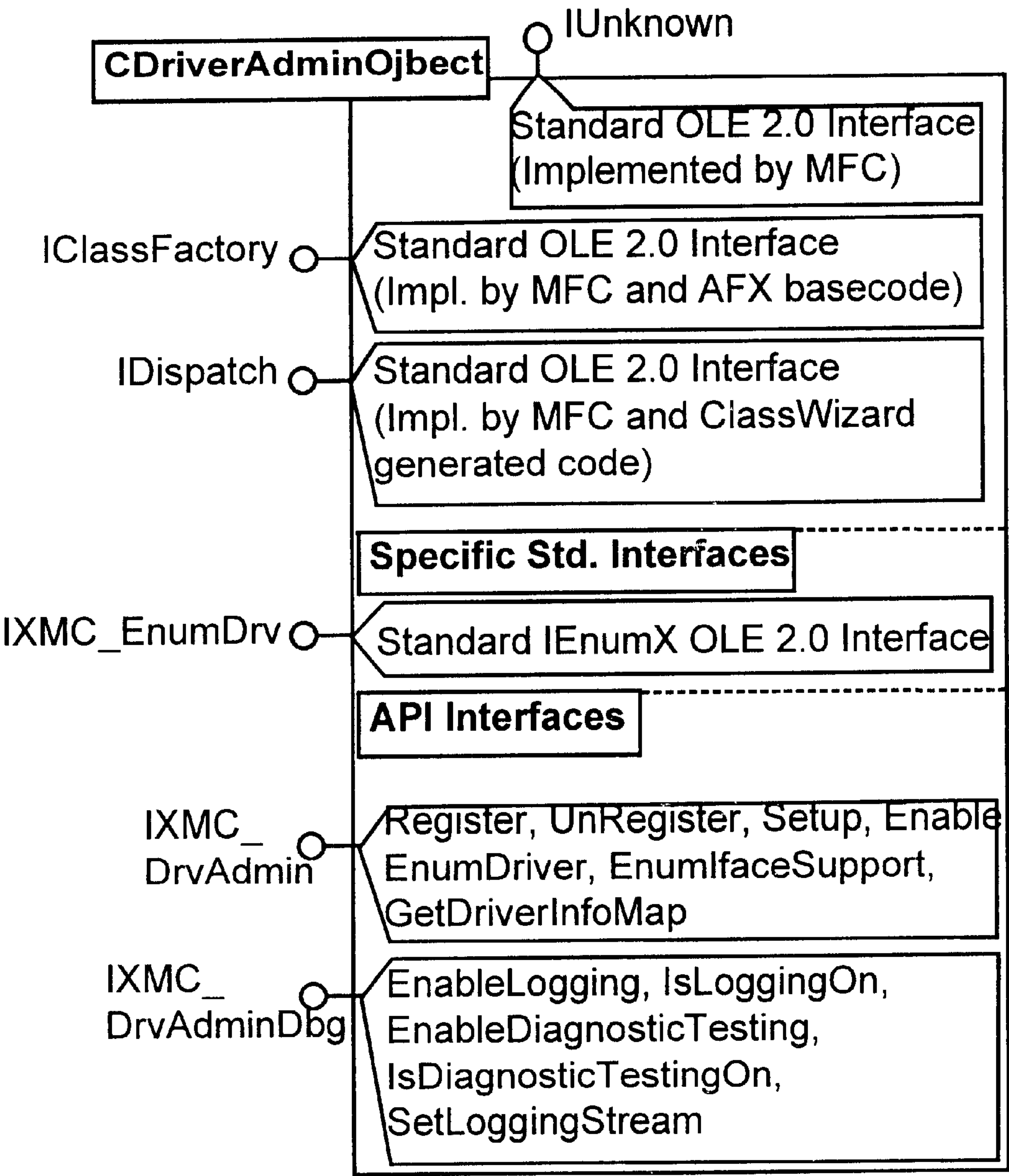
FIG. 50 Interface-Map.
