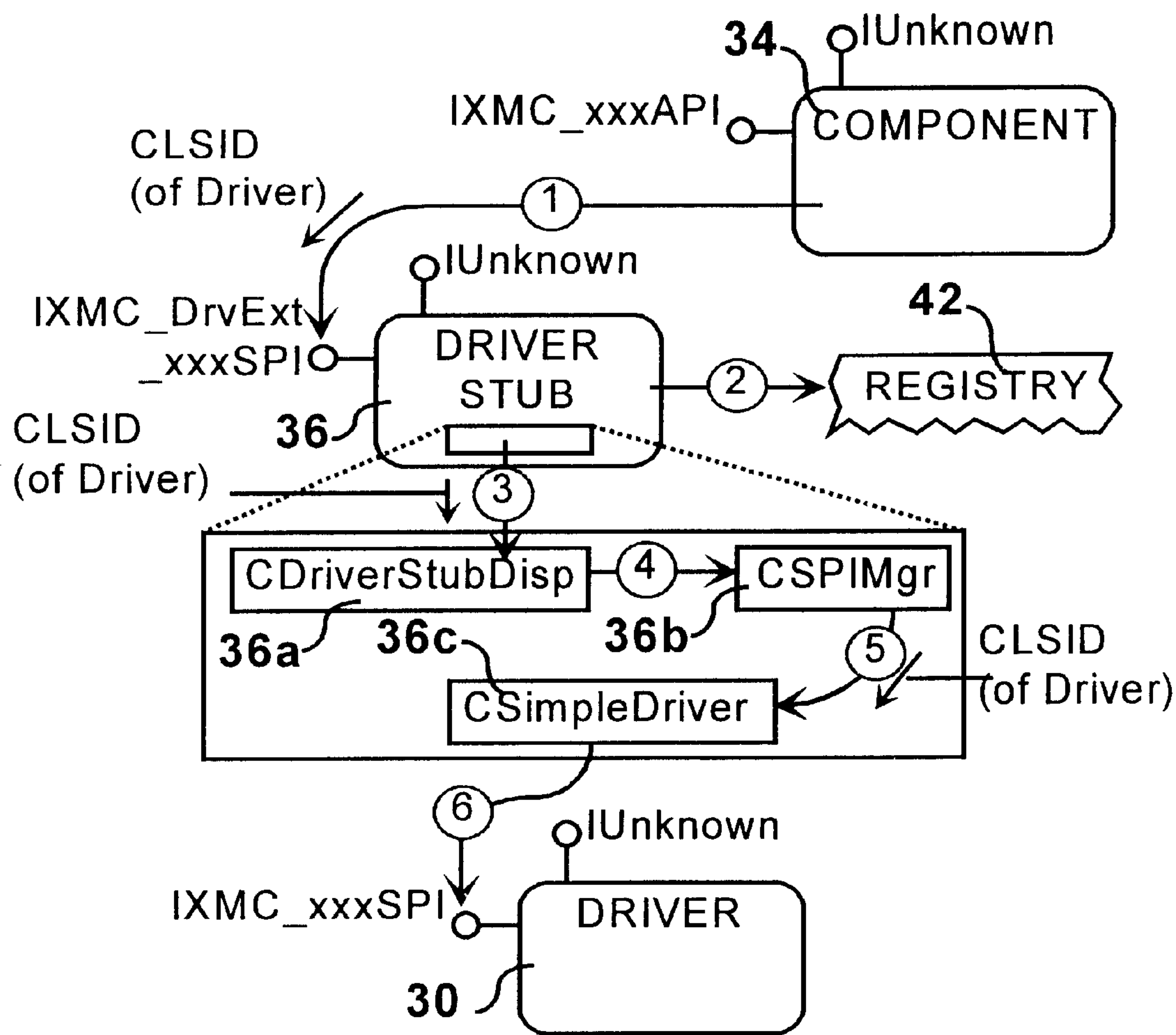
FIG. 36 Scenario-Map - Initialization
