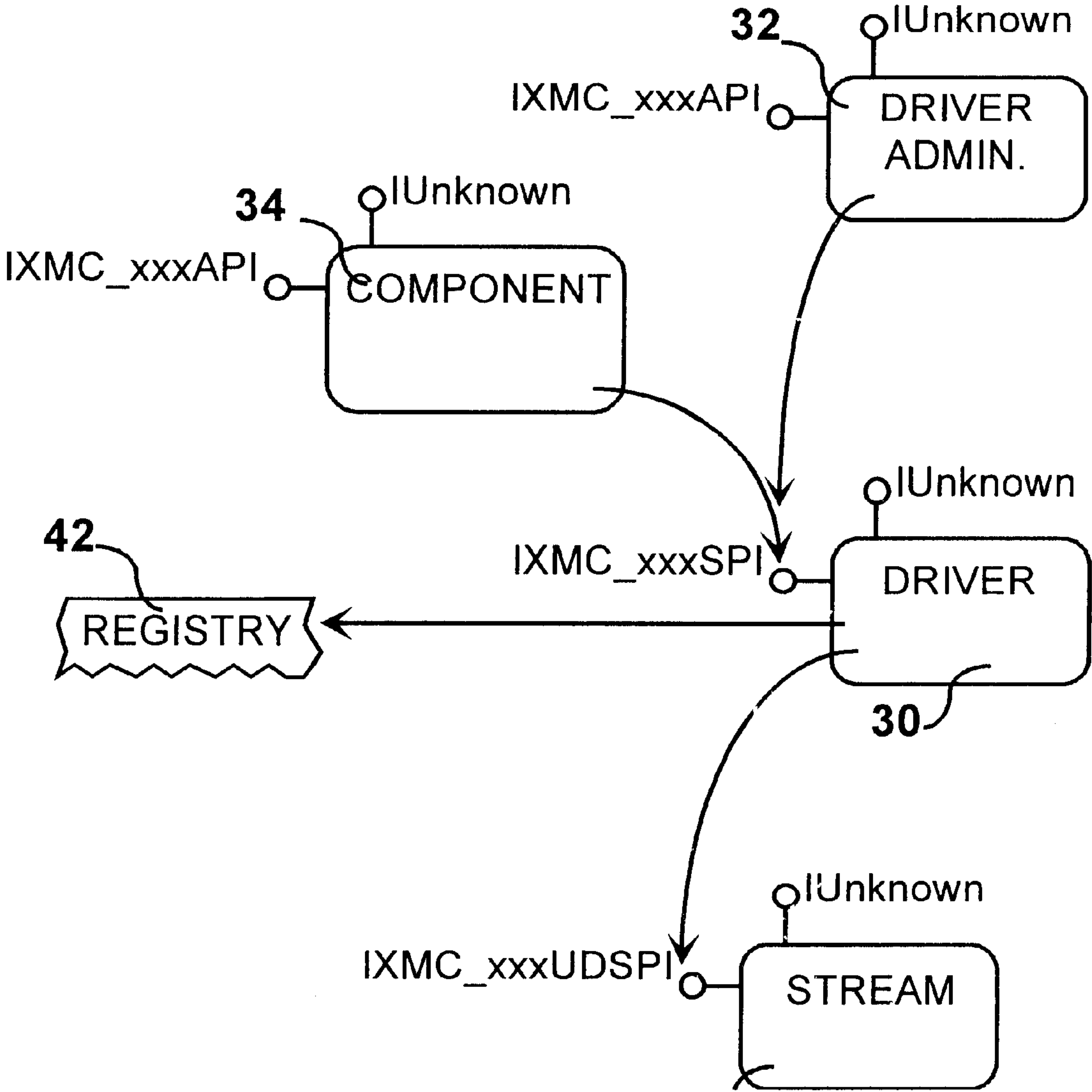
FIG. 11 Module Interaction-Map
