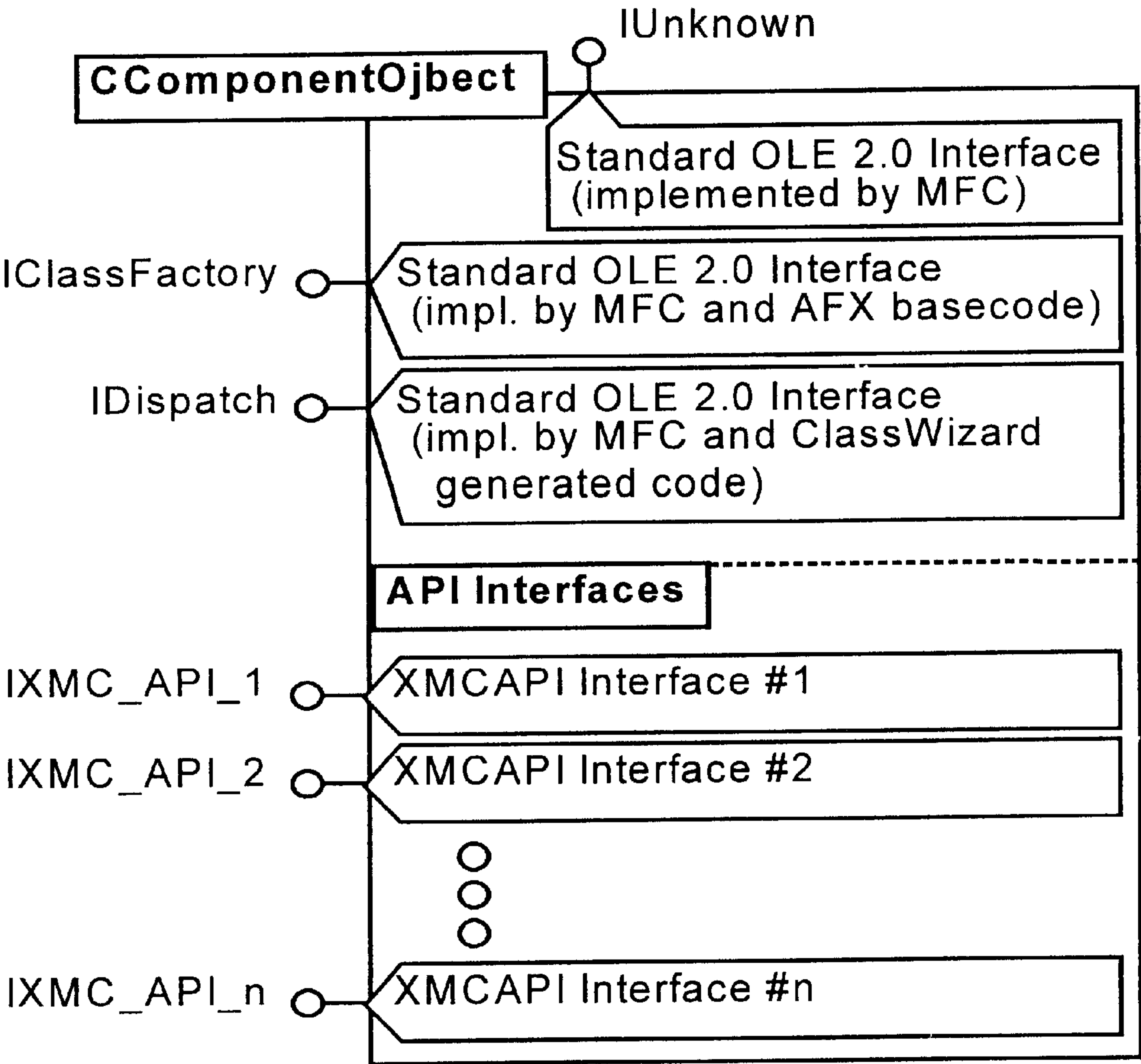
FIG. 9 Interface-Map
