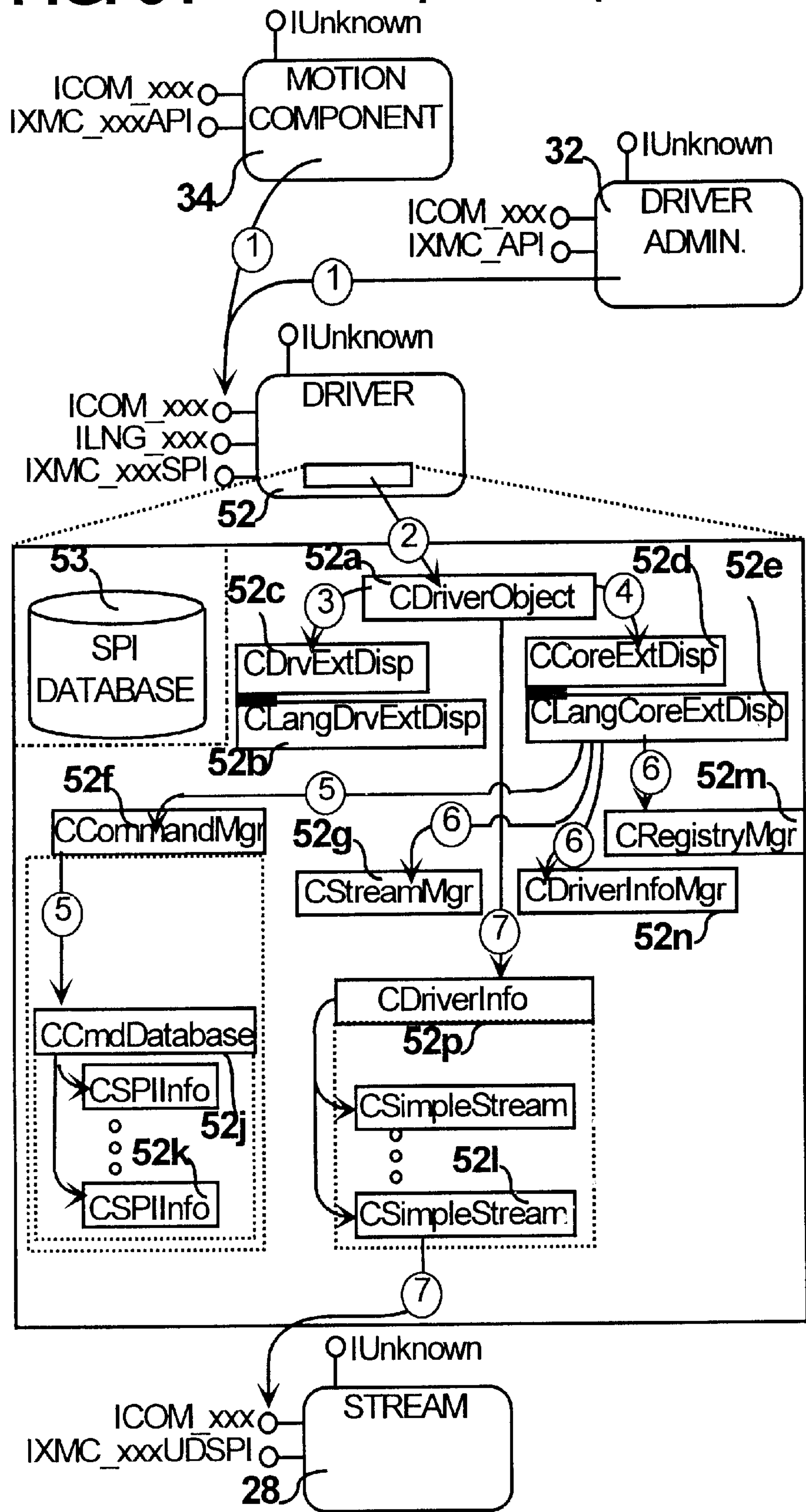
FIG. 64 Scenario-Map - Clean-up
