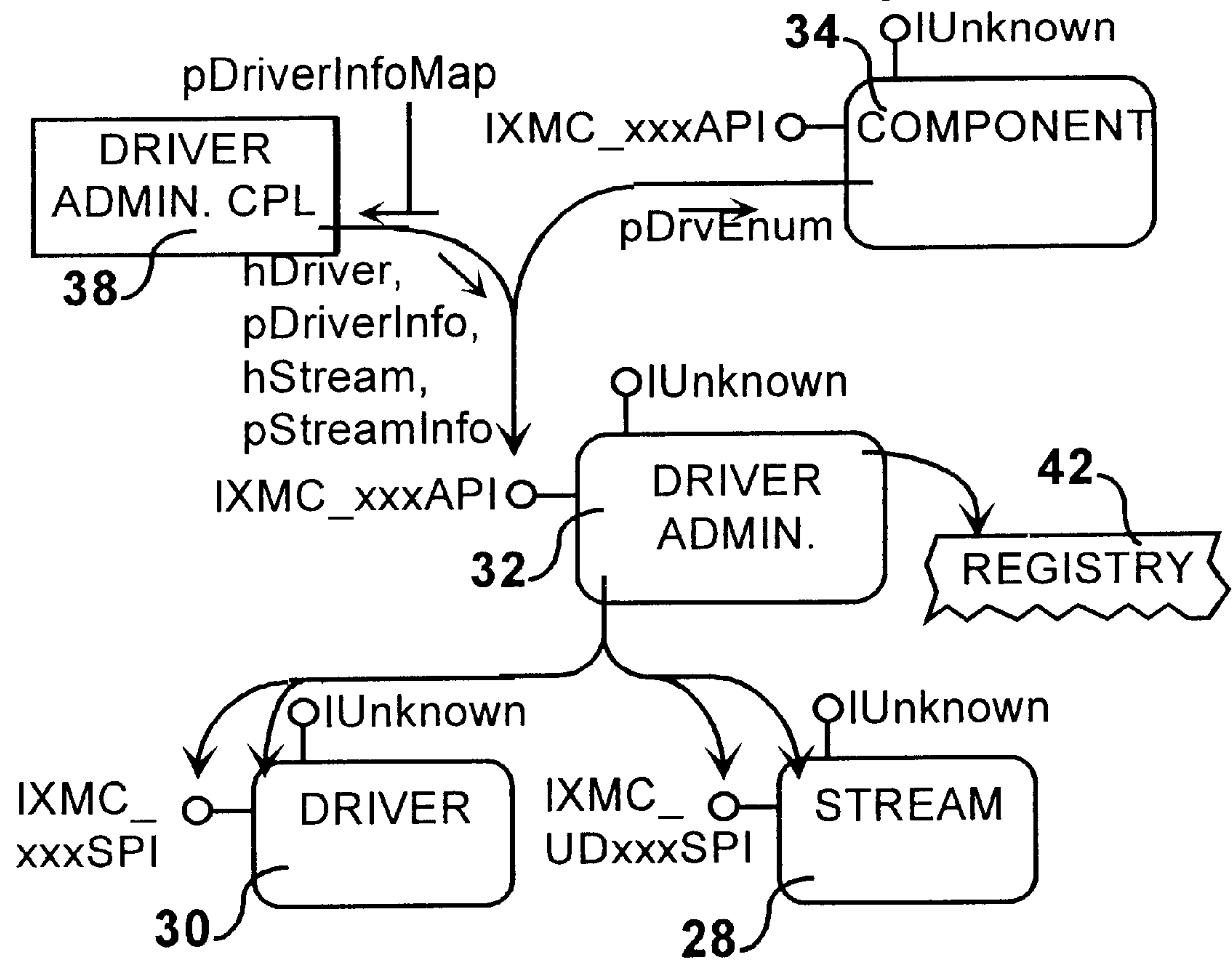
FIG. 40 Module Interaction-Map
