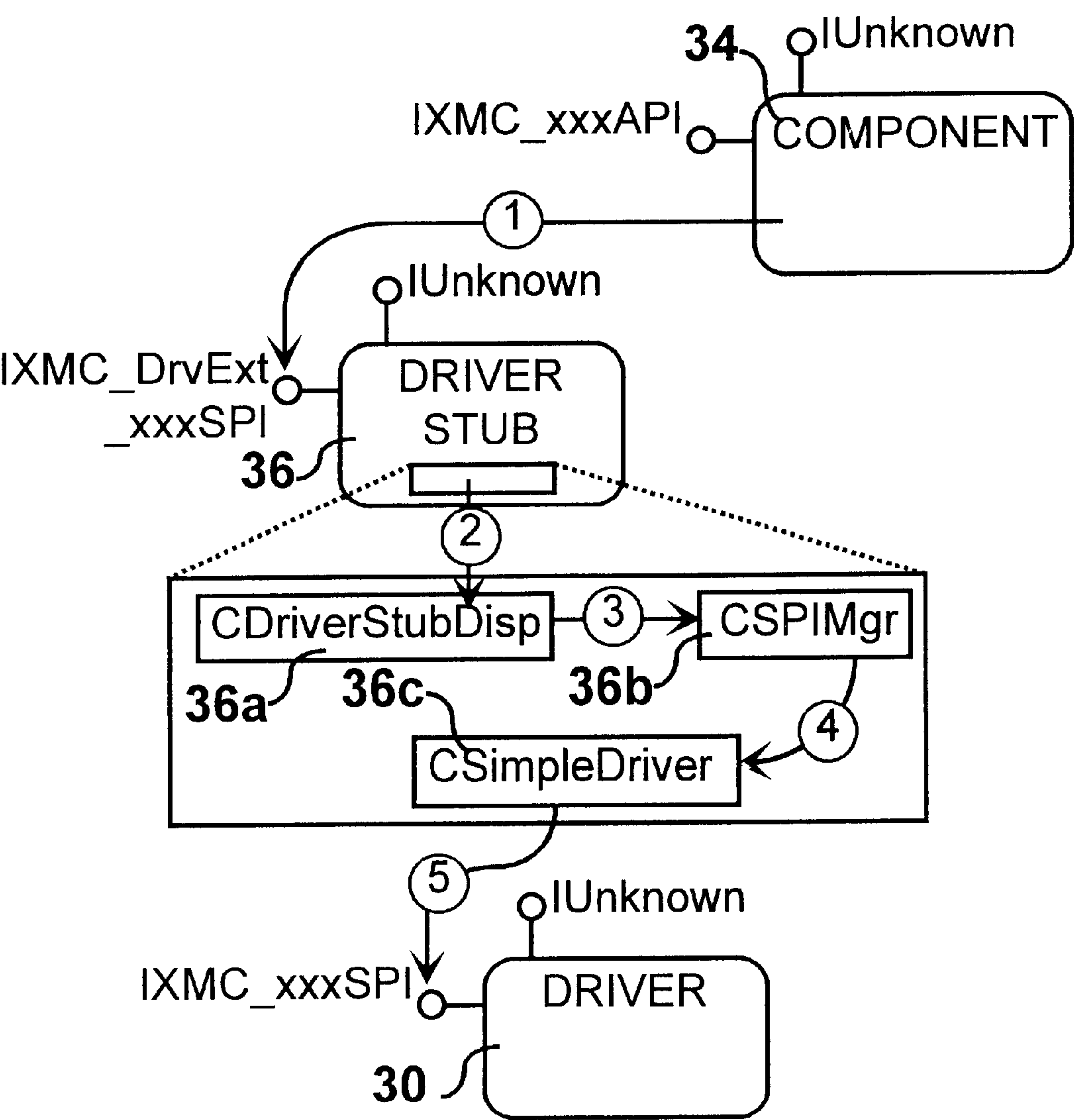
FIG. 38 Scenario-Map - Clean-up
