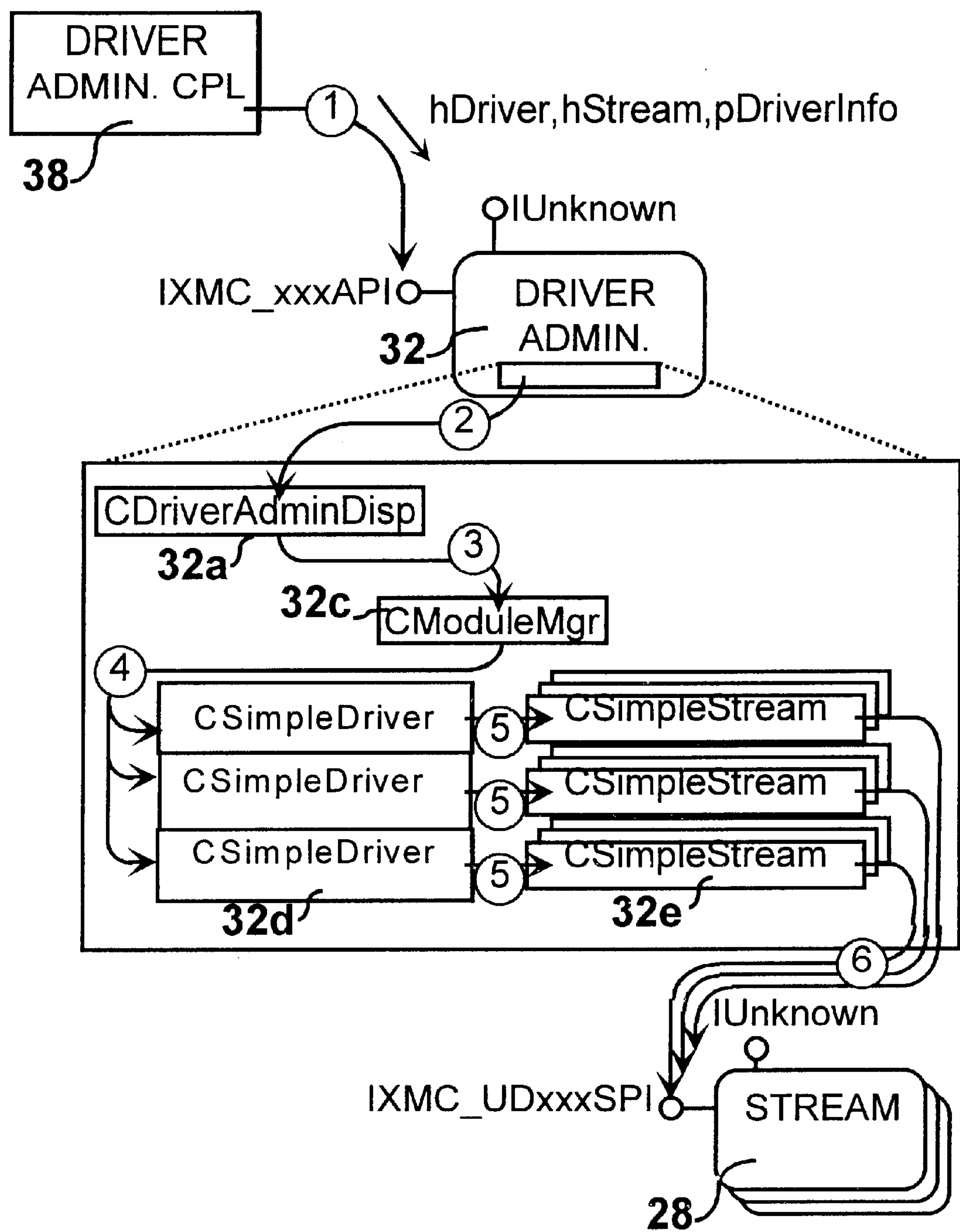
FIG. 46 Scenario-Map - Setting Stream Info.
