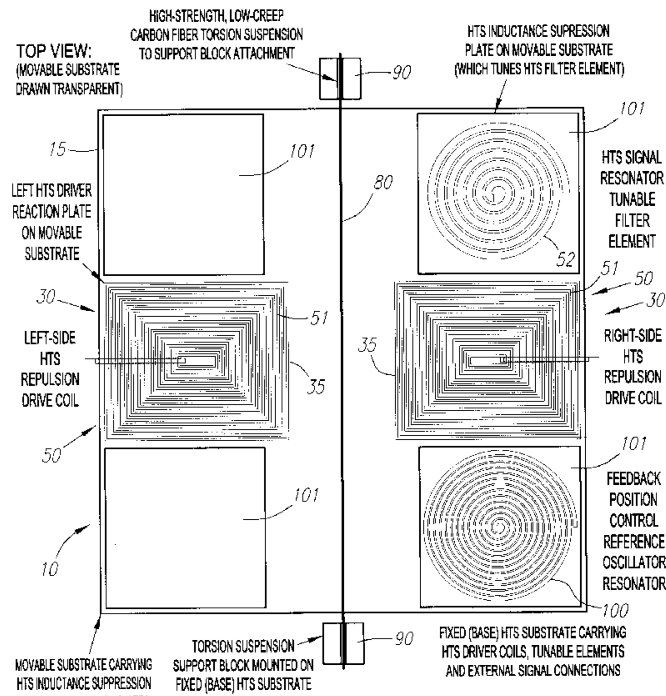
MAGNETICALLY-DRIVEN TORSIONALLY-SUSPENDED FEEDBACK-CONTROLLED ALL-HTS TUNABLE FILTER
