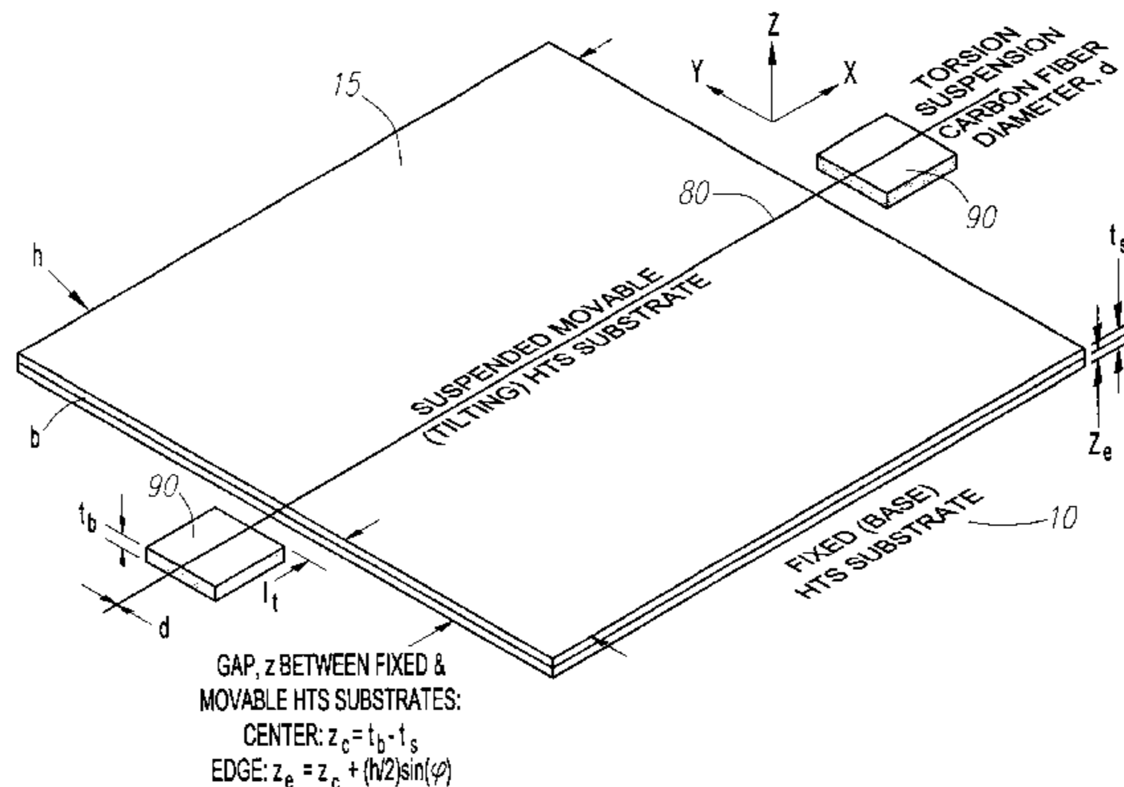
MAGNETICALLY-DRIVEN TORSIONALLY-SUSPENDED FEEDBACK-CONTROLLED ALL-HTS TUNABLE FILTER
