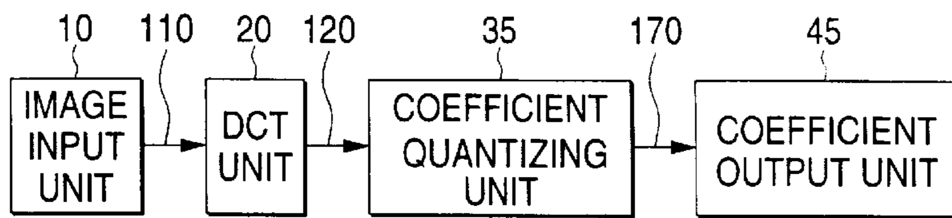
ENCODING APPARATUS
