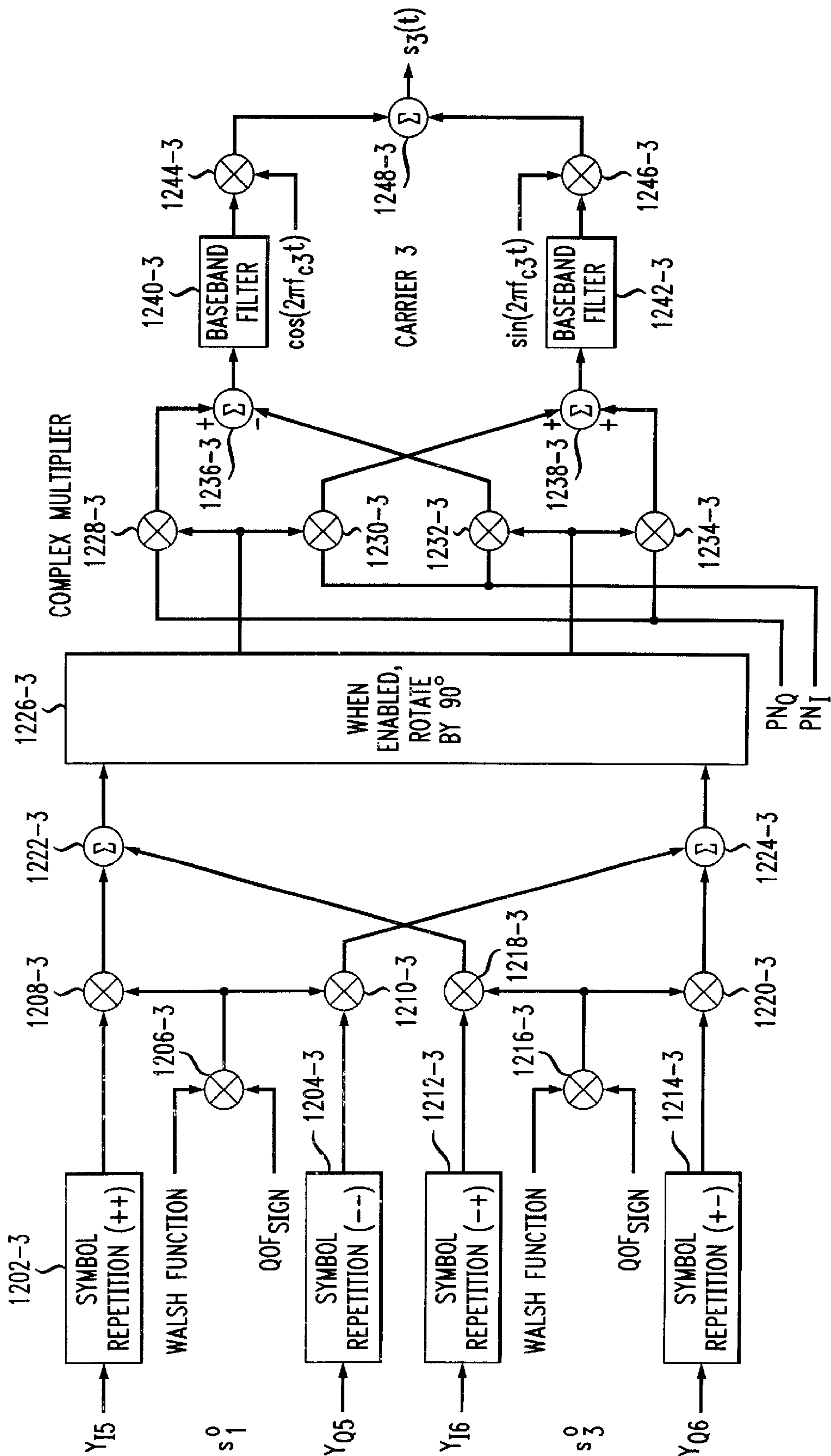
FIG. 12C P/O ANTENNA 2
