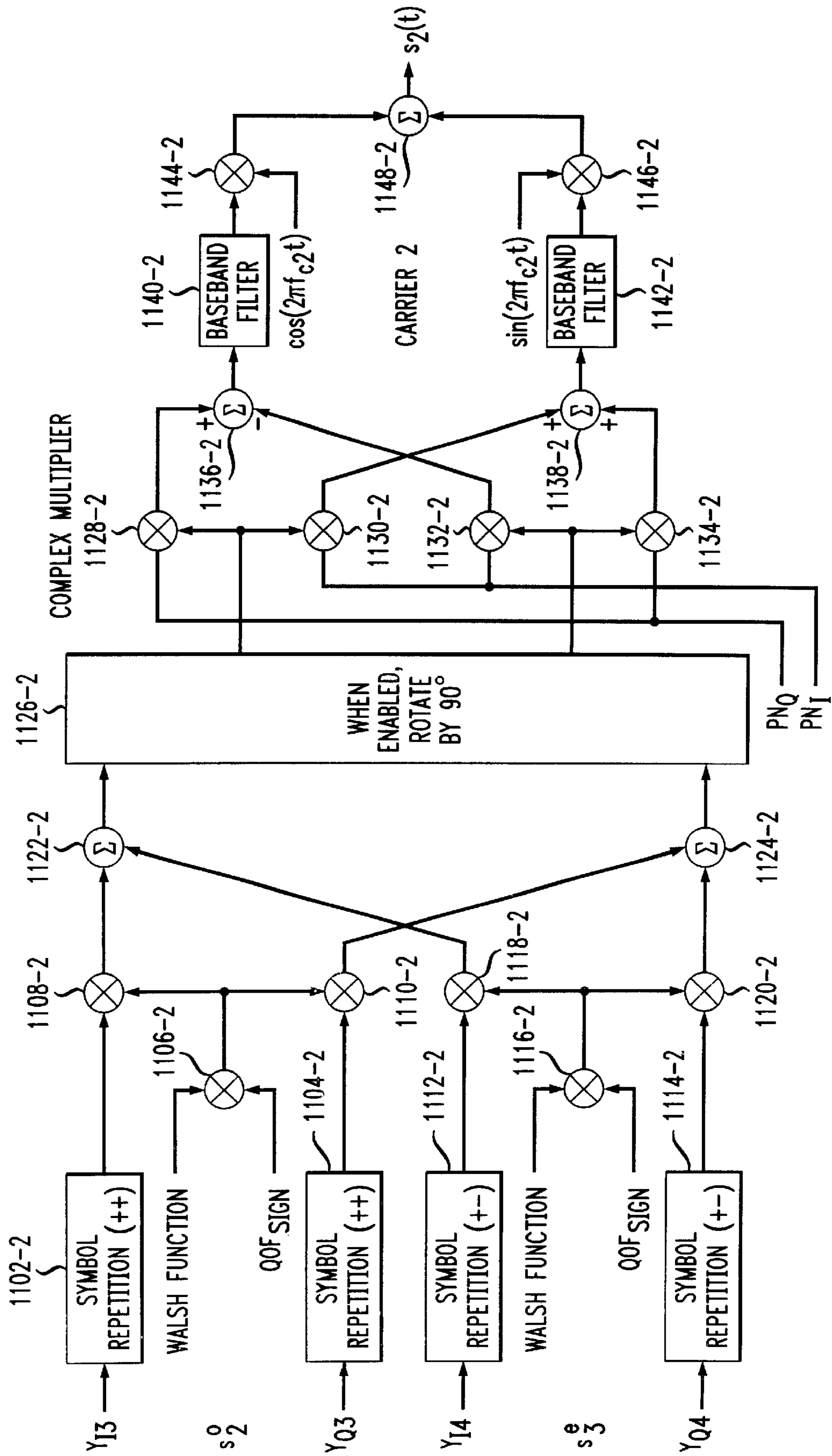
FIG. 11B P/O ANTENNA 1
