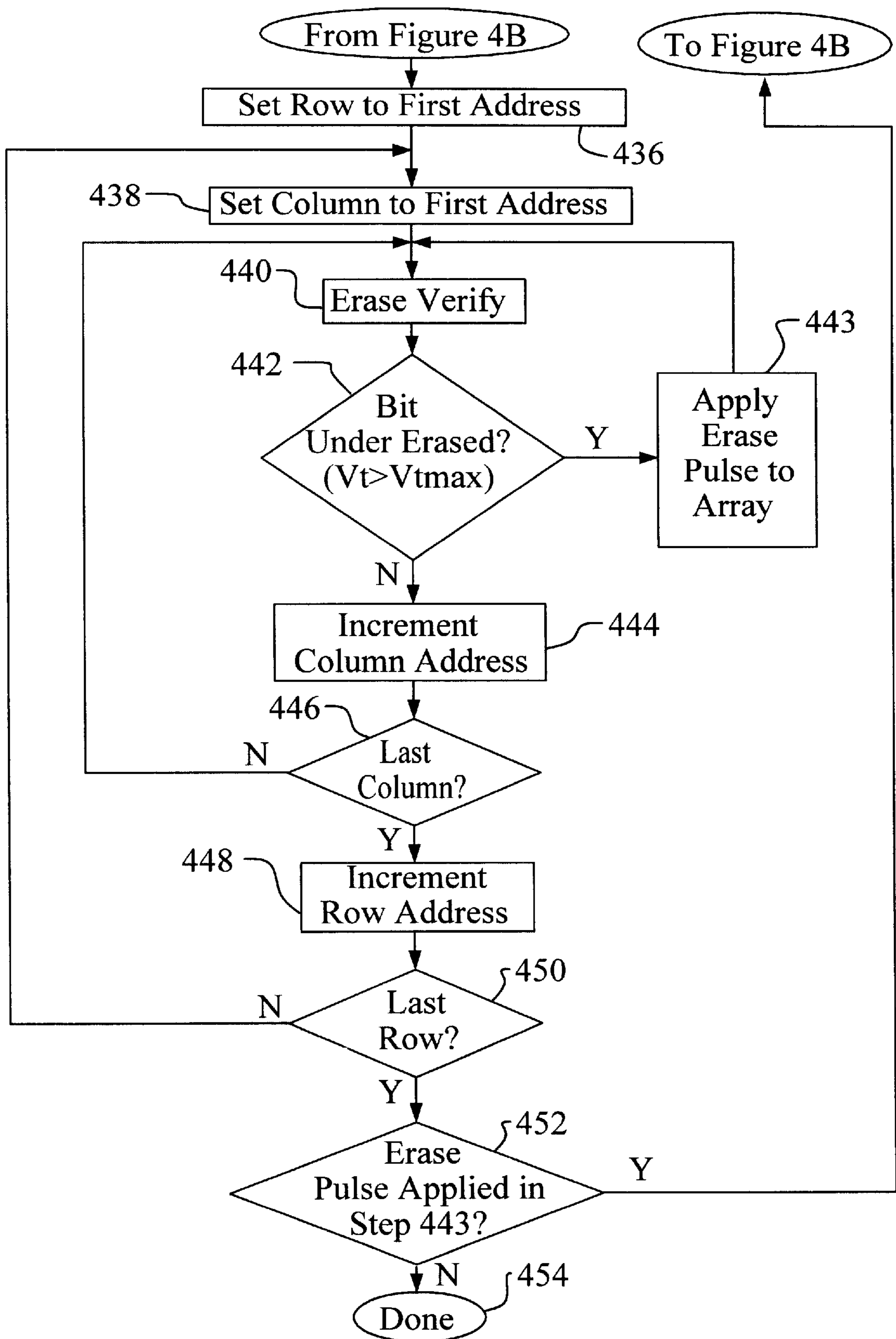
FIG. 4C Prior Art
