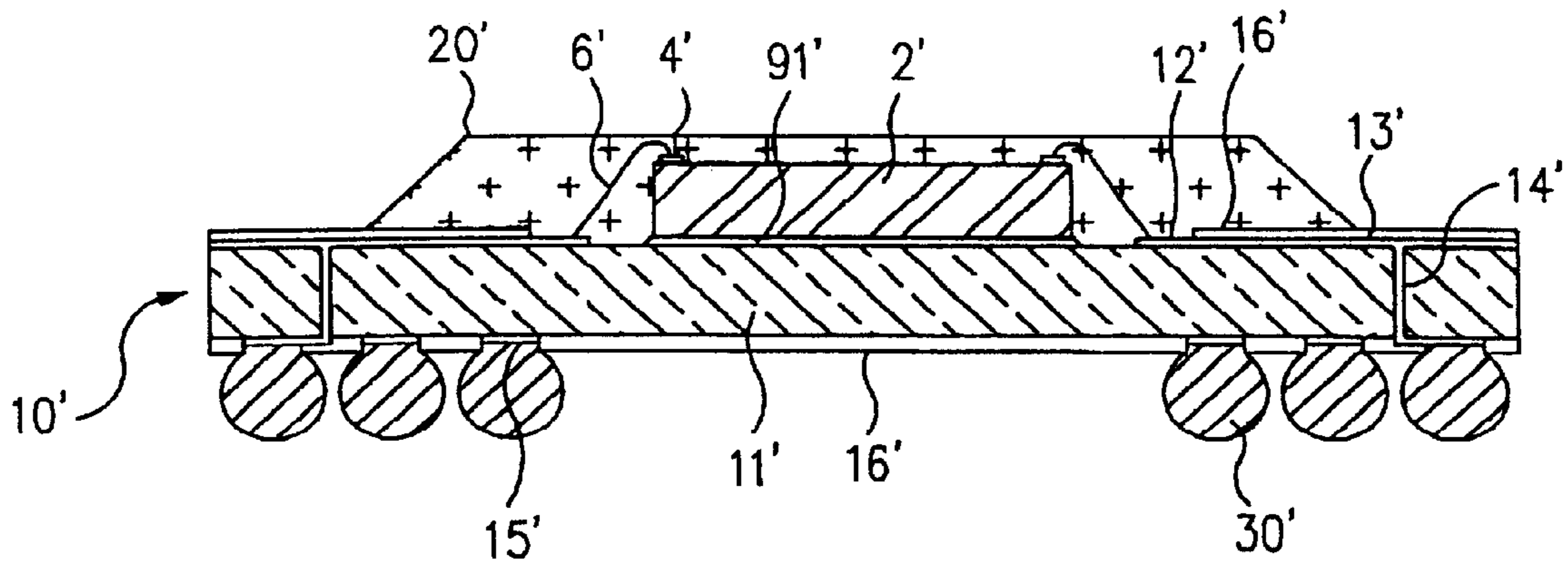
FIG. 16 (PRIOR ART)
