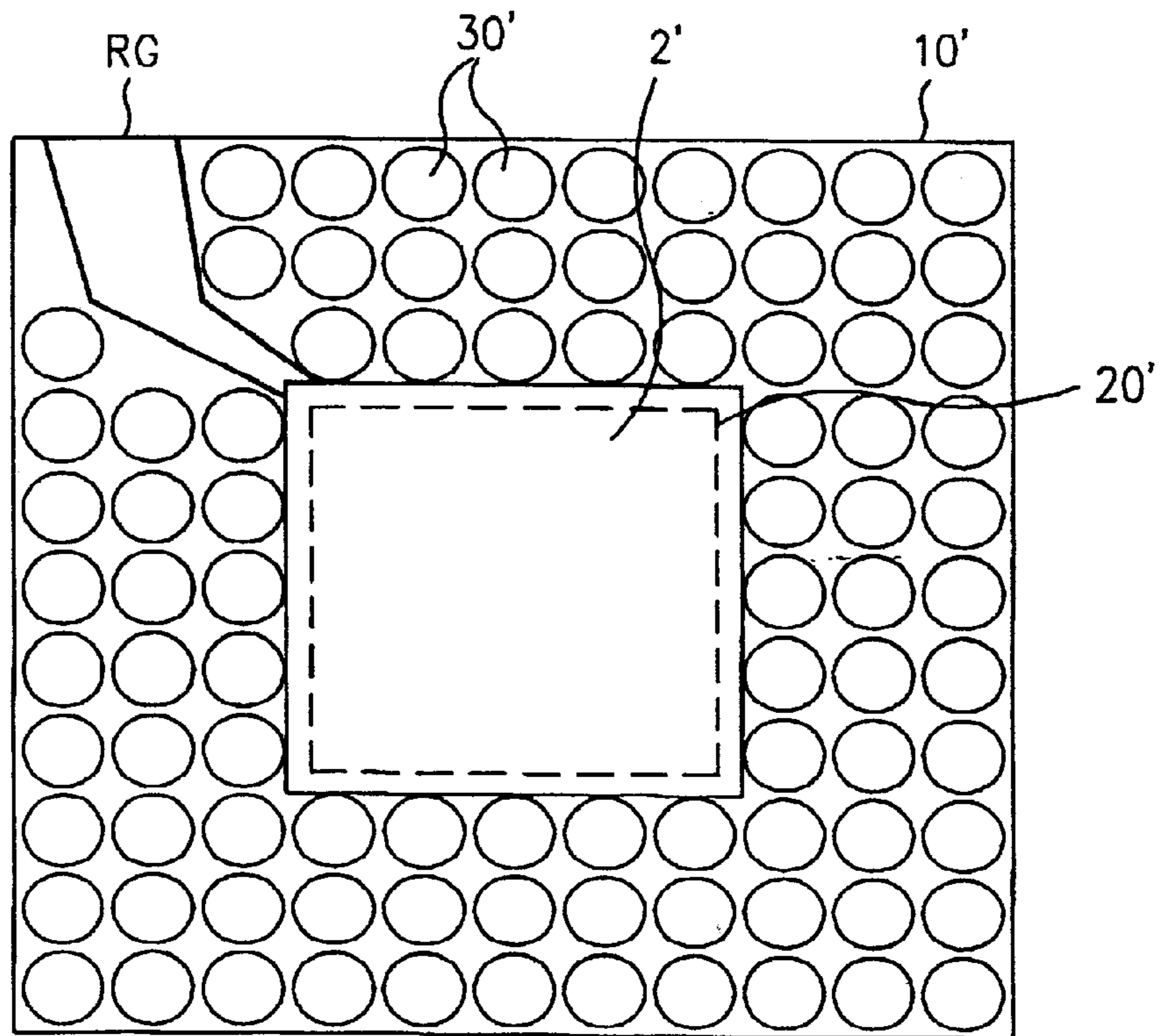
FIG. 17 (PRIOR ART)
