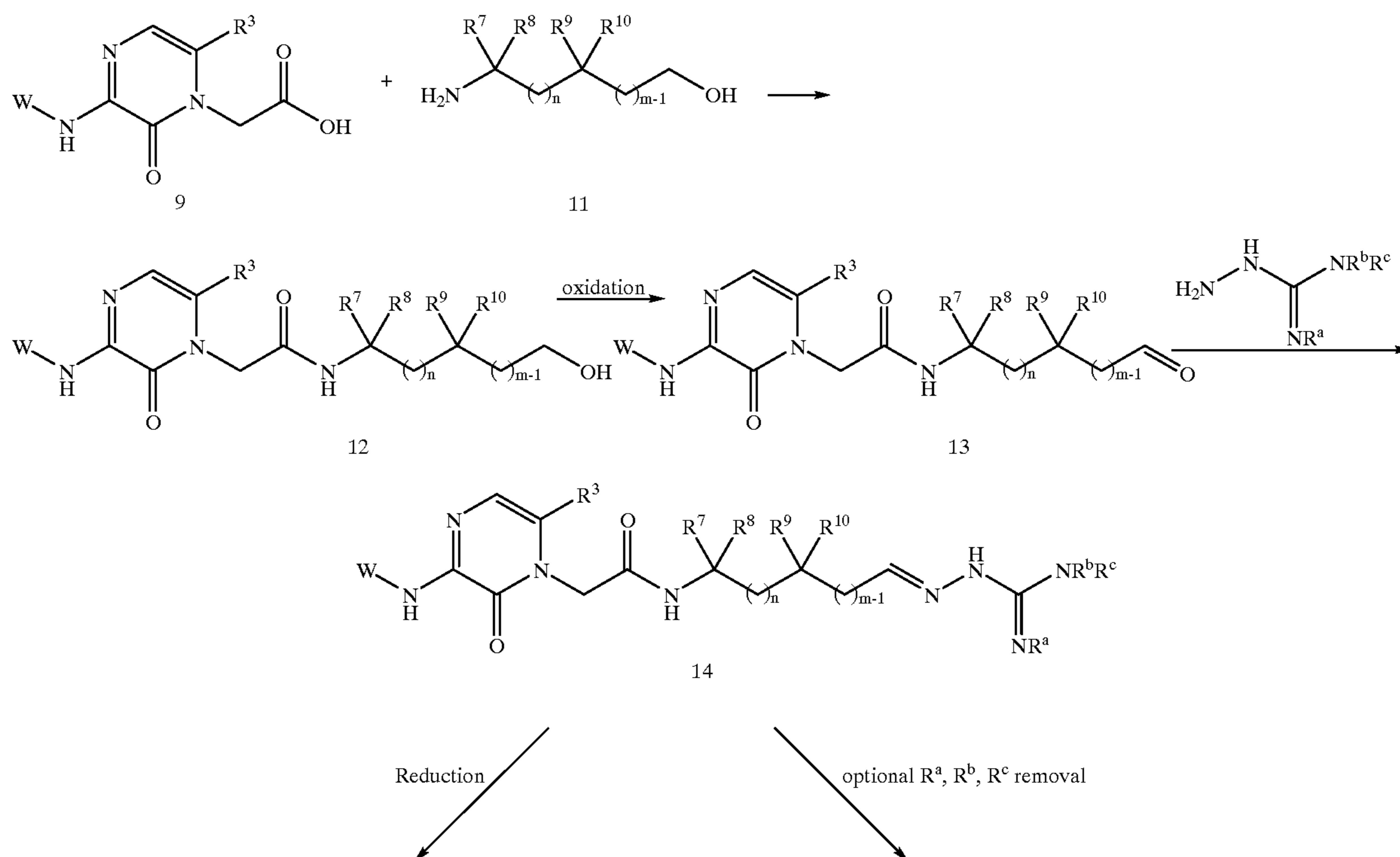
Scheme 3
