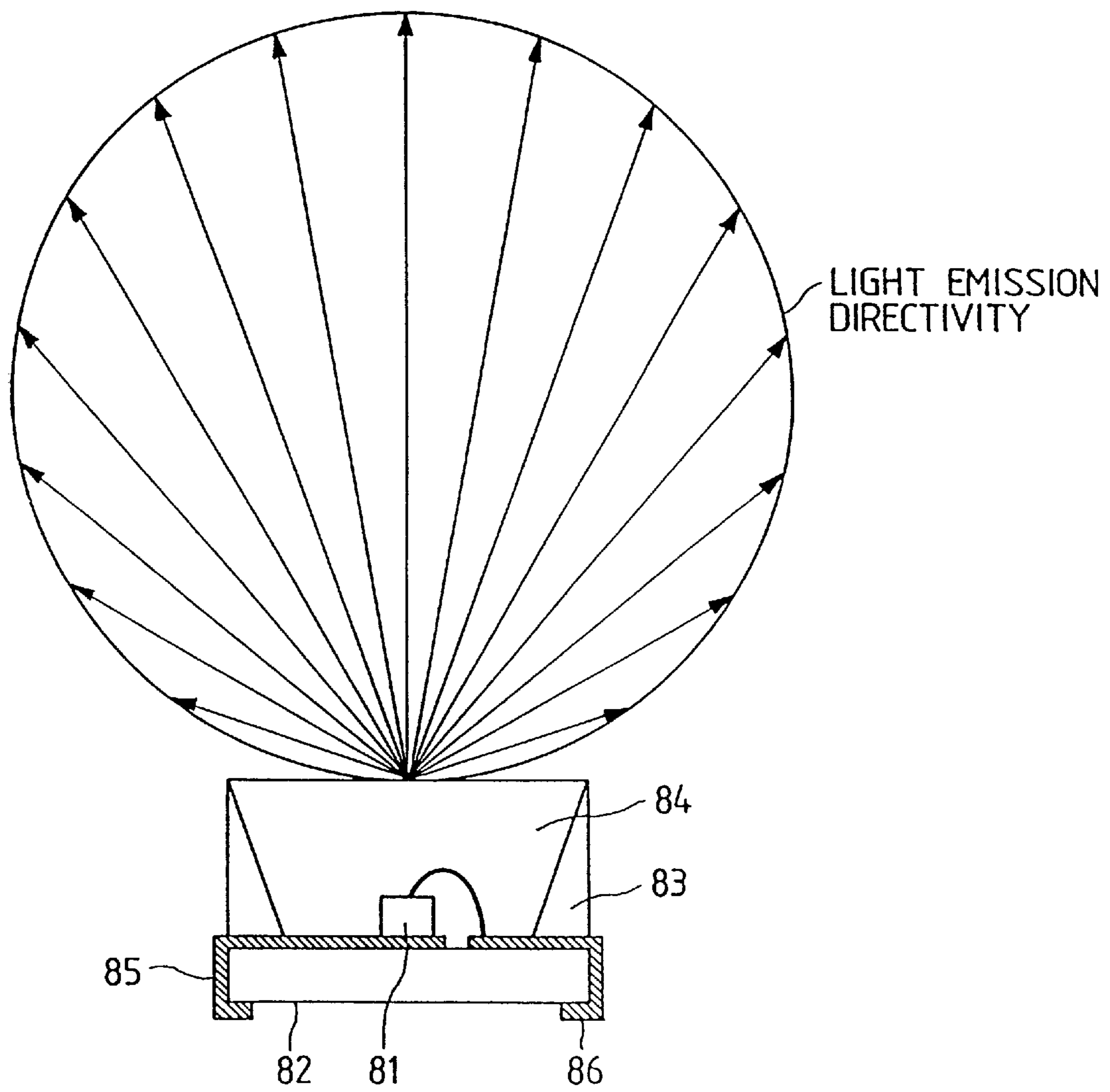
FIG. 7 PRIOR ART
