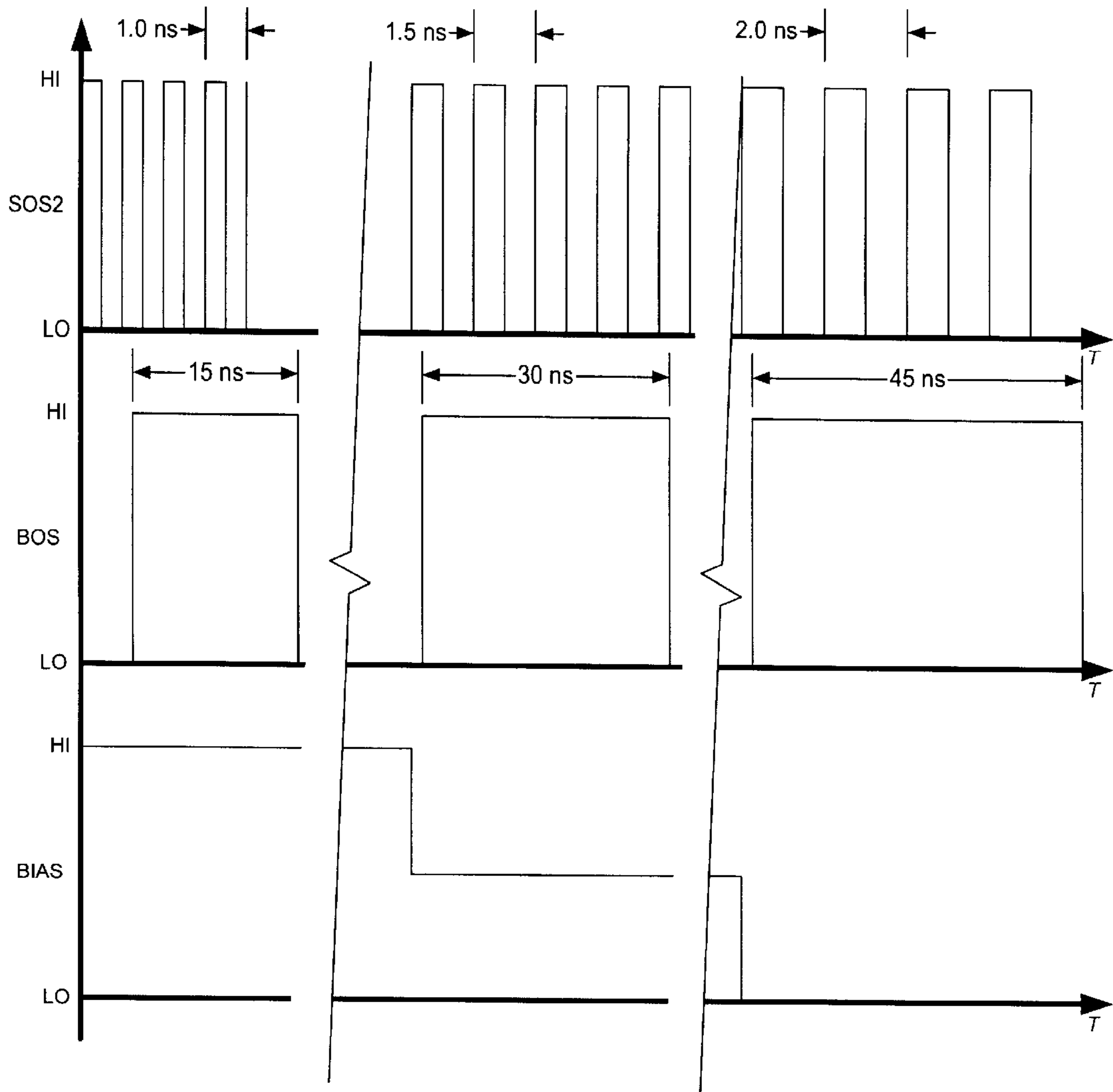
Variable Bias Control of Oscillators
