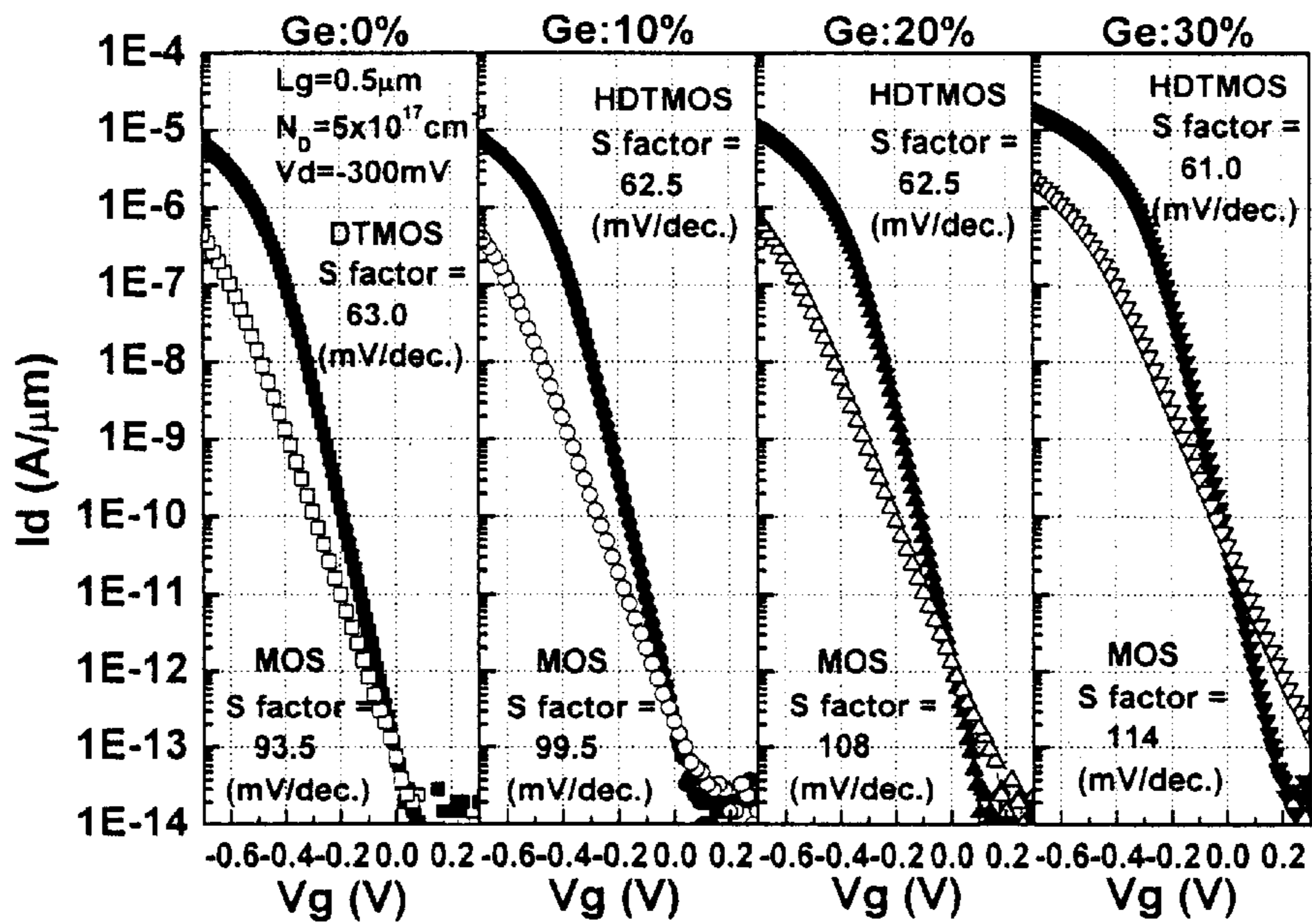
I_d - V_g characteristics
