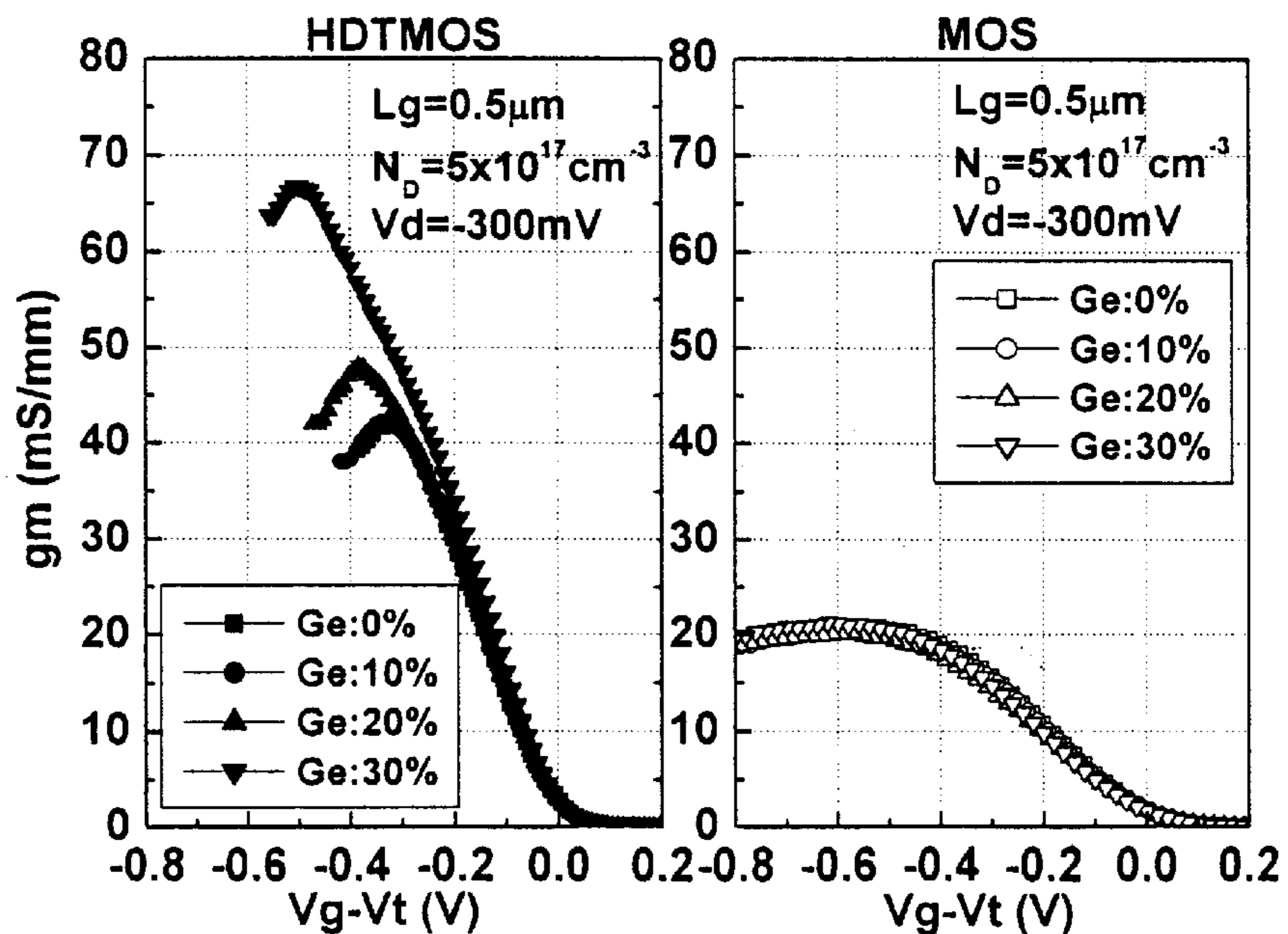
g_m - V_g characteristics
