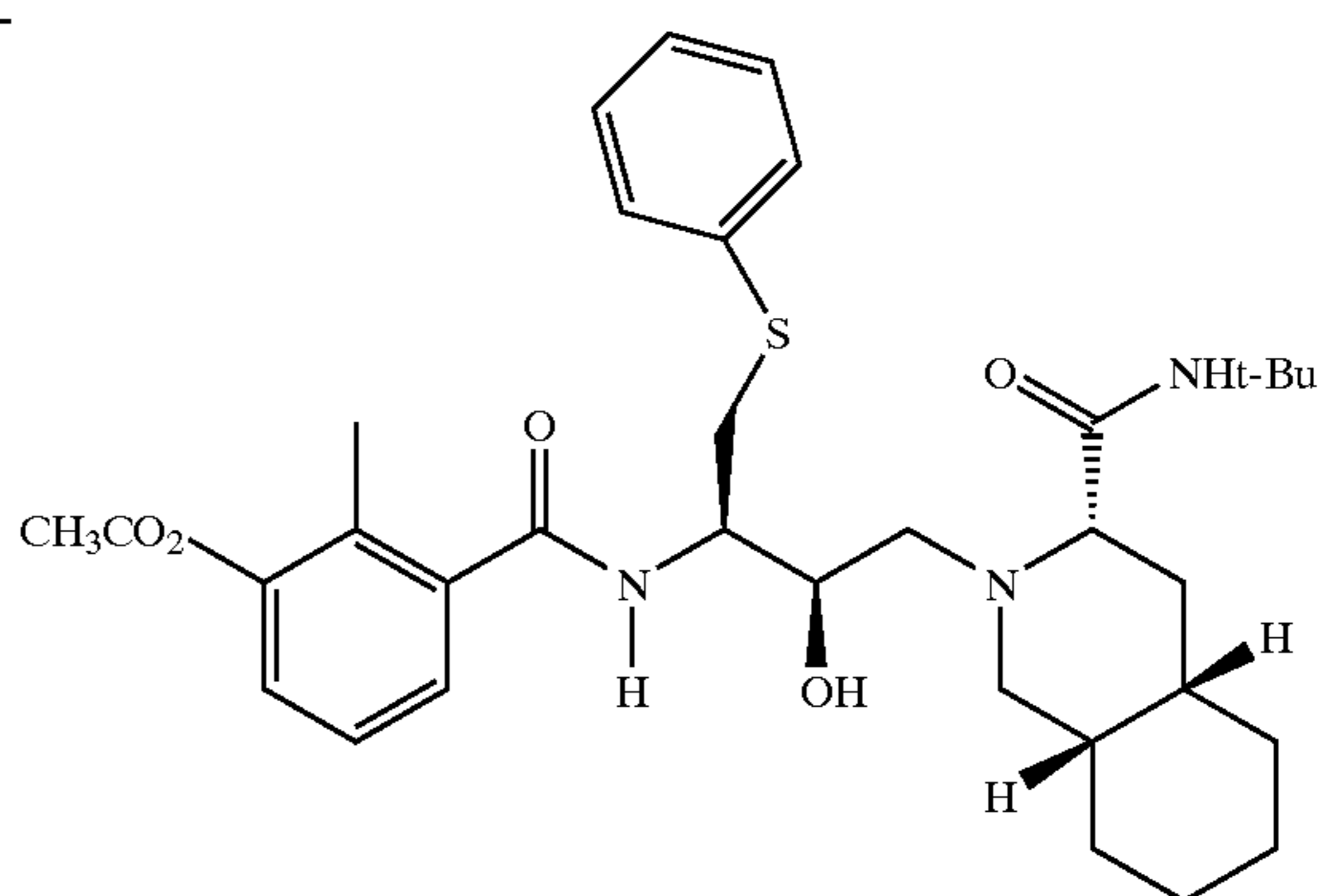
C_{34}H_{47}N_3O_3S 609.83
