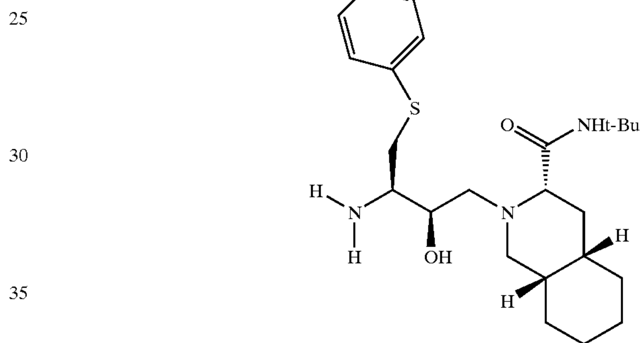
6 C_{24}H_{39}N_3SO_3 433.65
