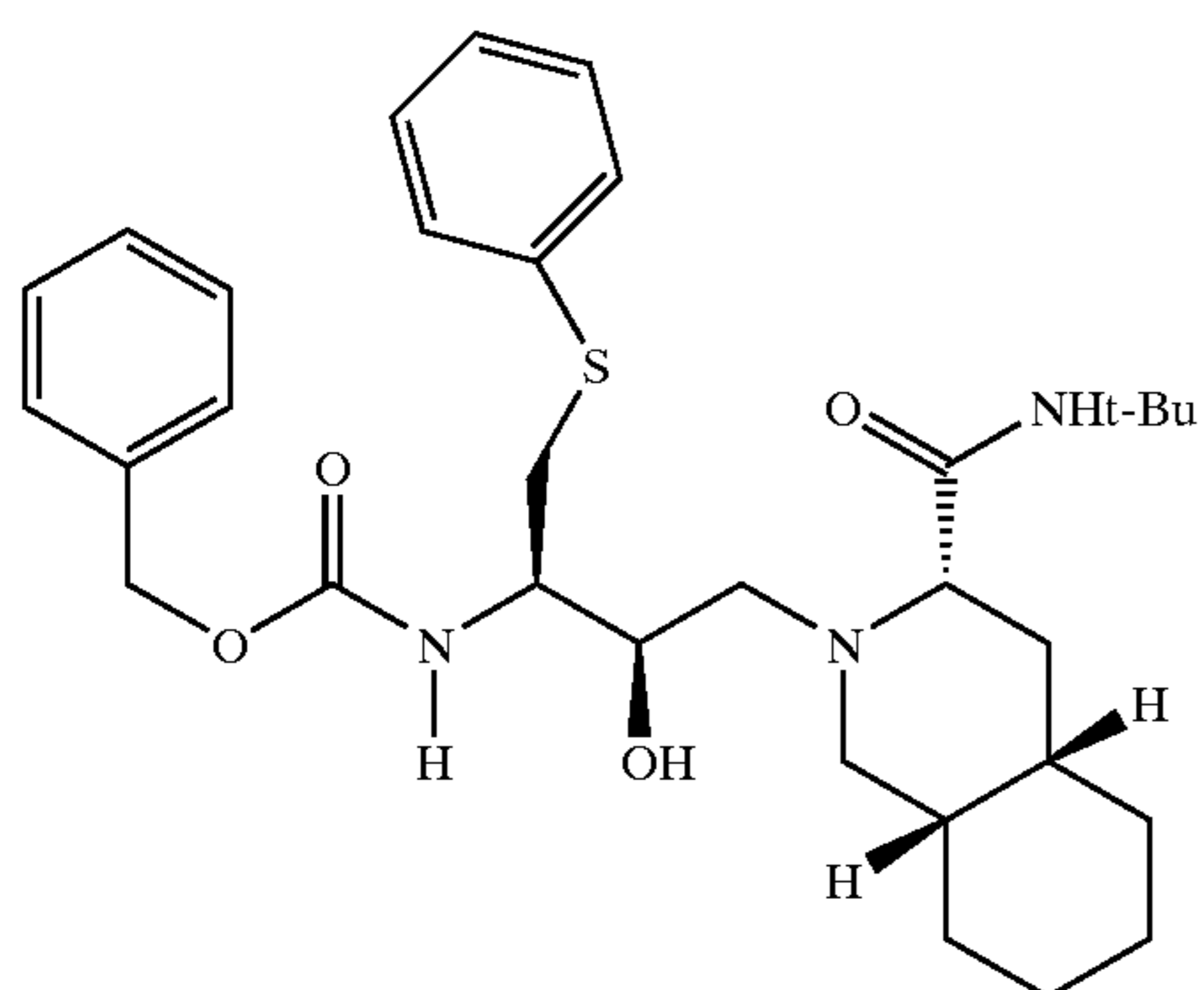
5 C_{32}H_{45}N_3O_4S 567.79
