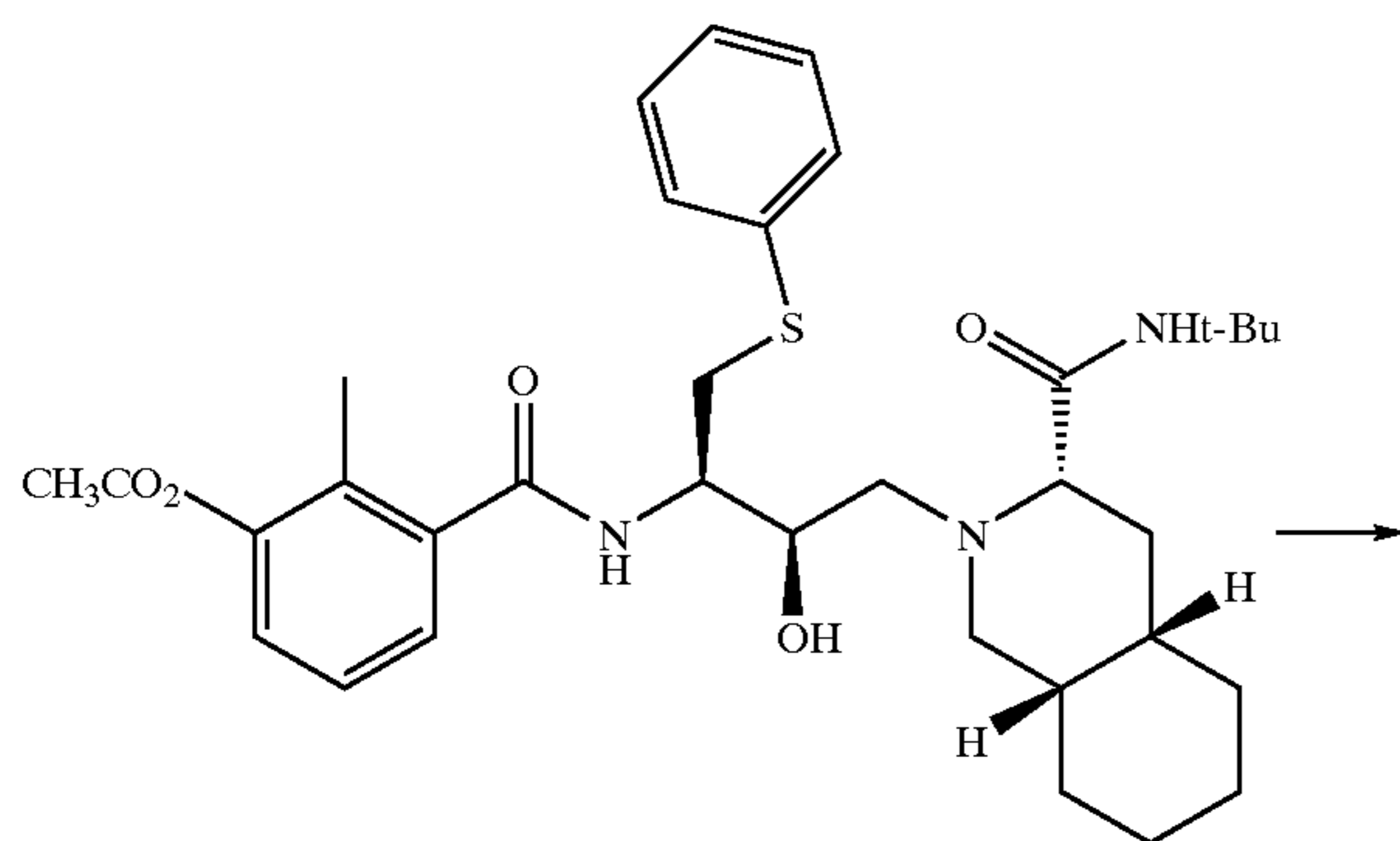
Acetate of Compound 4 C_{36}H_{47}N_3O_5S 609.83
