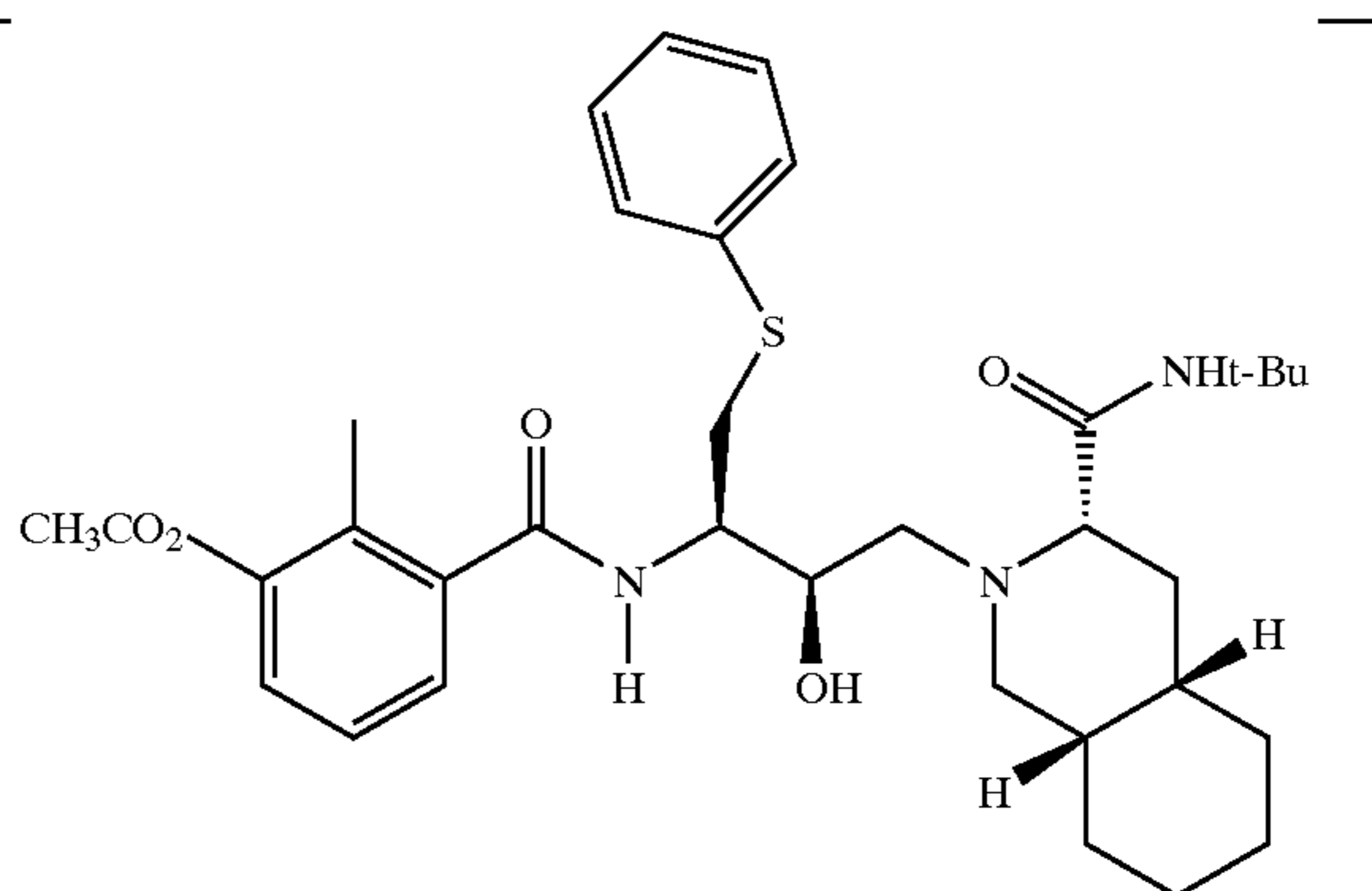
C_{34}H_{47}N_3O_3S 609.83
