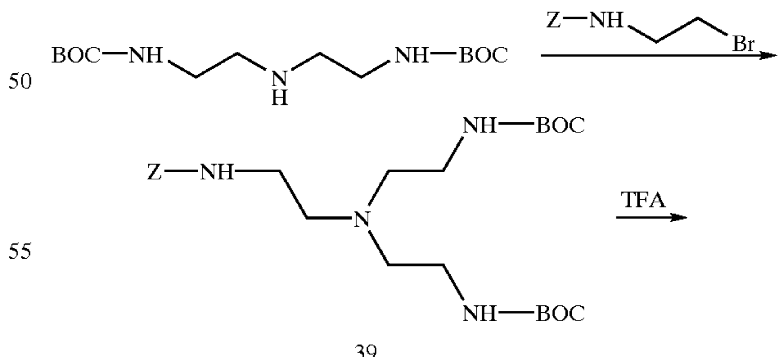
SCHEME VII SYNTHESIS OF 46
