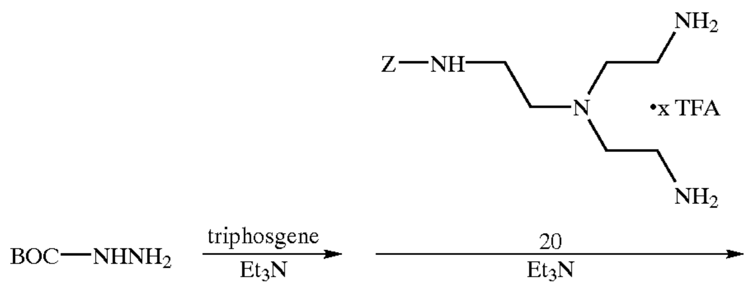
SCHEME VI SYNTHESIS OF 38
