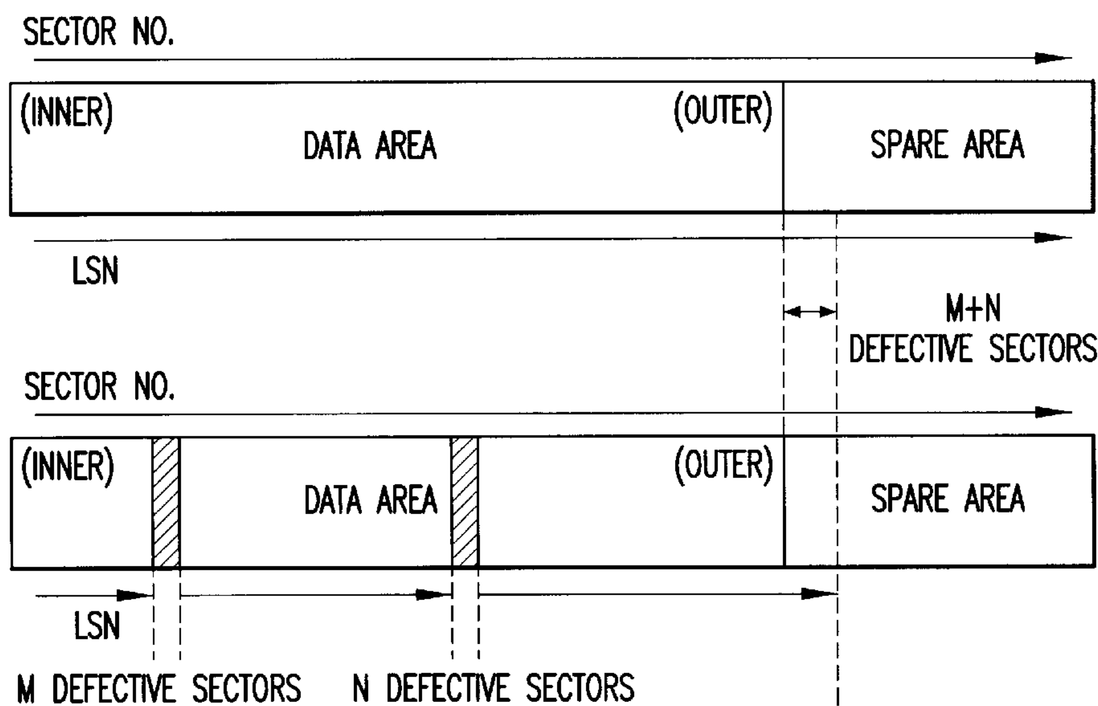
FIG.2 CONVENTIONAL ART
