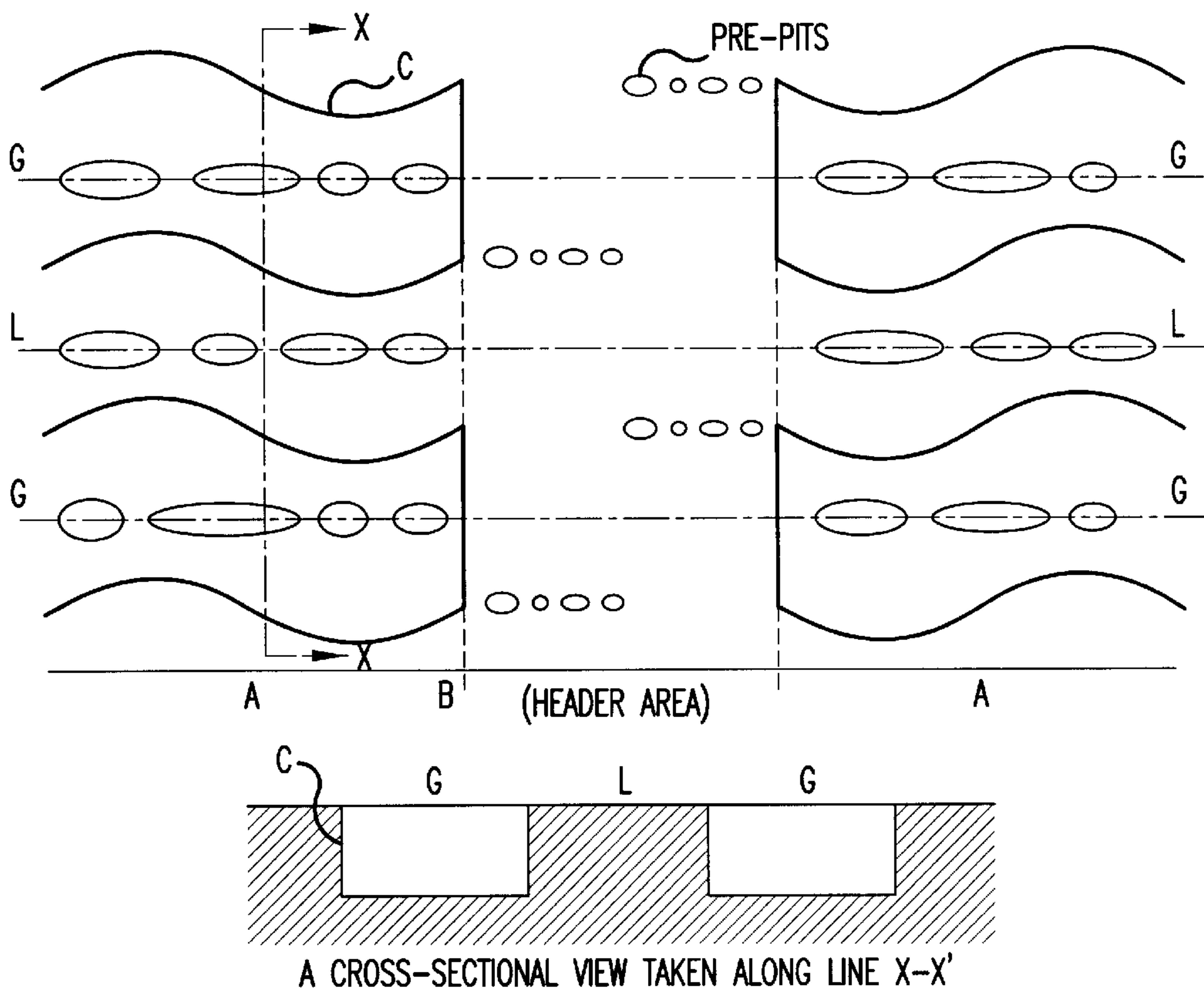
FIG. 4 CONVENTIONAL ART
