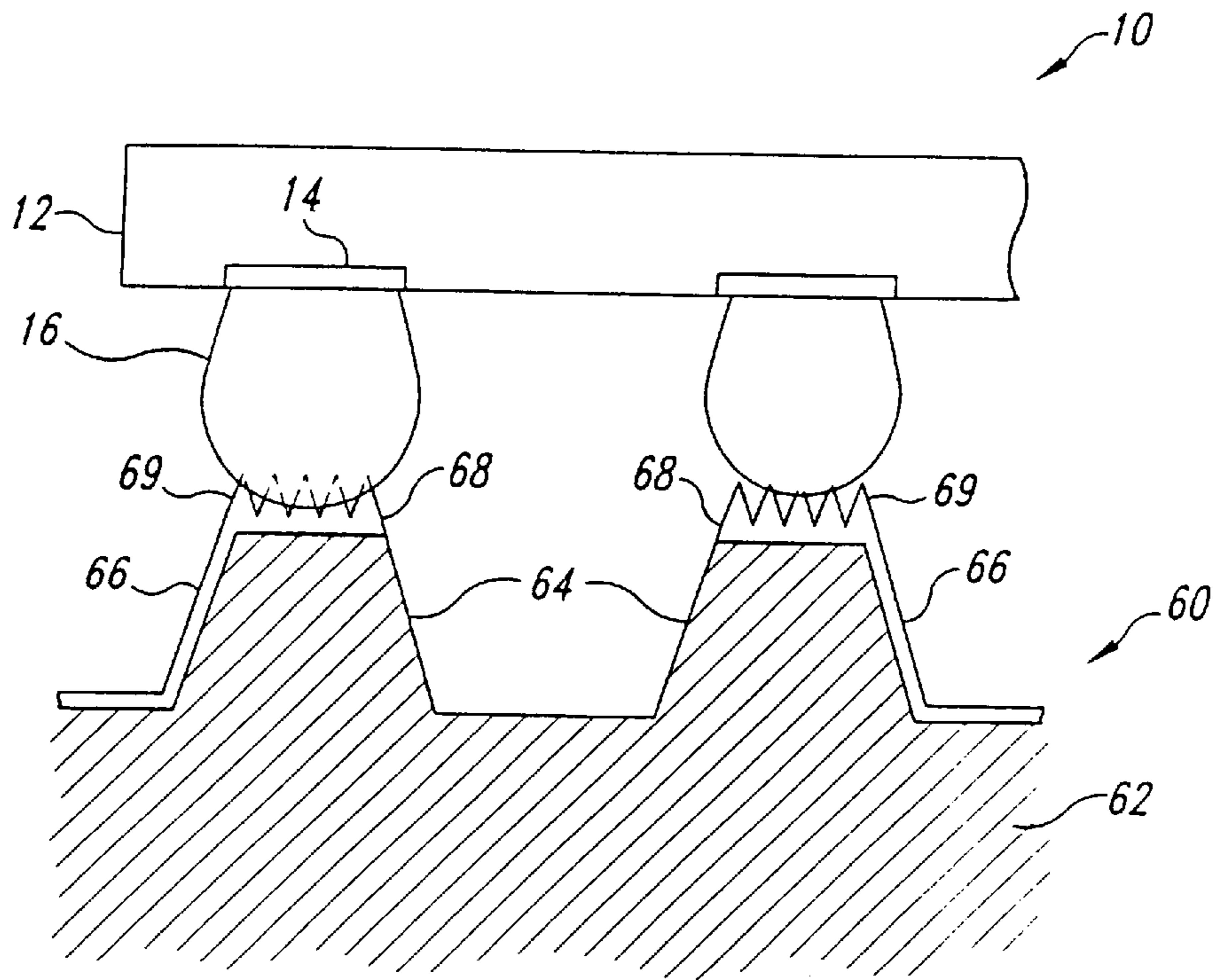
Fig. 3 (Prior Art)
