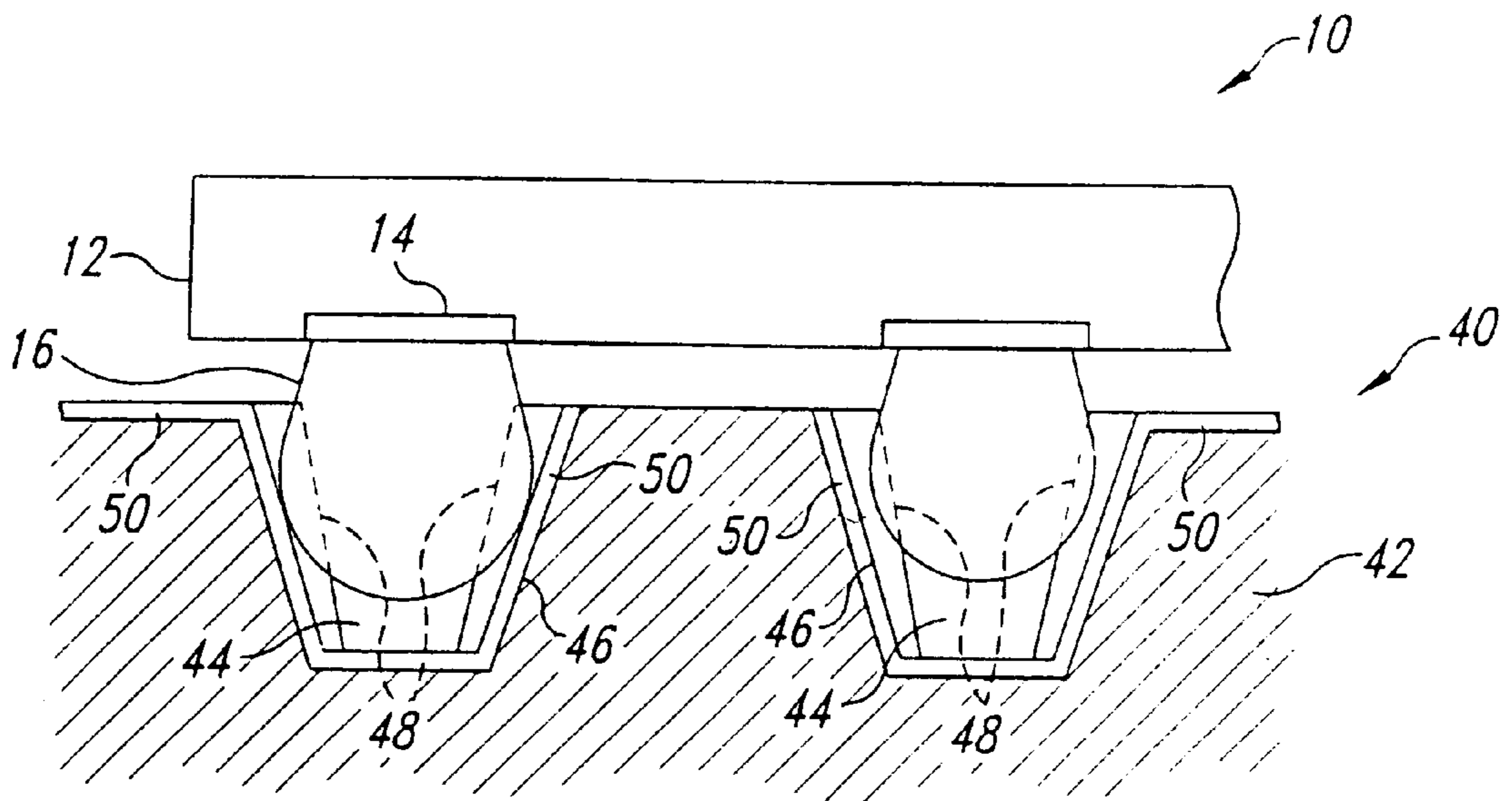
Fig. 2 (Prior Art)
