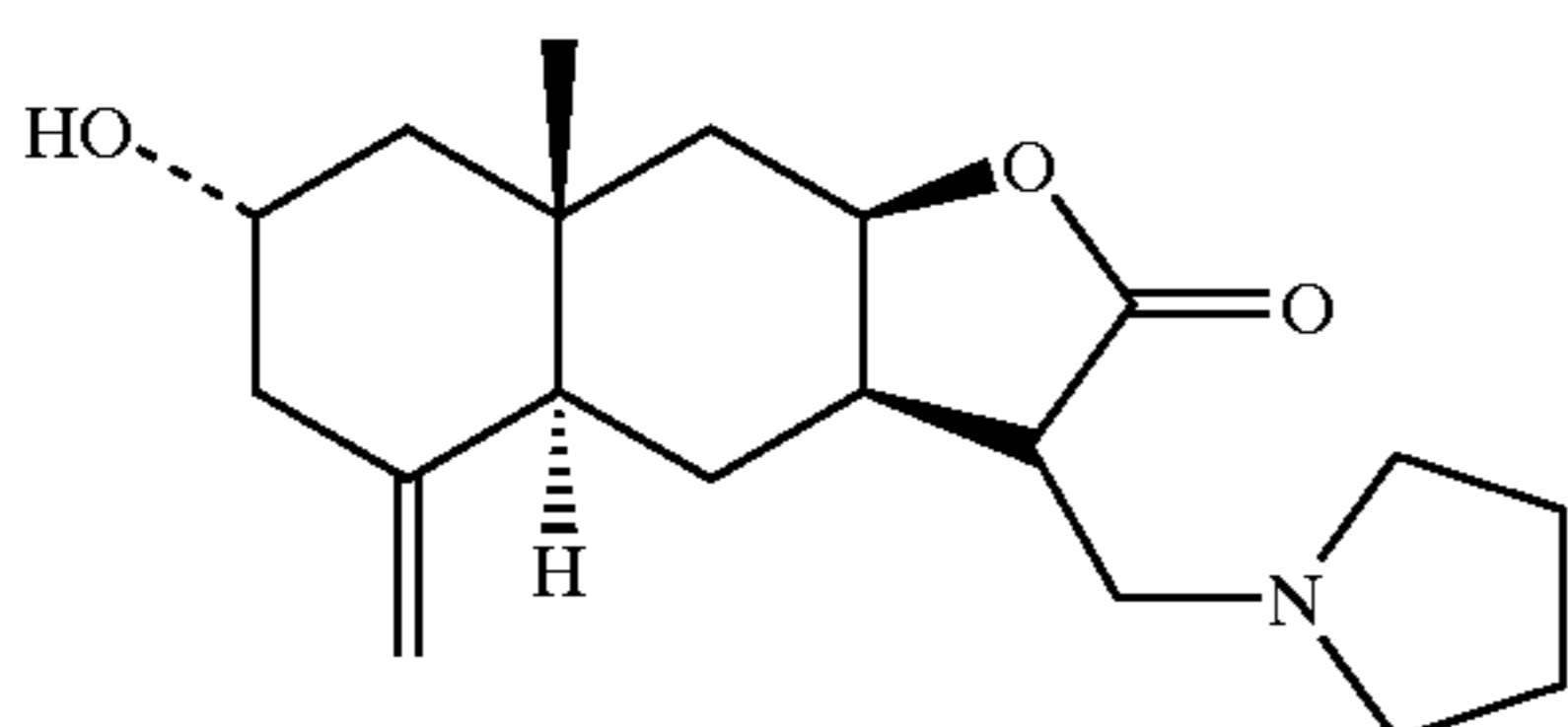
1-[2α-benzoyloxy-11,12-dihydro-5,7,8αH-eudesm-4(15)-en-8,12-olidyl]-pyrrolidine
