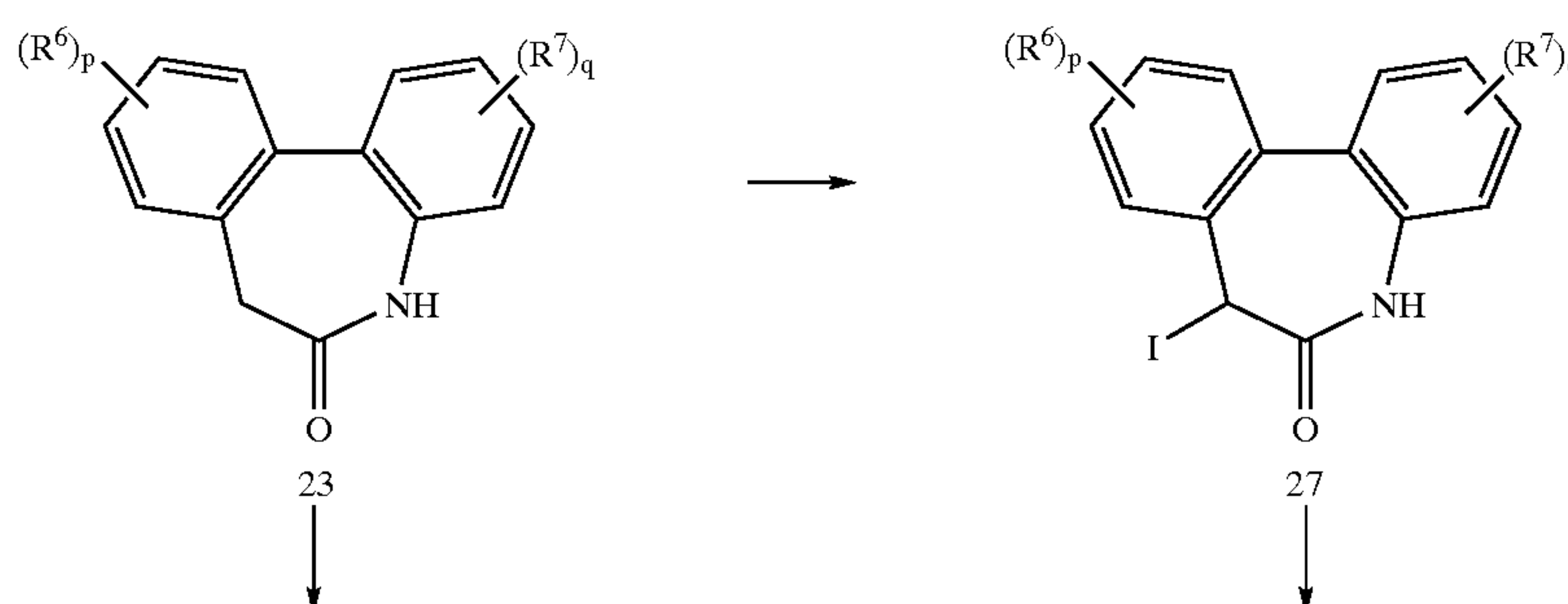
Scheme 8
