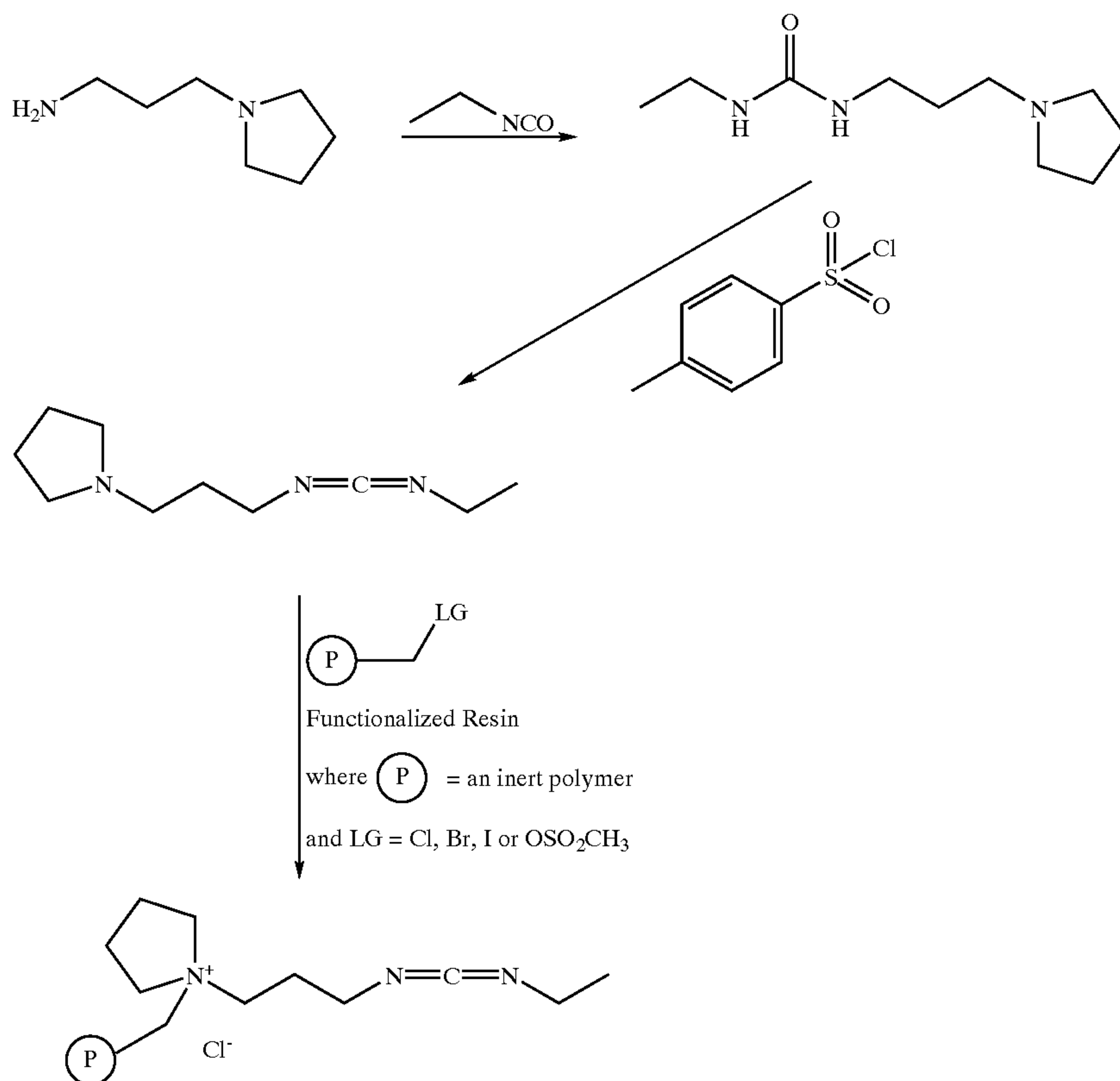
Scheme 6
