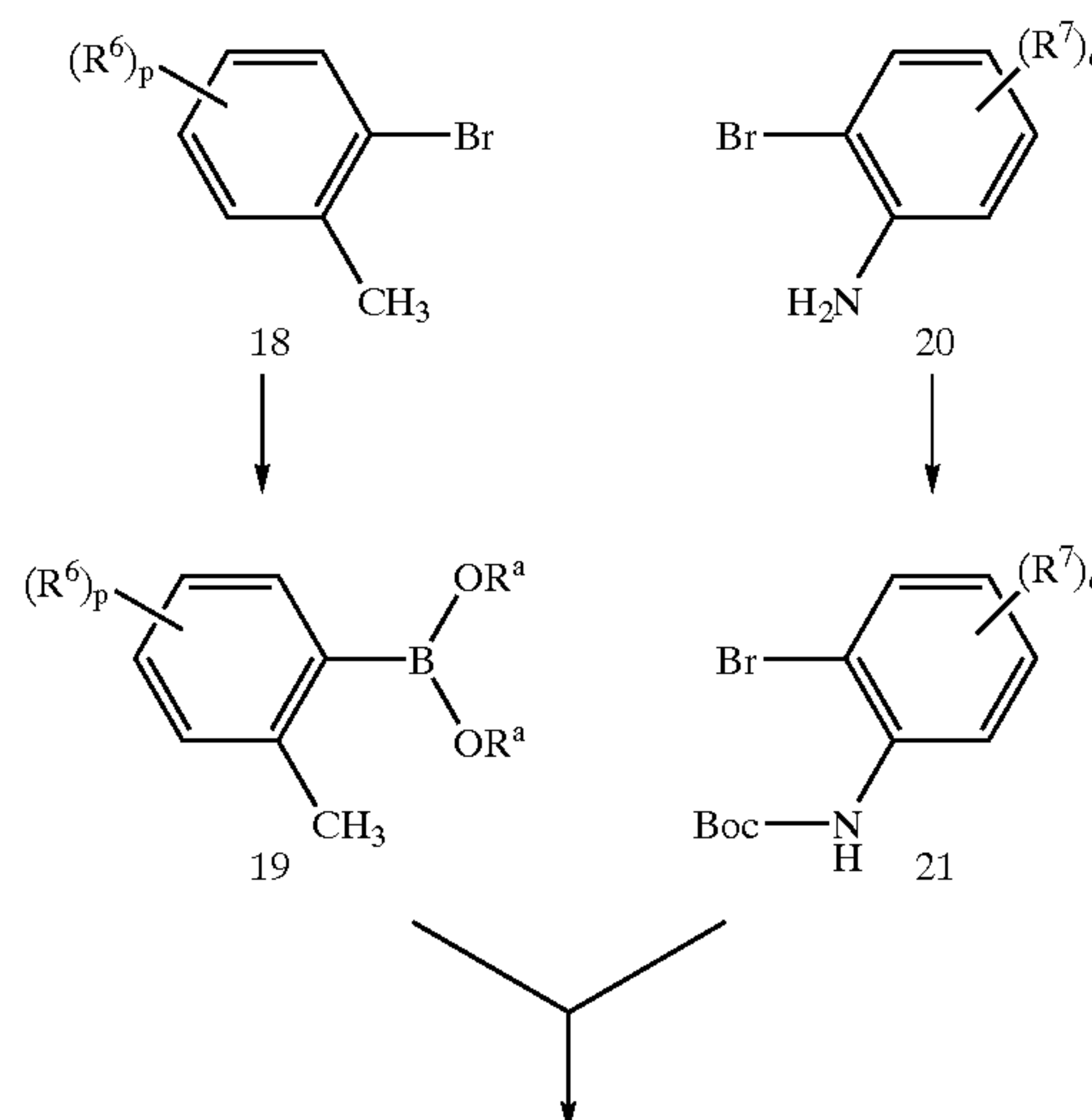
Scheme 7
