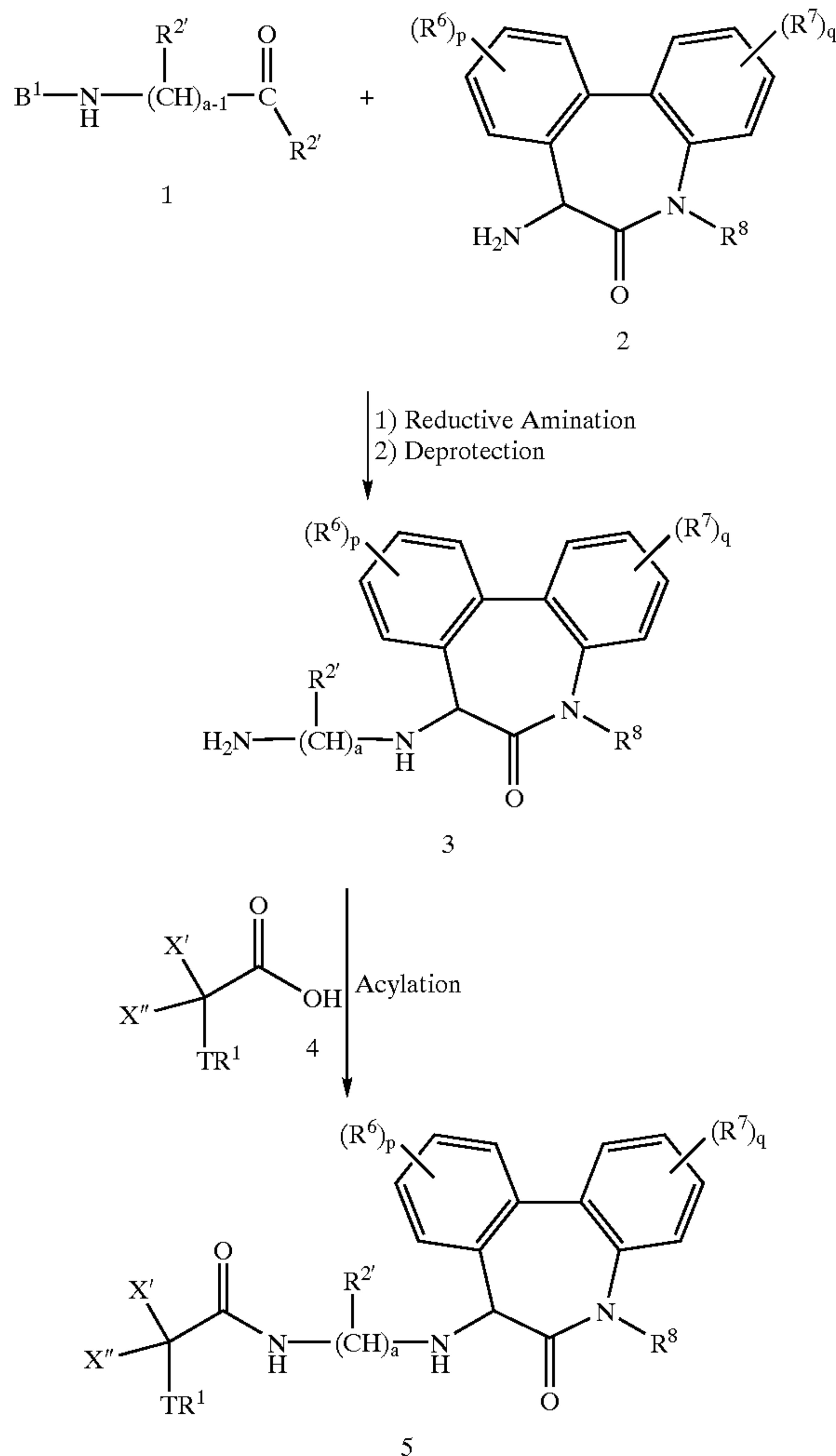
Scheme 1
