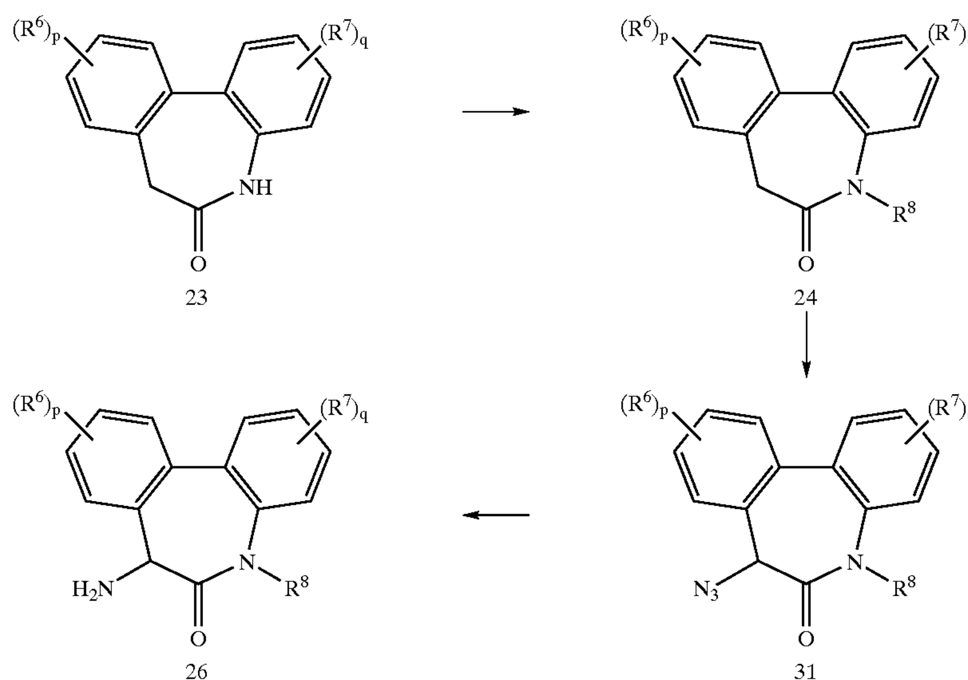
Scheme 9
