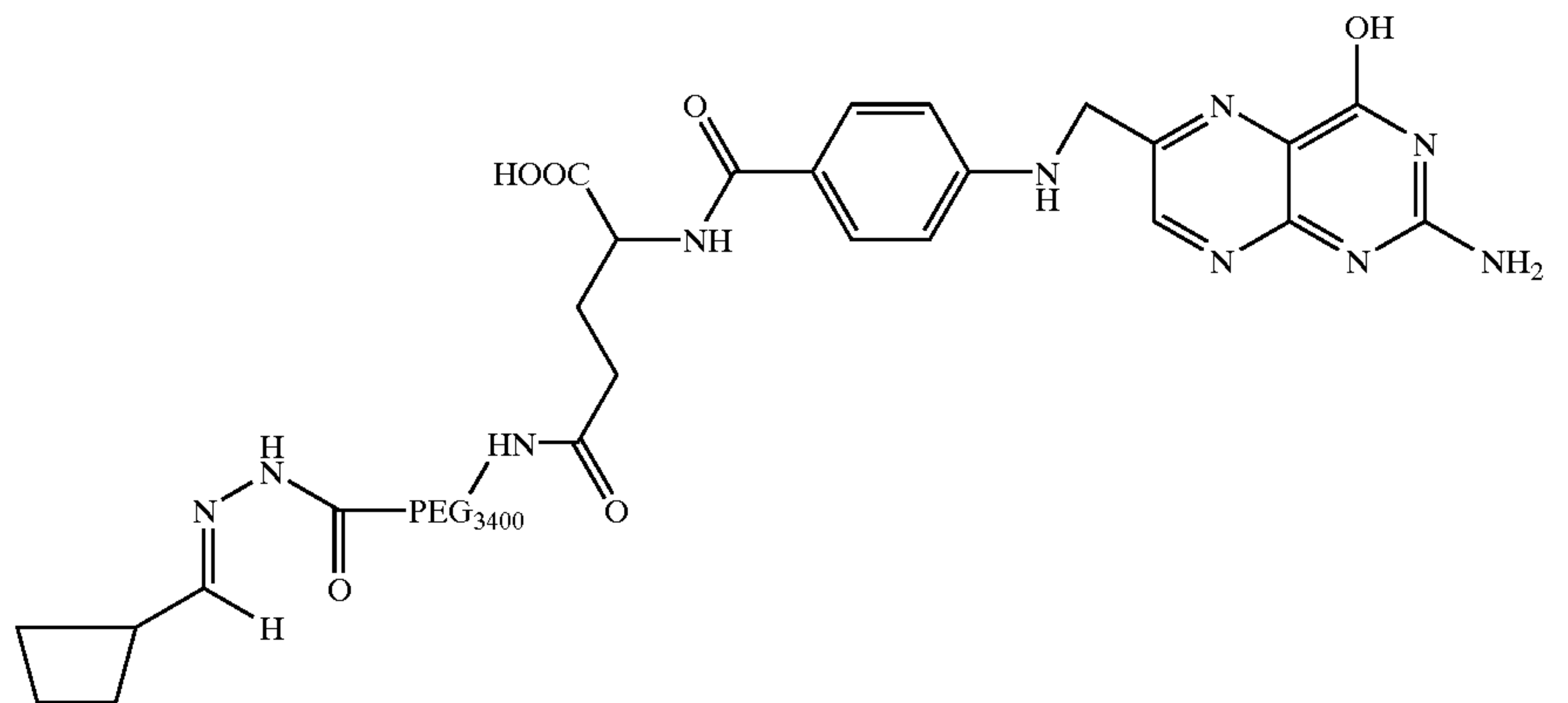
Cyclodextrin-Linker-Folate
