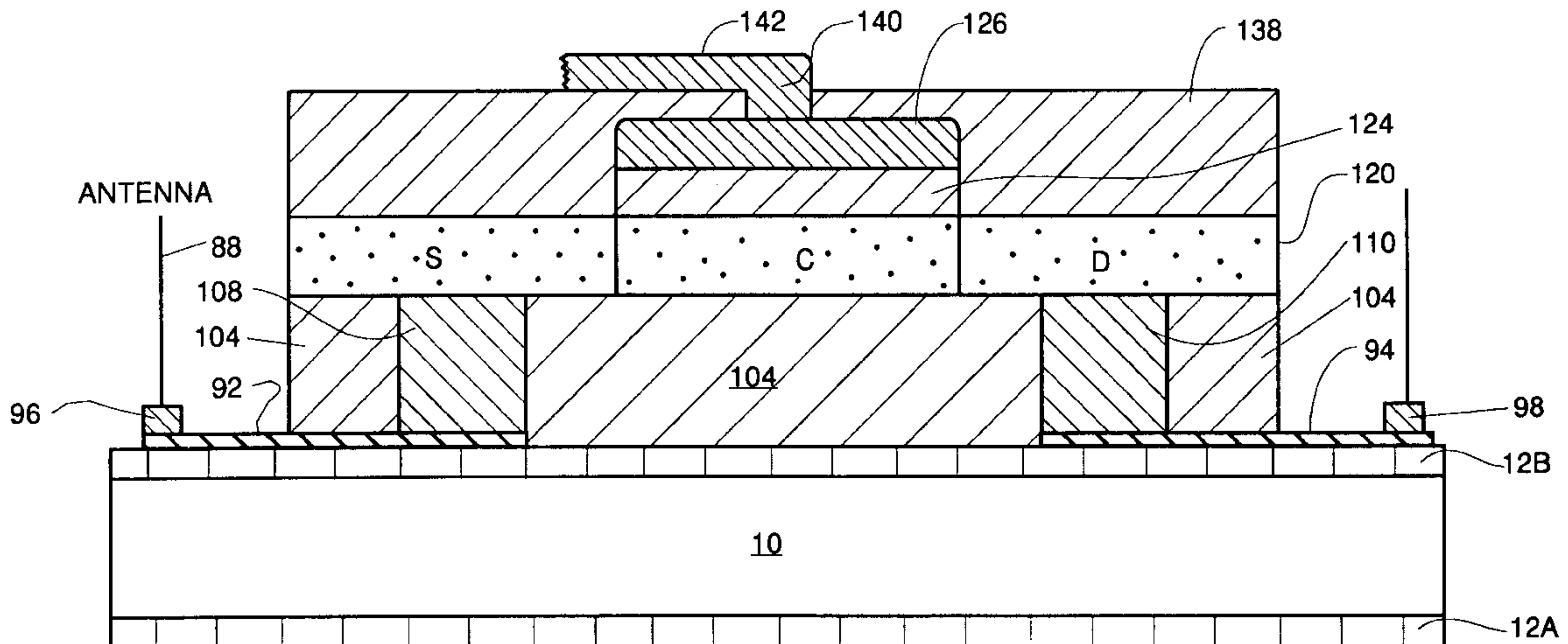
UPSIDE DOWN TRANSISTOR ON TOP OF PRINTED ANTENNA
